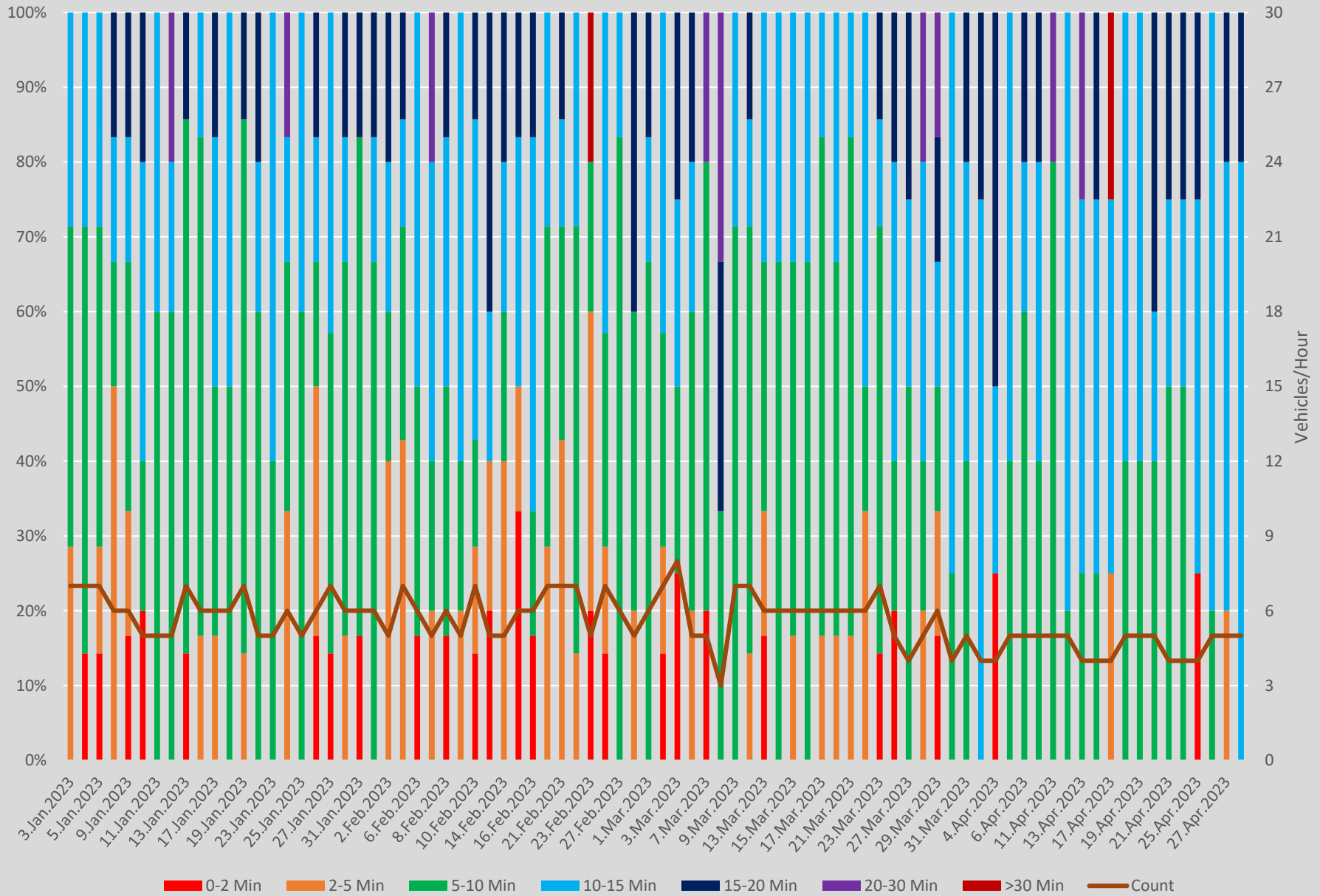
Headway Distributions 935 Jane Express Lawrence Southbound 800 to 900
