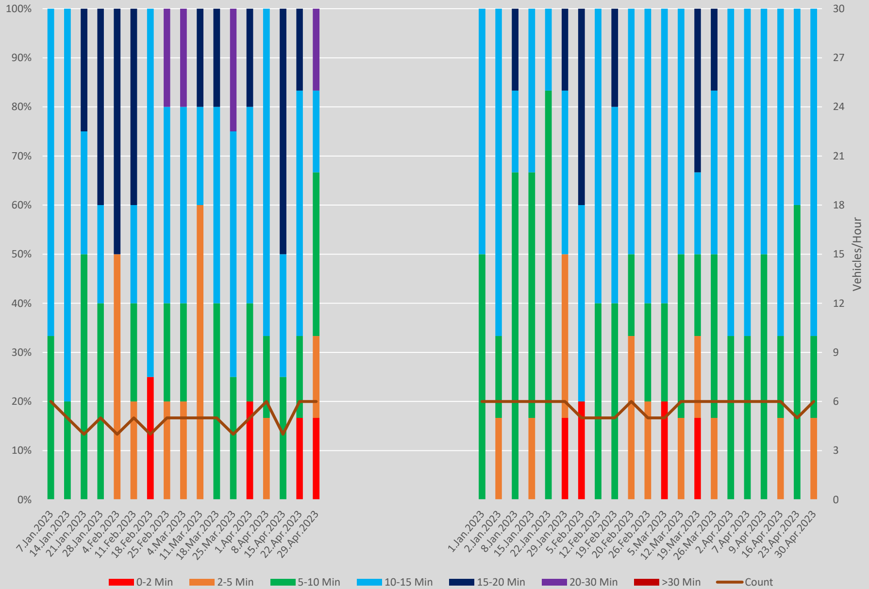
Headway Distributions 935 Jane Express Lawrence Southbound 1000 to 1100 Weekends
