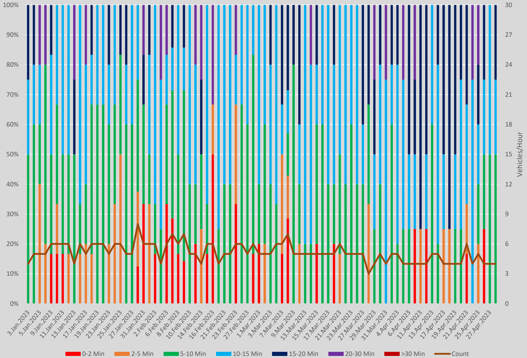
Headway Distributions 935 Jane Express Lawrence Southbound 900 to 1000
