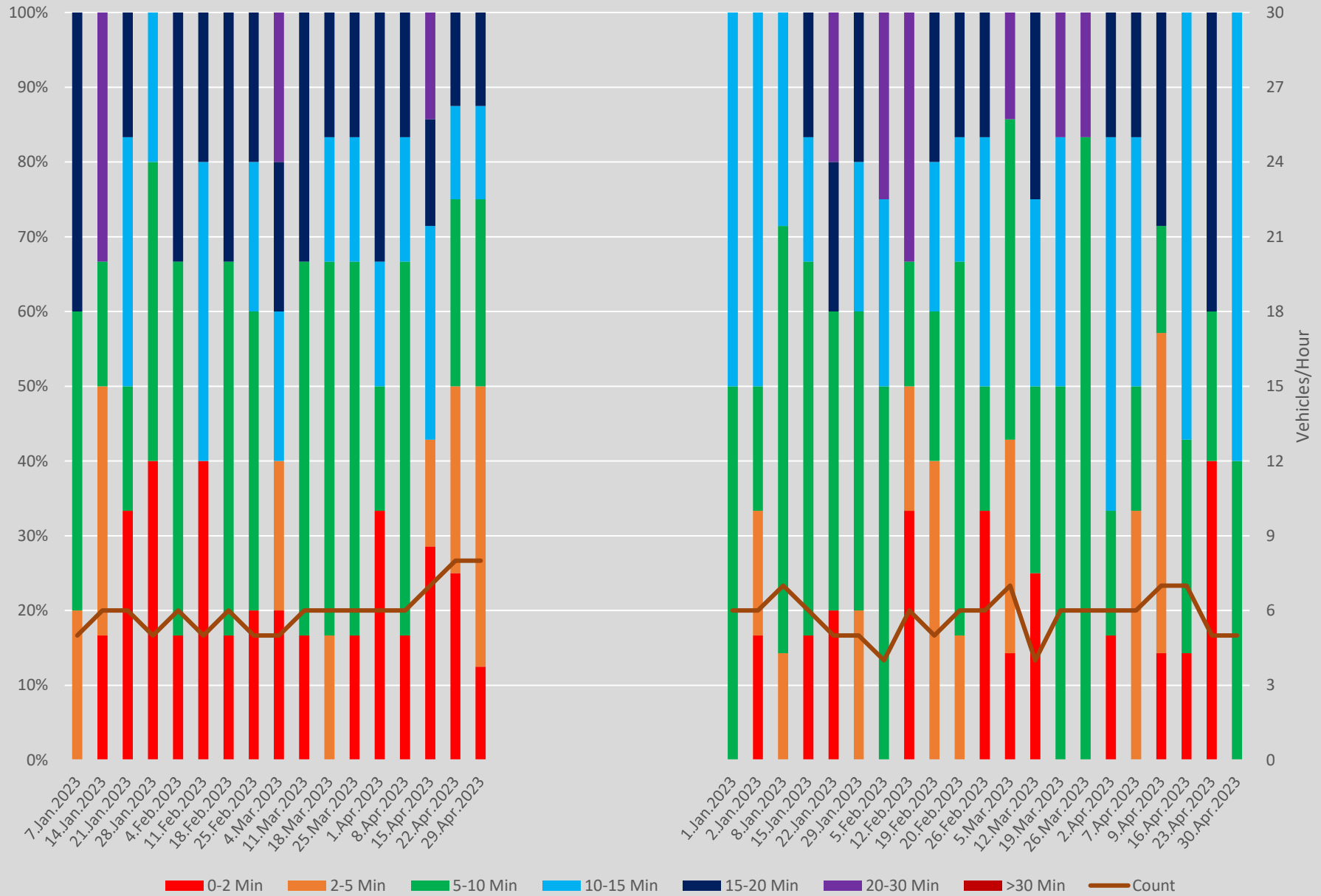
Headway Distributions 935 Jane Express Lawrence Southbound 1400 to 1500 Weekends
