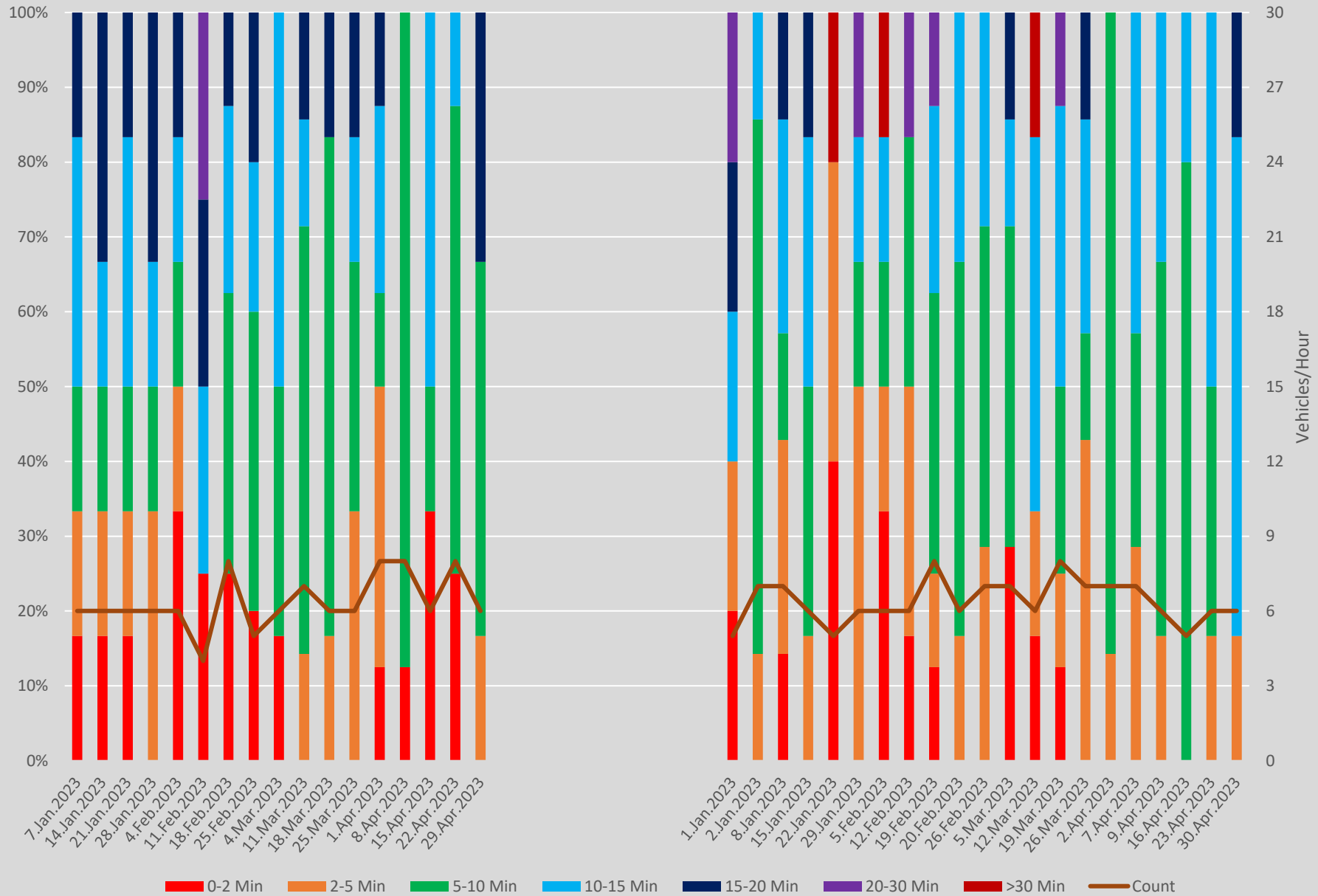
Headway Distributions 935 Jane Express Lawrence Southbound 1800 to 1900 Weekends
