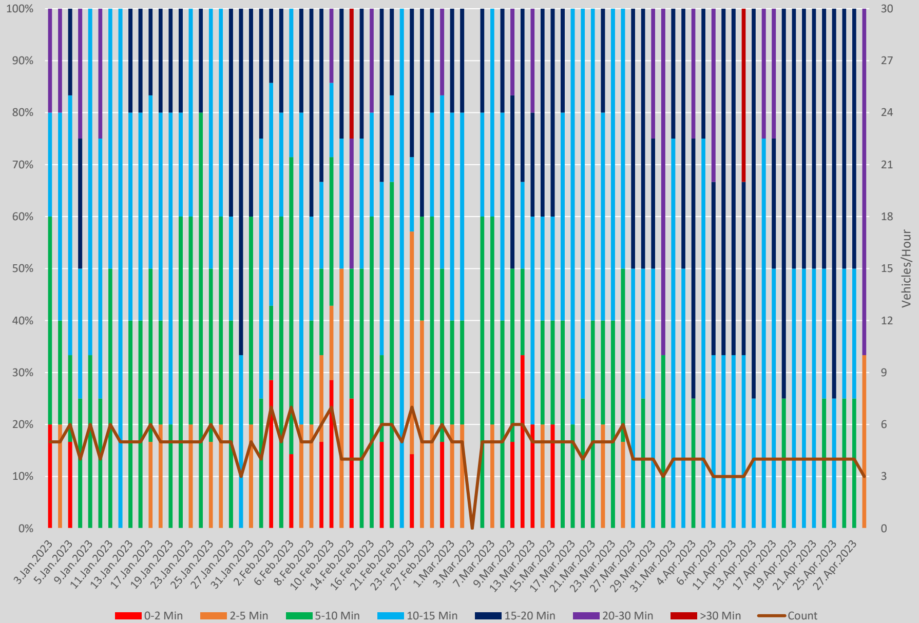
Headway Distributions 935 Jane Express Lawrence Southbound 1200 to 1300
