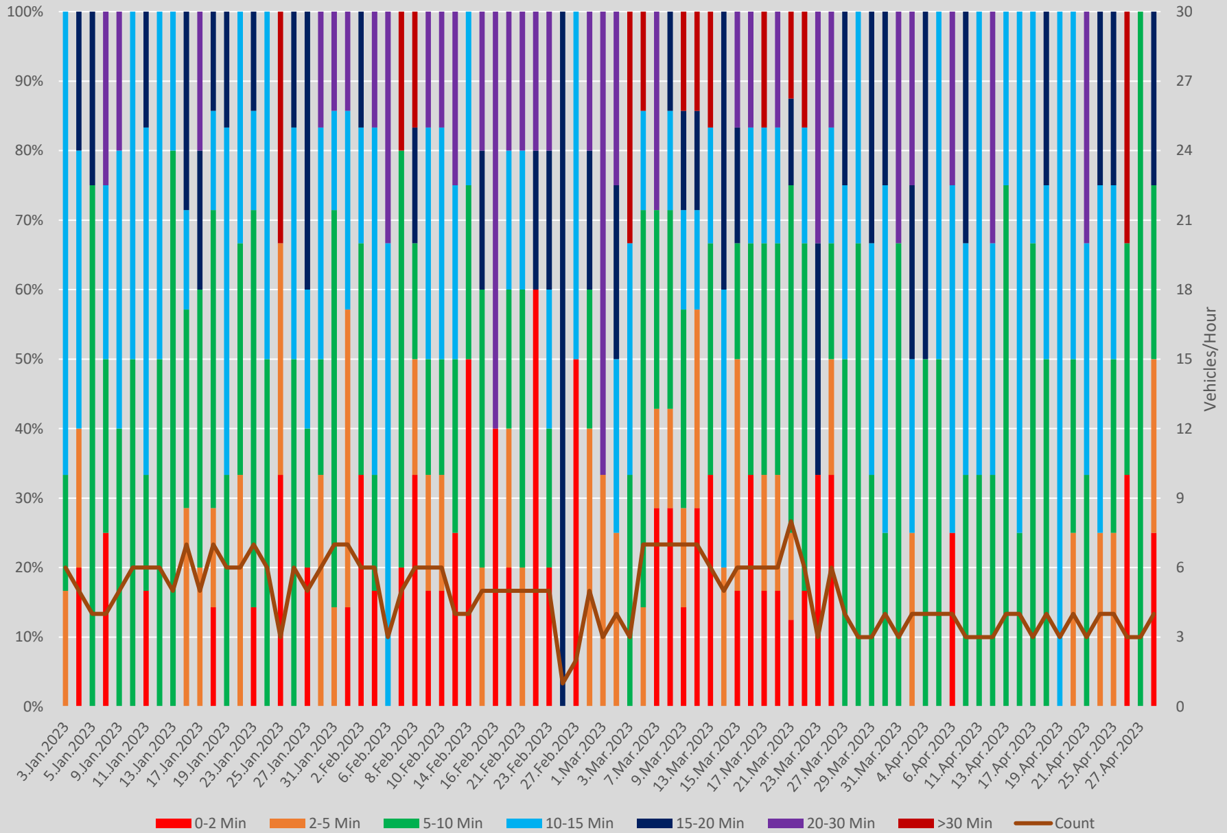
Headway Distributions 935 Jane Express Lawrence Southbound 1900 to 2000
