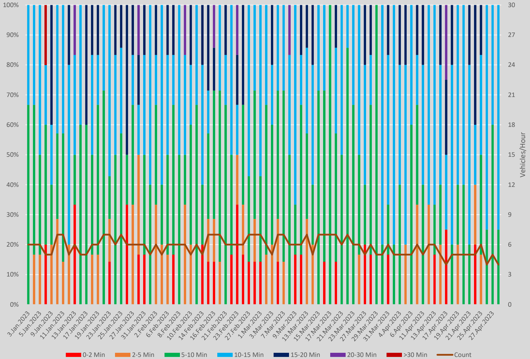
Headway Distributions 935 Jane Express Lawrence Southbound 700 to 800
