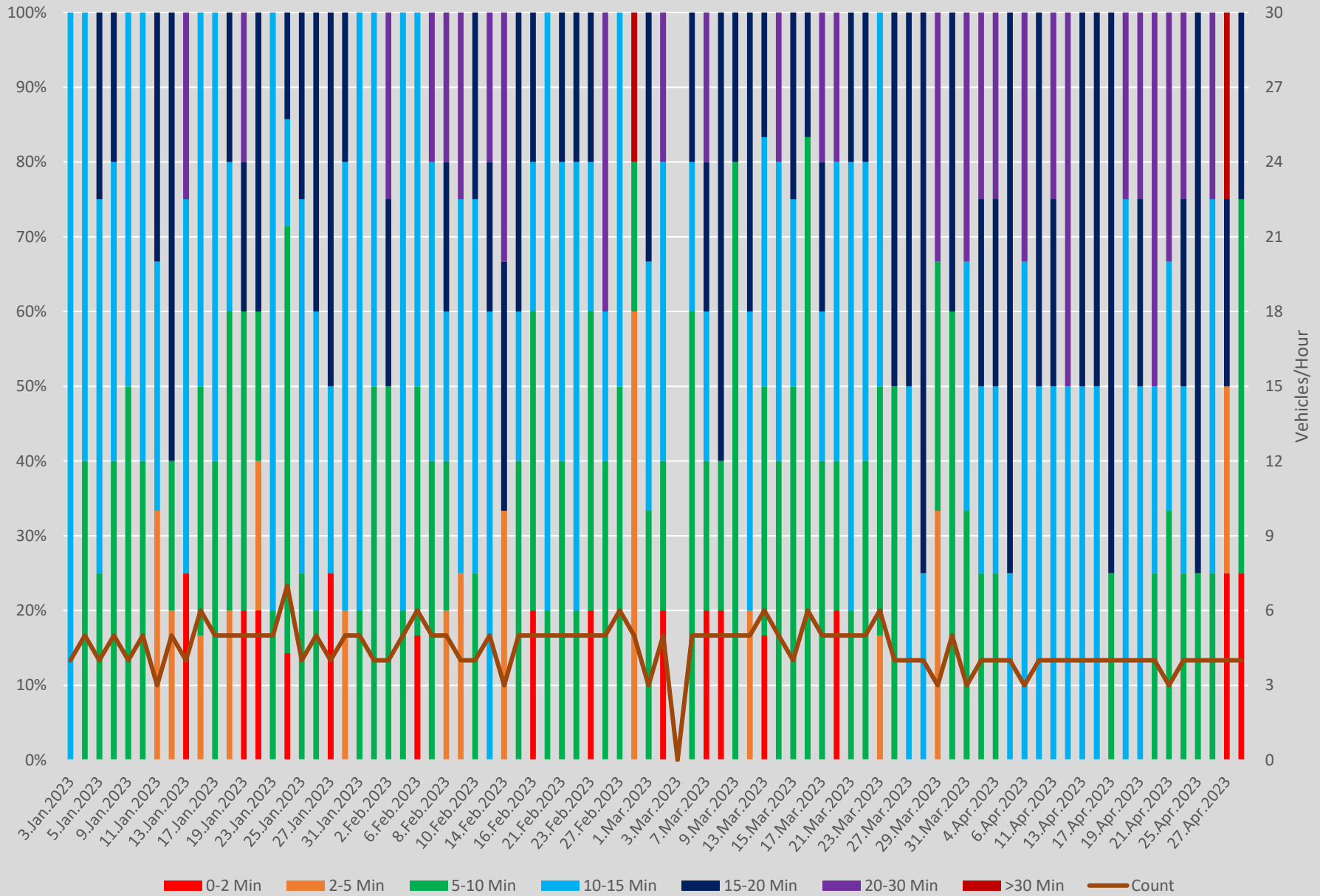
Headway Distributions 935 Jane Express Lawrence Southbound 1300 to 1400
