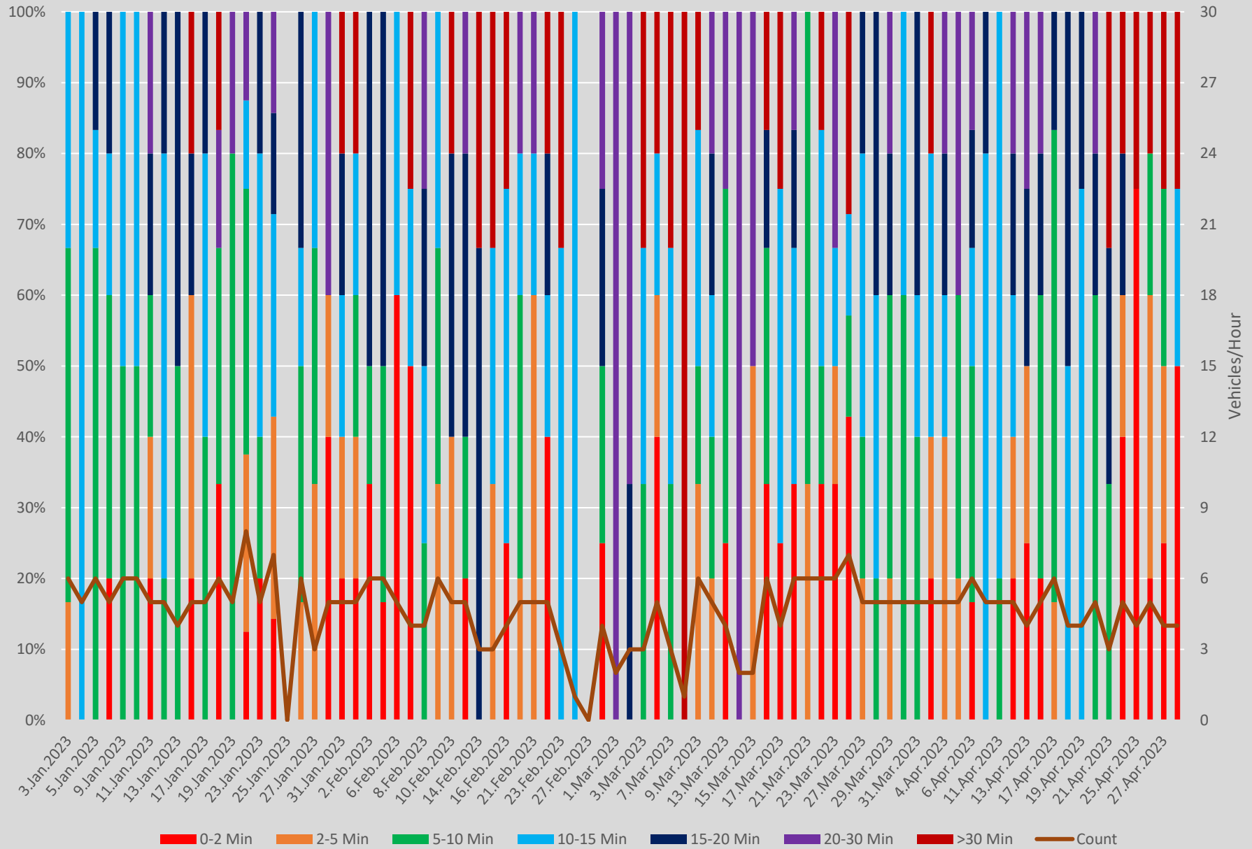
Headway Distributions 935 Jane Express Lawrence Southbound 1700 to 1800
