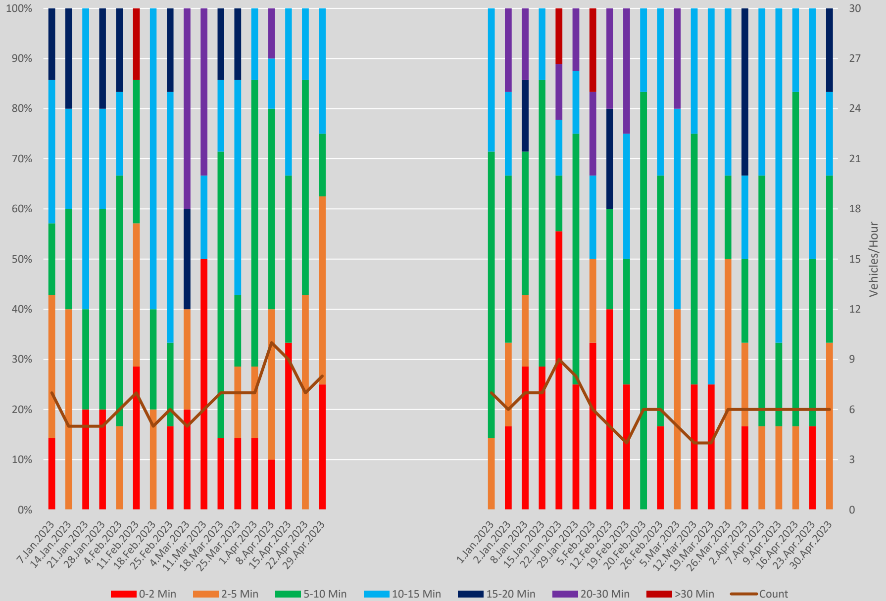
Headway Distributions 935 Jane Express Lawrence Southbound 1700 to 1800 Weekends
