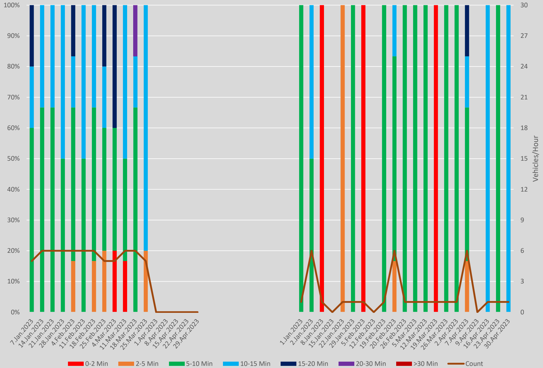
Headway Distributions 935 Jane Express Lawrence Southbound 700 to 800 Weekends
