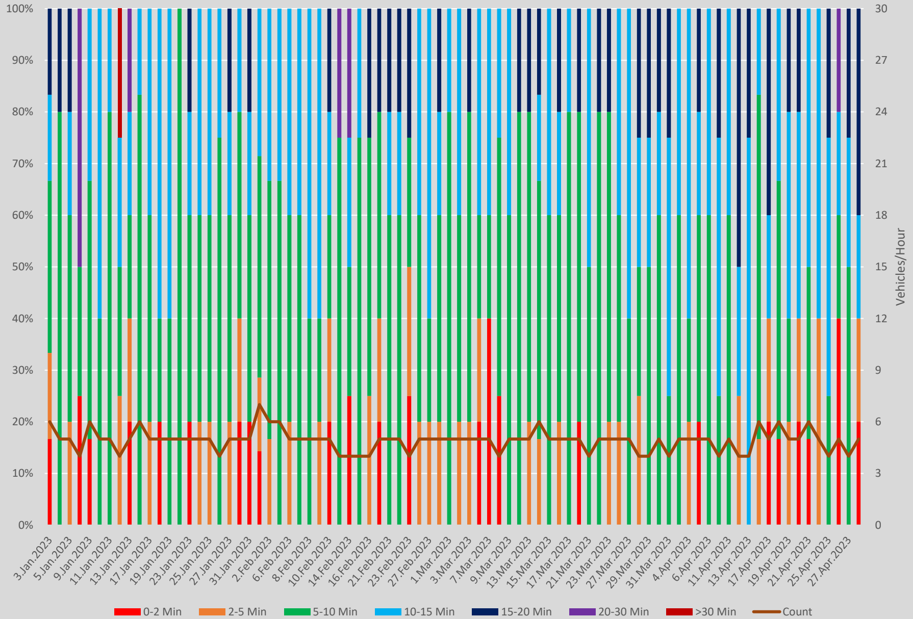
Headway Distributions 935 Jane Express Lawrence Southbound 600 to 700
