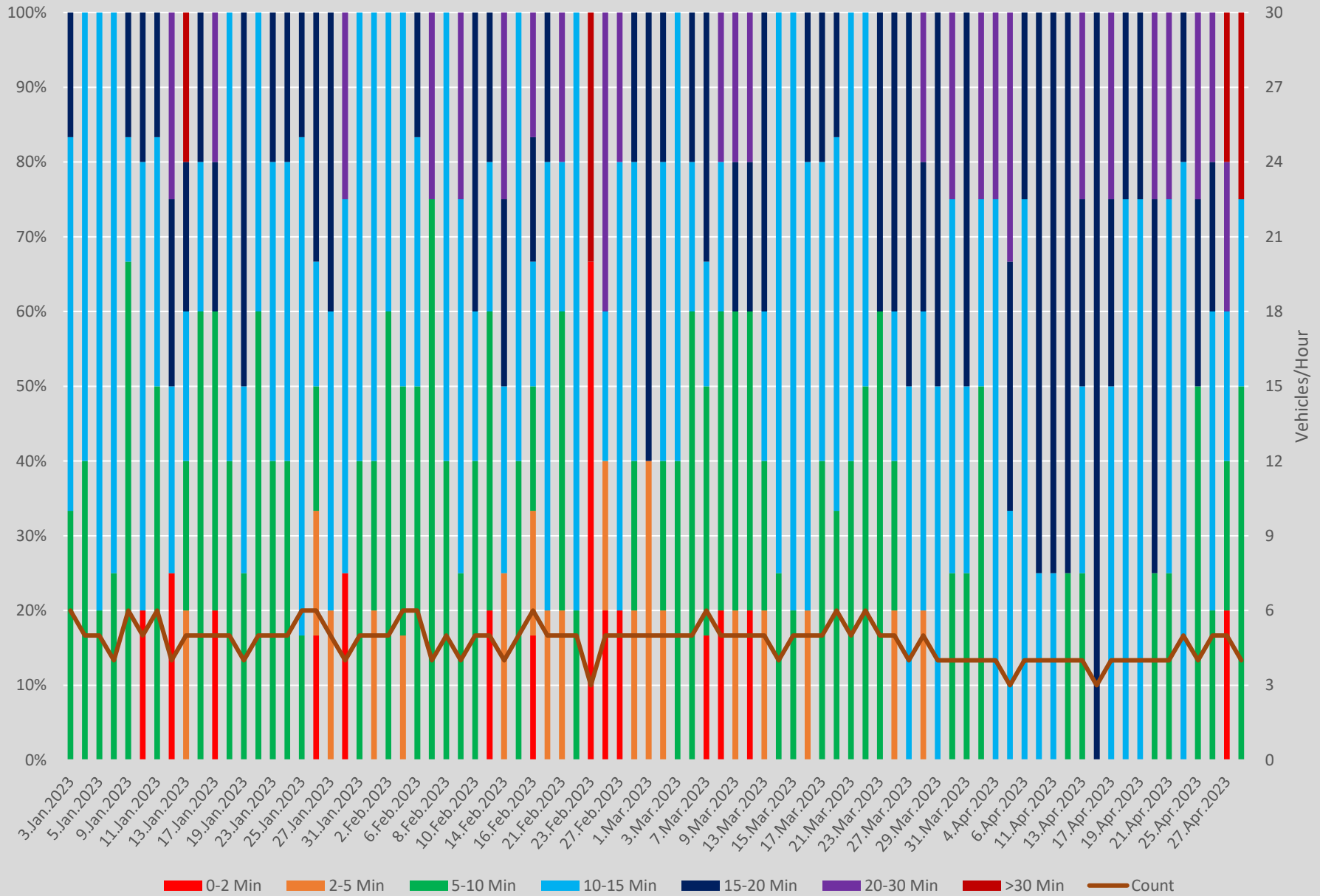
Headway Distributions 935 Jane Express Lawrence Southbound 1000 to 1100
