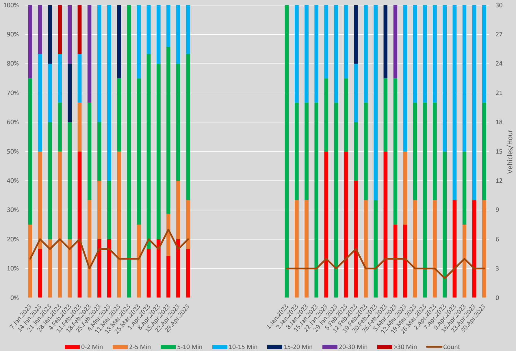
Headway Distributions 935 Jane Express Lawrence Southbound 1900 to 2000 Weekends
