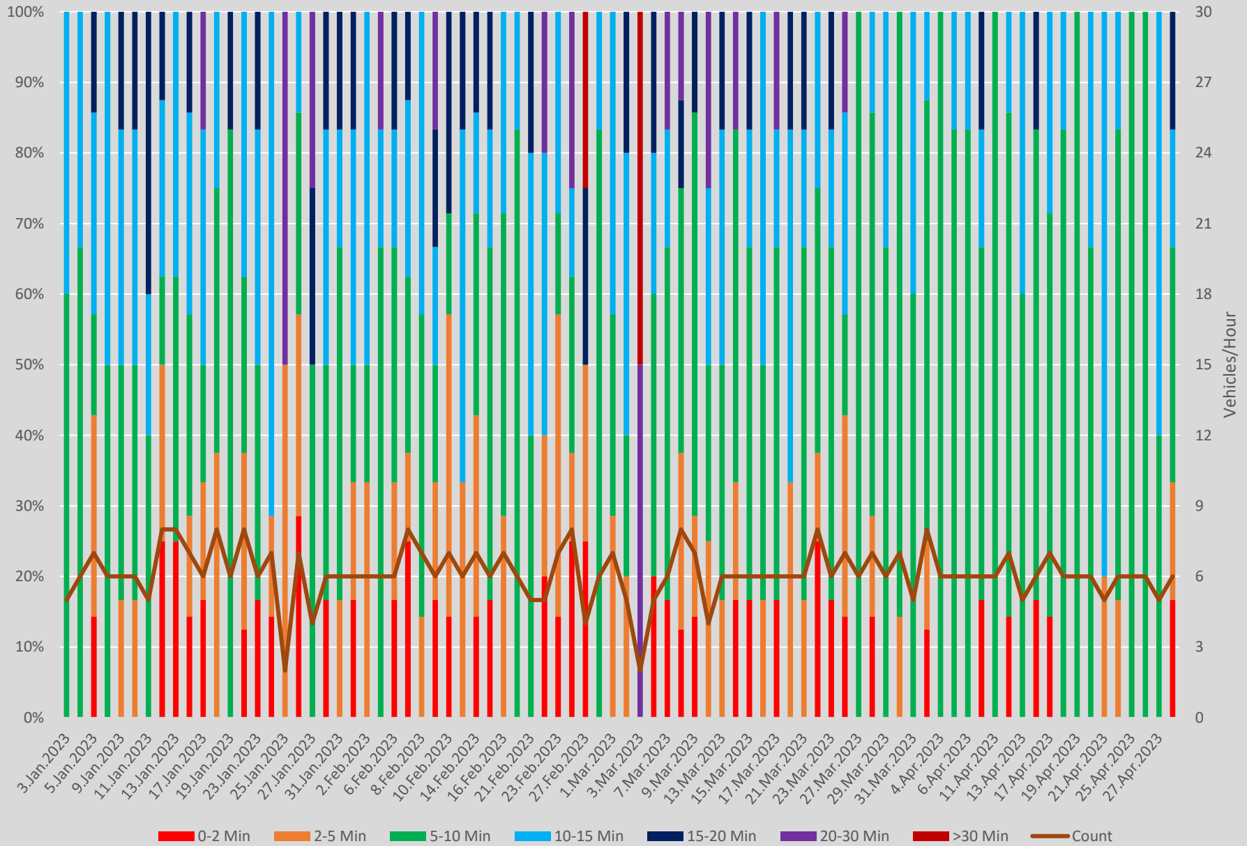
Headway Distributions 86 Scarborough E of Kennedy Stn Eastbound 2100 to 2200
