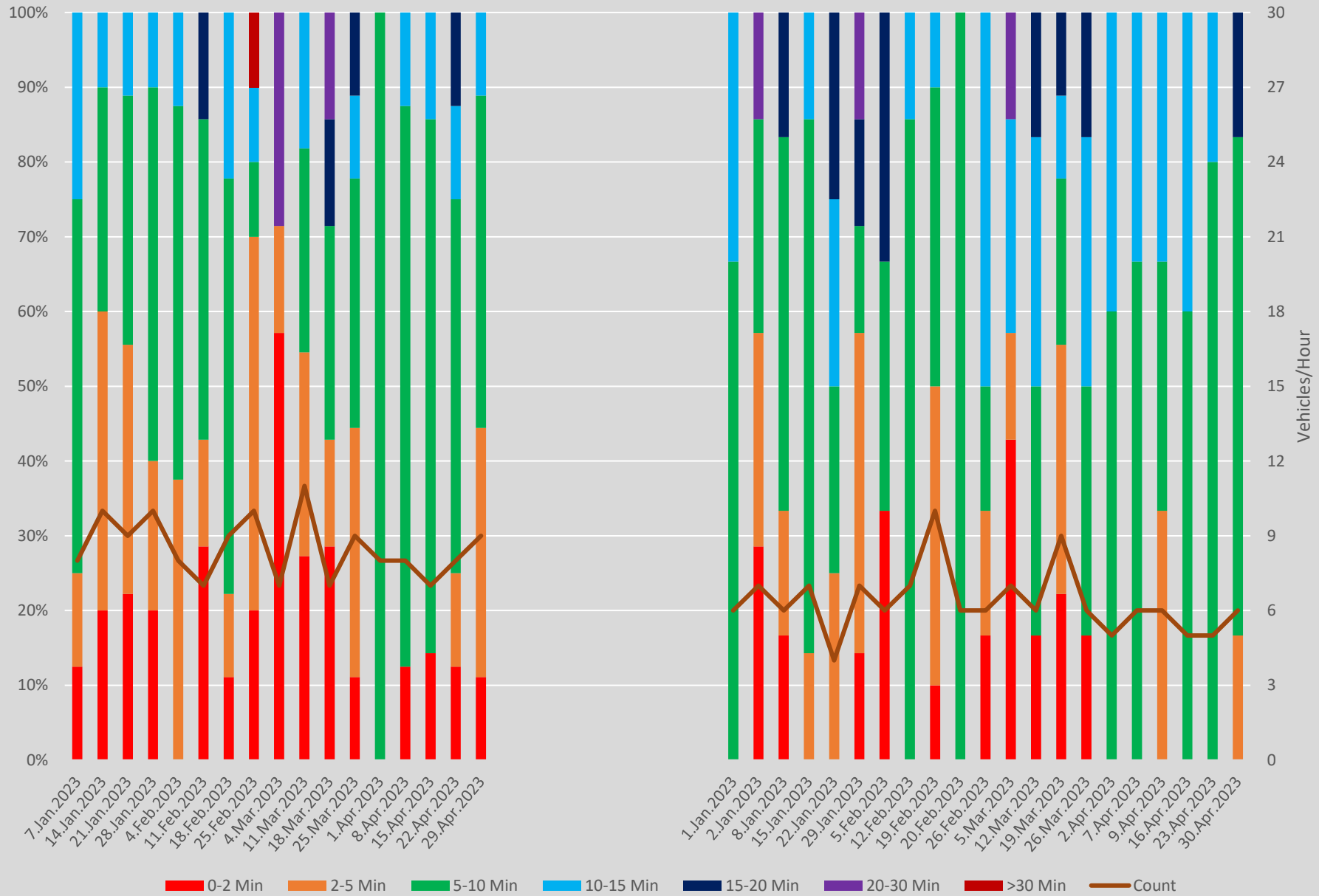
Headway Distributions 86 Scarborough E of Kennedy Stn Eastbound 2100 to 2200 Weekends
