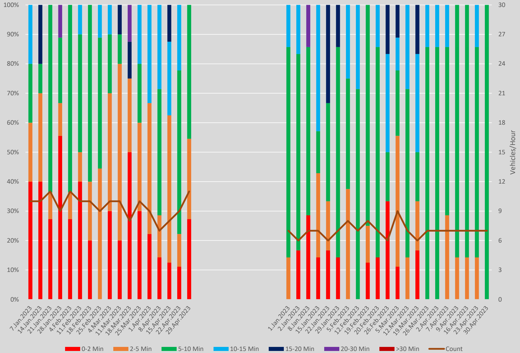
Headway Distributions 86 Scarborough E of Kennedy Stn Eastbound 1600 to 1700 Weekends
