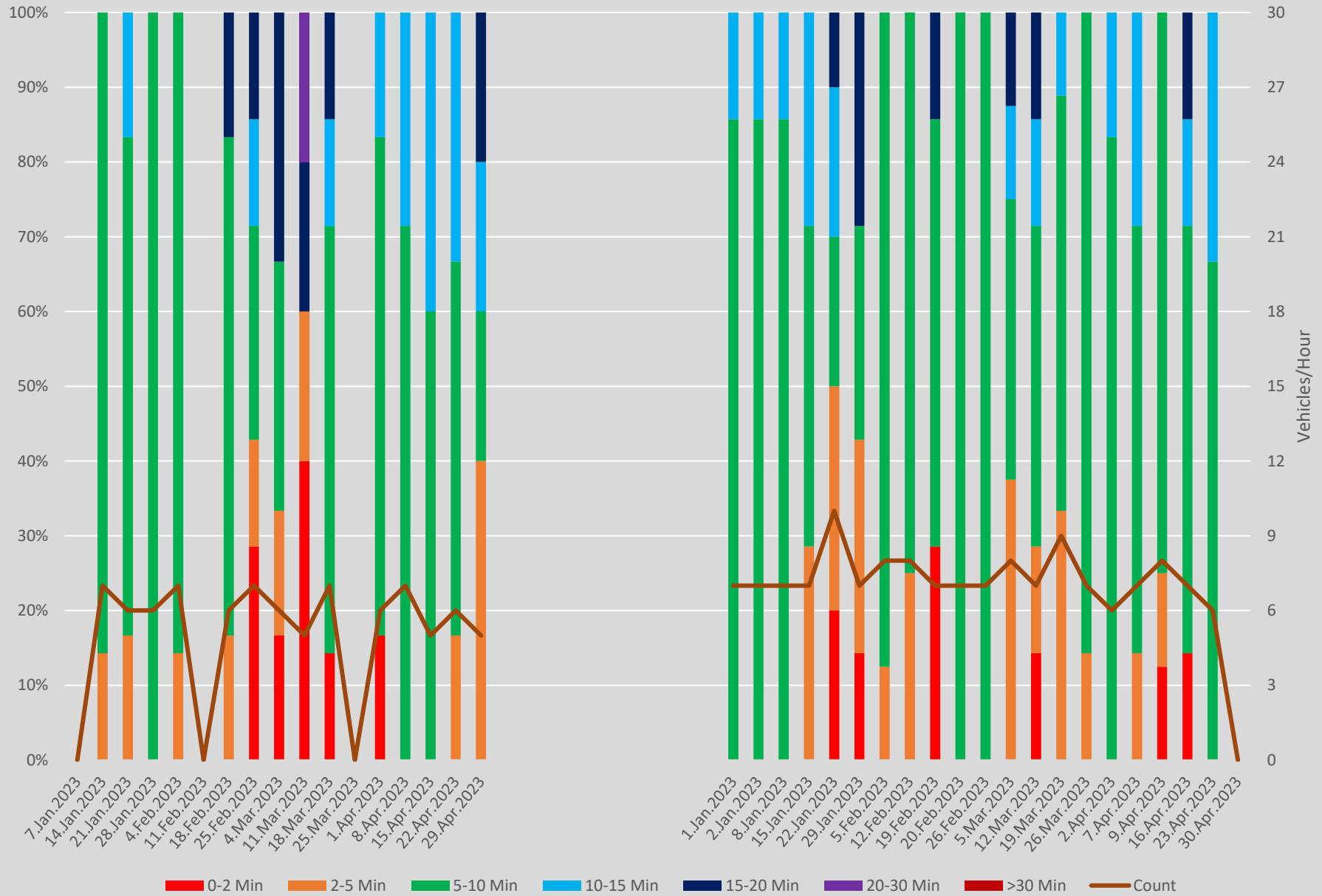
Headway Distributions 86 Scarborough E of Kennedy Stn Eastbound 2400 to 2500 Weekends
