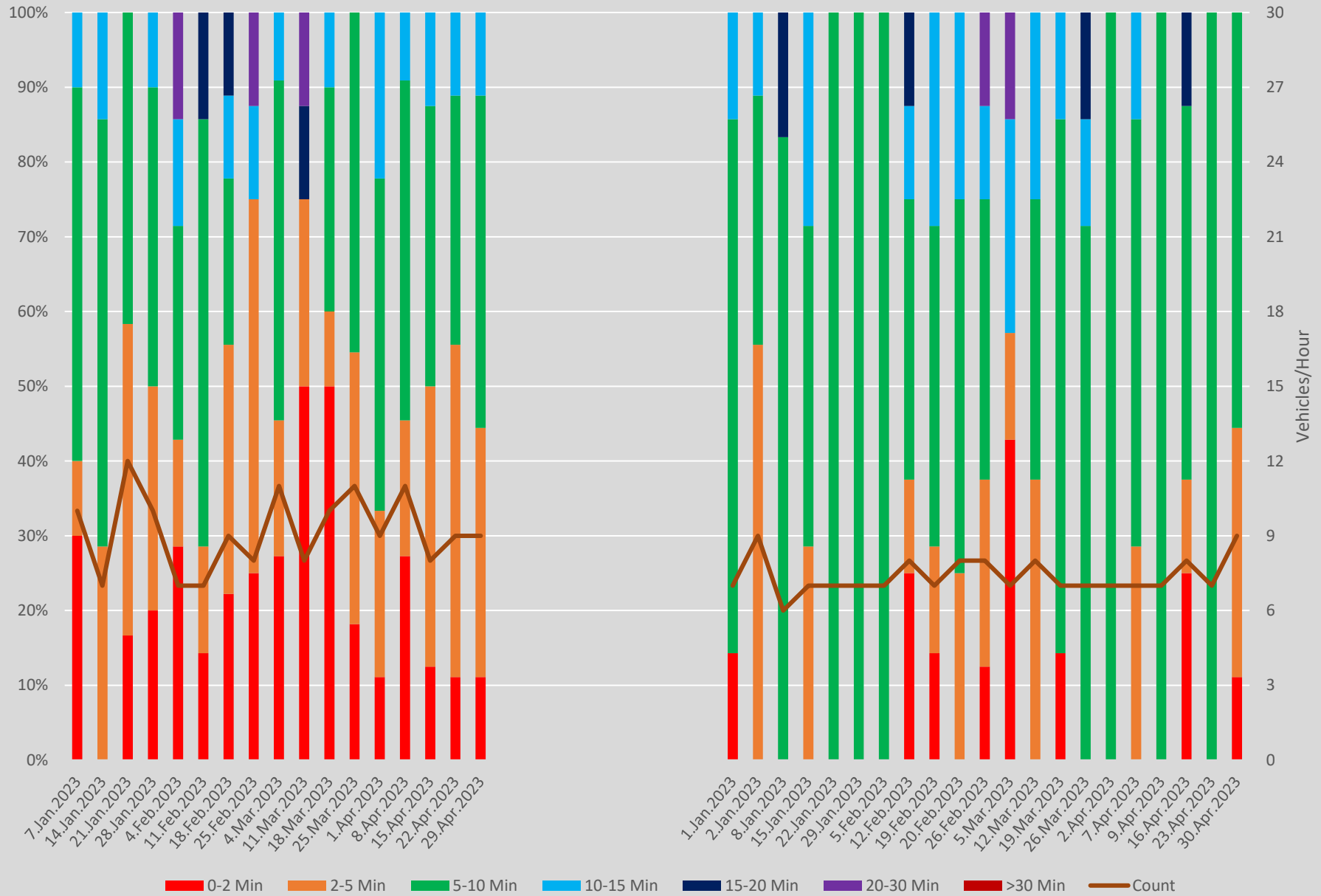
Headway Distributions 86 Scarborough E of Kennedy Stn Eastbound 1200 to 1300 Weekends
