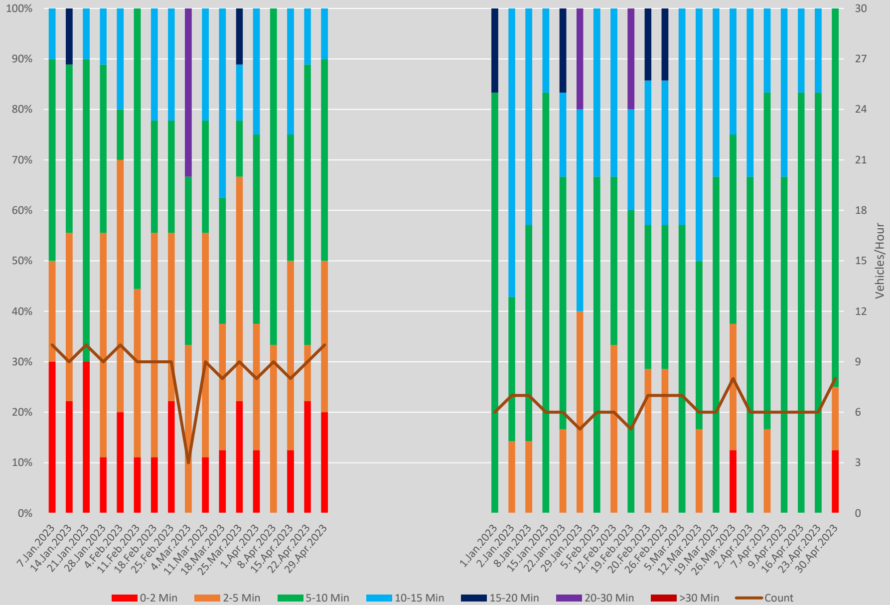
Headway Distributions 86 Scarborough E of Kennedy Stn Eastbound 700 to 800 Weekends
