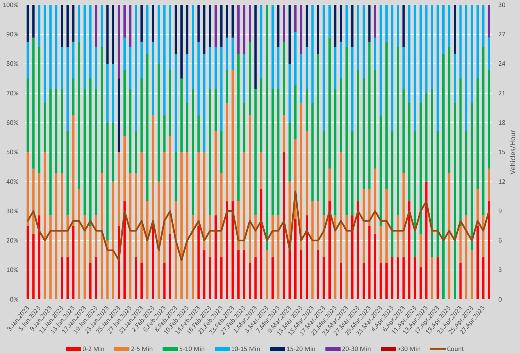
Headway Distributions 86 Scarborough E of Kennedy Stn Eastbound 1900 to 2000
