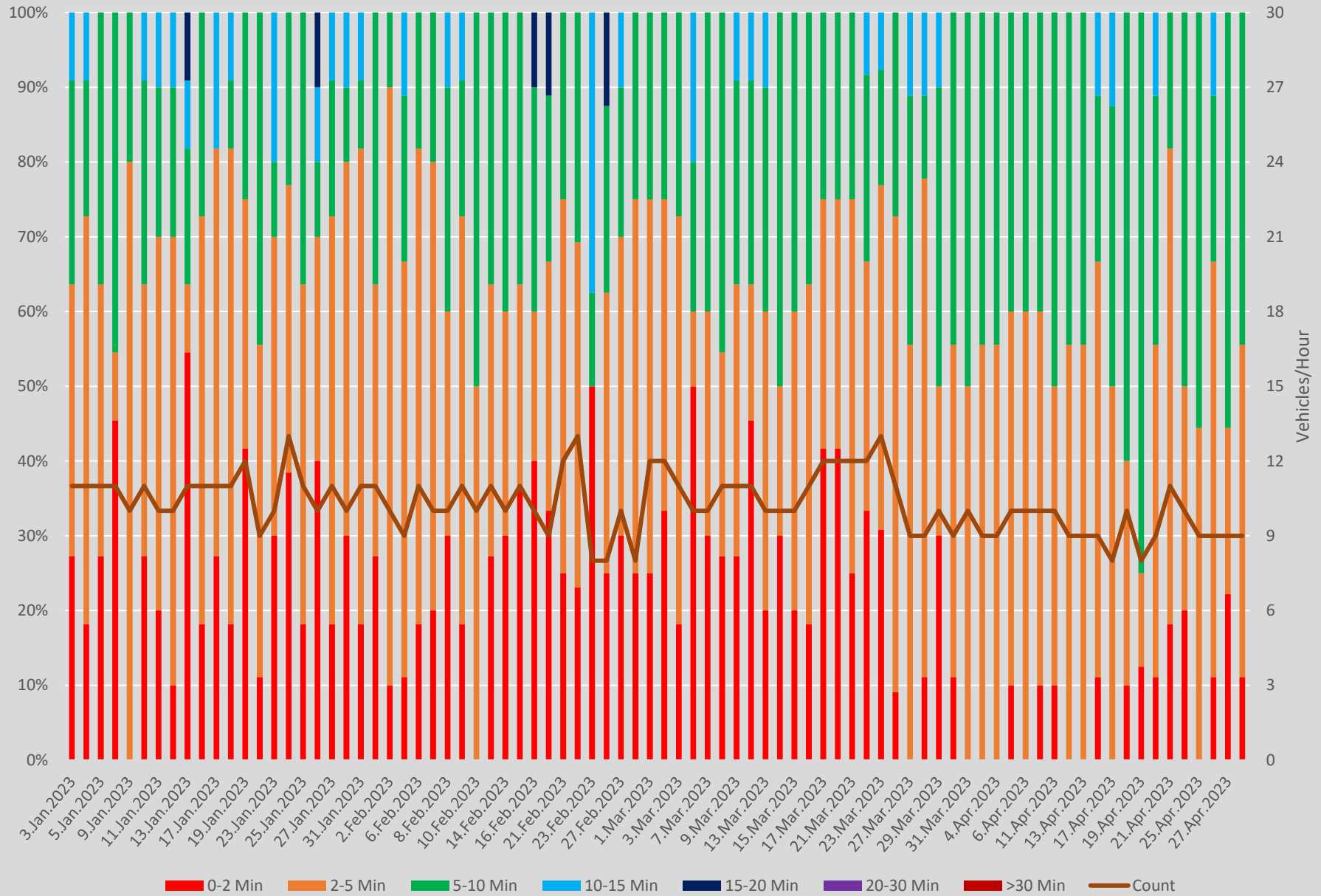
Headway Distributions 86 Scarborough E of Kennedy Stn Eastbound 600 to 700
