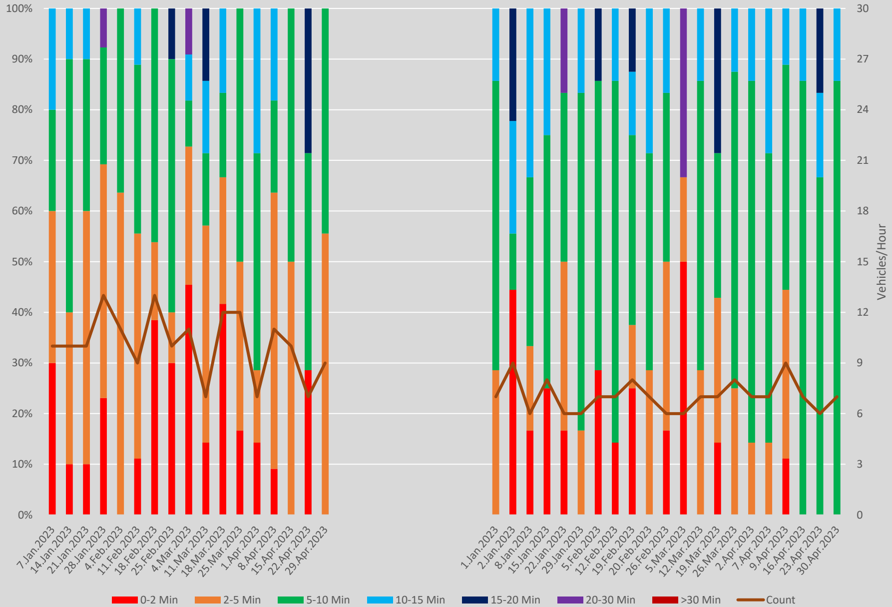
Headway Distributions 86 Scarborough E of Kennedy Stn Eastbound 1700 to 1800 Weekends
