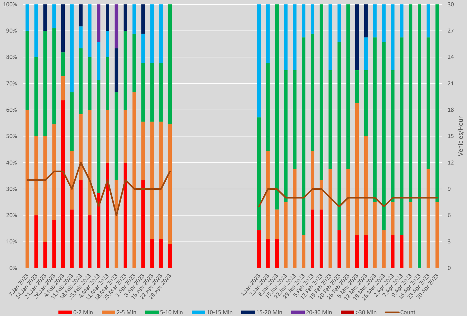
Headway Distributions 86 Scarborough E of Kennedy Stn Eastbound 1100 to 1200 Weekends
