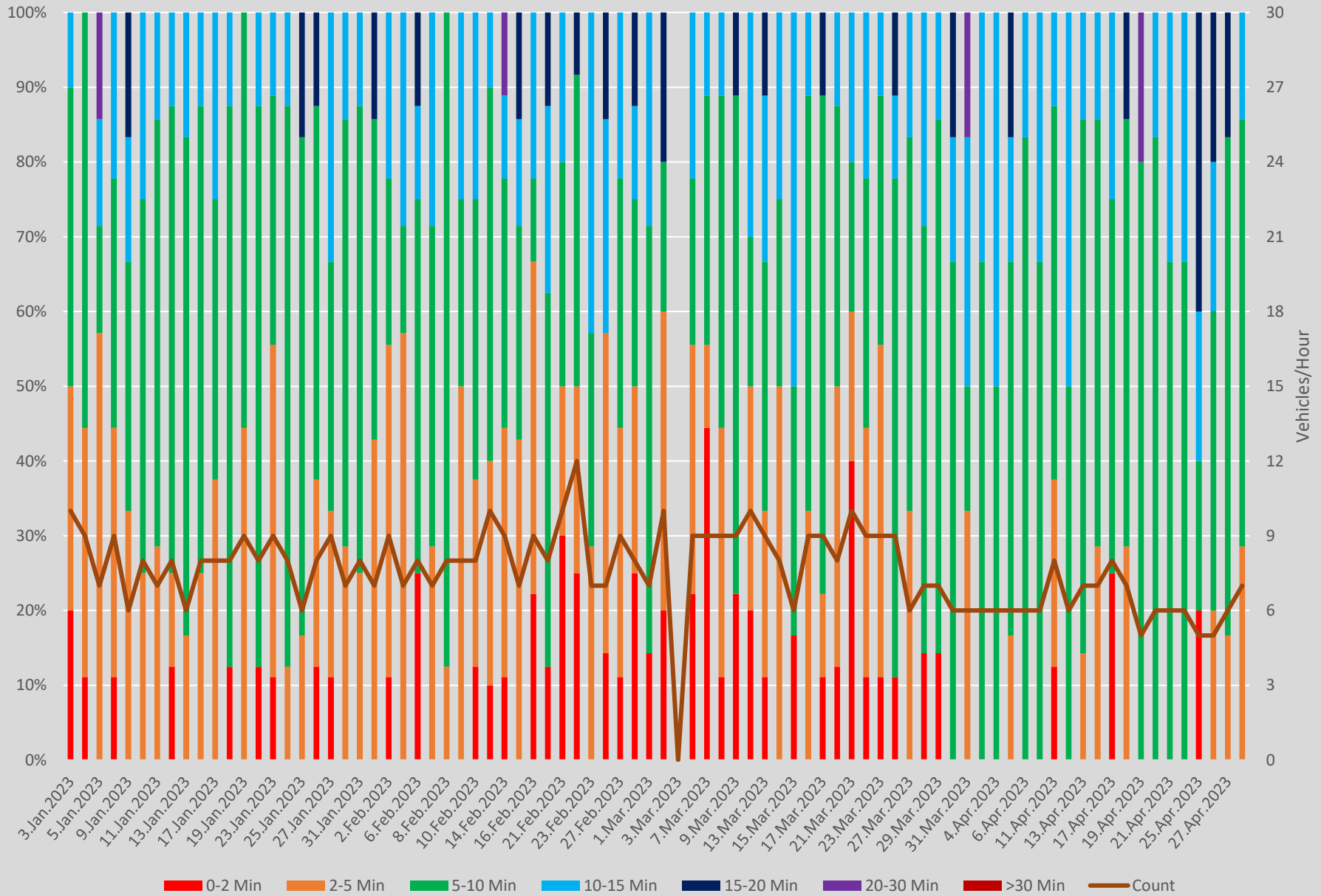
Headway Distributions 86 Scarborough E of Kennedy Stn Eastbound 1200 to 1300
