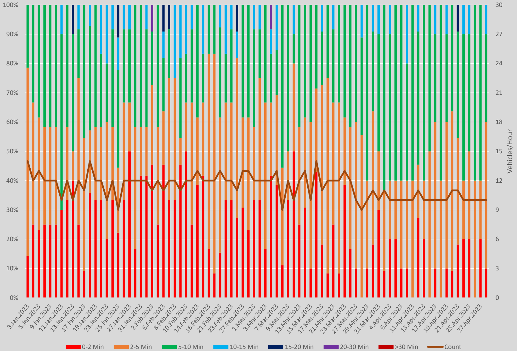
Headway Distributions 86 Scarborough E of Kennedy Stn Eastbound 1700 to 1800
