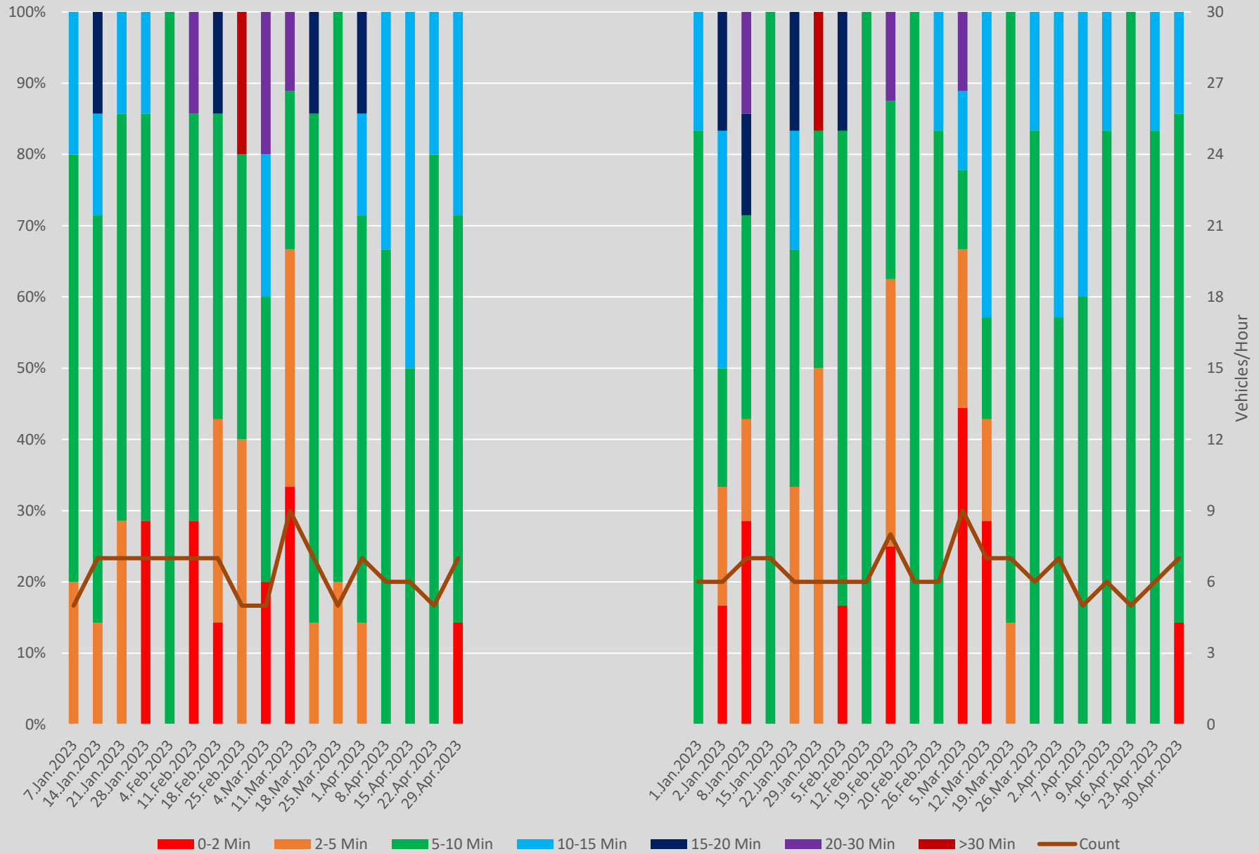
Headway Distributions 86 Scarborough E of Kennedy Stn Eastbound 2300 to 2400 Weekends
