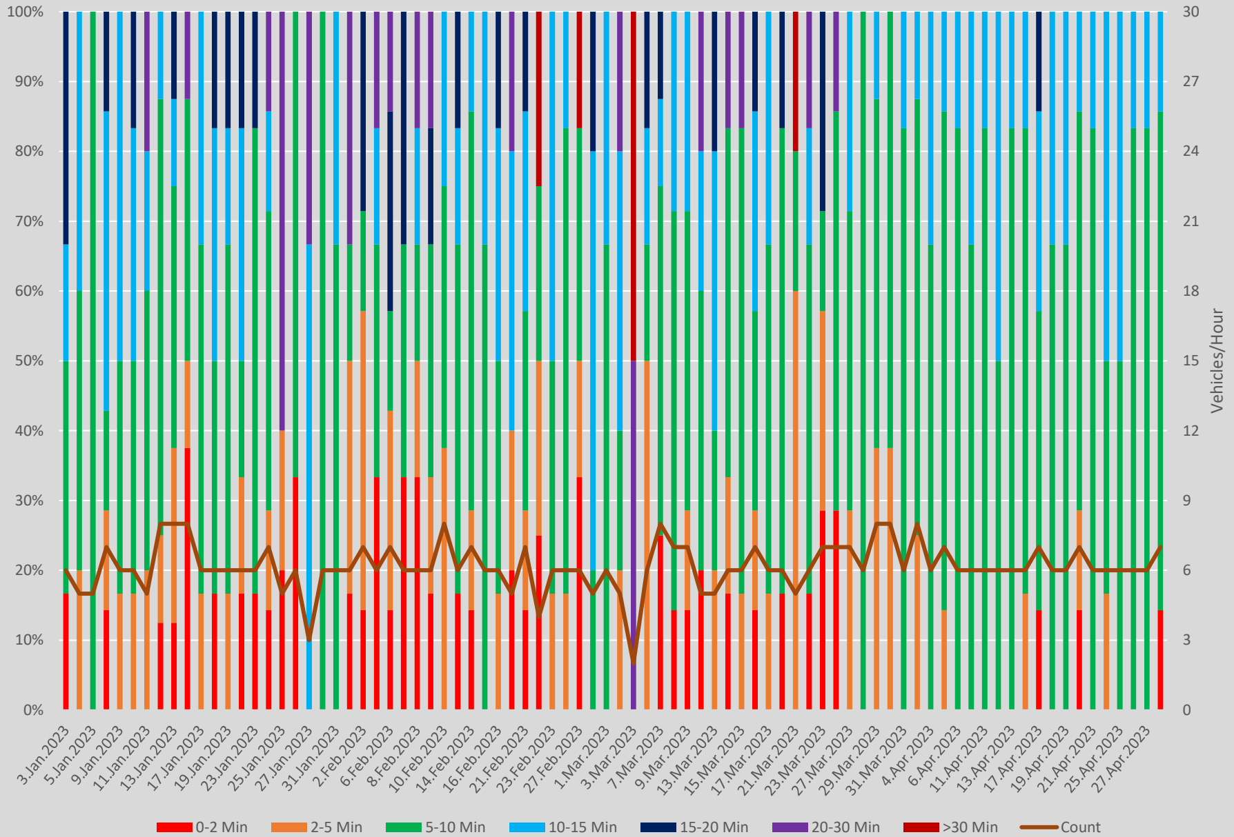
Headway Distributions 86 Scarborough E of Kennedy Stn Eastbound 2300 to 2400
