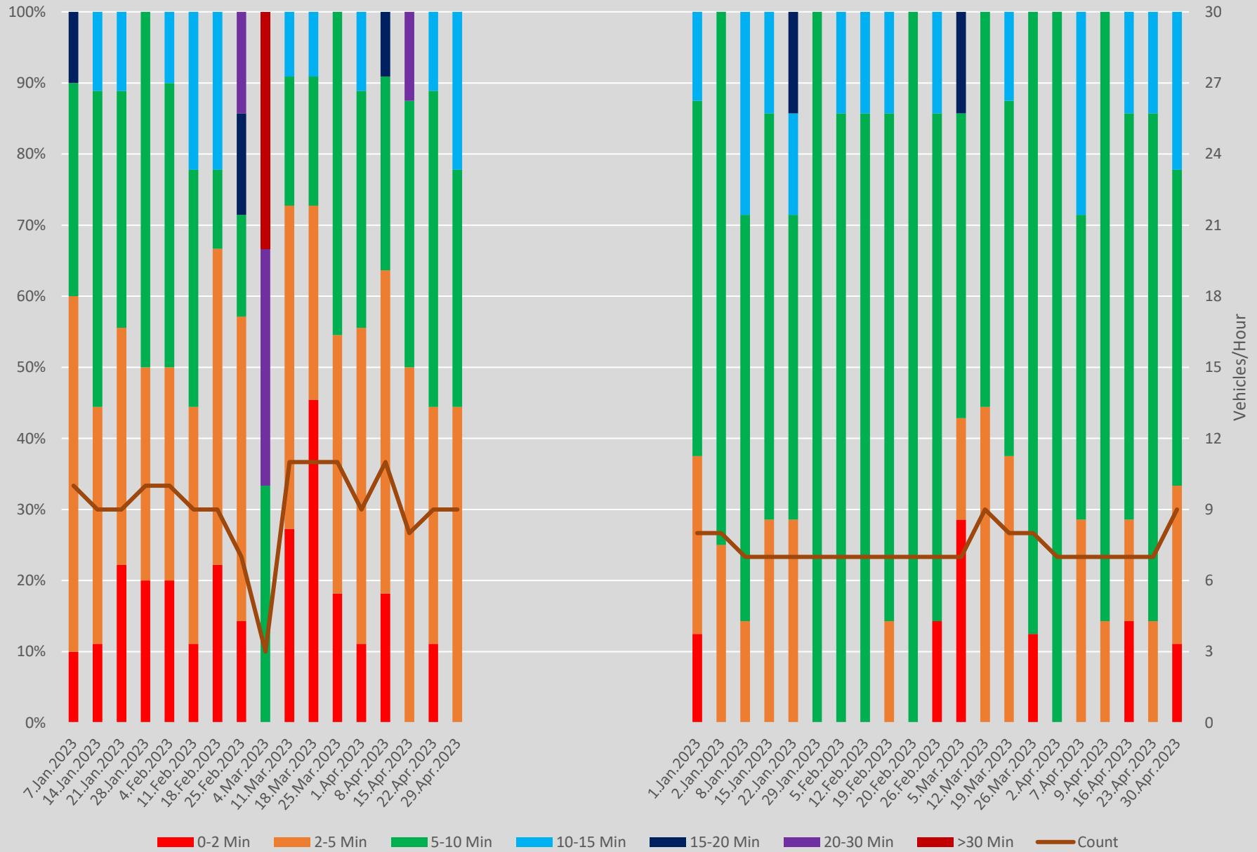
Headway Distributions 86 Scarborough E of Kennedy Stn Eastbound 1000 to 1100 Weekends
