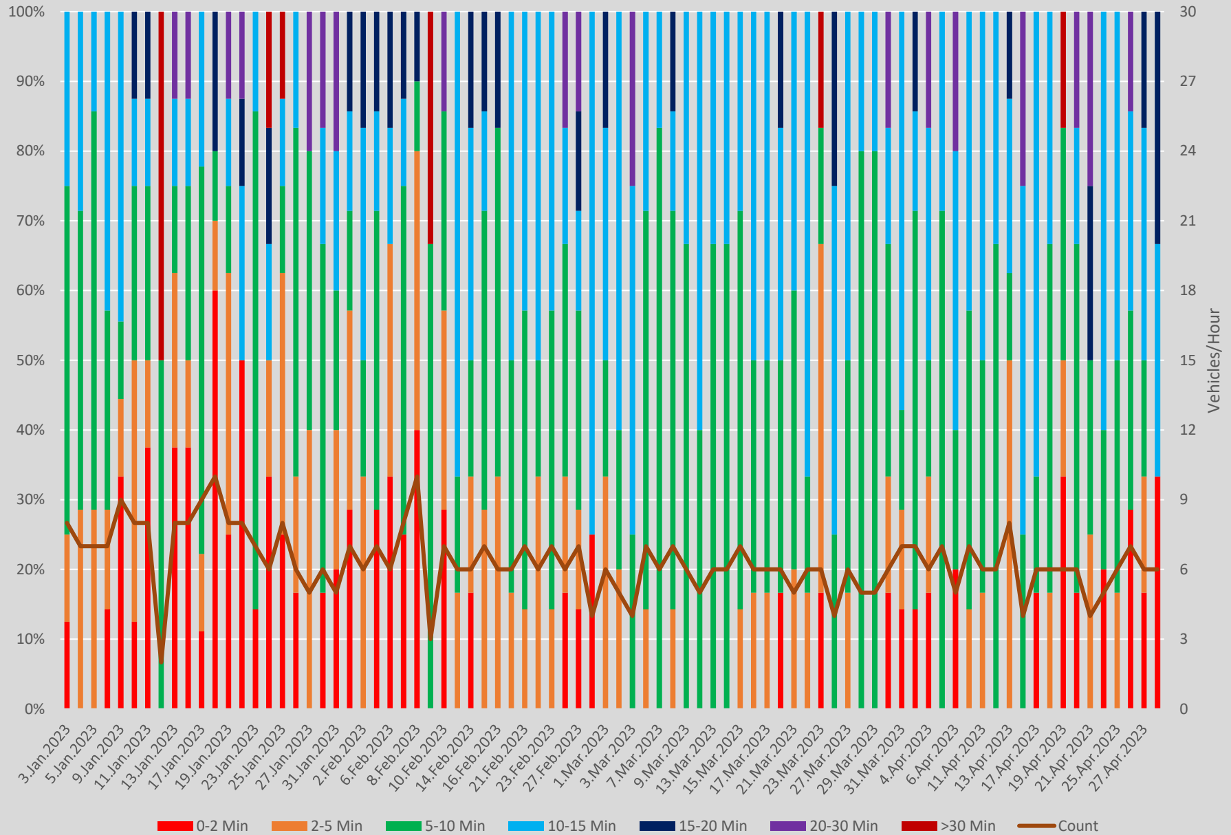
Headway Distributions 505 Dundas Yonge Westbound 2000 to 2100
