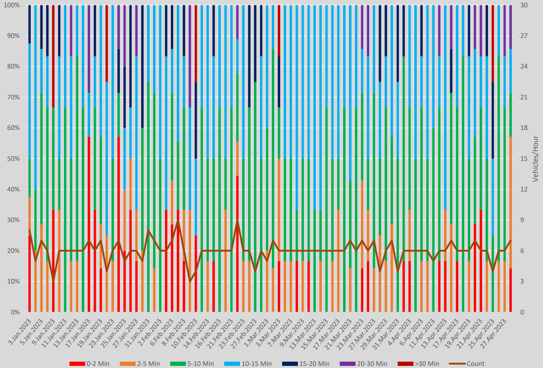
Headway Distributions 505 Dundas Yonge Westbound 2300 to 2400
