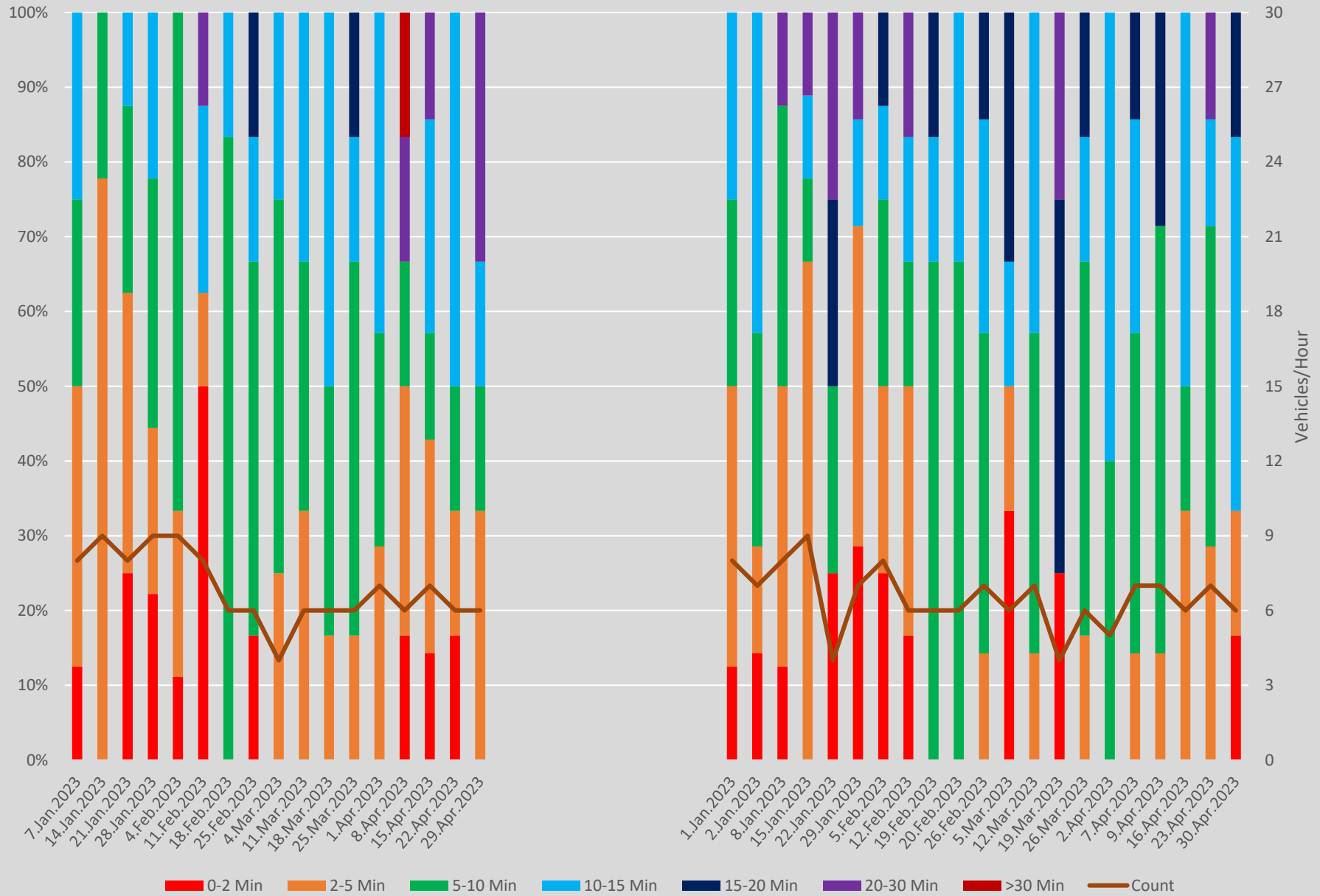
Headway Distributions 505 Dundas Yonge Westbound 1500 to 1600 Weekends
