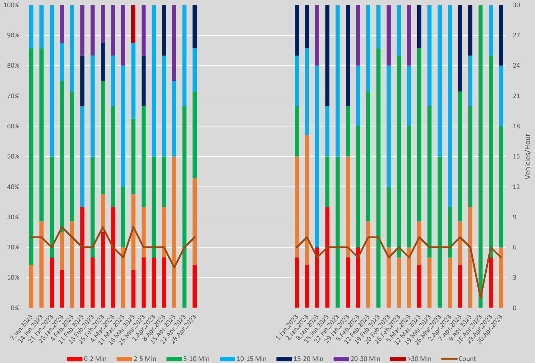
Headway Distributions 505 Dundas Yonge Westbound 2300 to 2400 Weekends
