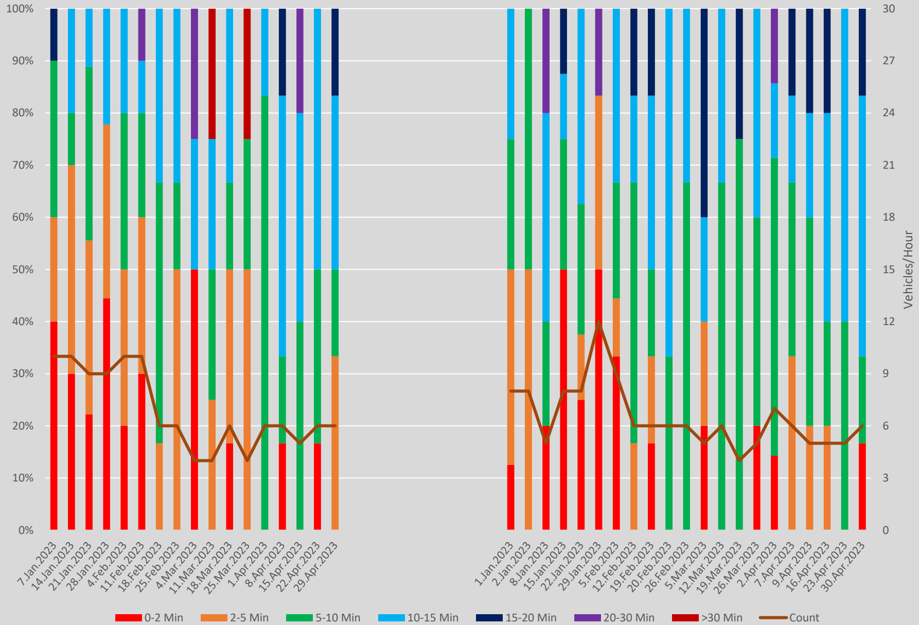
Headway Distributions 505 Dundas Yonge Westbound 1200 to 1300 Weekends
