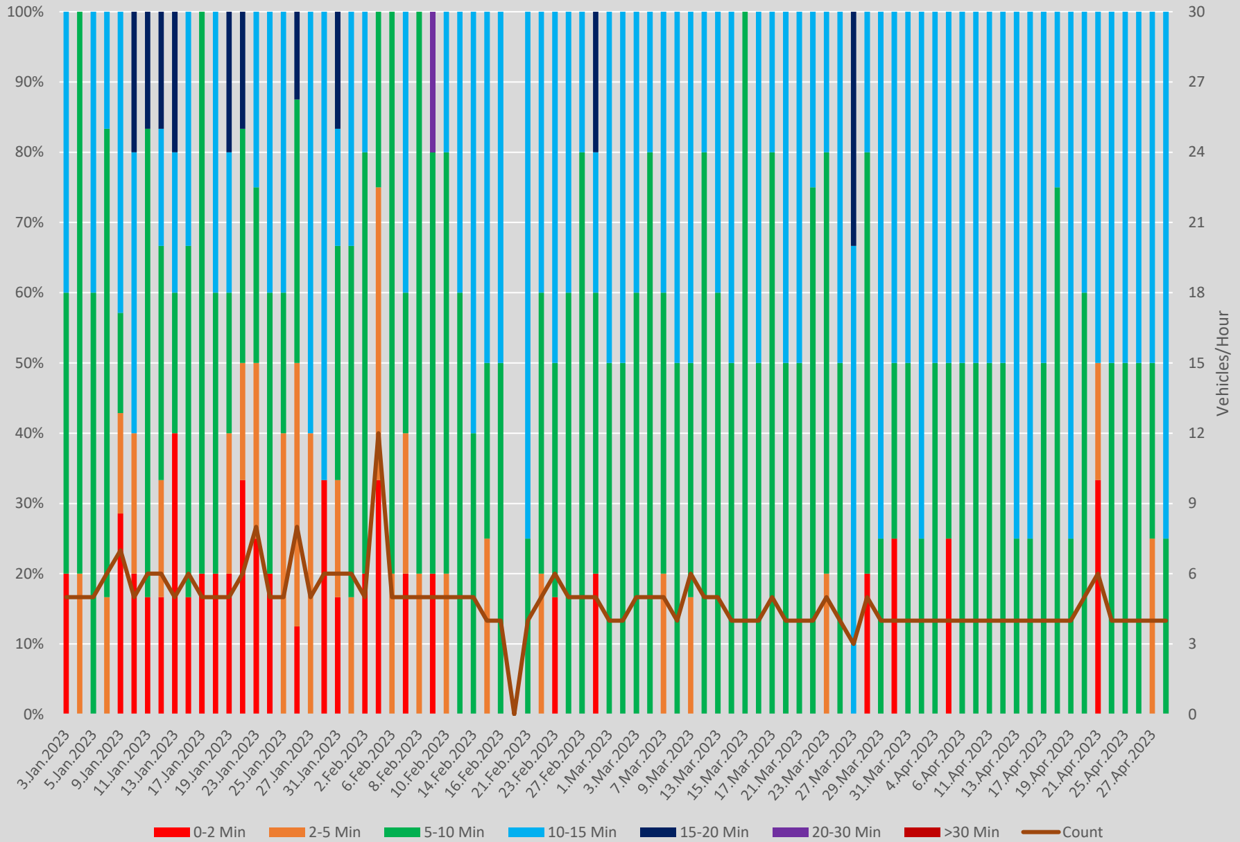
Headway Distributions 505 Dundas Yonge Westbound 600 to 700
