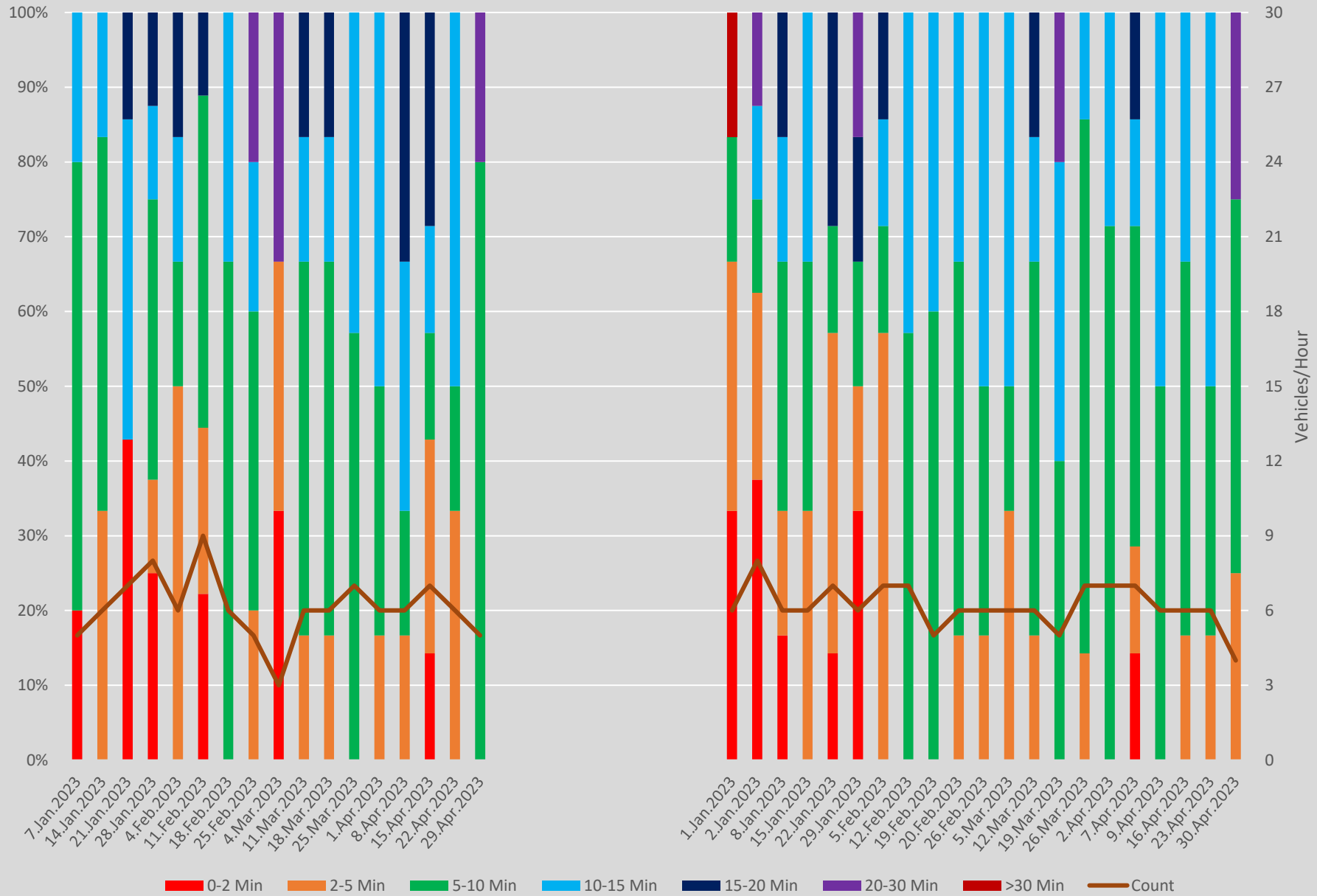
Headway Distributions 505 Dundas Yonge Westbound 2000 to 2100 Weekends
