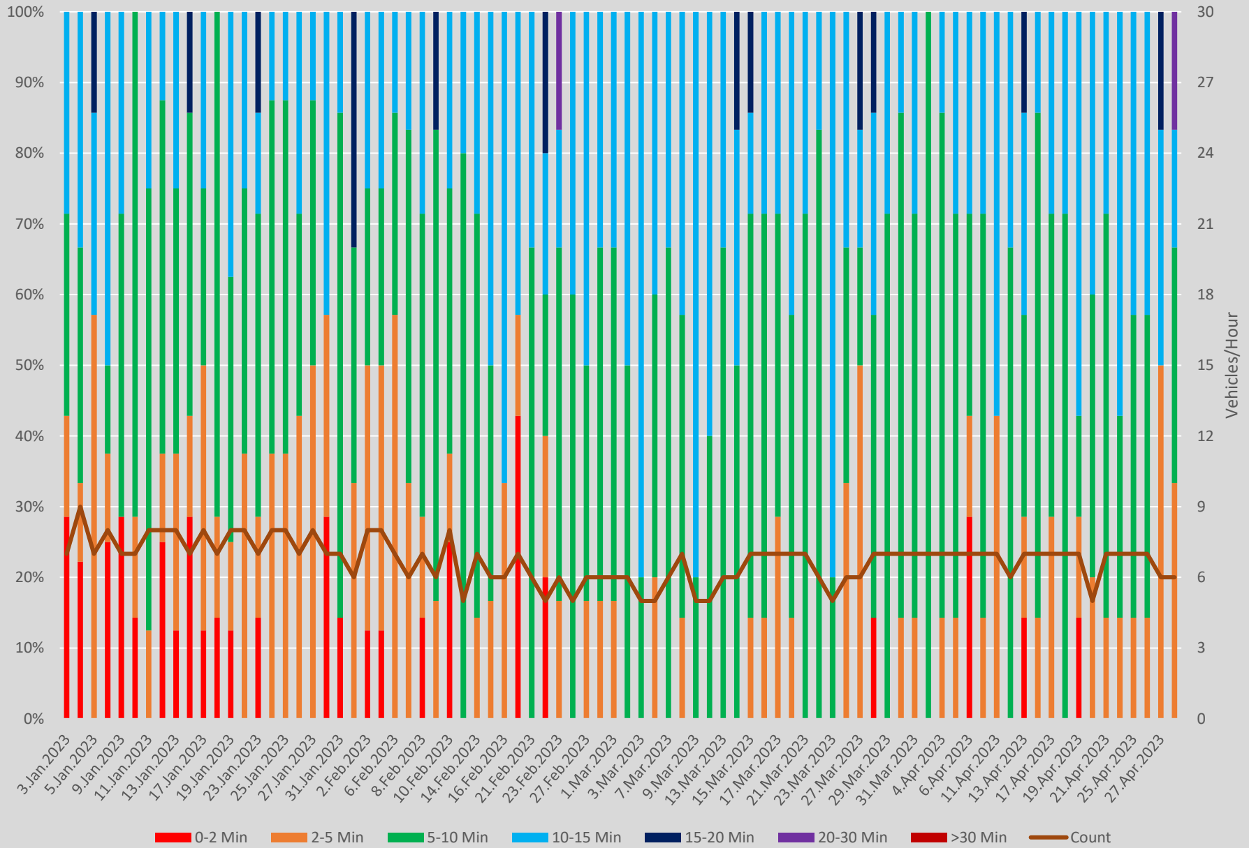
Headway Distributions 505 Dundas Yonge Westbound 700 to 800
