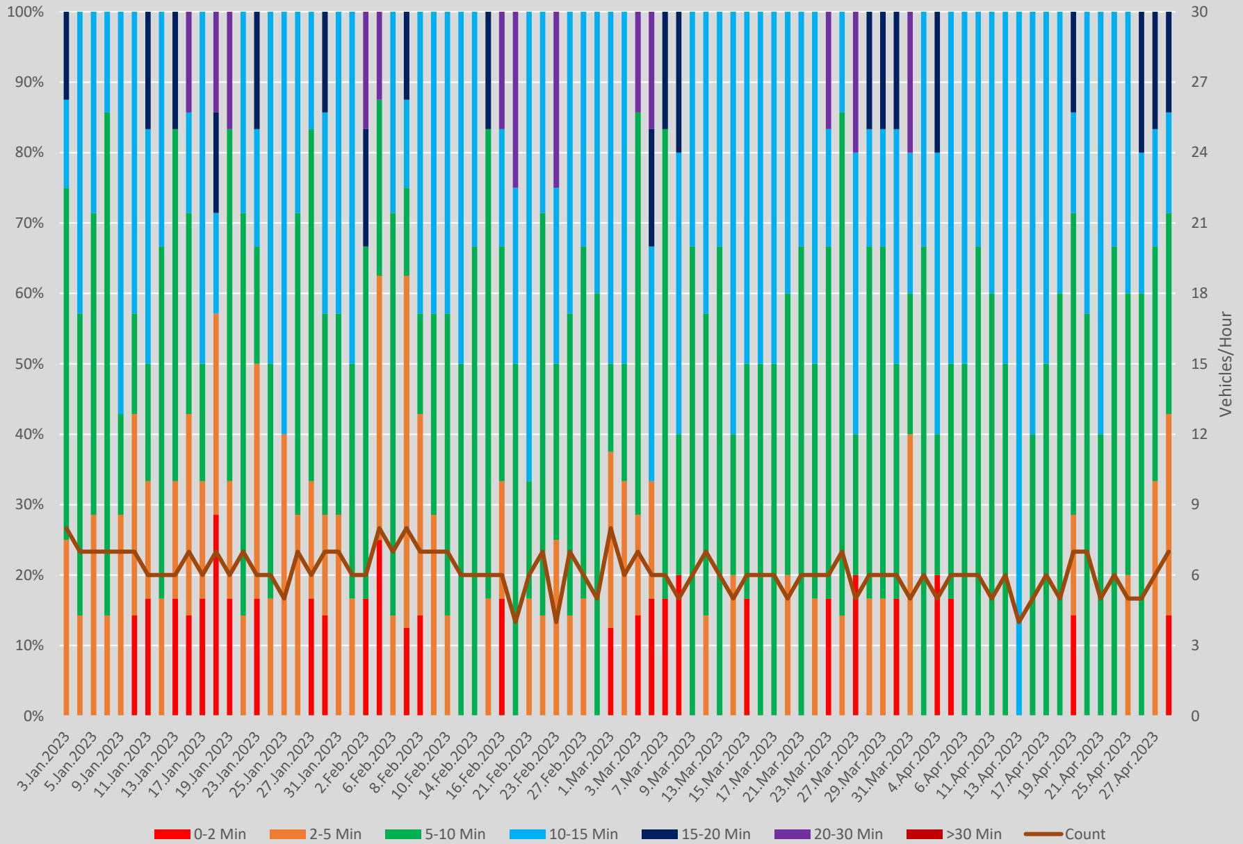
Headway Distributions 505 Dundas Yonge Westbound 800 to 900
