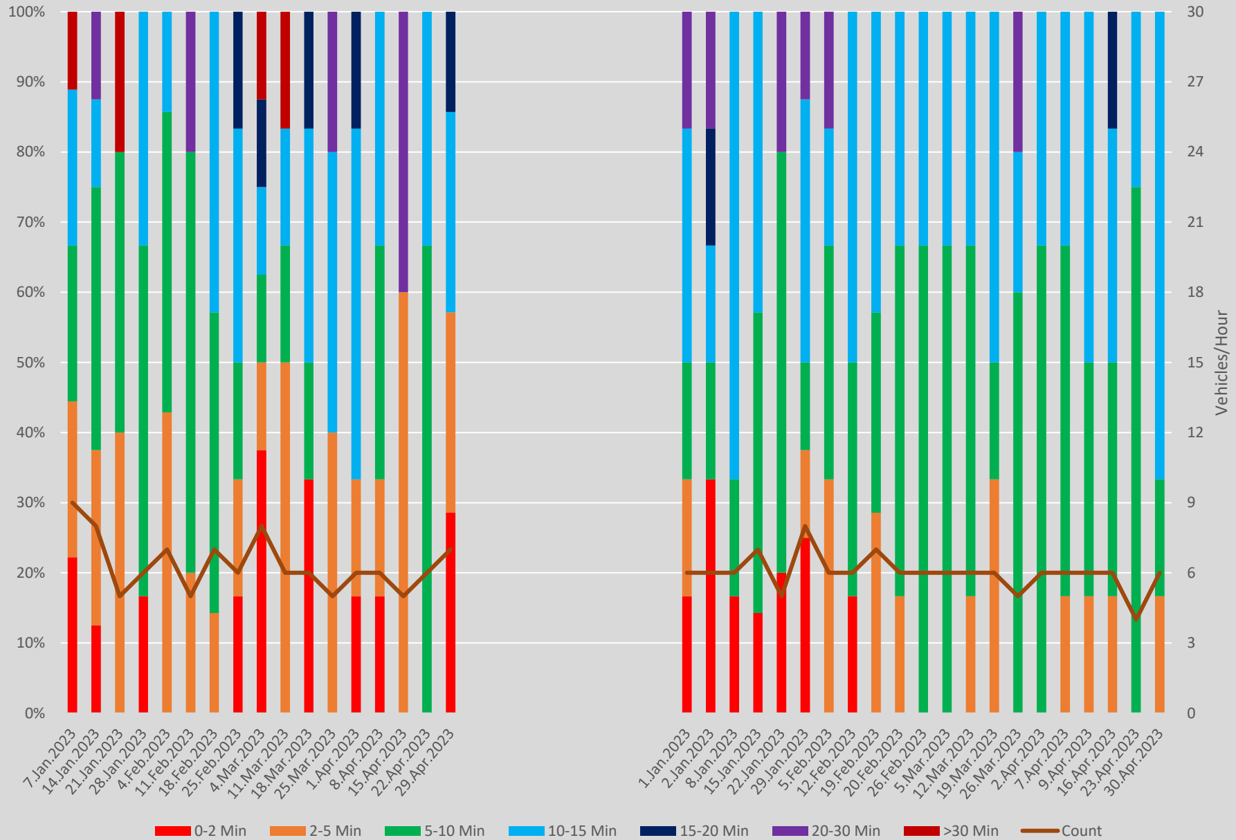
Headway Distributions 505 Dundas Yonge Westbound 2100 to 2200 Weekends
