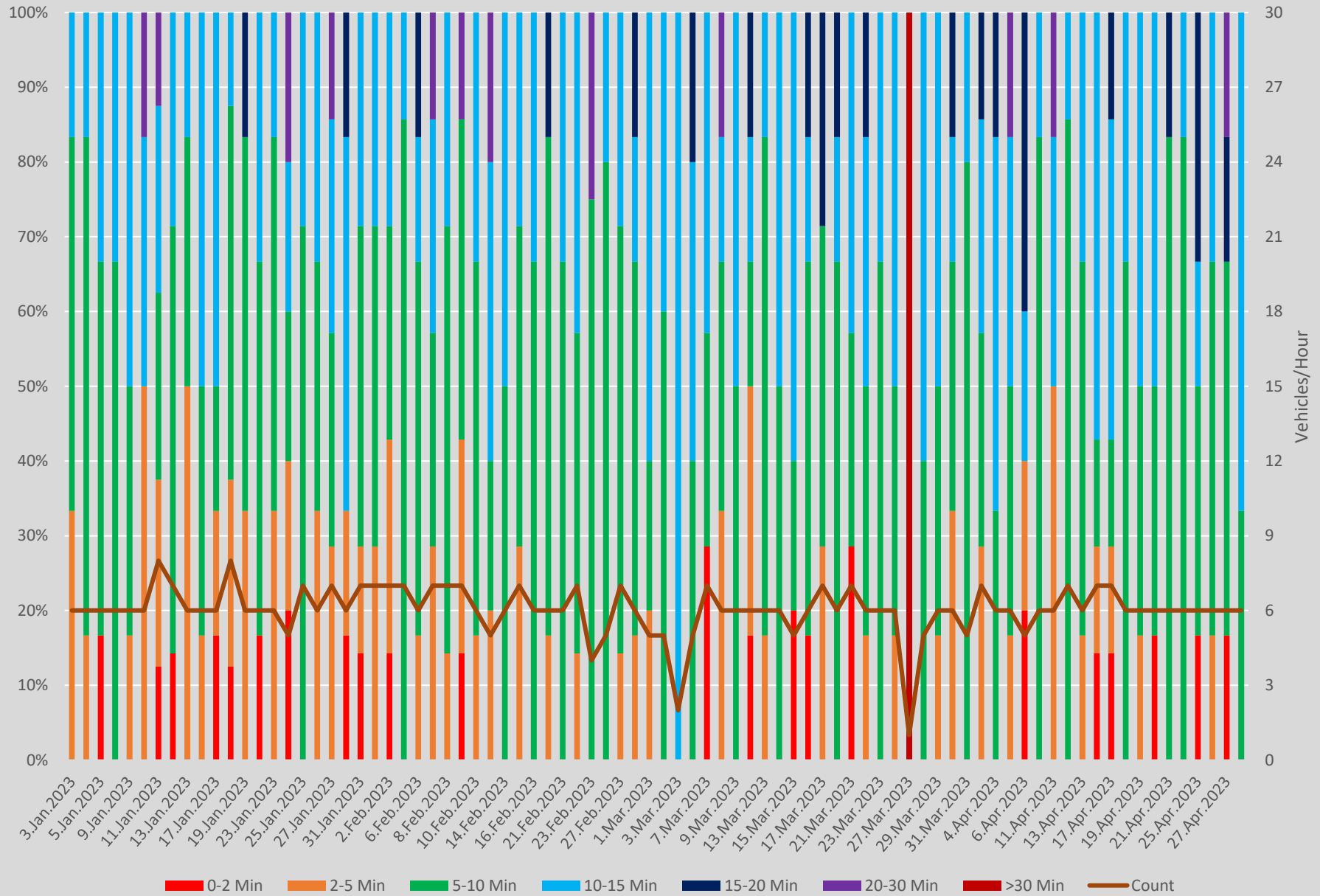
Headway Distributions 505 Dundas Yonge Westbound 1100 to 1200
