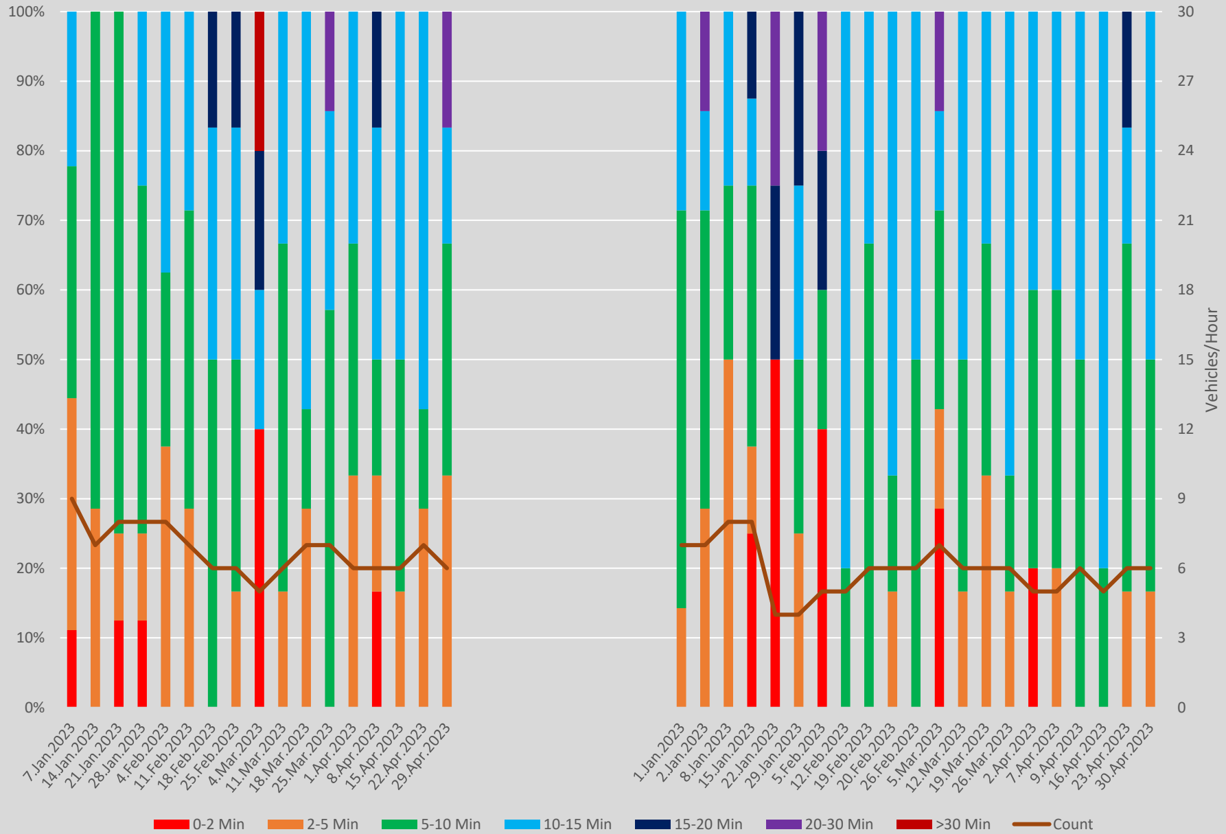
Headway Distributions 505 Dundas Yonge Westbound 1100 to 1200 Weekends
