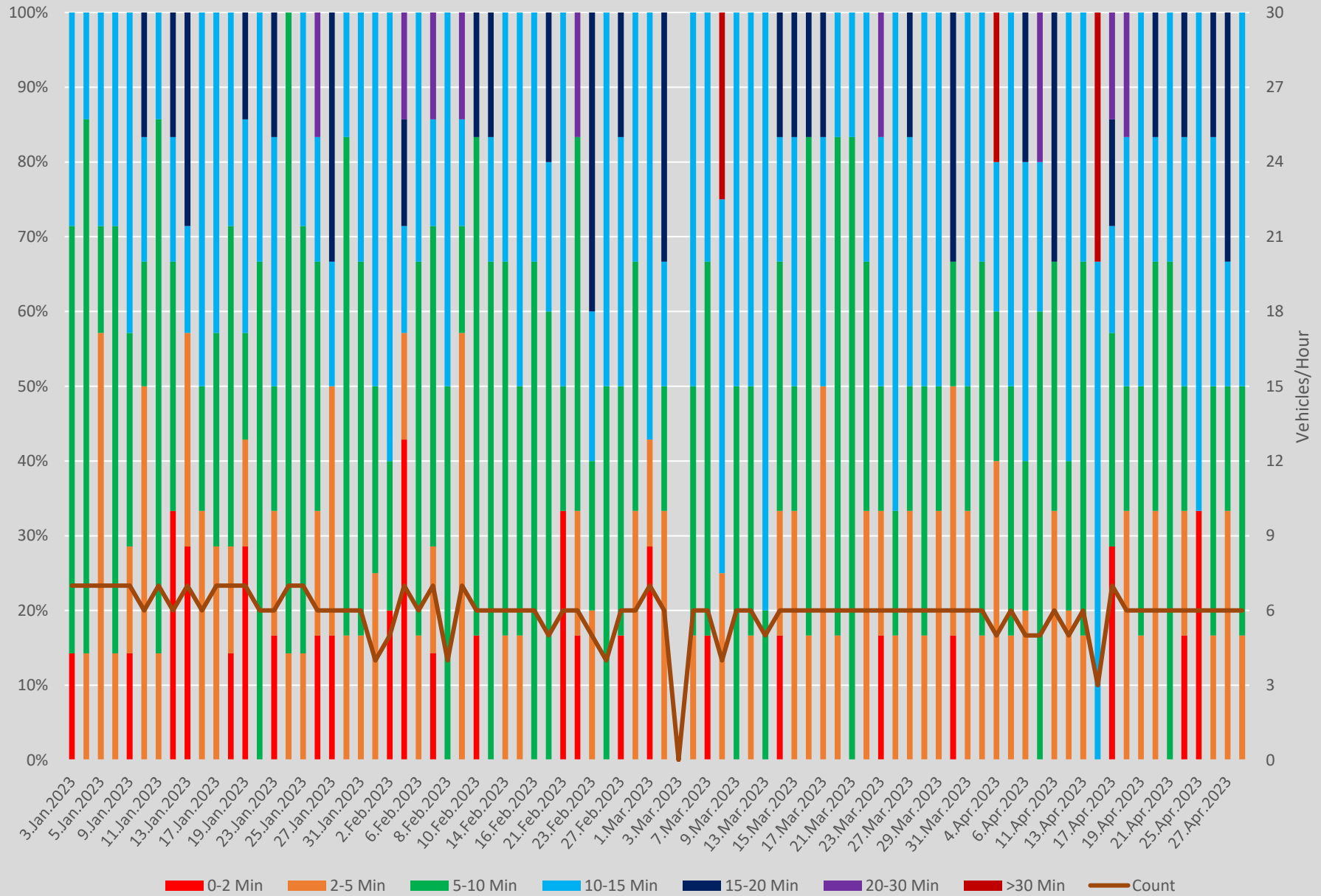
Headway Distributions 505 Dundas Yonge Westbound 1300 to 1400
