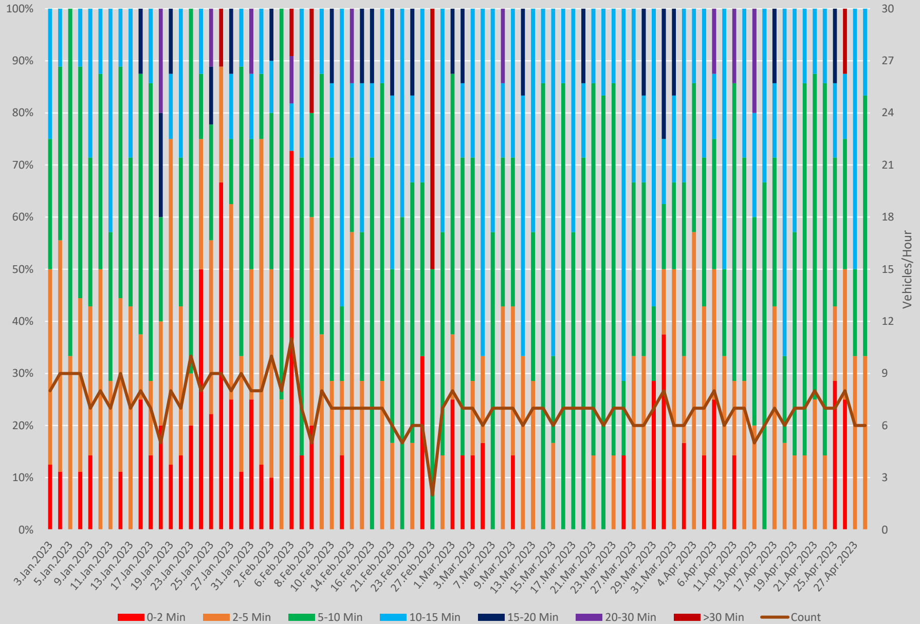
Headway Distributions 505 Dundas Yonge Westbound 1900 to 2000
