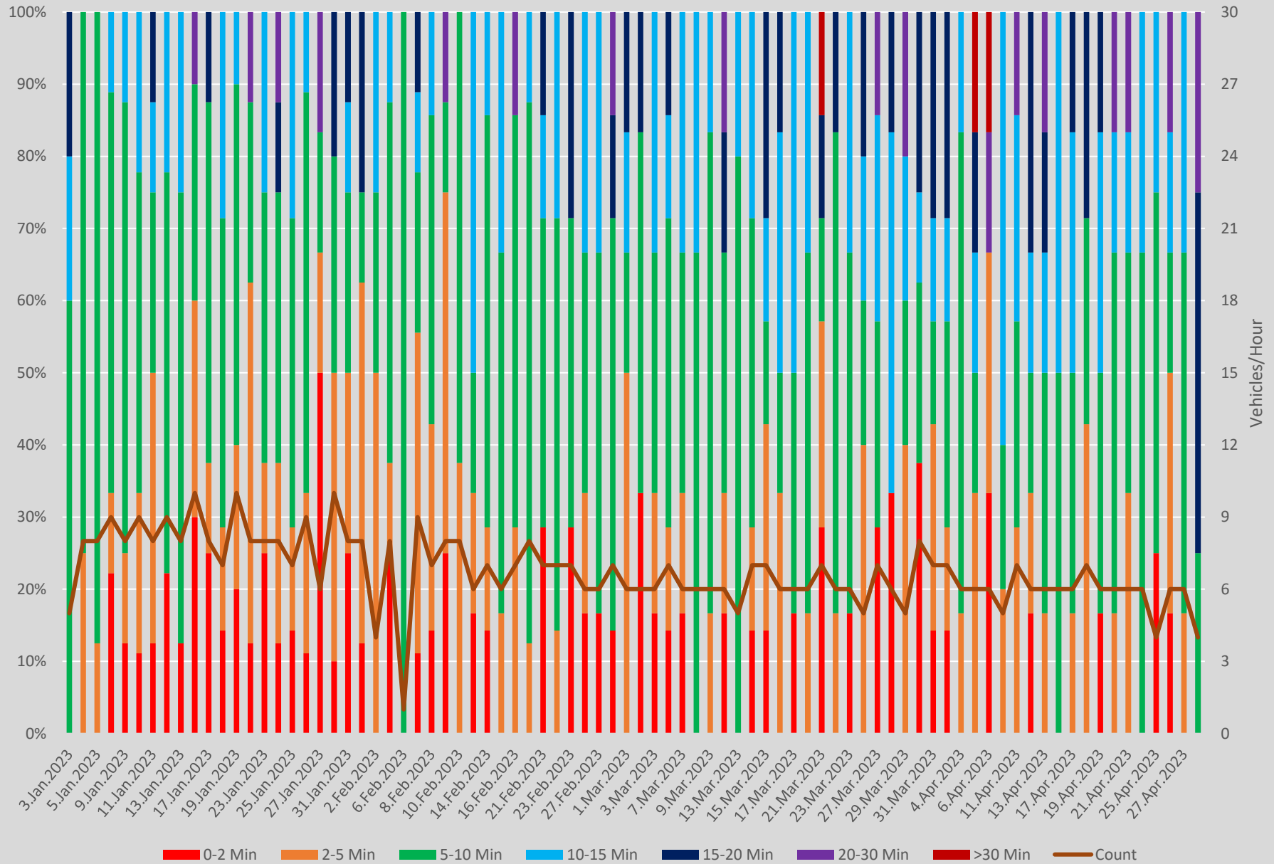
Headway Distributions 505 Dundas Yonge Westbound 1600 to 1700
