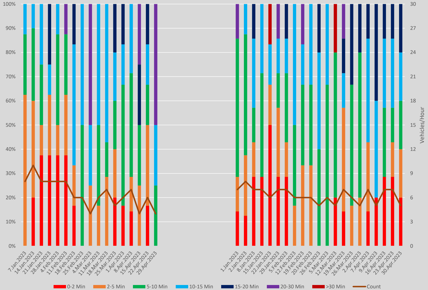
Headway Distributions 505 Dundas Yonge Westbound 1300 to 1400 Weekends
