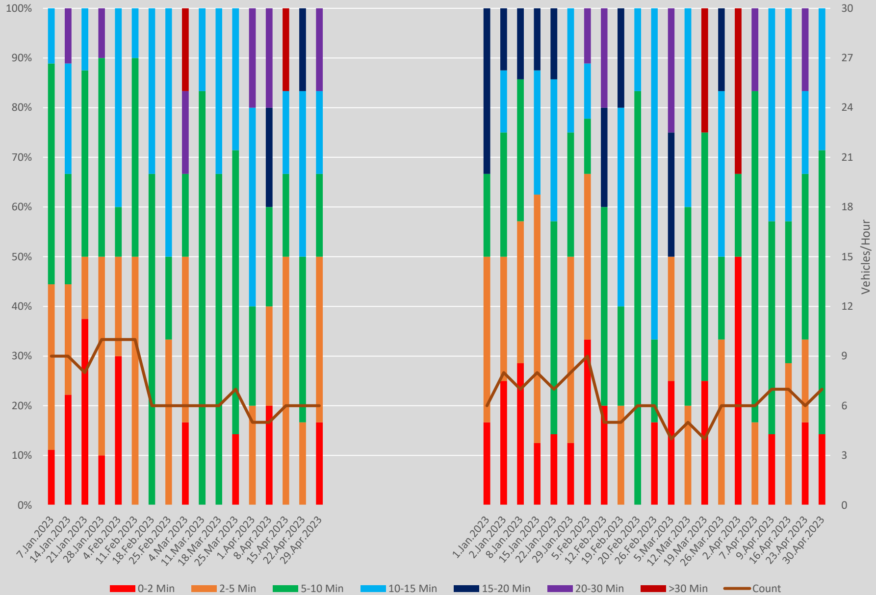
Headway Distributions 505 Dundas Yonge Westbound 1700 to 1800 Weekends
