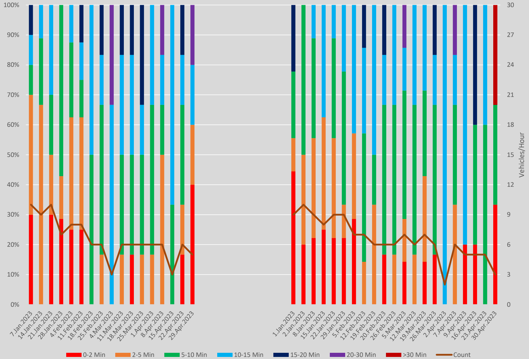
Headway Distributions 505 Dundas Yonge Westbound 1600 to 1700 Weekends
