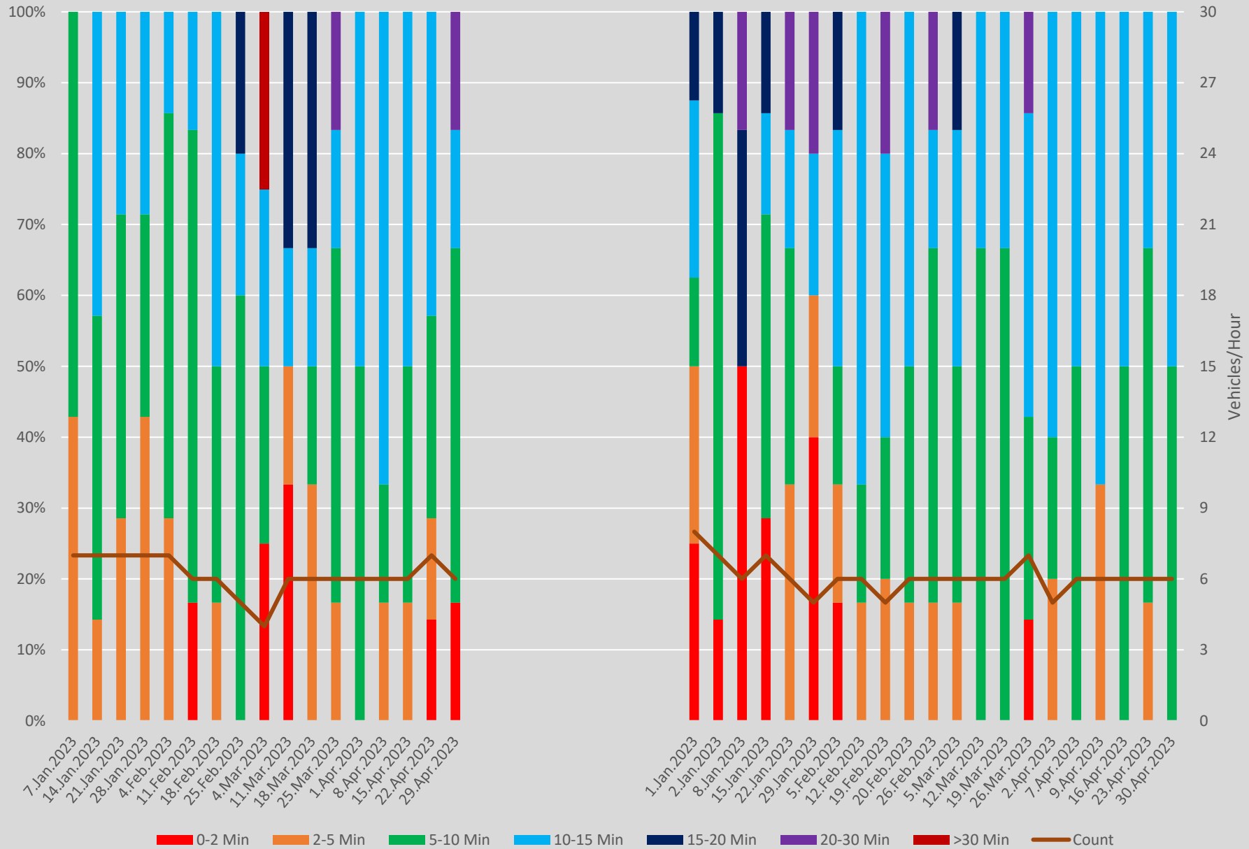
Headway Distributions 505 Dundas Yonge Westbound 900 to 1000 Weekends
