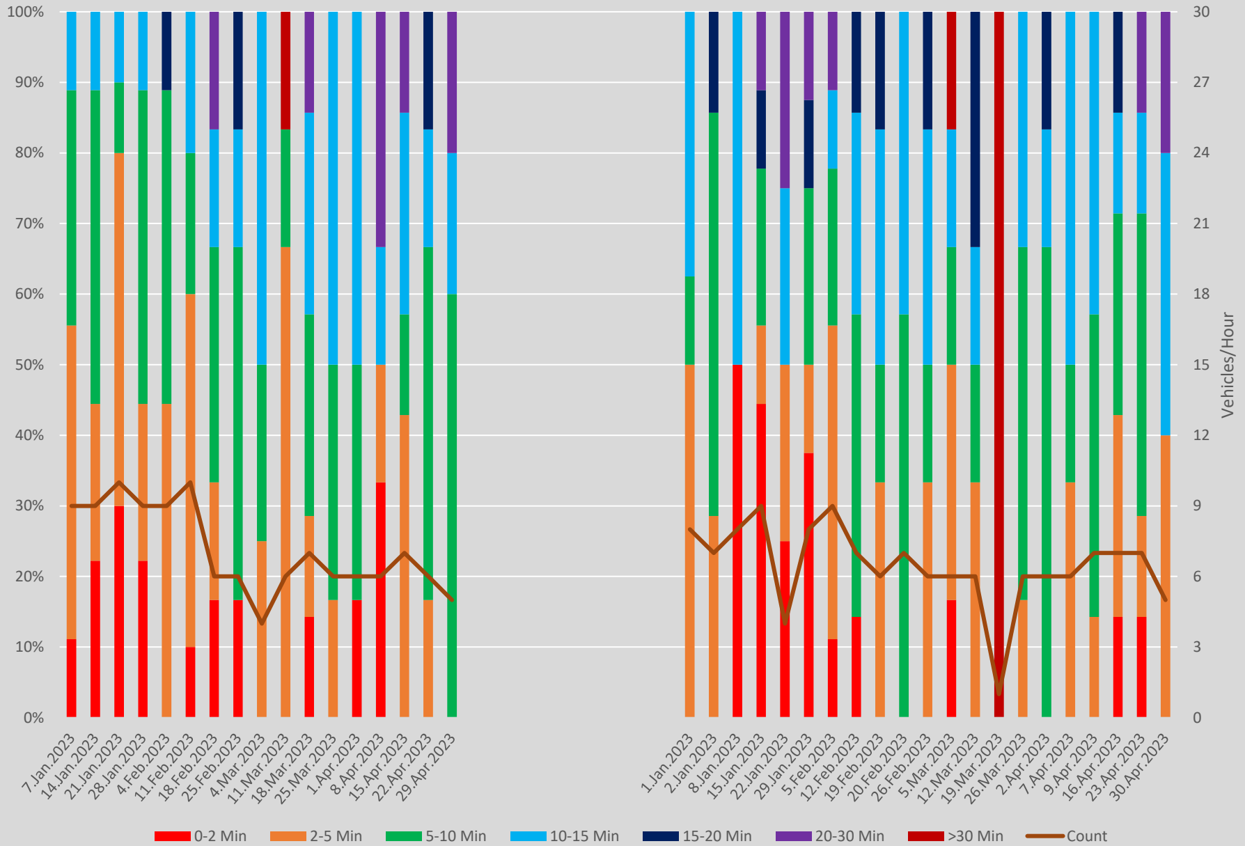
Headway Distributions 505 Dundas Yonge Eastbound 1400 to 1500 Weekends
