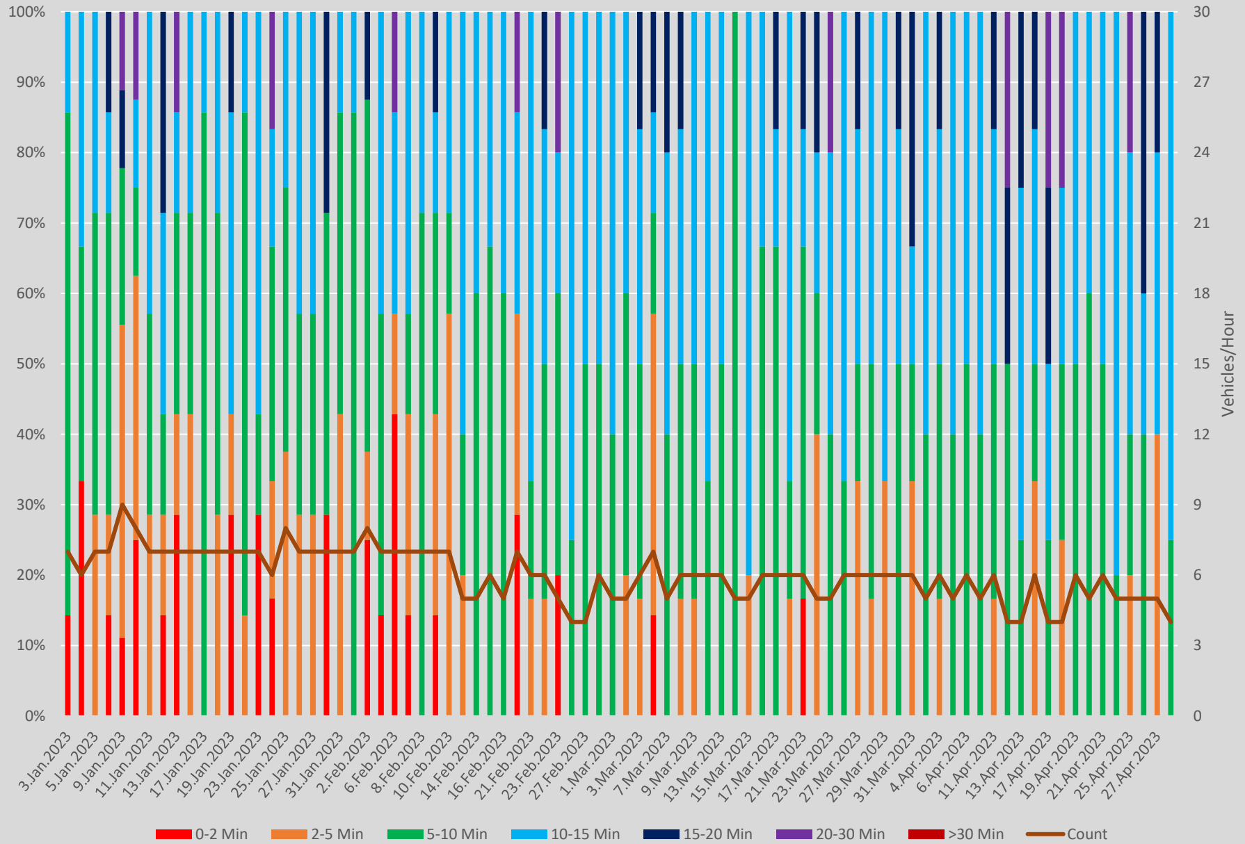
Headway Distributions 505 Dundas Yonge Eastbound 800 to 900
