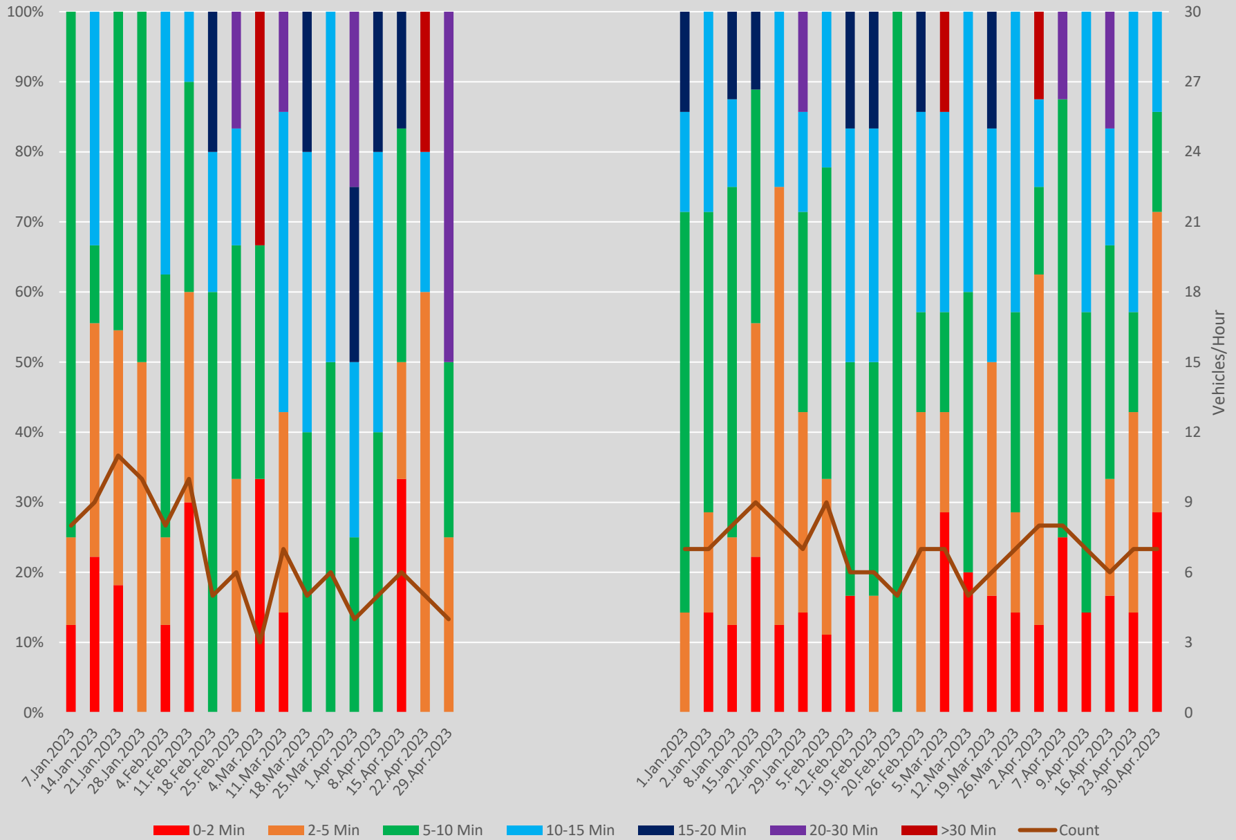
Headway Distributions 505 Dundas Yonge Eastbound 1900 to 2000 Weekends
