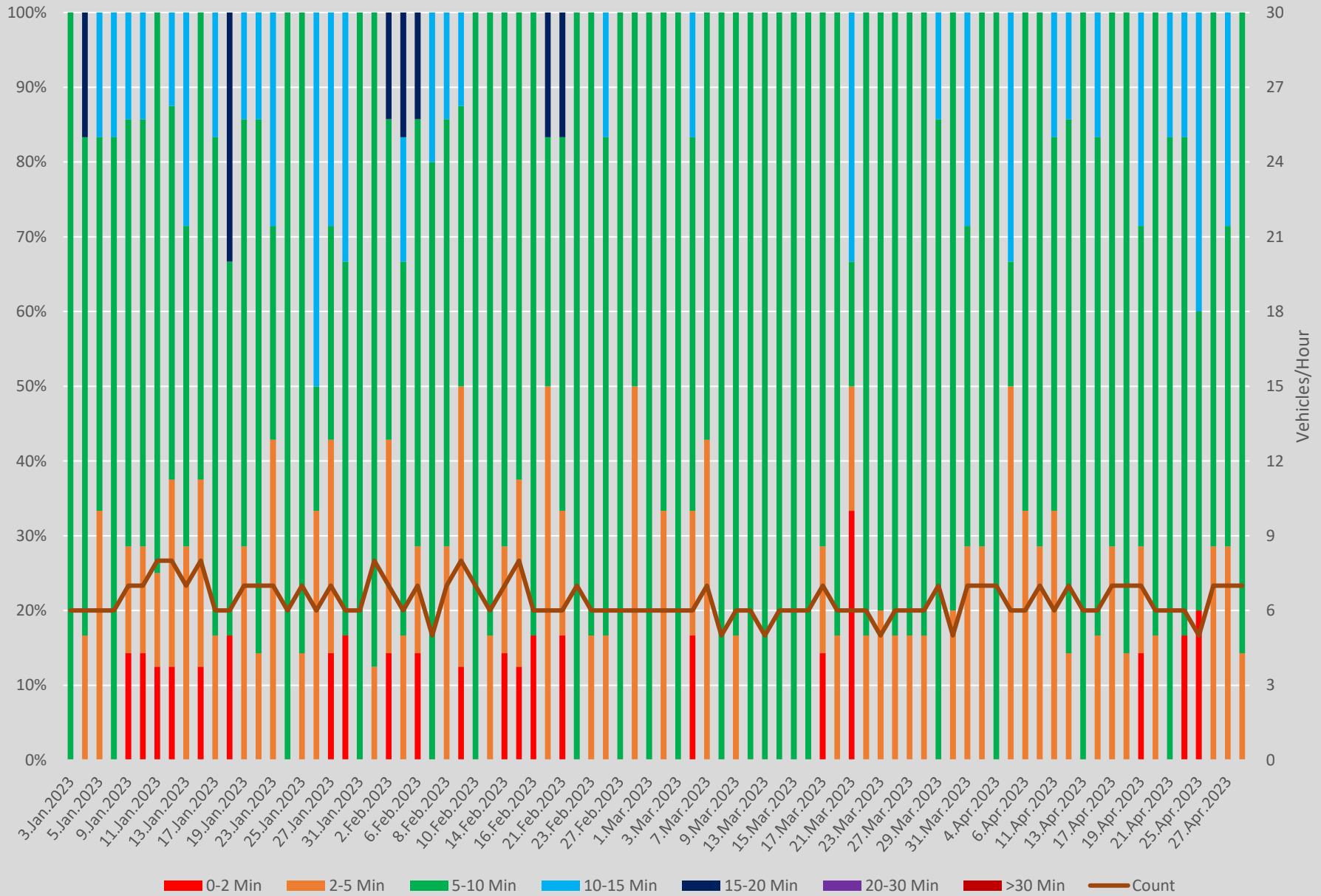
Headway Distributions 503 Kingston Road West of Bingham Loop Westbound 600 to 700
