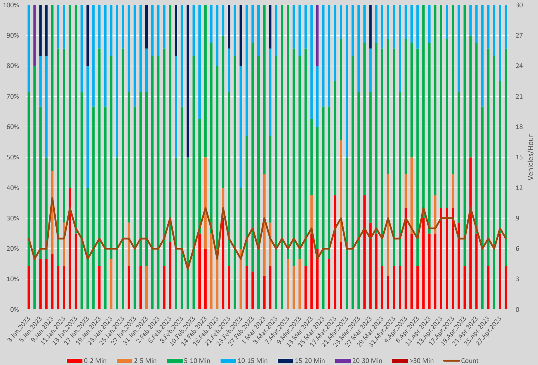
Headway Distributions 503 Kingston Road West of Bingham Loop Westbound 900 to 1000
