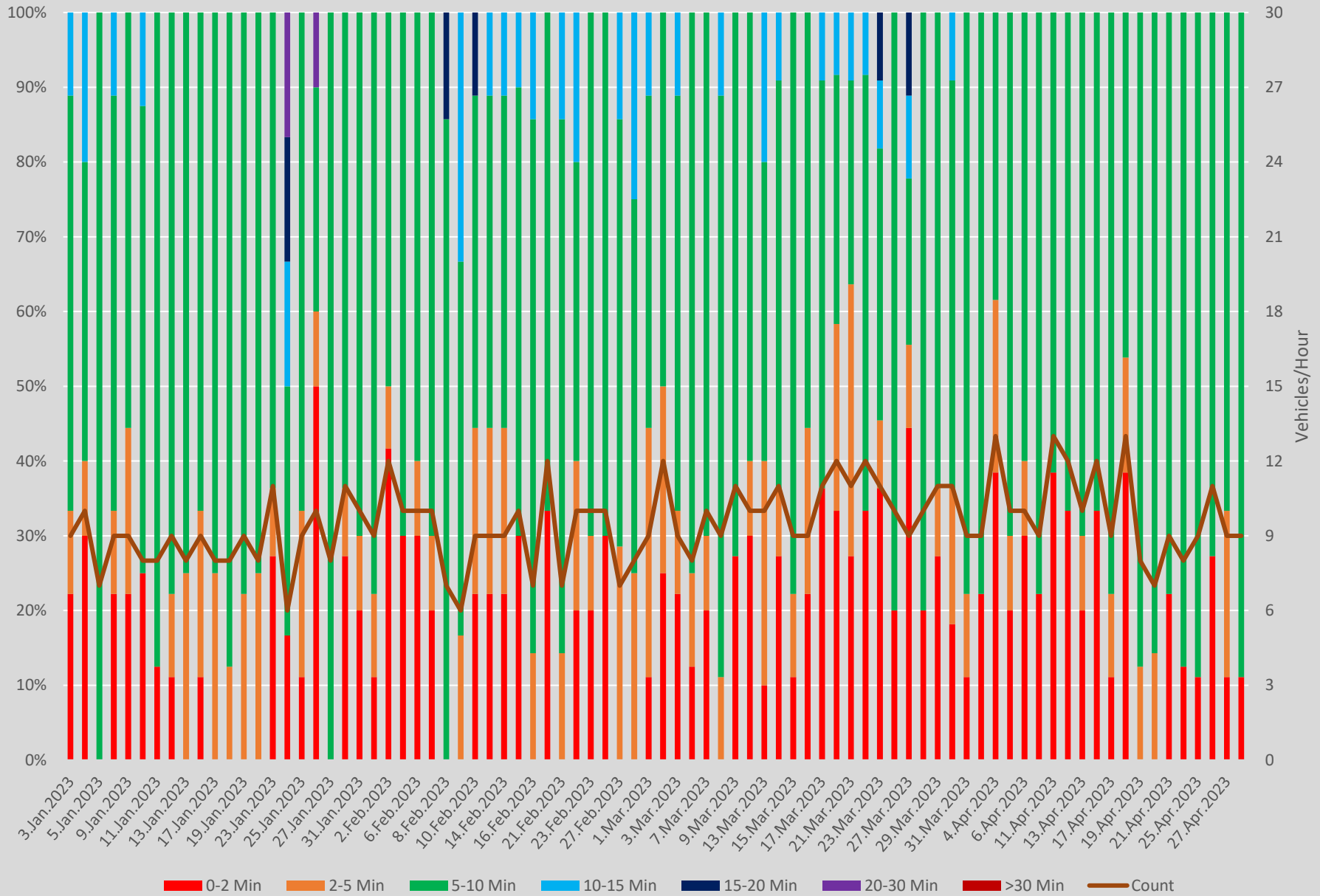
Headway Distributions 503 Kingston Road West of Bingham Loop Westbound 700 to 800
