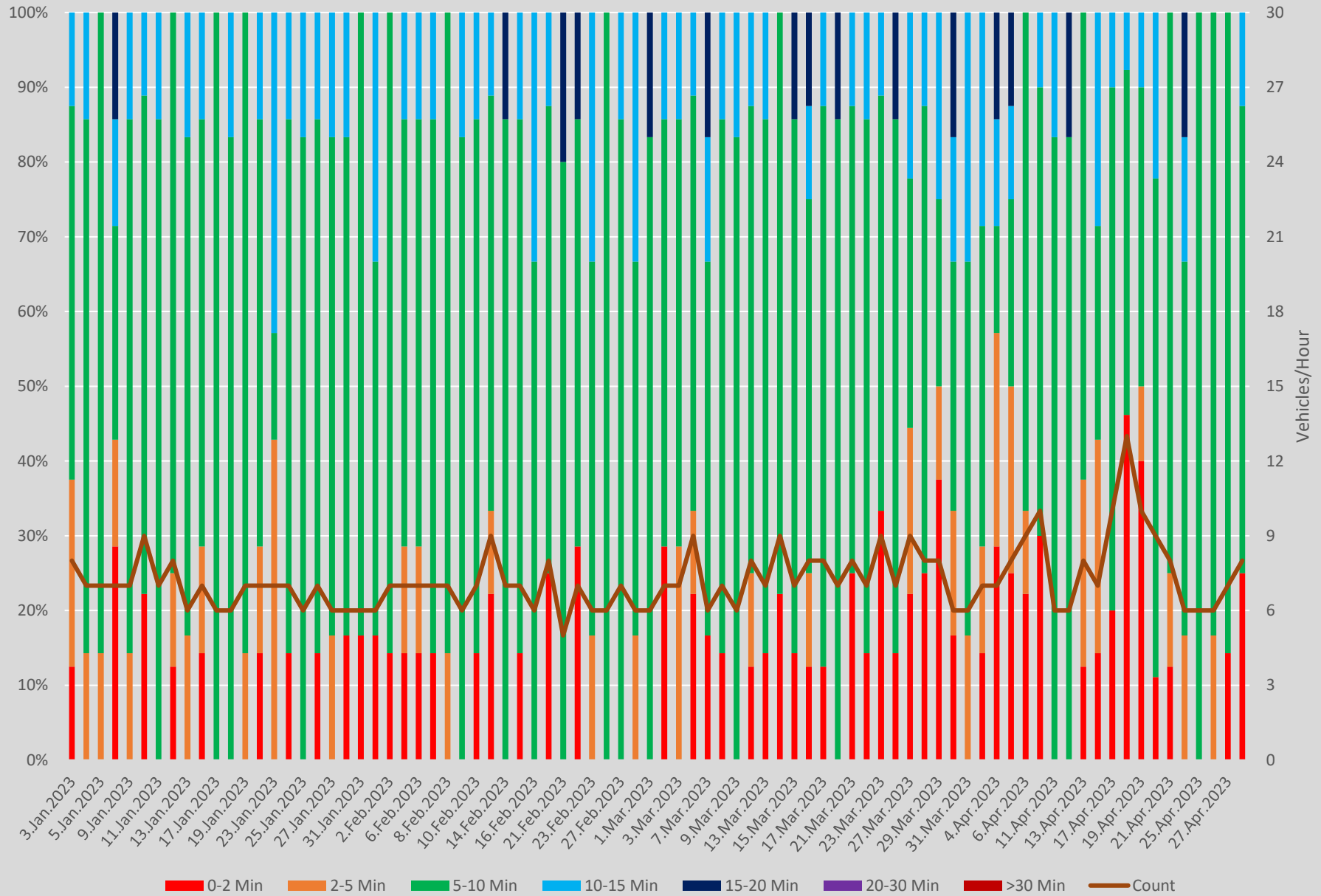
Headway Distributions 503 Kingston Road West of Bingham Loop Westbound 800 to 900
