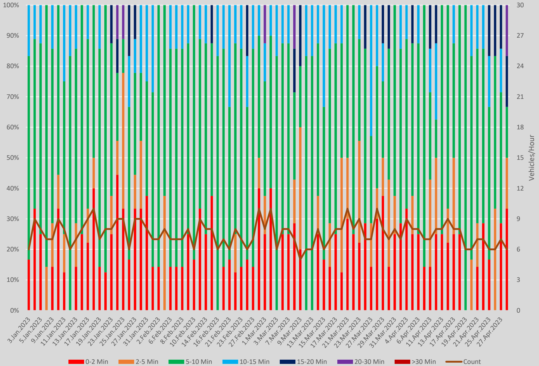
Headway Distributions 503 Kingston Road West of Bingham Loop Westbound 1800 to 1900
