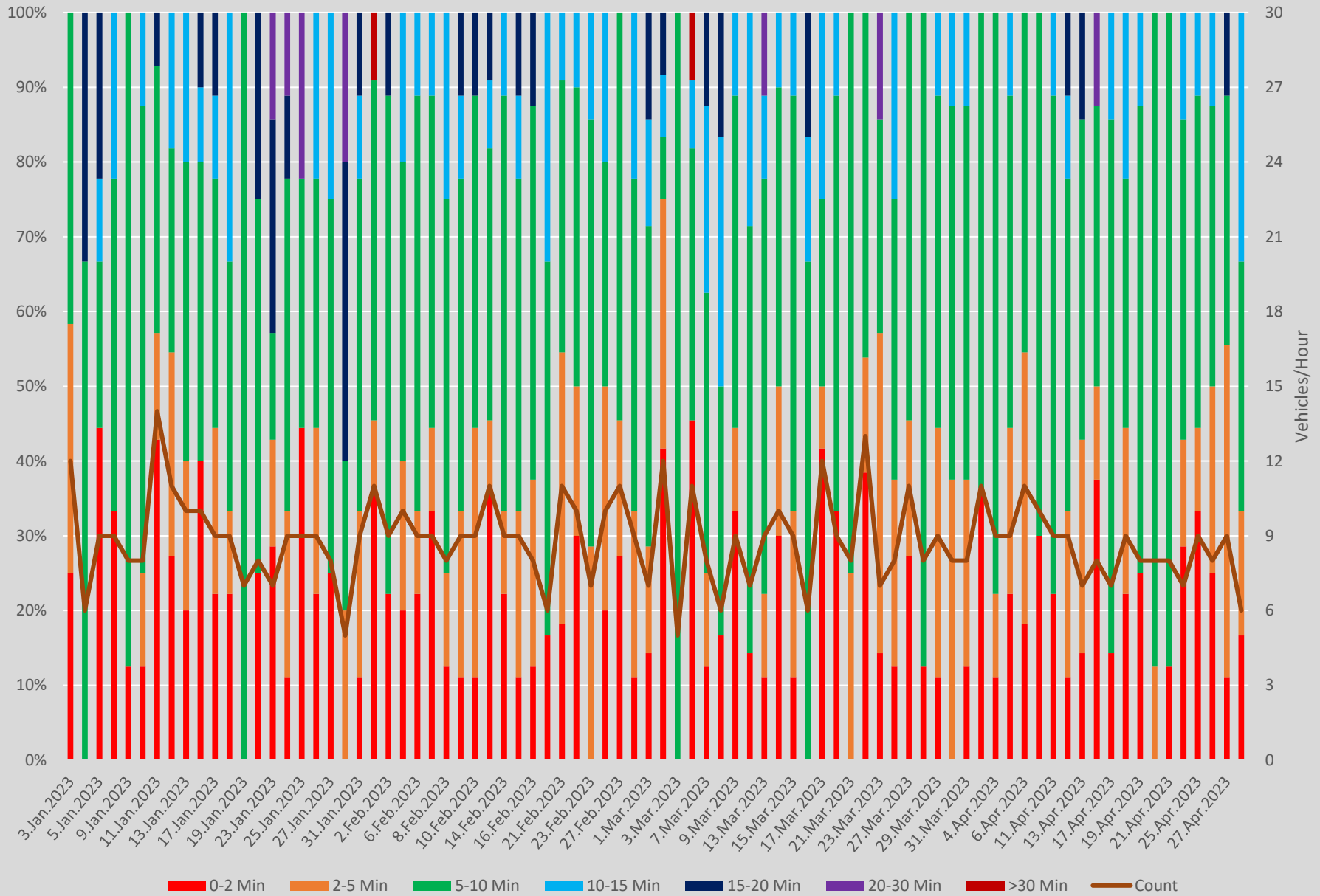
Headway Distributions 503 Kingston Road West of Bingham Loop Westbound 1500 to 1600
