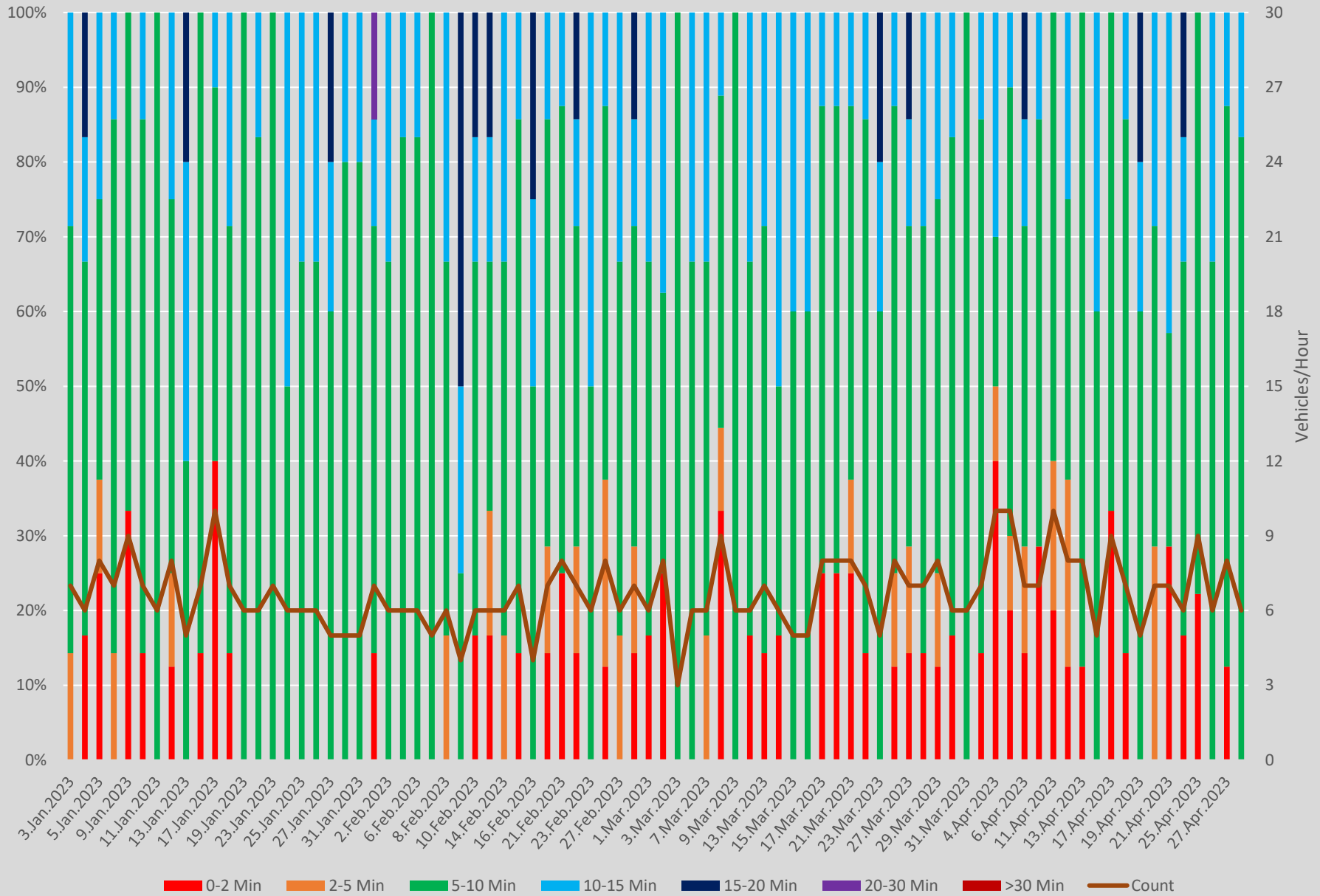
Headway Distributions 503 Kingston Road West of Bingham Loop Westbound 1100 to 1200
