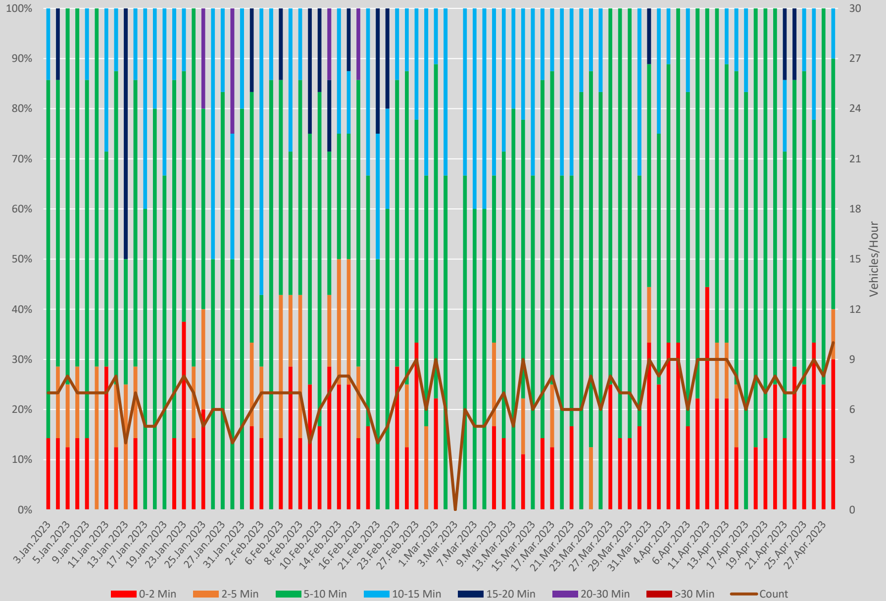
Headway Distributions 503 Kingston Road West of Bingham Loop Westbound 1300 to 1400
