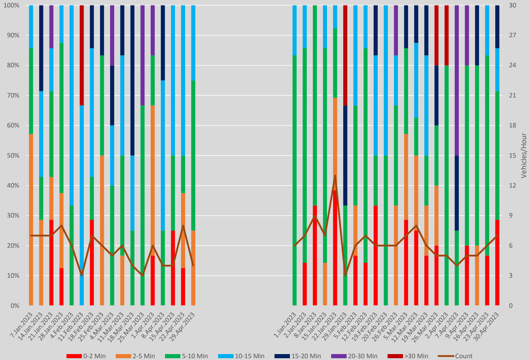
Headway Distributions 501 Queen East of Coxwell Ave. Westbound 2200 to 2300 Weekends
