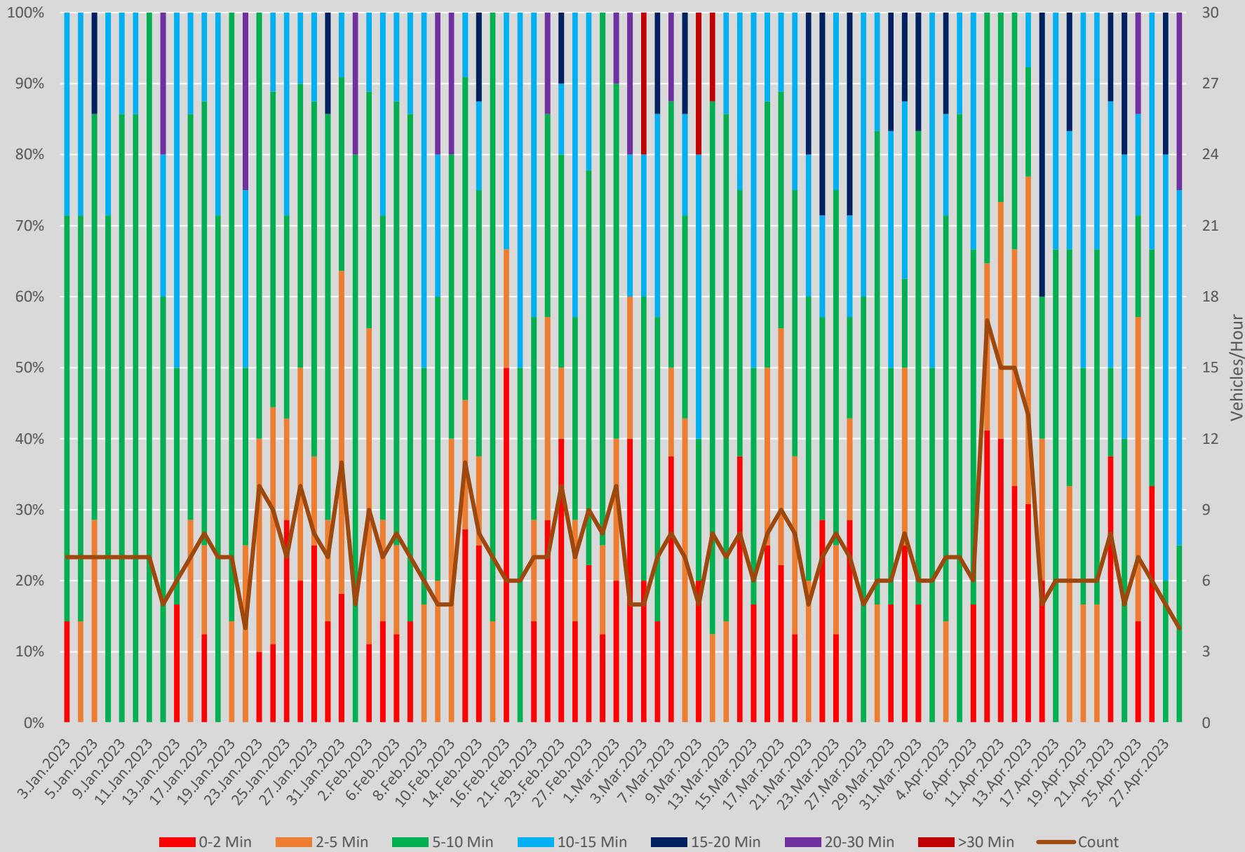
Headway Distributions 501 Queen East of Coxwell Ave. Westbound 2200 to 2300
