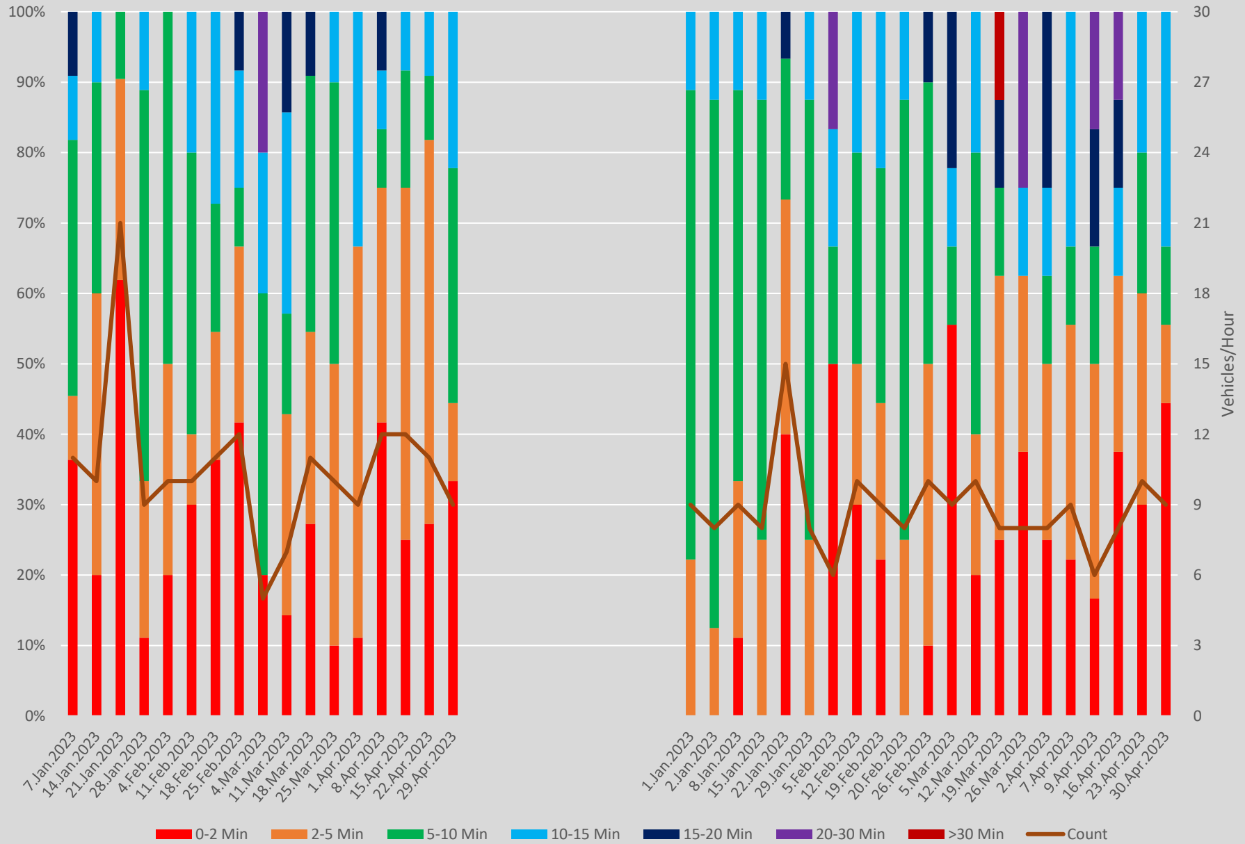
Headway Distributions 501 Queen East of Coxwell Ave. Westbound 1200 to 1300 Weekends
