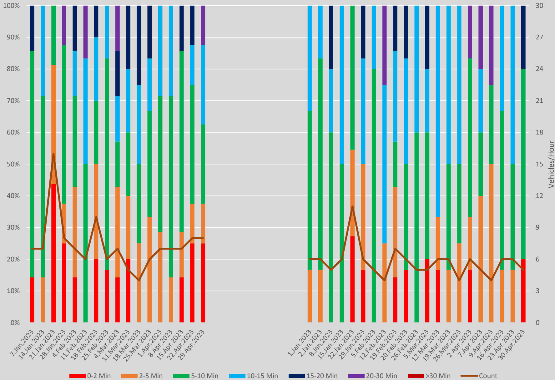
Headway Distributions 501 Queen East of Coxwell Ave. Westbound 800 to 900 Weekends
