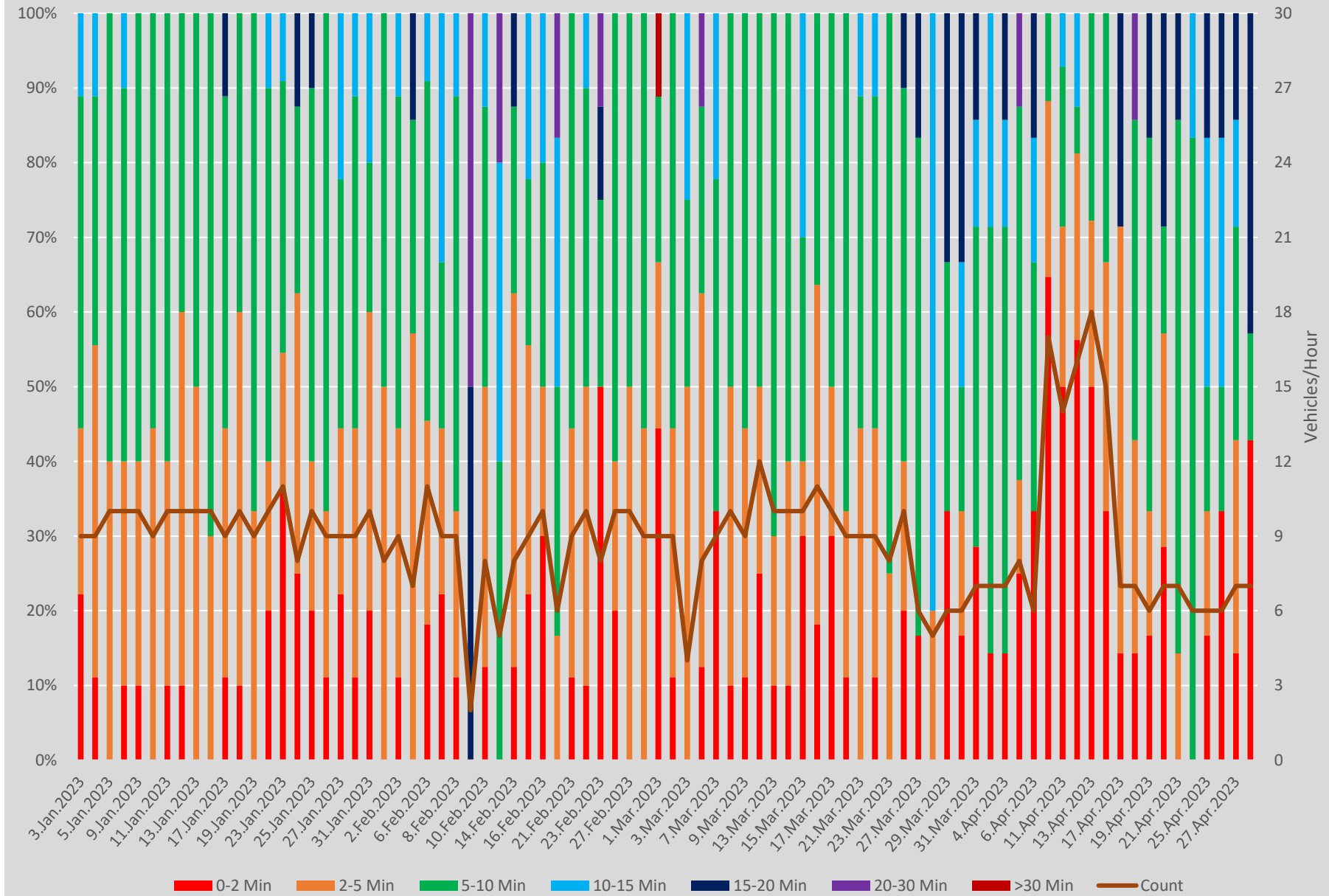
Headway Distributions 501 Queen East of Coxwell Ave. Westbound 1100 to 1200
