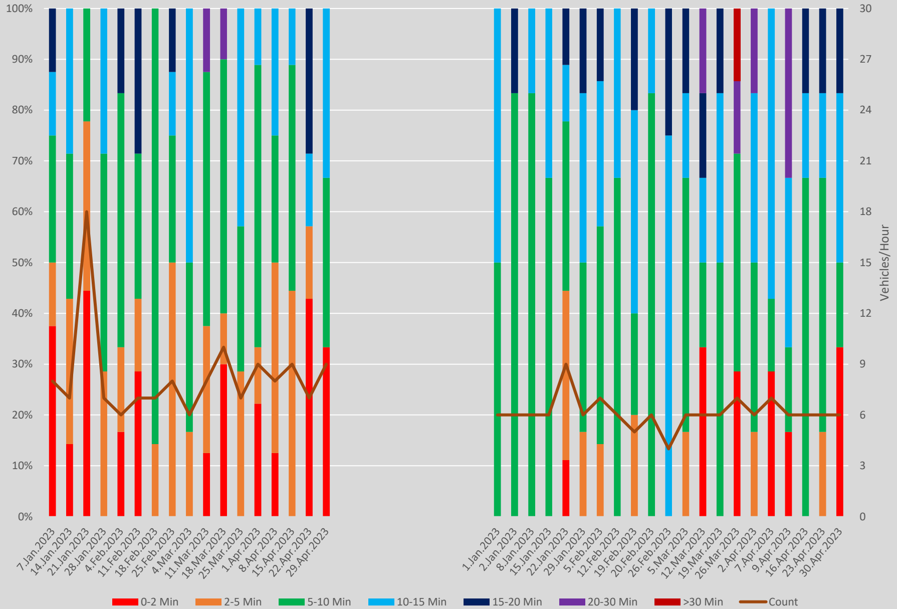
Headway Distributions 501 Queen East of Coxwell Ave. Westbound 900 to 1000 Weekends
