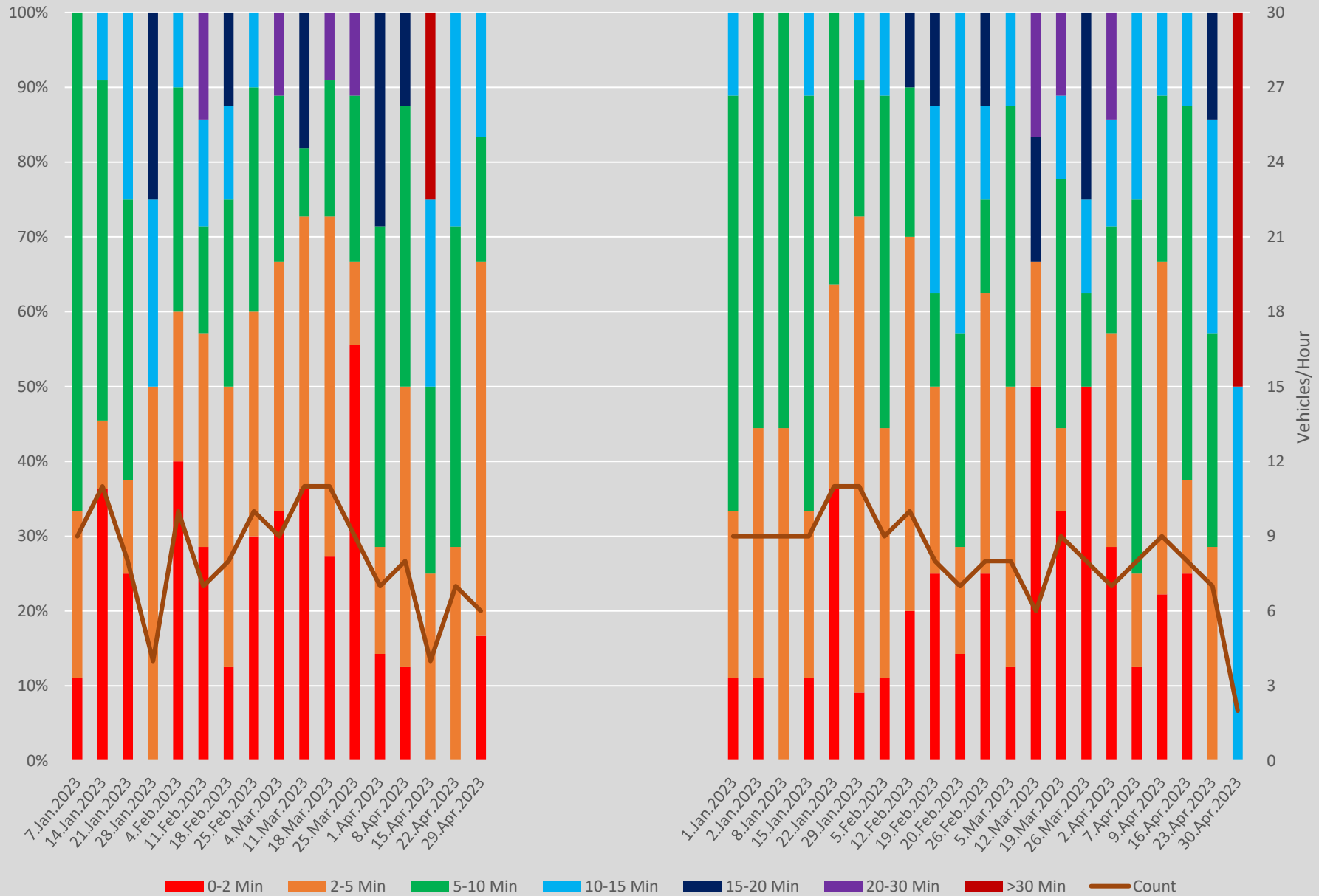
Headway Distributions 501 Queen East of Coxwell Ave. Westbound 1600 to 1700 Weekends
