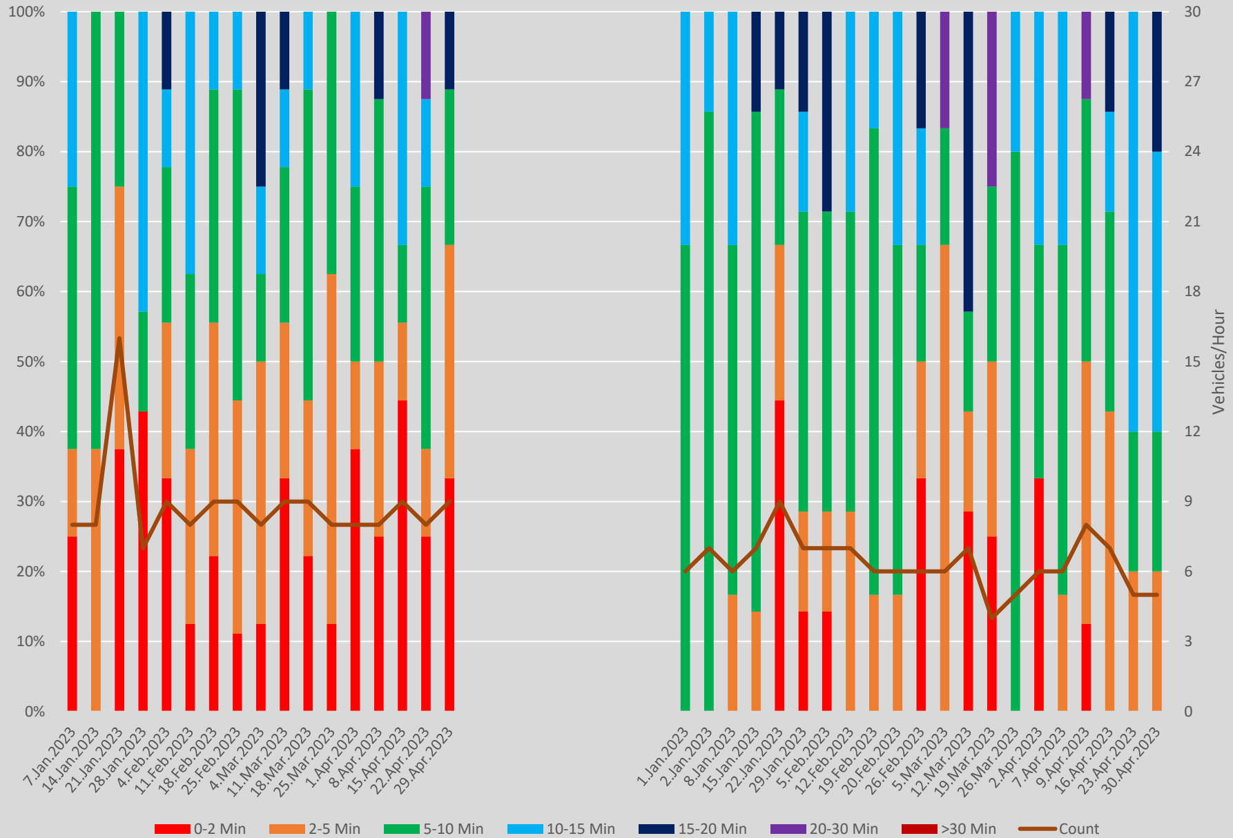
Headway Distributions 501 Queen East of Coxwell Ave. Westbound 1100 to 1200 Weekends
