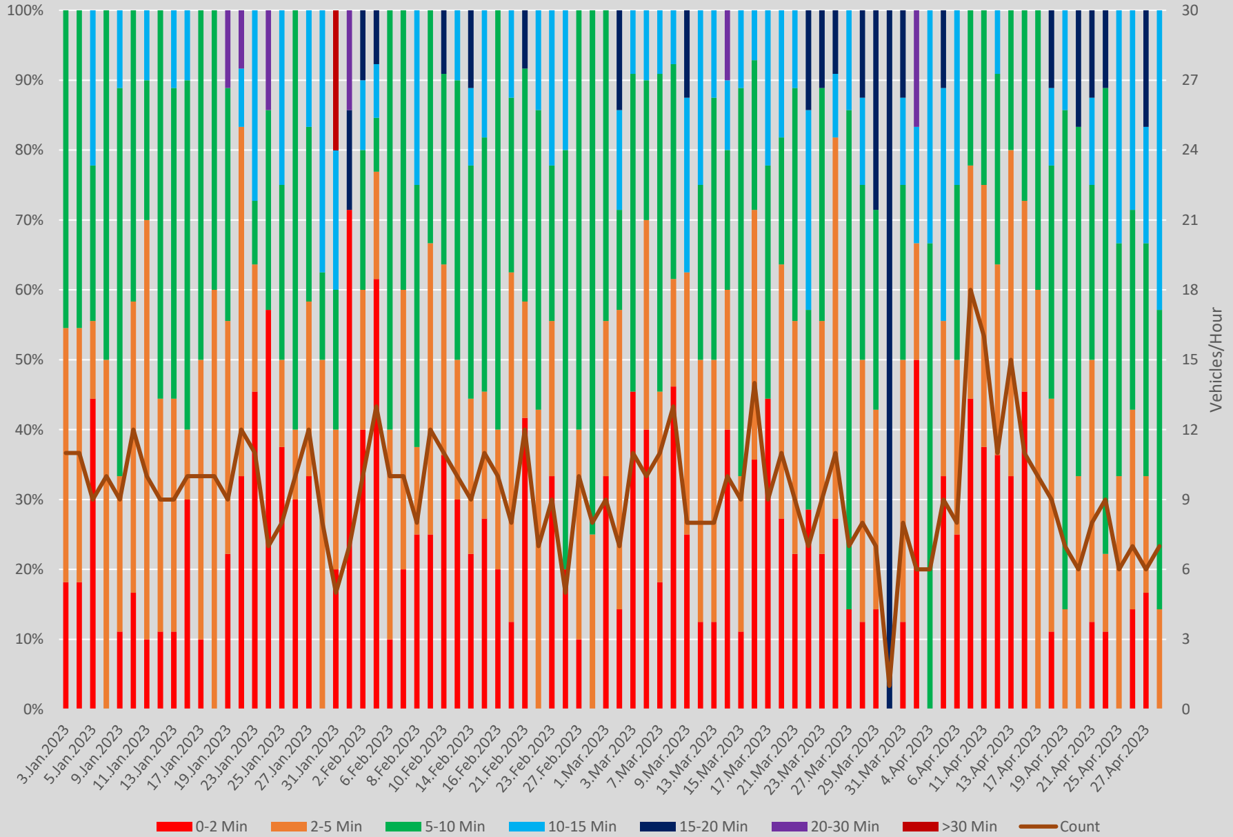
Headway Distributions 501 Queen East of Coxwell Ave. Westbound 1600 to 1700
