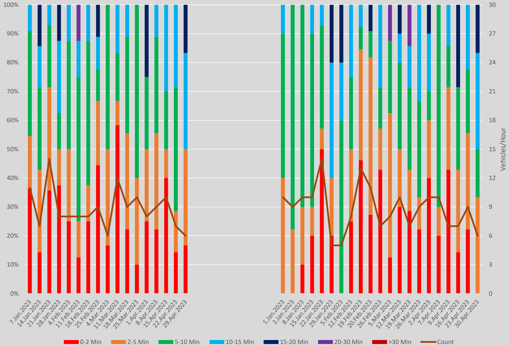
Headway Distributions 501 Queen East of Coxwell Ave. Westbound 1400 to 1500 Weekends
