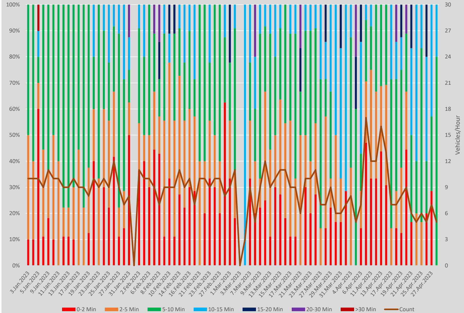
Headway Distributions 501 Queen East of Coxwell Ave. Westbound 1400 to 1500
