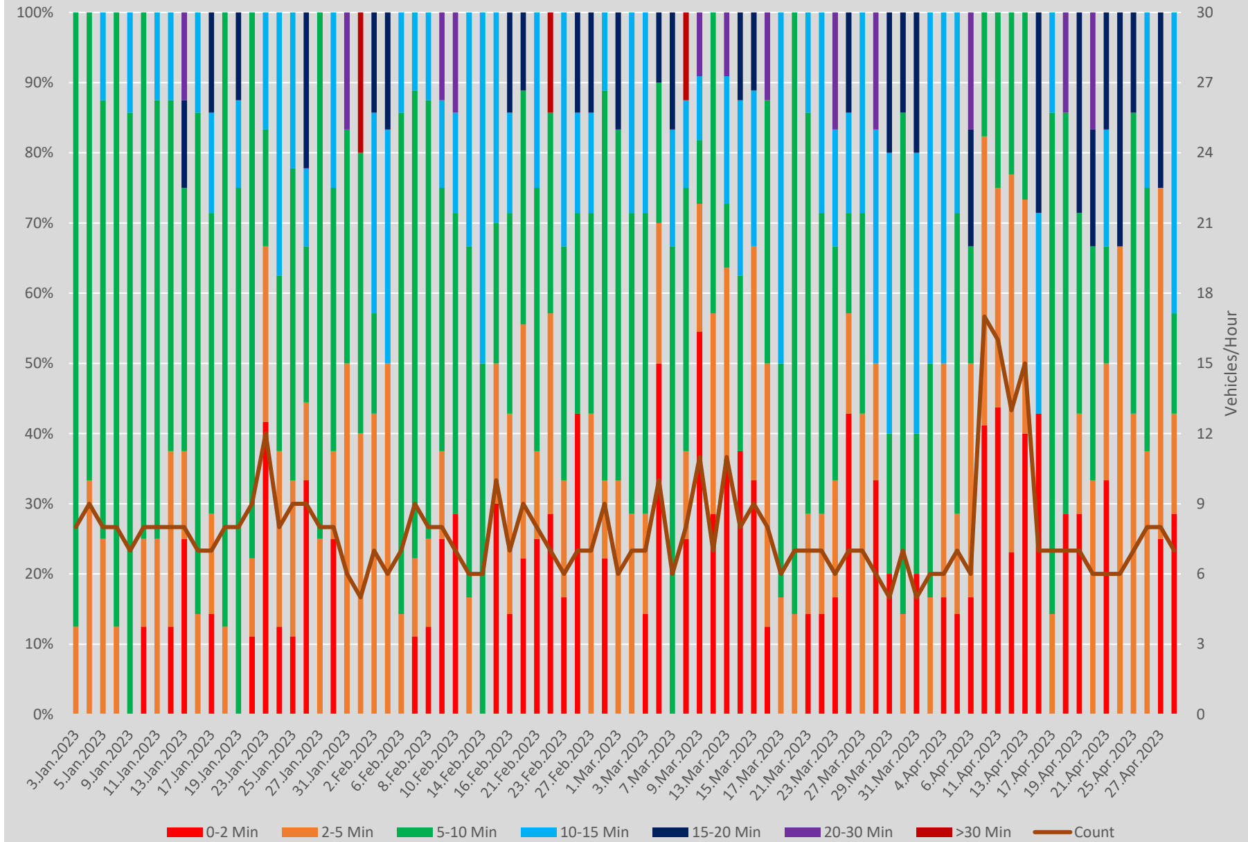
Headway Distributions 501 Queen East of Coxwell Ave. Westbound 2100 to 2200
