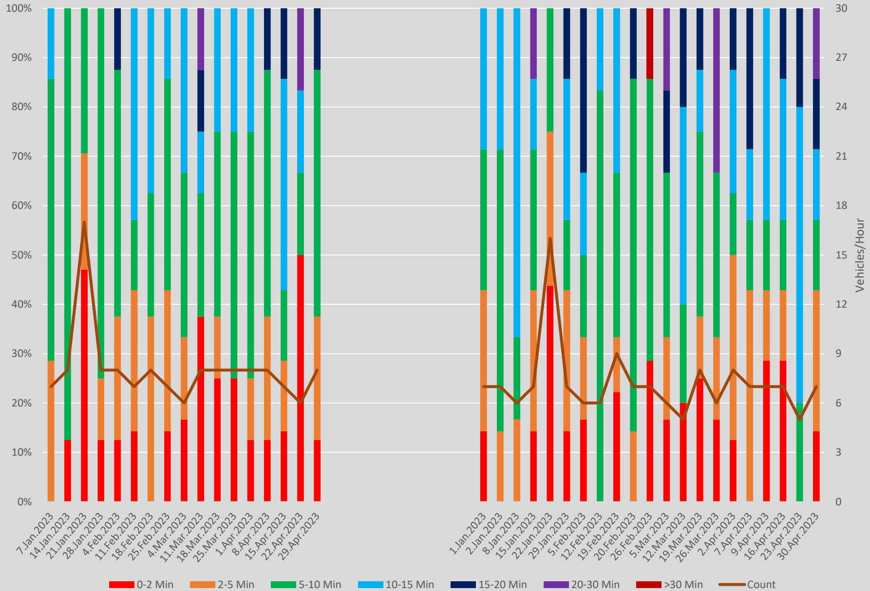
Headway Distributions 501 Queen East of Coxwell Ave. Westbound 1000 to 1100 Weekends
