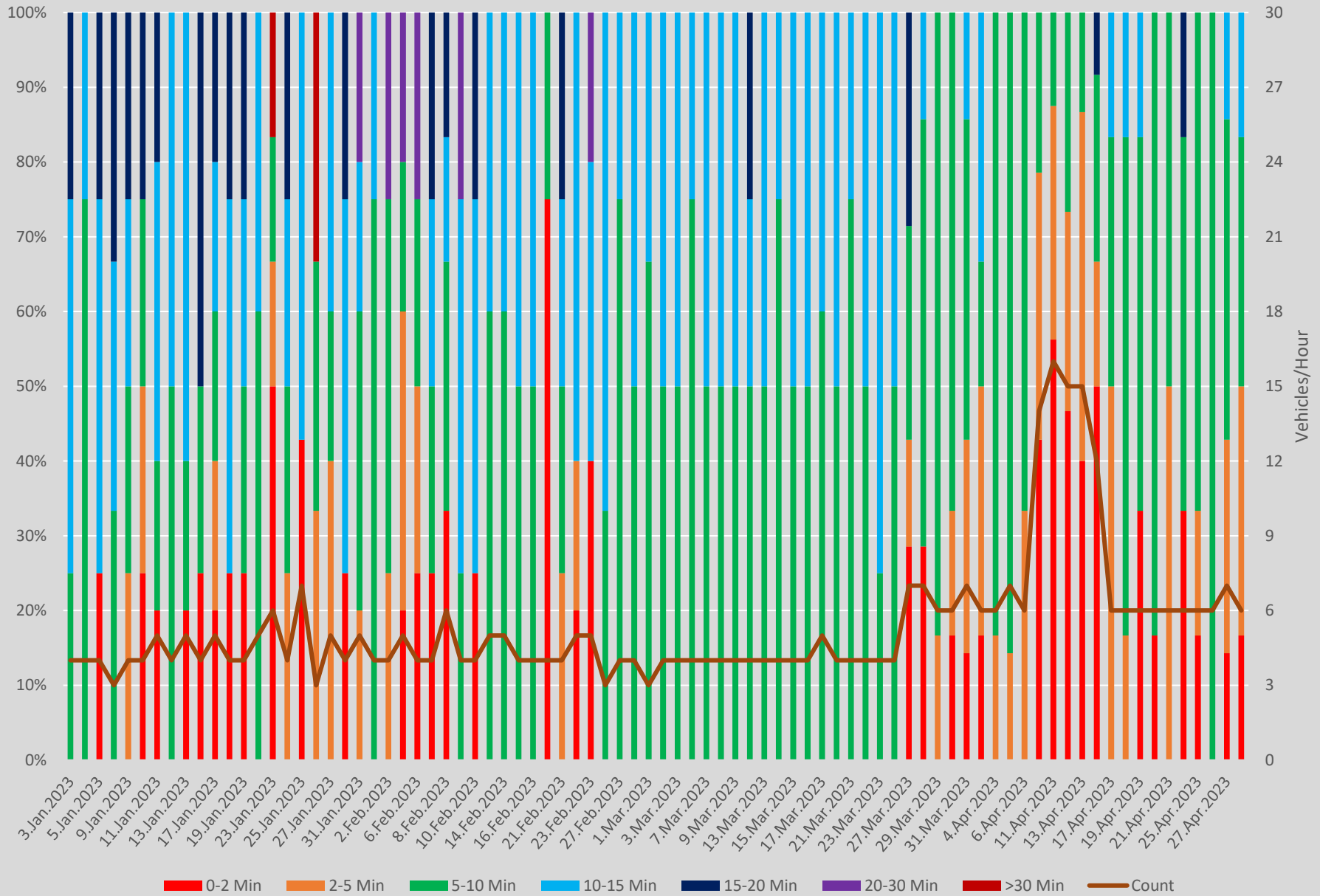
Headway Distributions 501 Queen East of Coxwell Ave. Westbound 600 to 700
