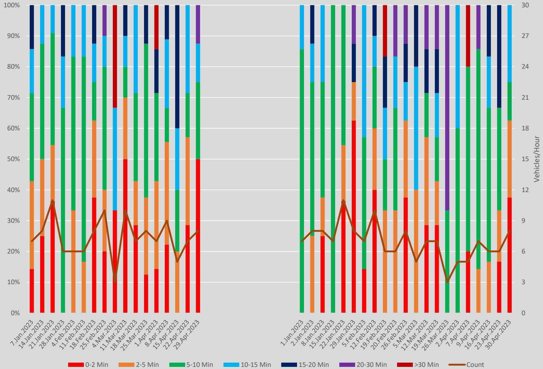
Headway Distributions 501 Queen East of Coxwell Ave. Westbound 2100 to 2200 Weekends
