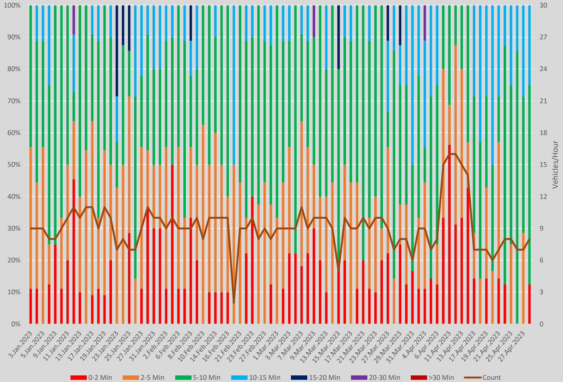
Headway Distributions 501 Queen East of Coxwell Ave. Westbound 900 to 1000
