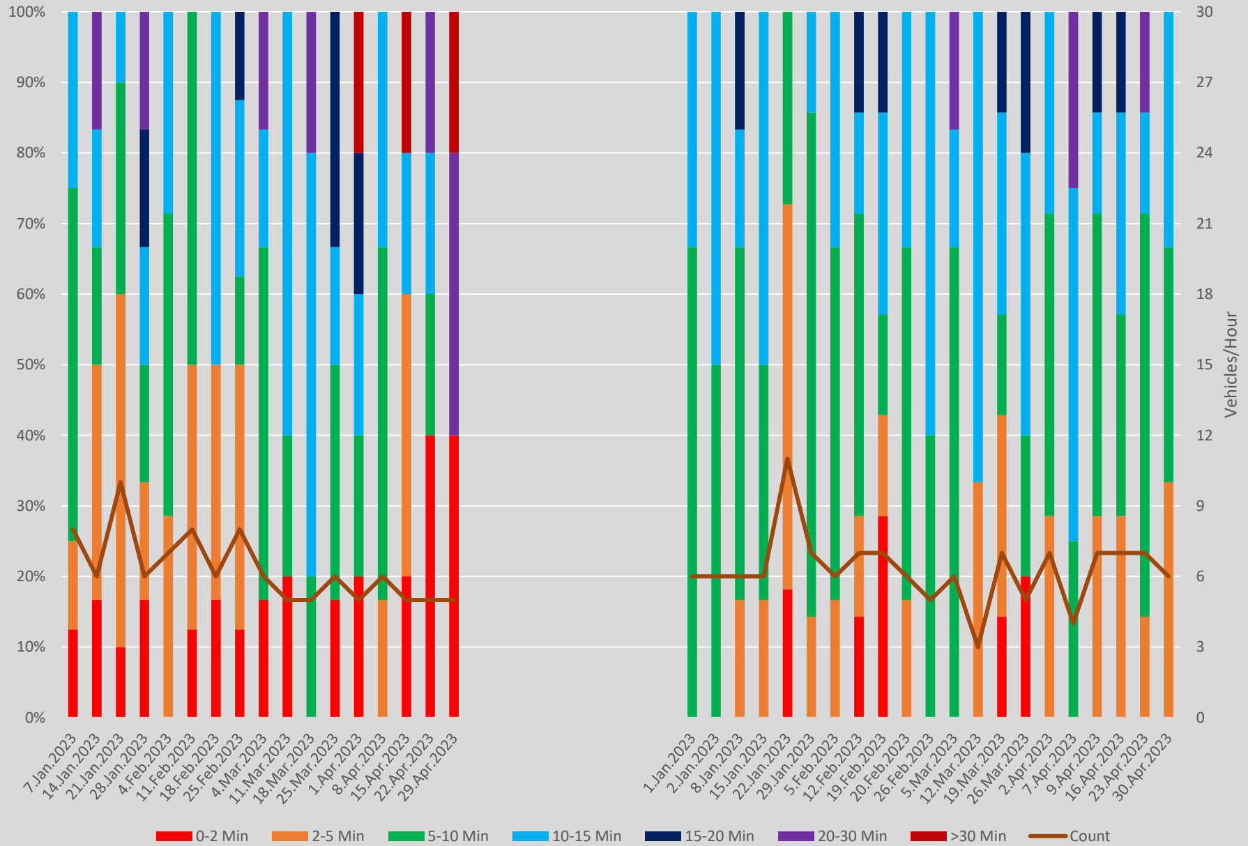
Headway Distributions 501 Queen East of Coxwell Ave. Westbound 2300 to 2400 Weekends
