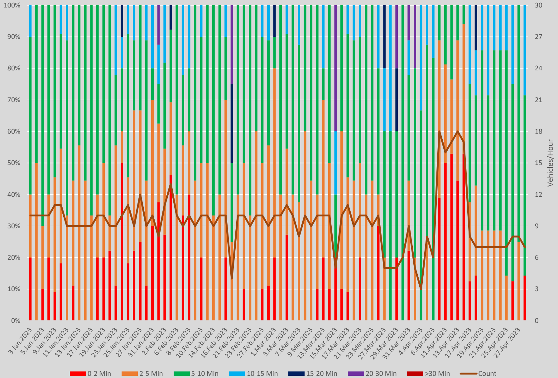
Headway Distributions 501 Queen East of Coxwell Ave. Westbound 800 to 900
