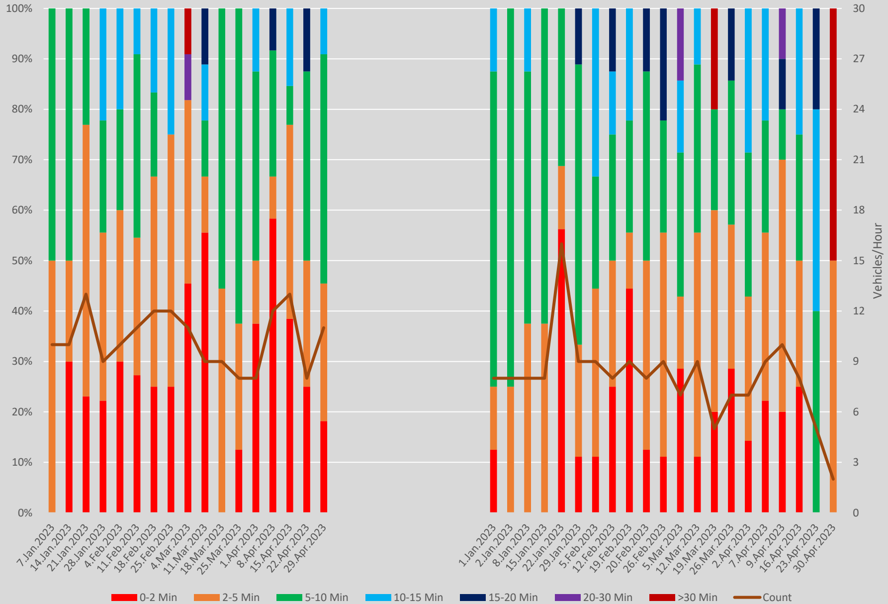
Headway Distributions 501 Queen East of Coxwell Ave. Westbound 1500 to 1600 Weekends
