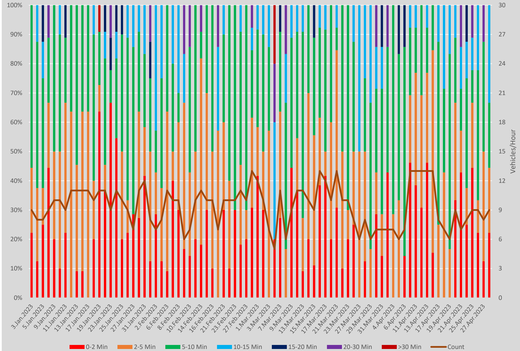
Headway Distributions 501 Queen East of Coxwell Ave. Westbound 1500 to 1600
