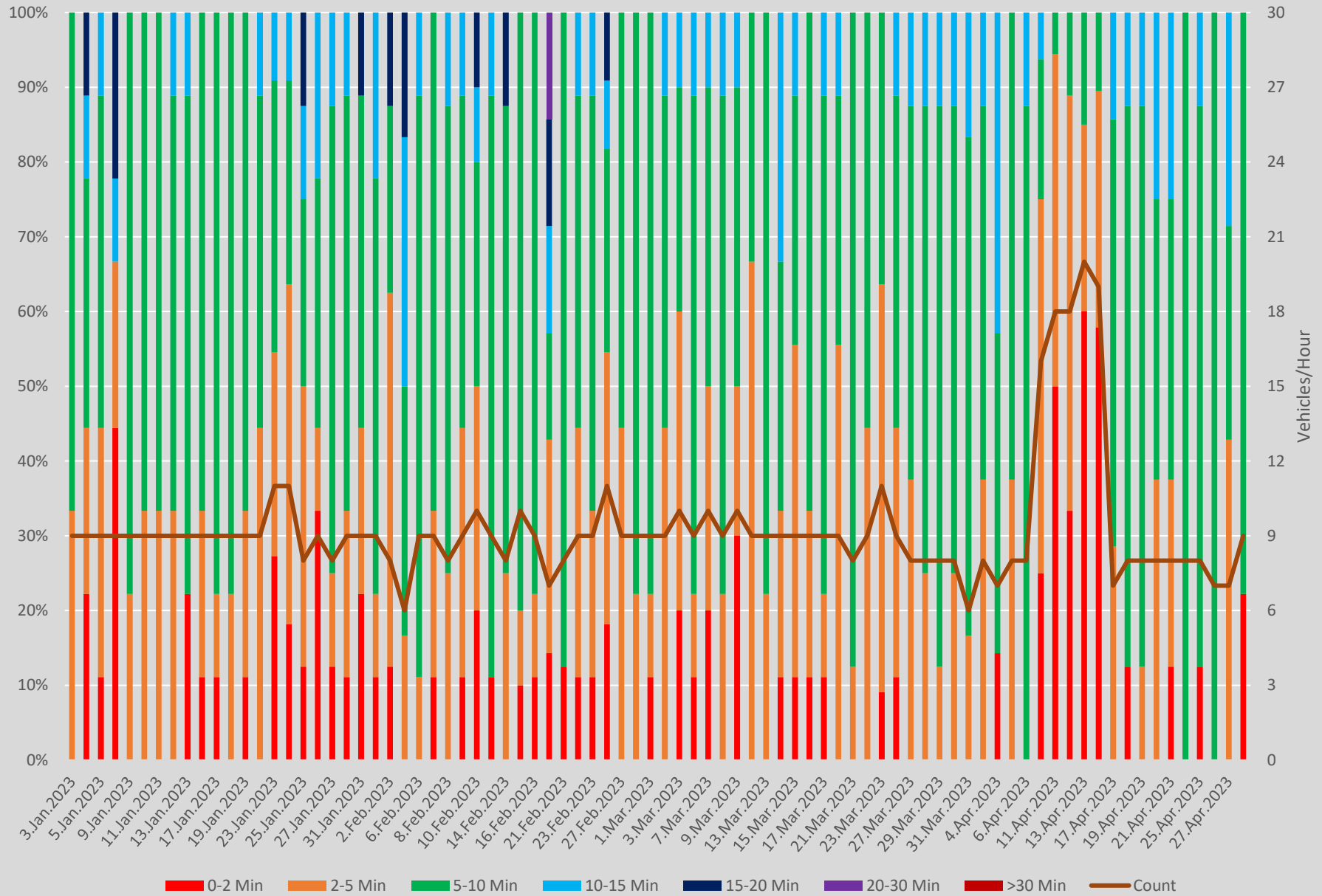
Headway Distributions 501 Queen East of Coxwell Ave. Westbound 700 to 800
