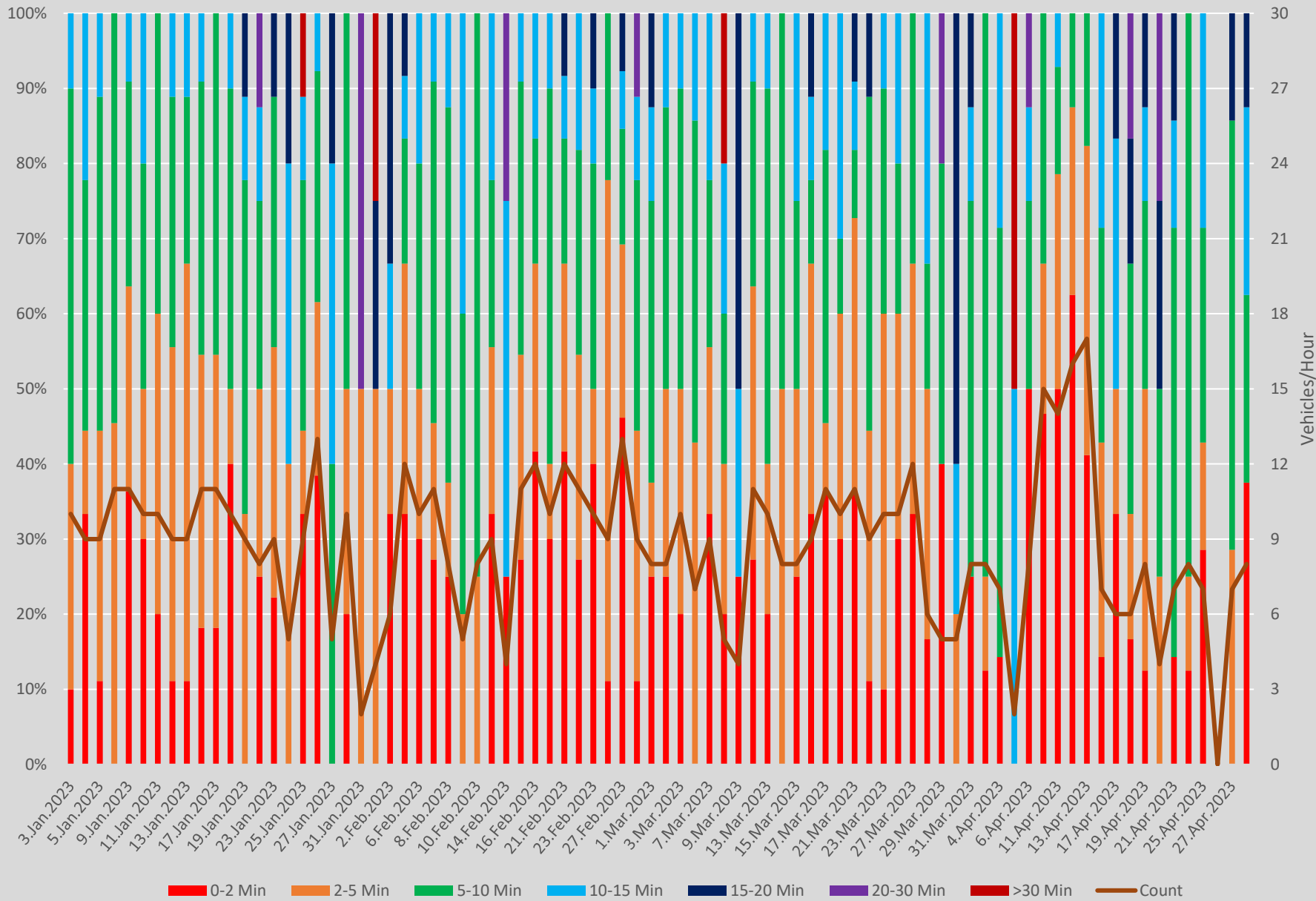
Headway Distributions 501 Queen East of Coxwell Ave. Westbound 1800 to 1900
