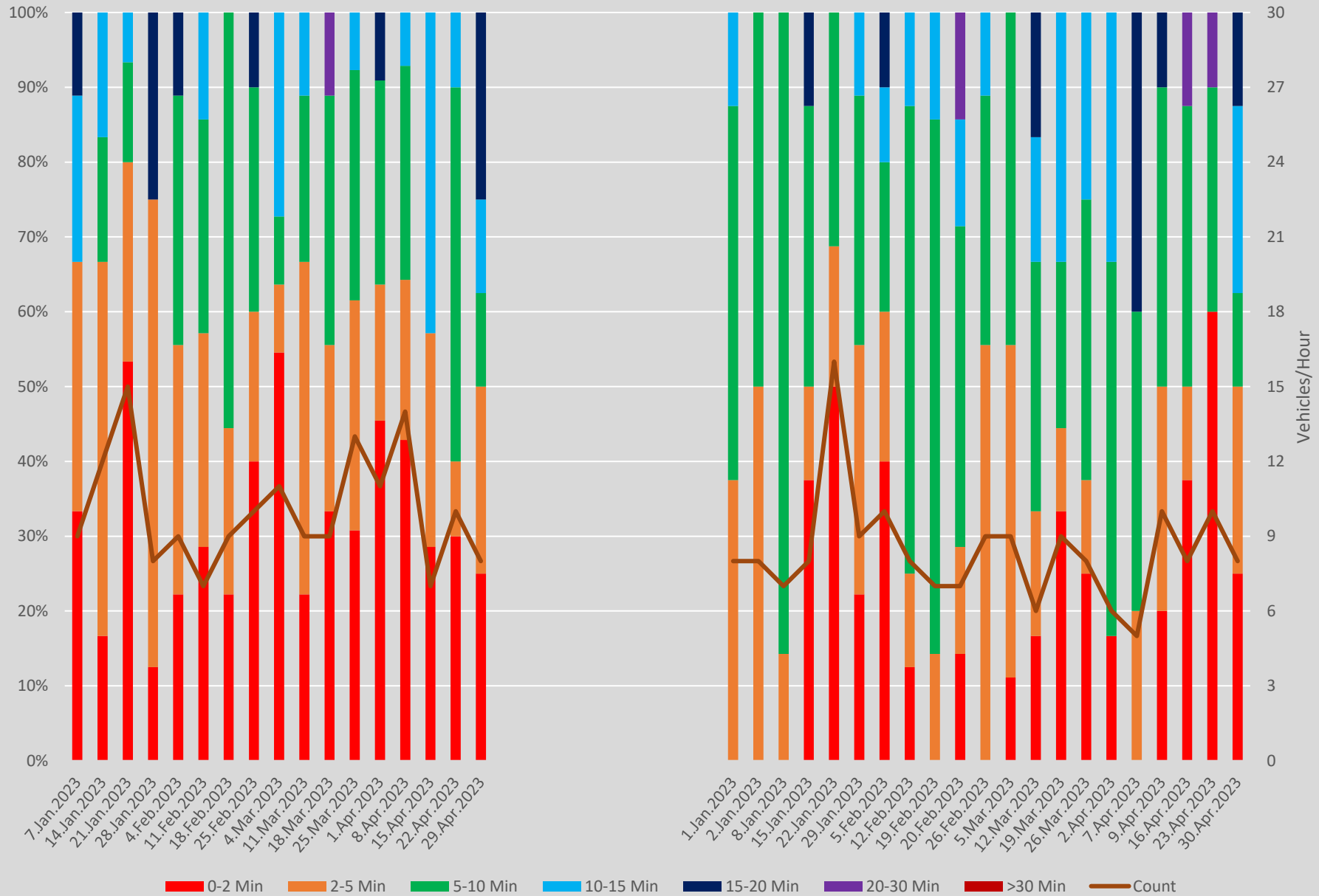
Headway Distributions 501 Queen East of Coxwell Ave. Westbound 1300 to 1400 Weekends
