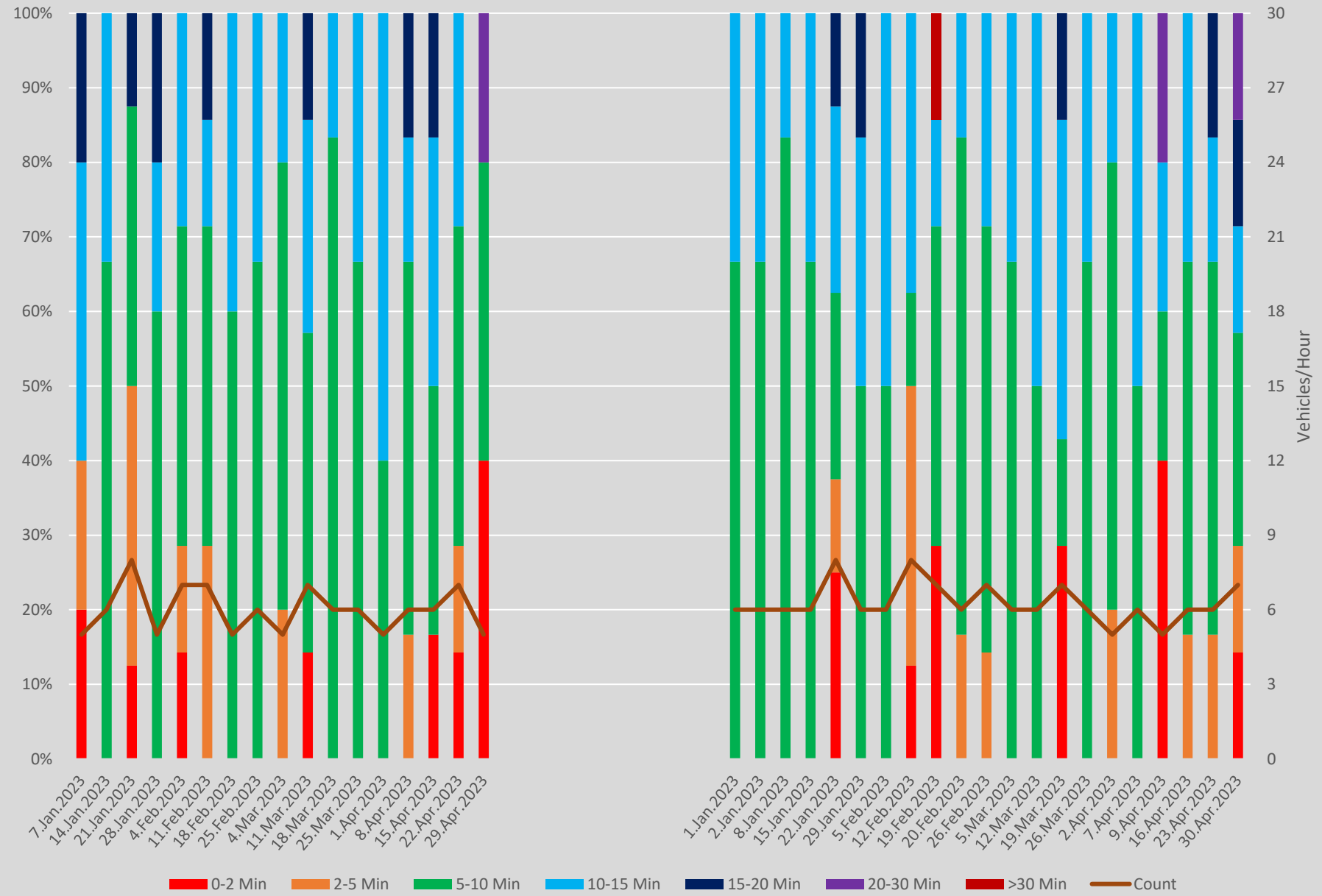
Headway Distributions 501 Queen East of Coxwell Ave. Westbound 700 to 800 Weekends
