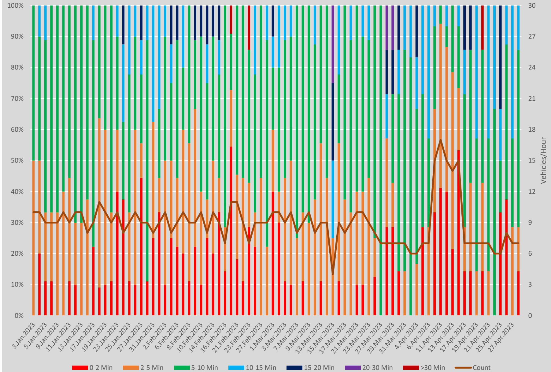
Headway Distributions 501 Queen East of Coxwell Ave. Westbound 1000 to 1100
