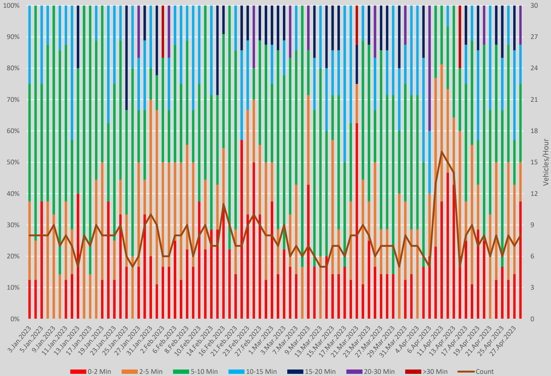
Headway Distributions 501 Queen East of Coxwell Ave. Westbound 2000 to 2100
