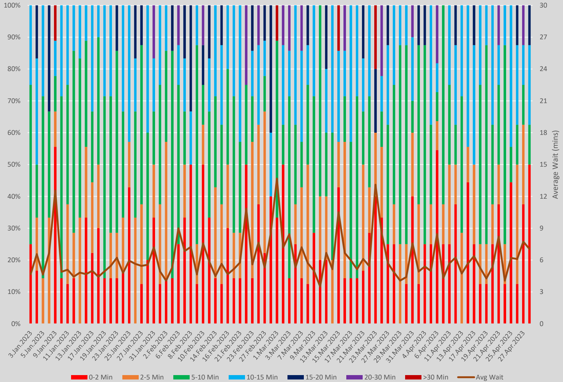
Headway Distributions and Wait Times 35 Jane Lawrence Southbound 2100 to 2200
