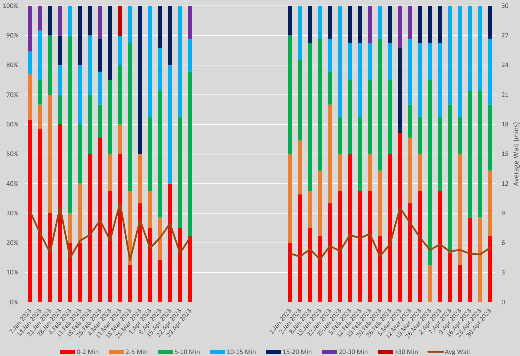
Headway Distributions and Wait Times 35 Jane Lawrence Southbound 2000 to 2100 Weekends
