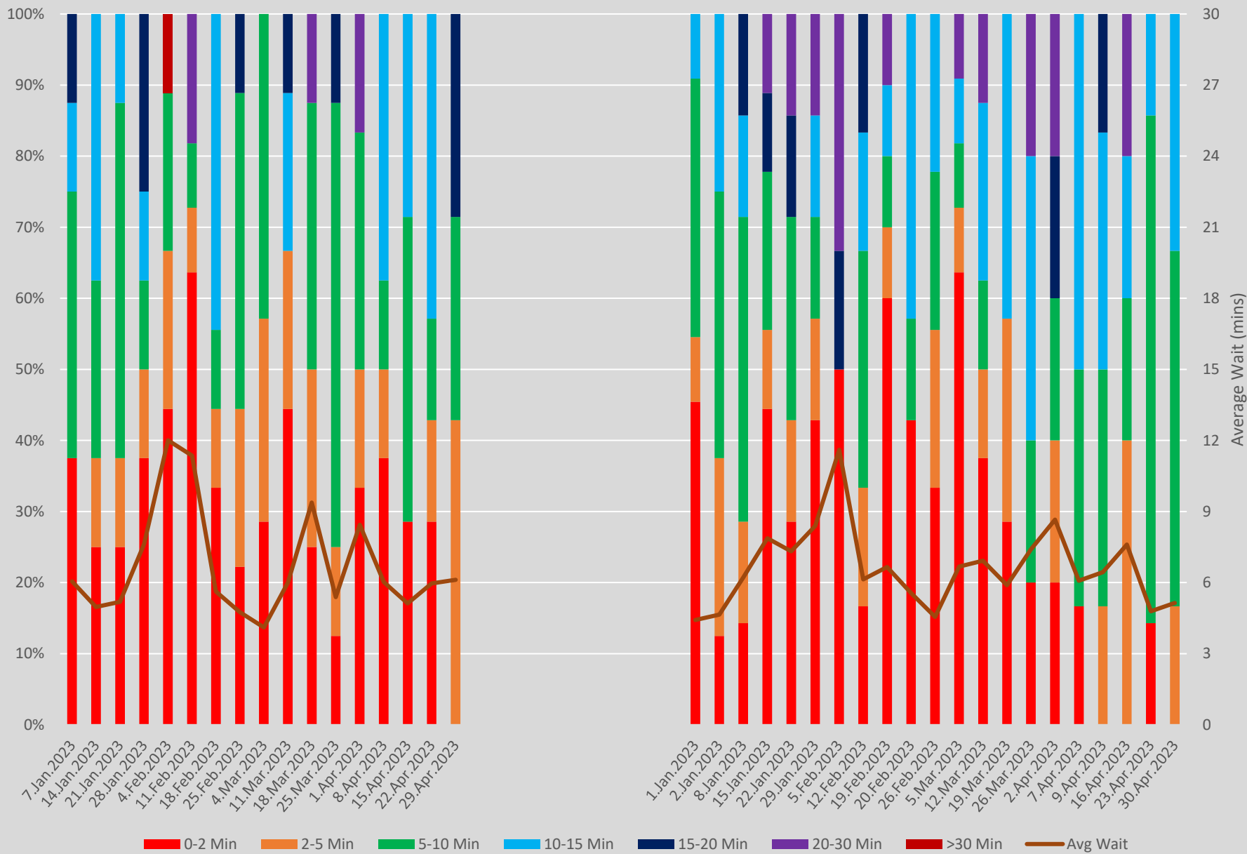
Headway Distributions and Wait Times 35 Jane Lawrence Southbound 1300 to 1400 Weekends
