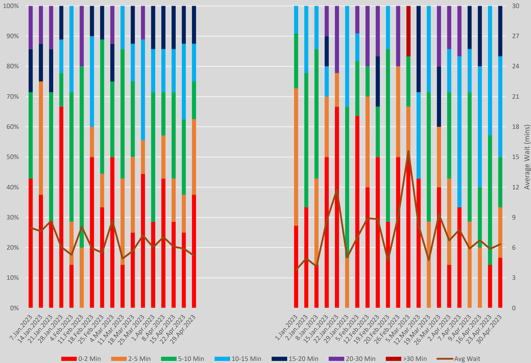
Headway Distributions and Wait Times 35 Jane Lawrence Southbound 1600 to 1700 Weekends
