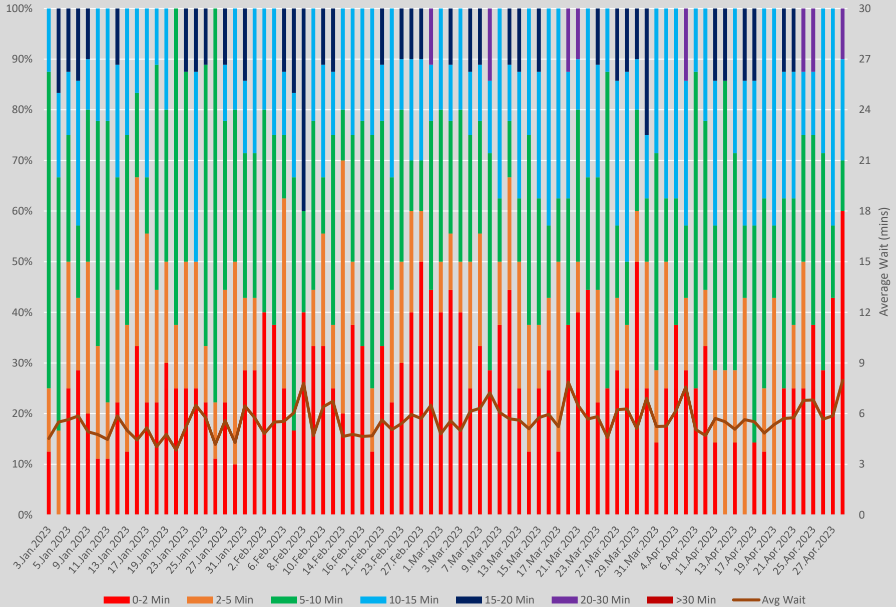
Headway Distributions and Wait Times 35 Jane Lawrence Southbound 1000 to 1100
