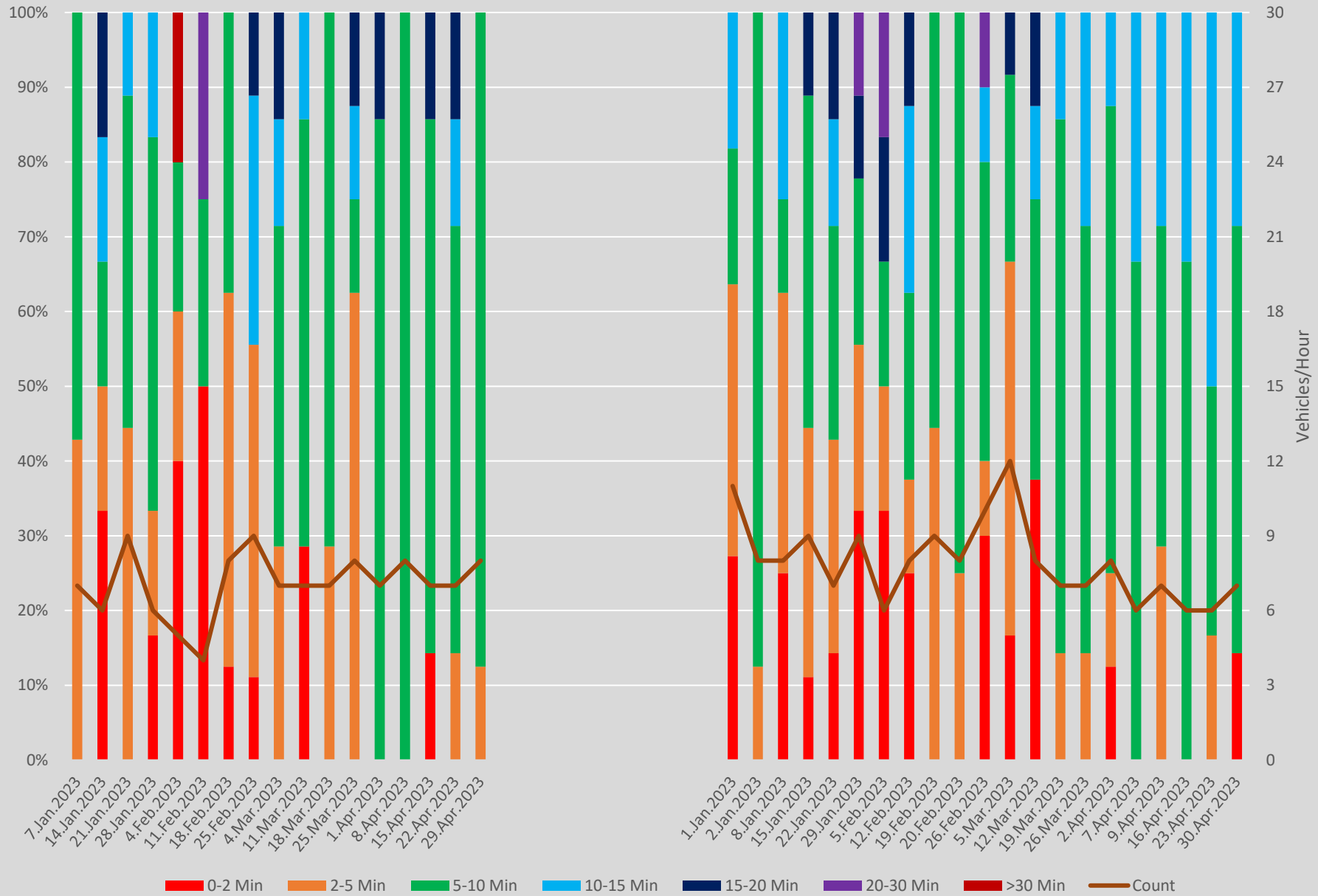
Headway Distributions 35 Jane N of Jane Stn Northbound 1300 to 1400 Weekends
