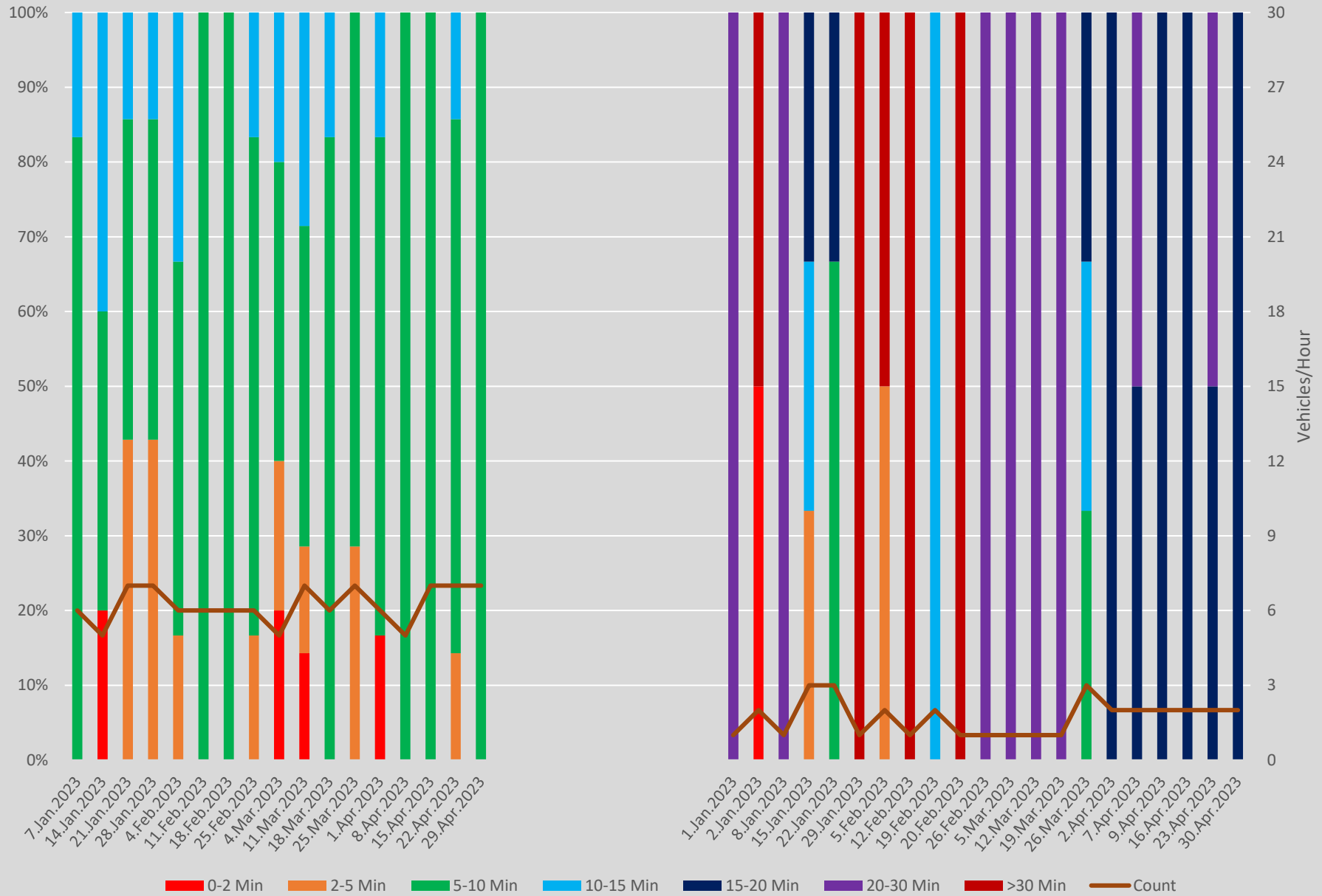
Headway Distributions 35 Jane N of Jane Stn Northbound 600 to 700 Weekends
