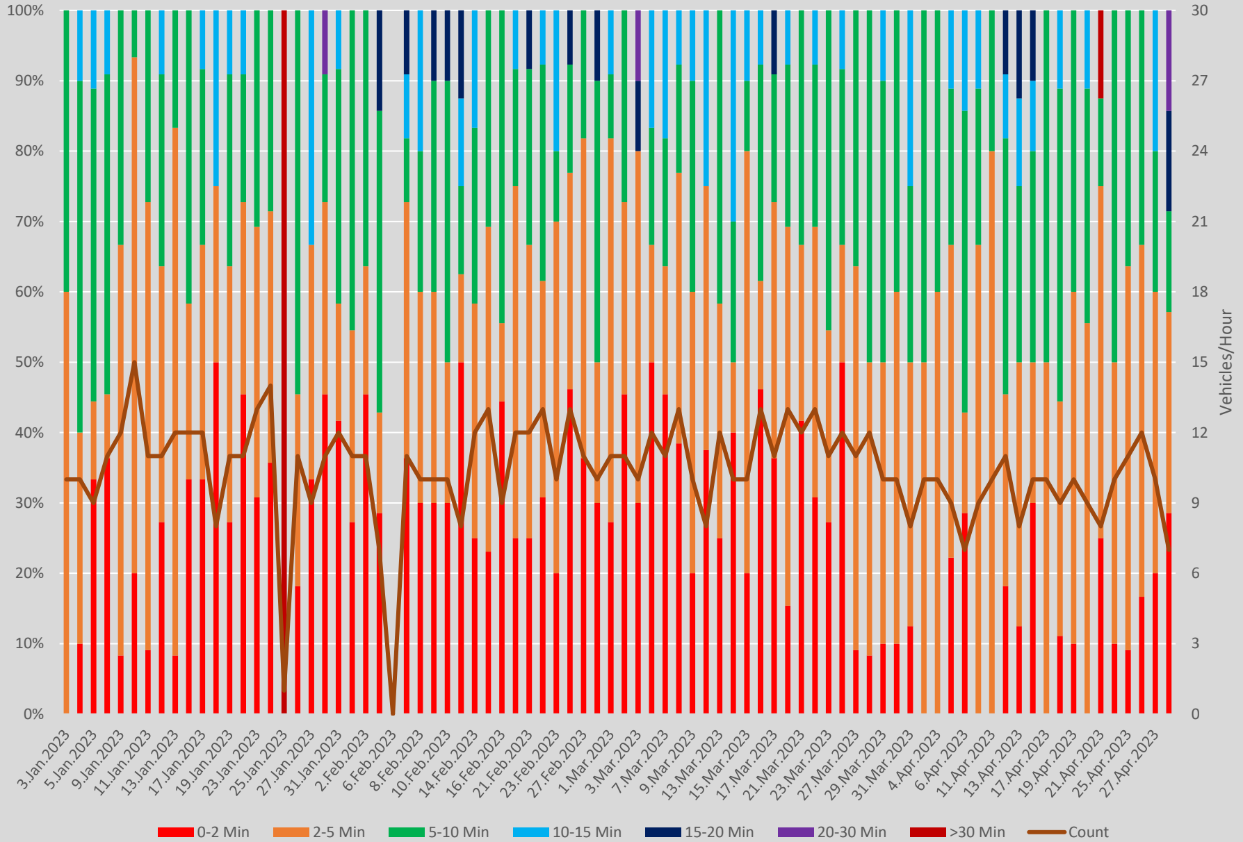
Headway Distributions 35 Jane N of Jane Stn Northbound 1600 to 1700
