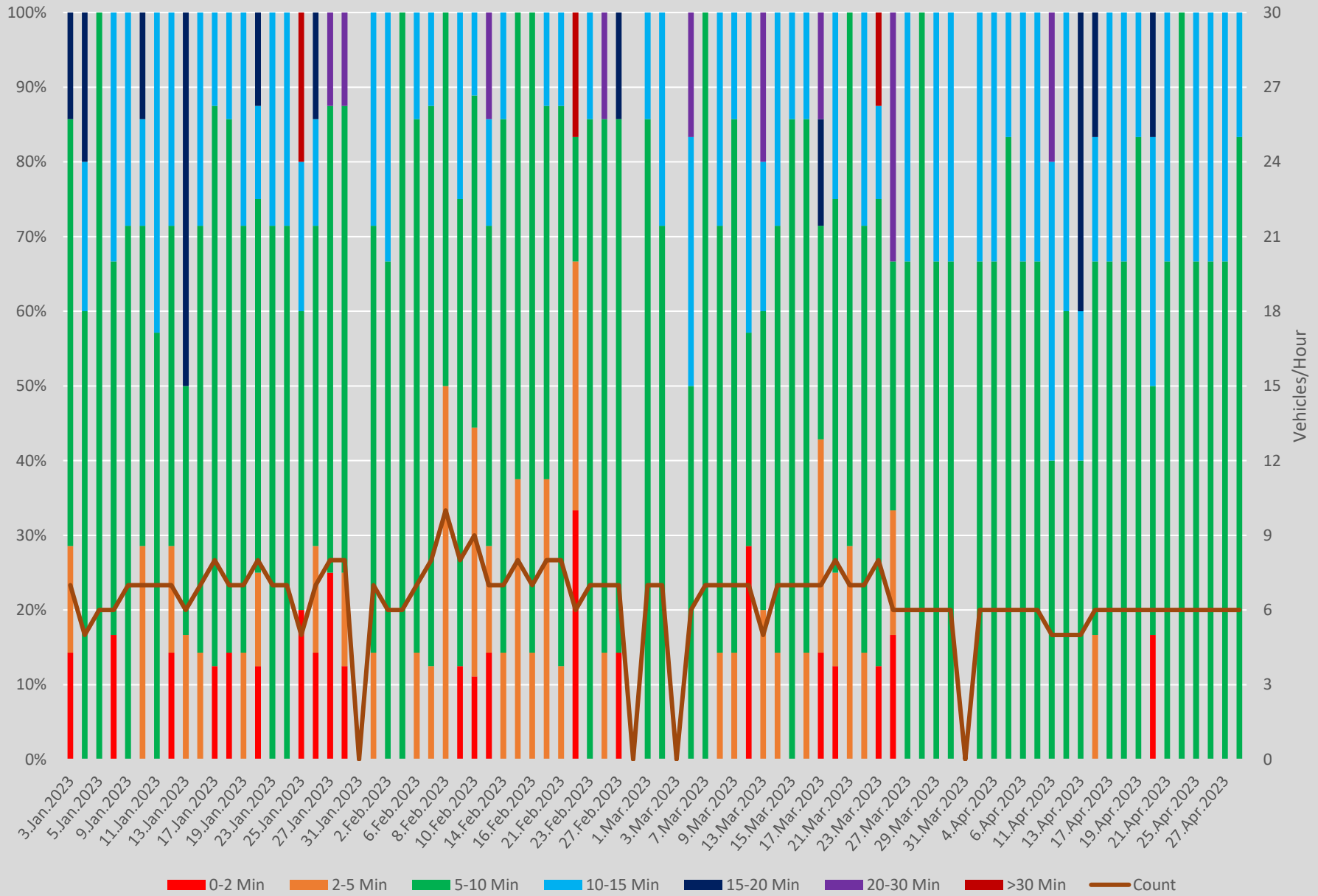
Headway Distributions 35 Jane N of Jane Stn Northbound 2400 to 2500
