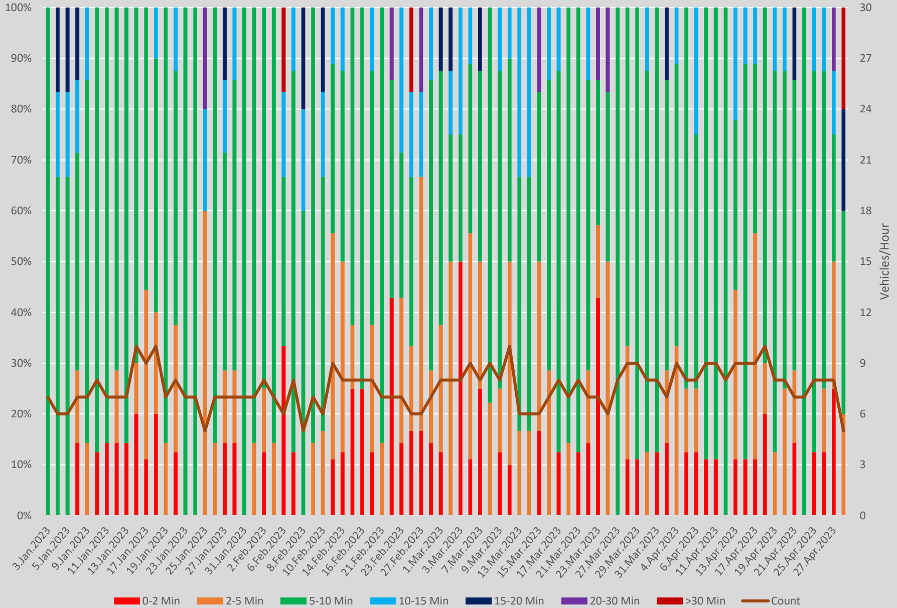
Headway Distributions 35 Jane N of Jane Stn Northbound 2000 to 2100
