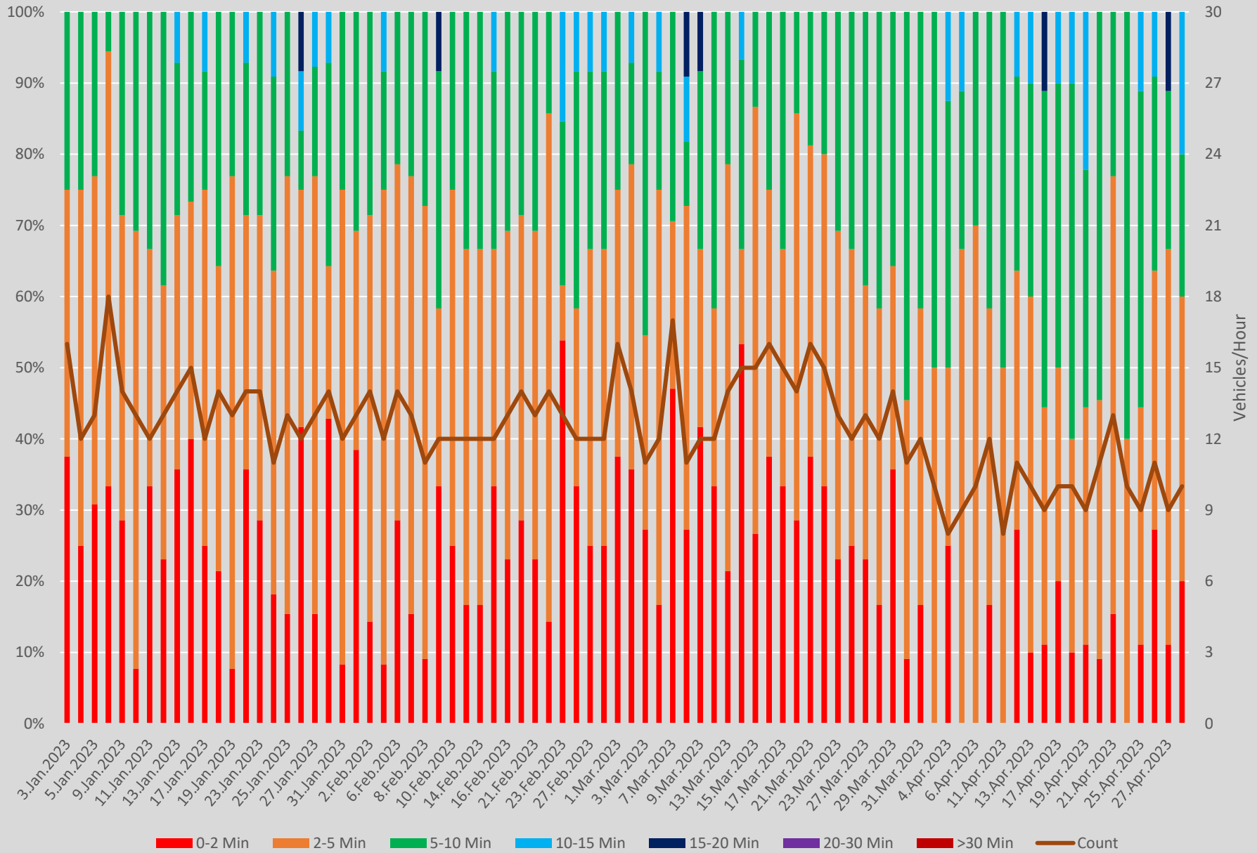
Headway Distributions 35 Jane N of Jane Stn Northbound 800 to 900
