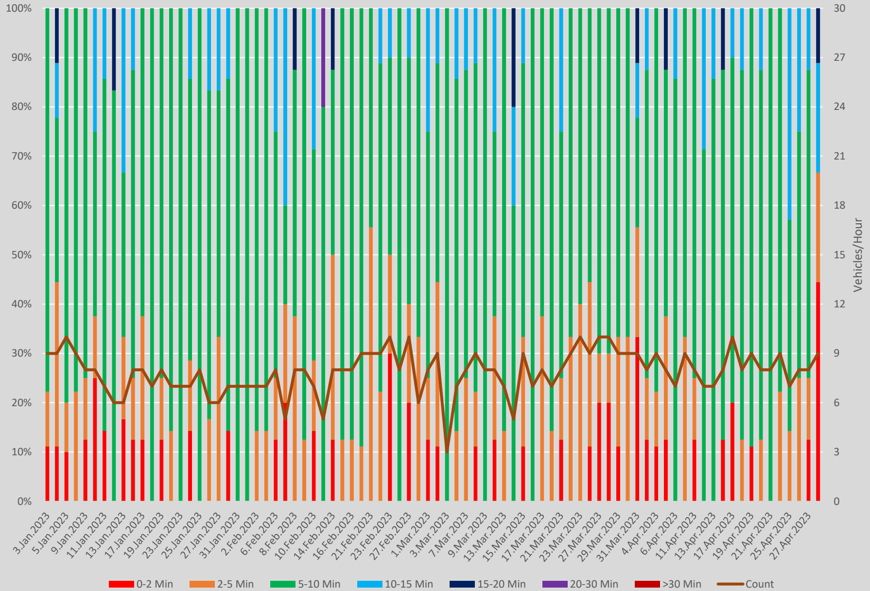
Headway Distributions 35 Jane N of Jane Stn Northbound 1100 to 1200
