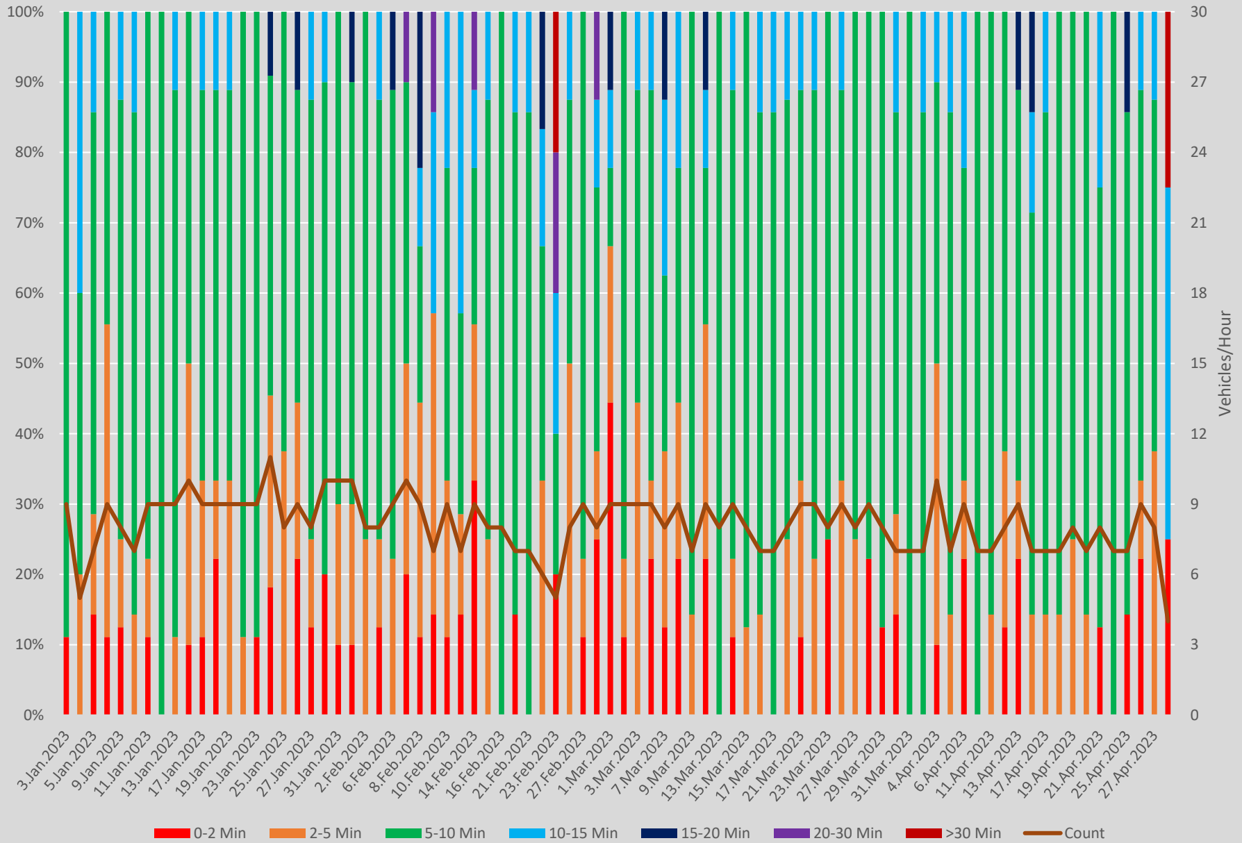
Headway Distributions 35 Jane N of Jane Stn Northbound 1000 to 1100
