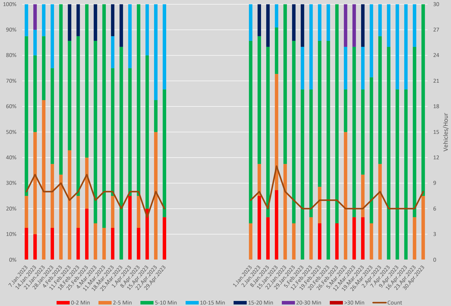
Headway Distributions 35 Jane N of Jane Stn Northbound 2200 to 2300 Weekends
