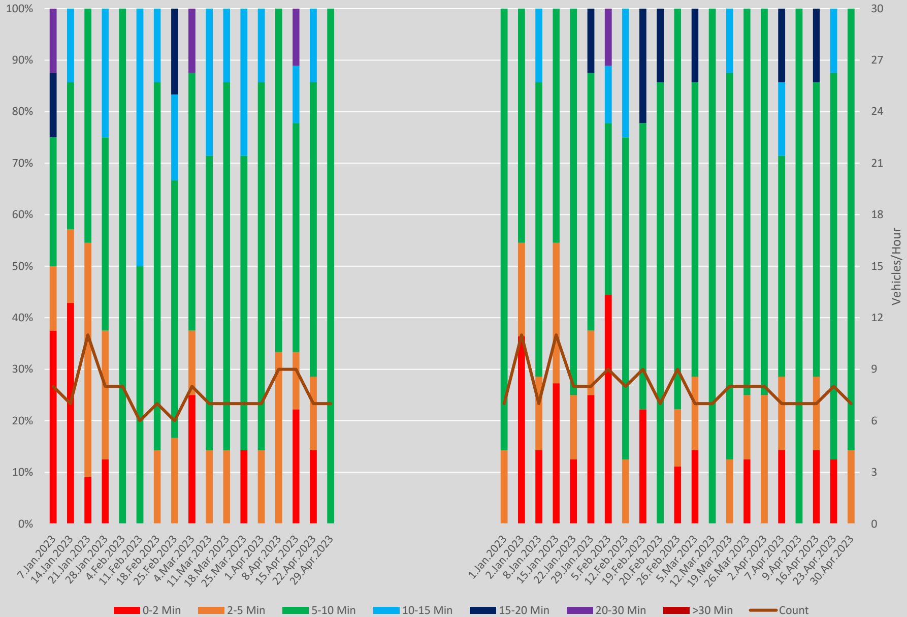
Headway Distributions 35 Jane N of Jane Stn Northbound 2100 to 2200 Weekends
