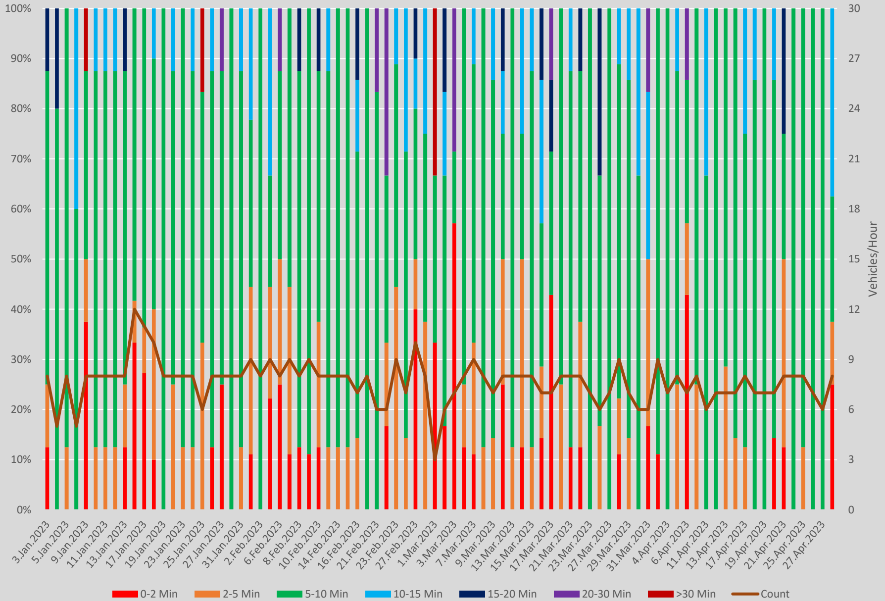
Headway Distributions 35 Jane N of Jane Stn Northbound 2100 to 2200
