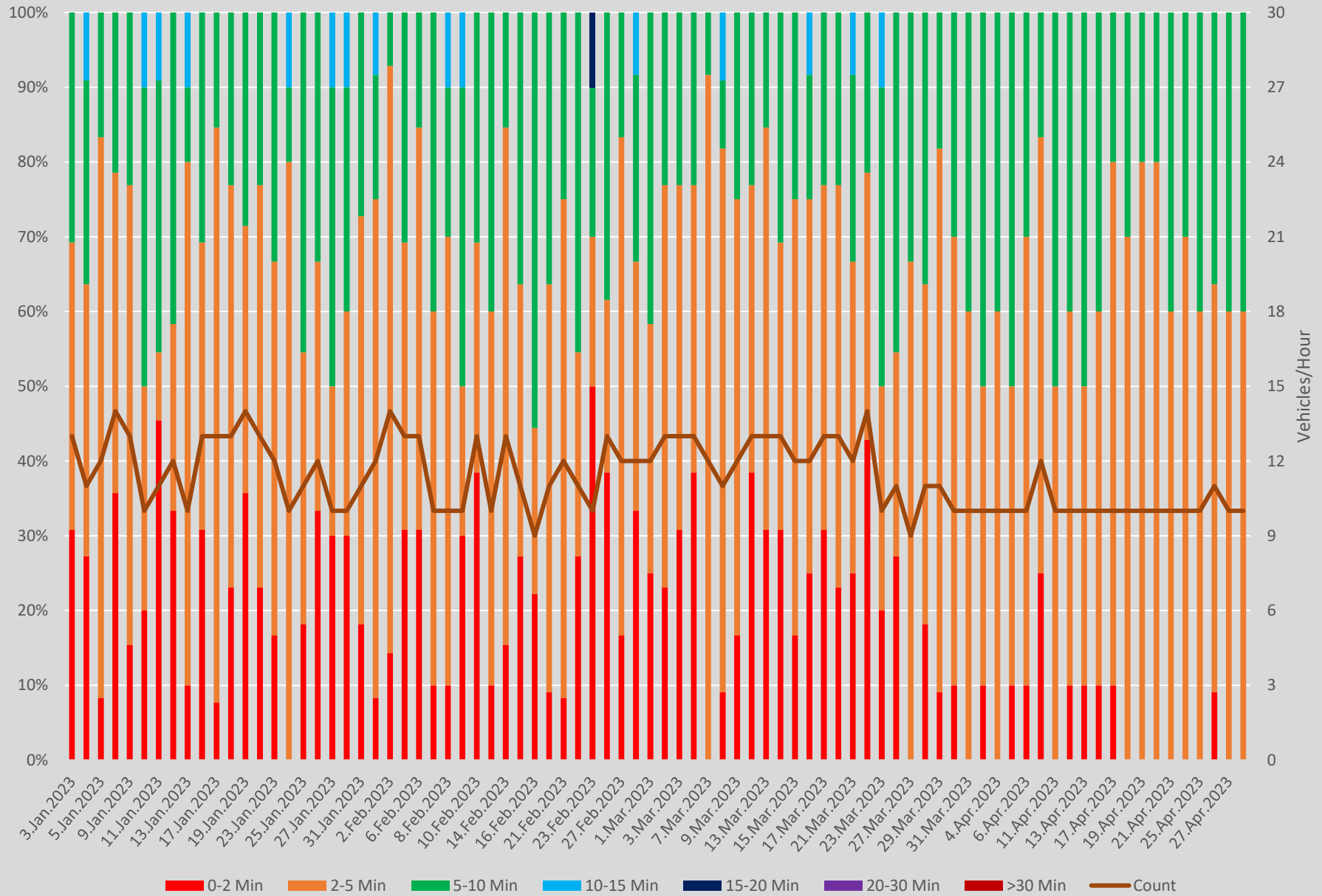
Headway Distributions 35 Jane N of Jane Stn Northbound 600 to 700
