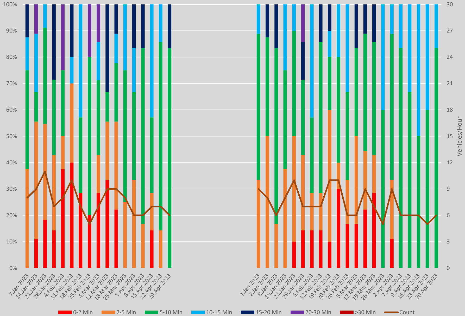
Headway Distributions 35 Jane N of Jane Stn Northbound 1200 to 1300 Weekends
