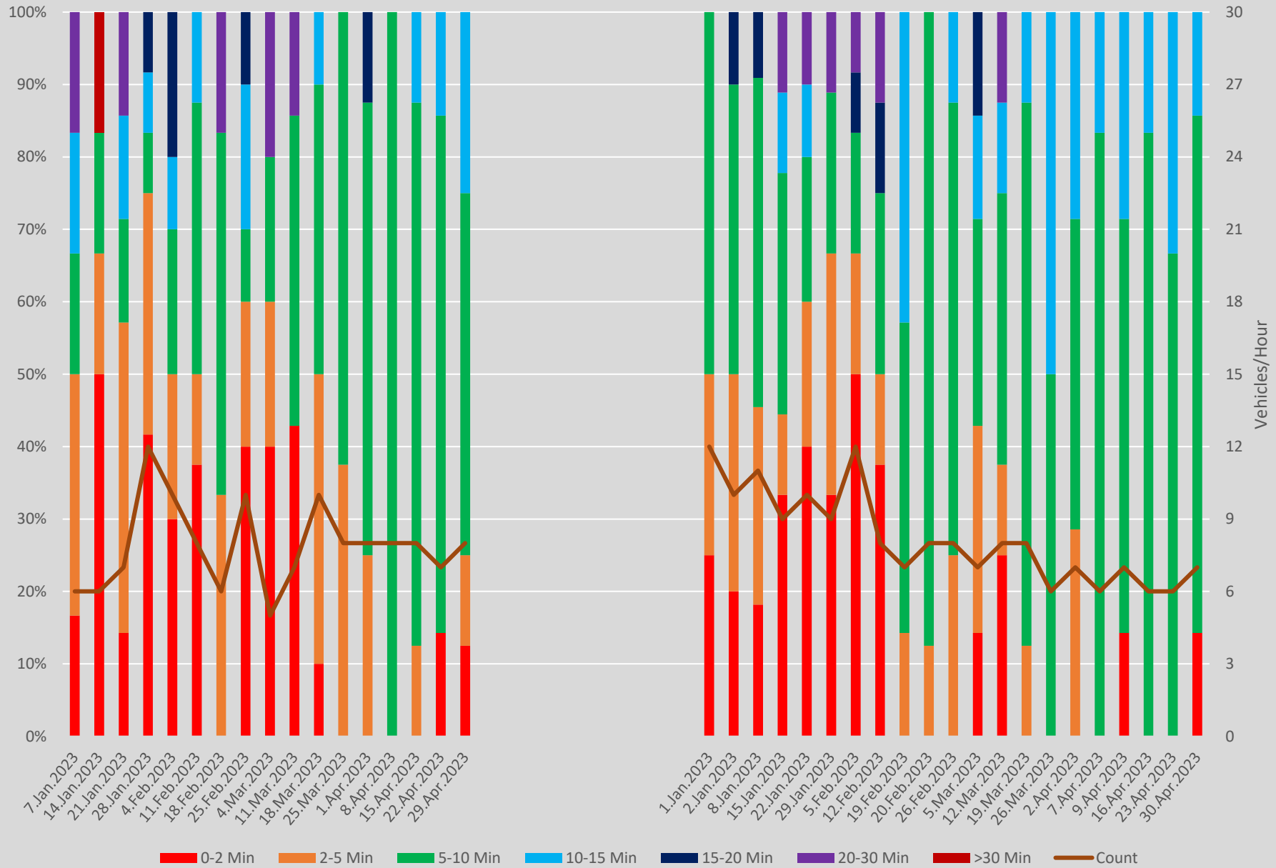
Headway Distributions 35 Jane N of Jane Stn Northbound 1800 to 1900 Weekends
