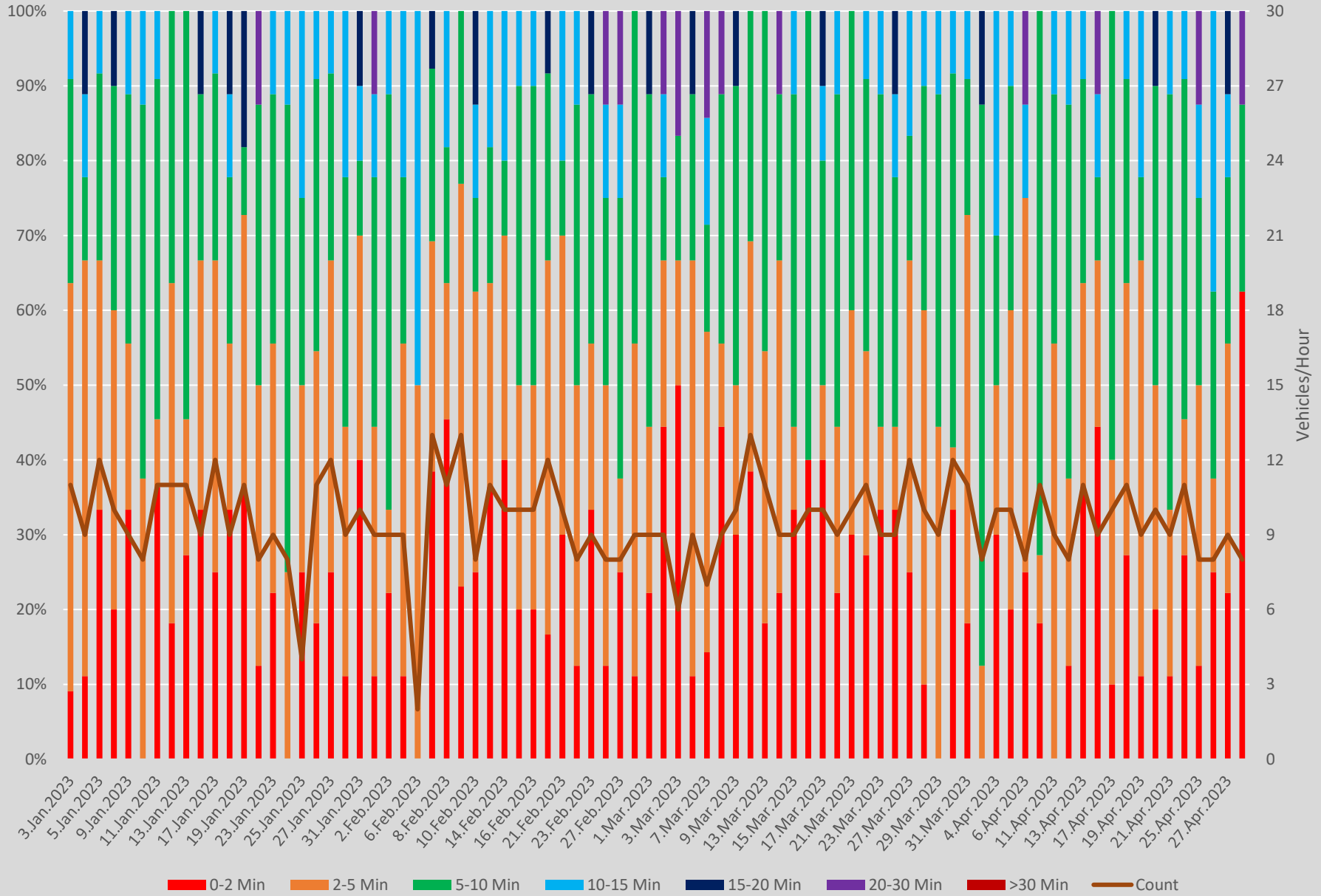
Headway Distributions 35 Jane N of Jane Stn Northbound 1500 to 1600
