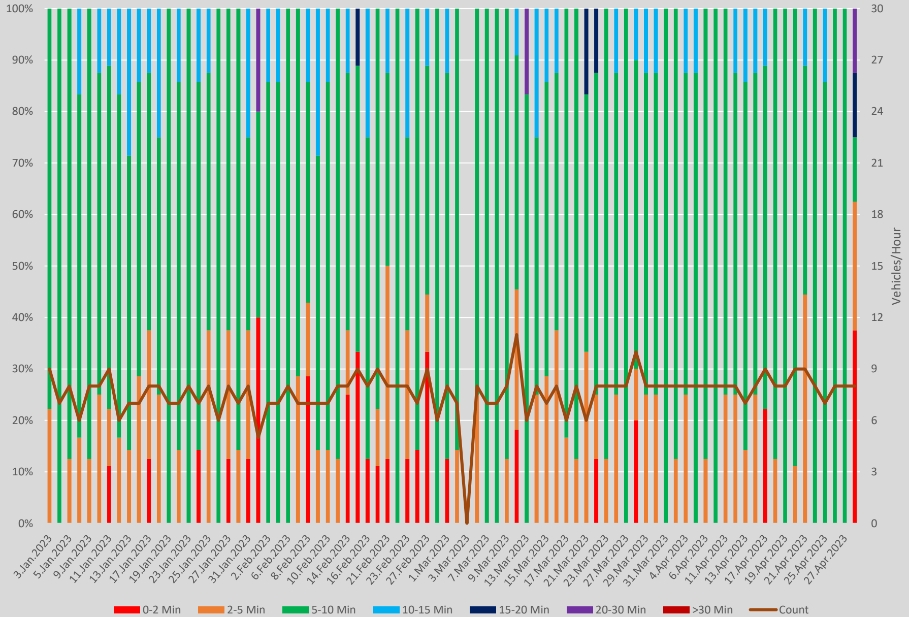
Headway Distributions 35 Jane N of Jane Stn Northbound 1300 to 1400
