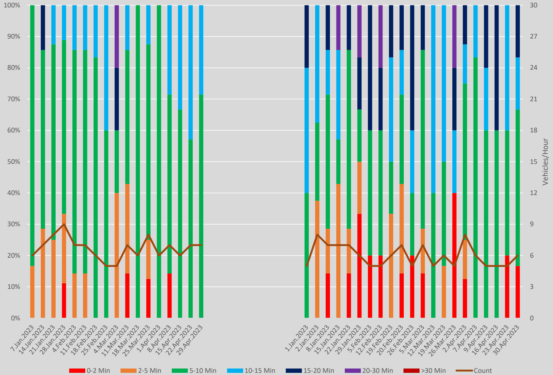
Headway Distributions 35 Jane N of Jane Stn Northbound 800 to 900 Weekends
