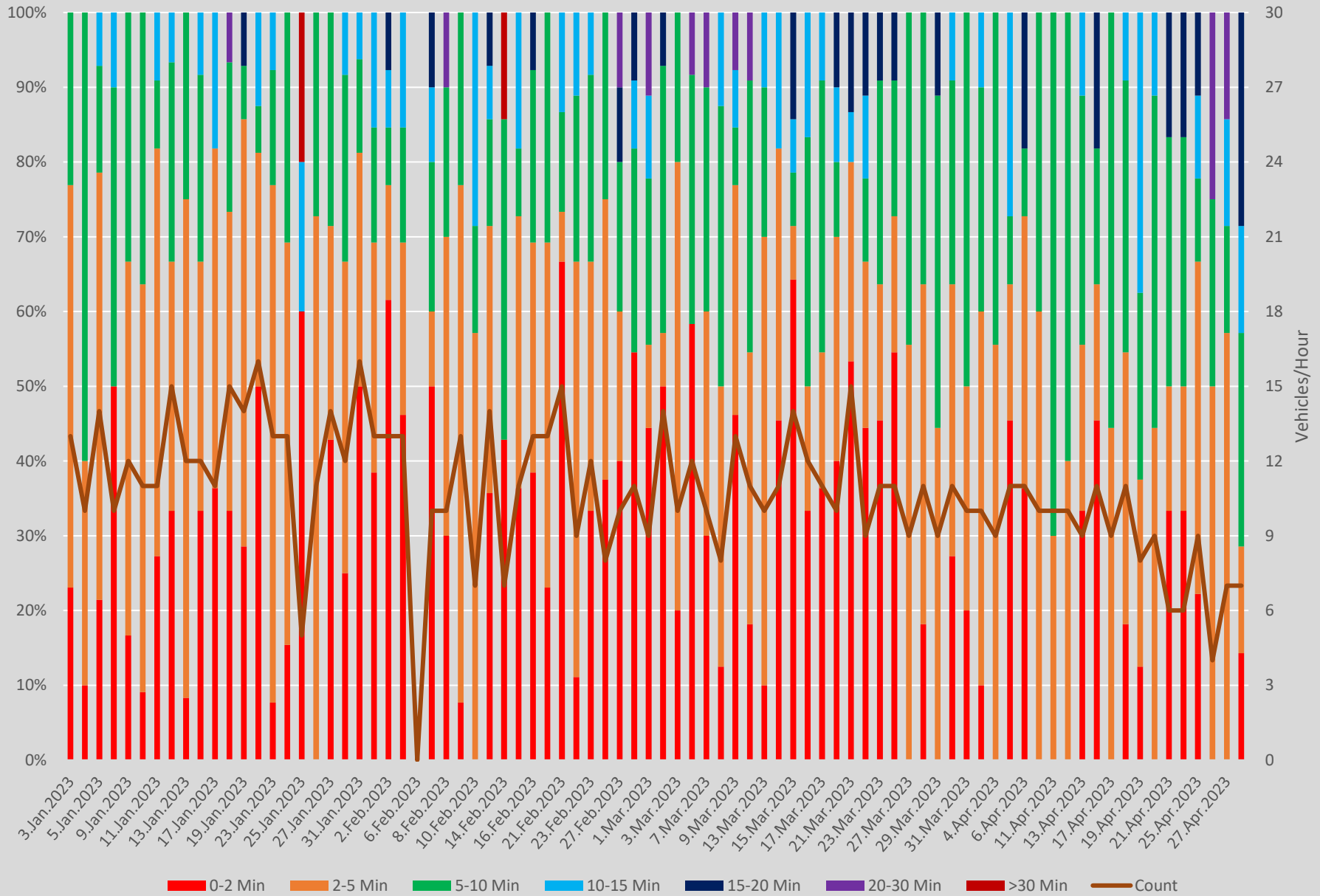
Headway Distributions 35 Jane N of Jane Stn Northbound 1700 to 1800
