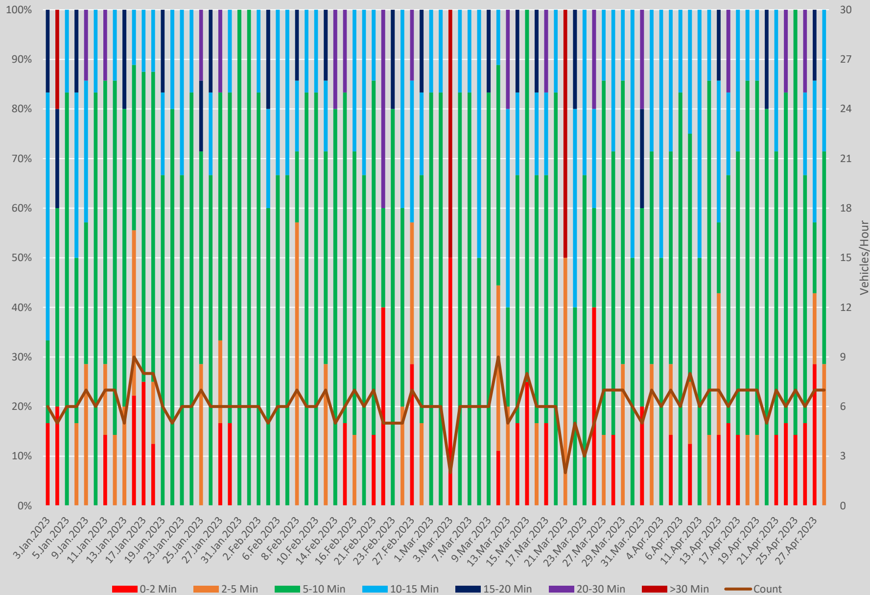
Headway Distributions 35 Jane N of Jane Stn Northbound 2300 to 2400
