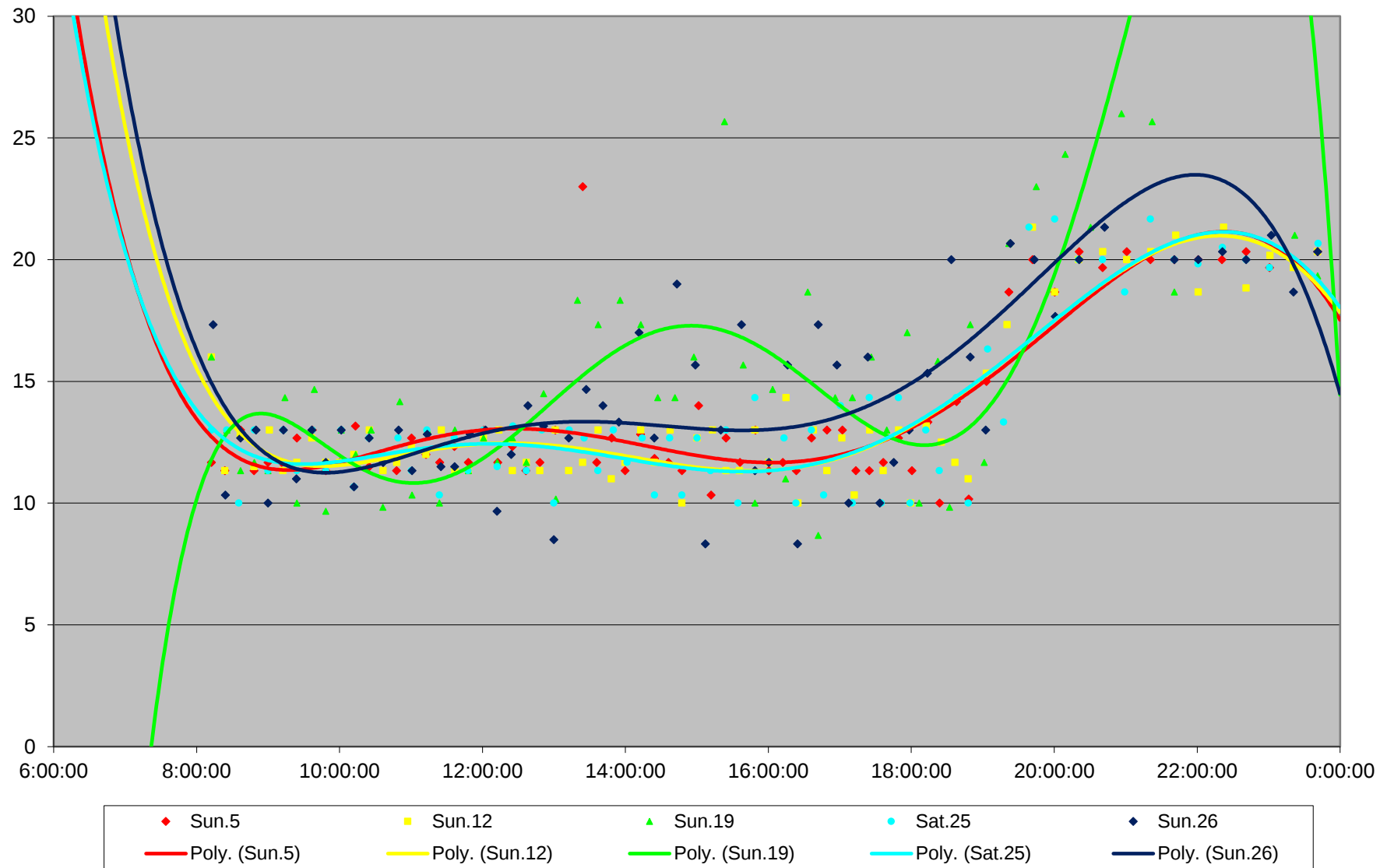
92 Woodbine South Headways at Danforth Ave Southbound December 2021 Sundays/Holidays
