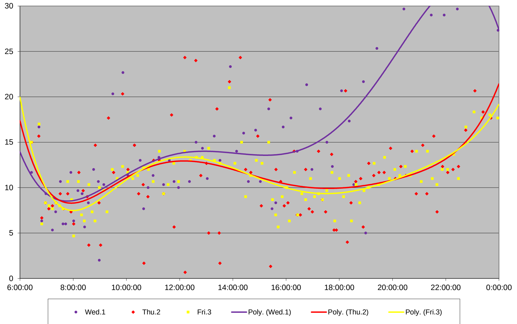
92 Woodbine South Headways at Sarah Ashbridge Northbound December 2021 Week 1
