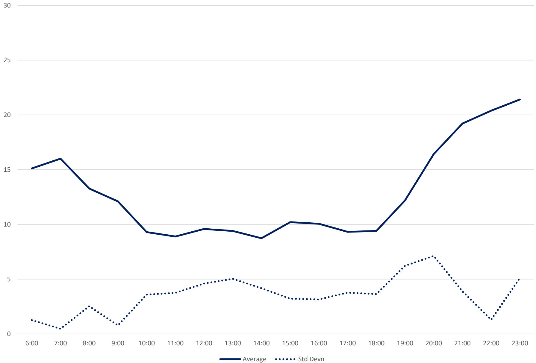
92 Woodbine South Headways at Sarah Ashbridge Northbound October 2021 Sunday Statistics
