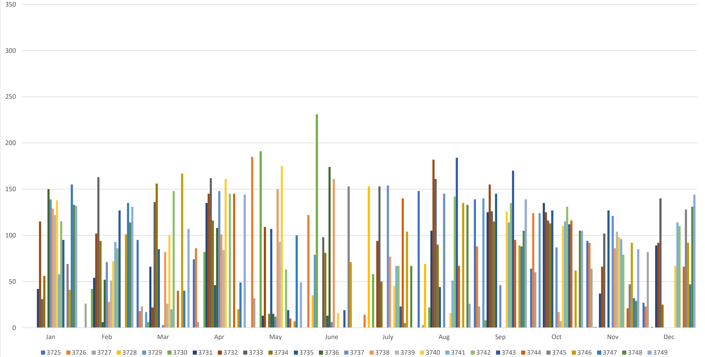
TTC eBus Vehicle Service Hours by Month - Jan to Dec 2021 - Proterra
