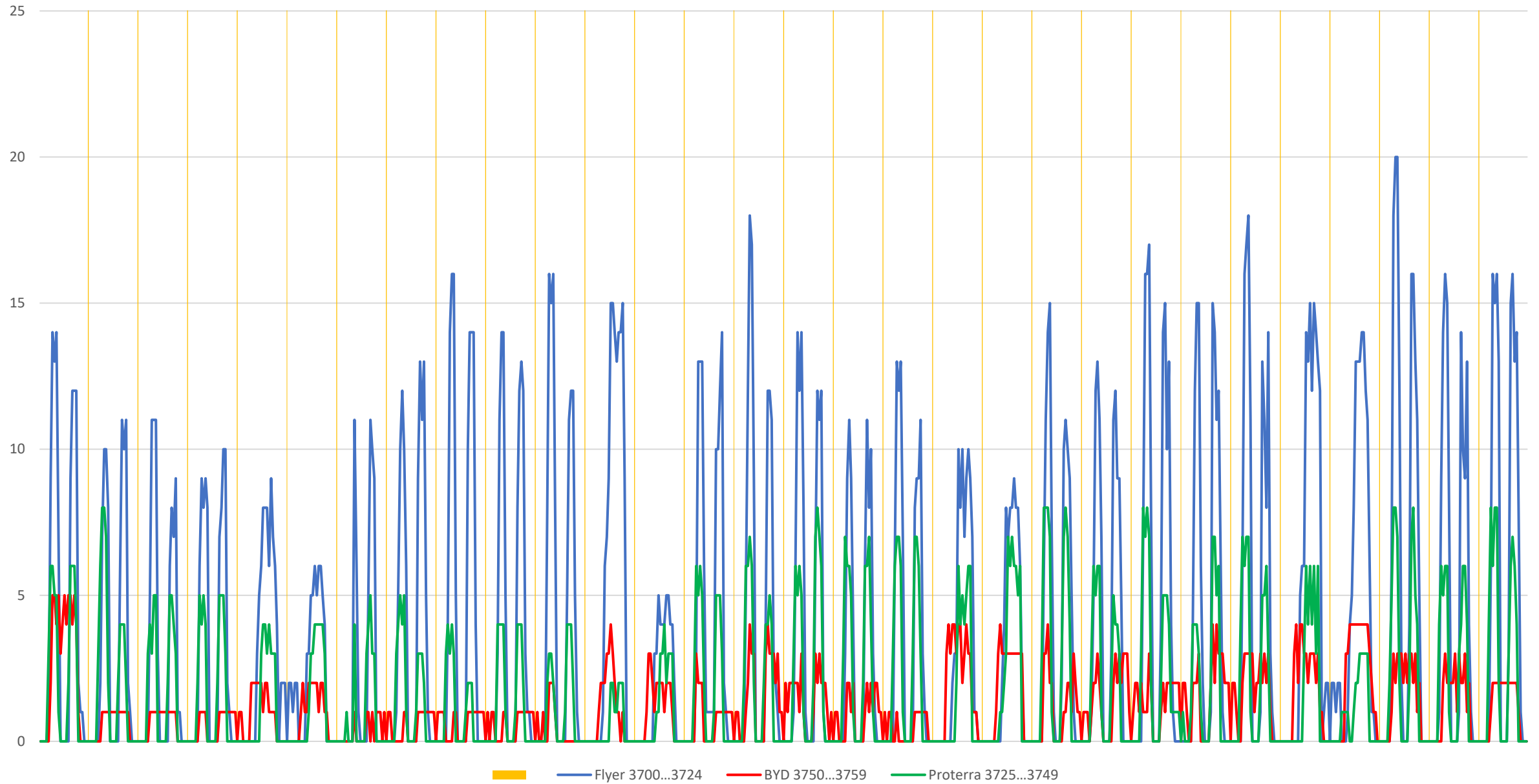
TTC Ebus Vehicles in Service by Hour - June 2021
