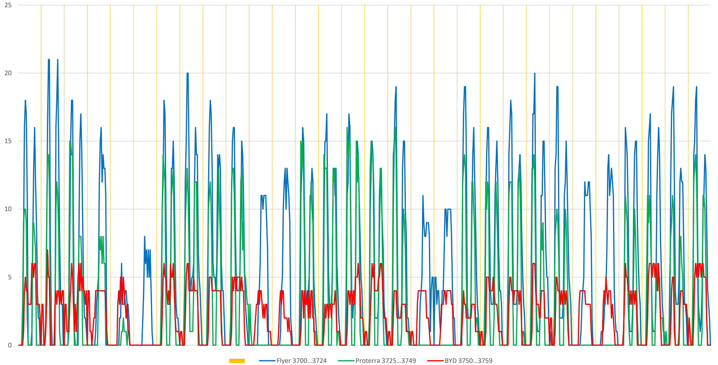
TTC Ebus Vehicles in Service by Hour - September 2021
