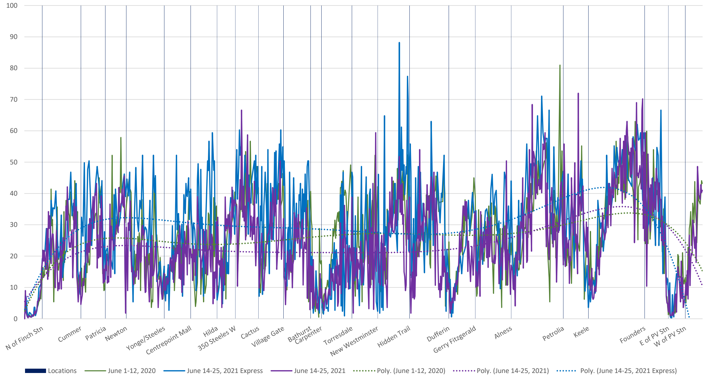
60 Steeles West Eastbound June 2020 vs June 2021 Average Speed 1800 to 1900
