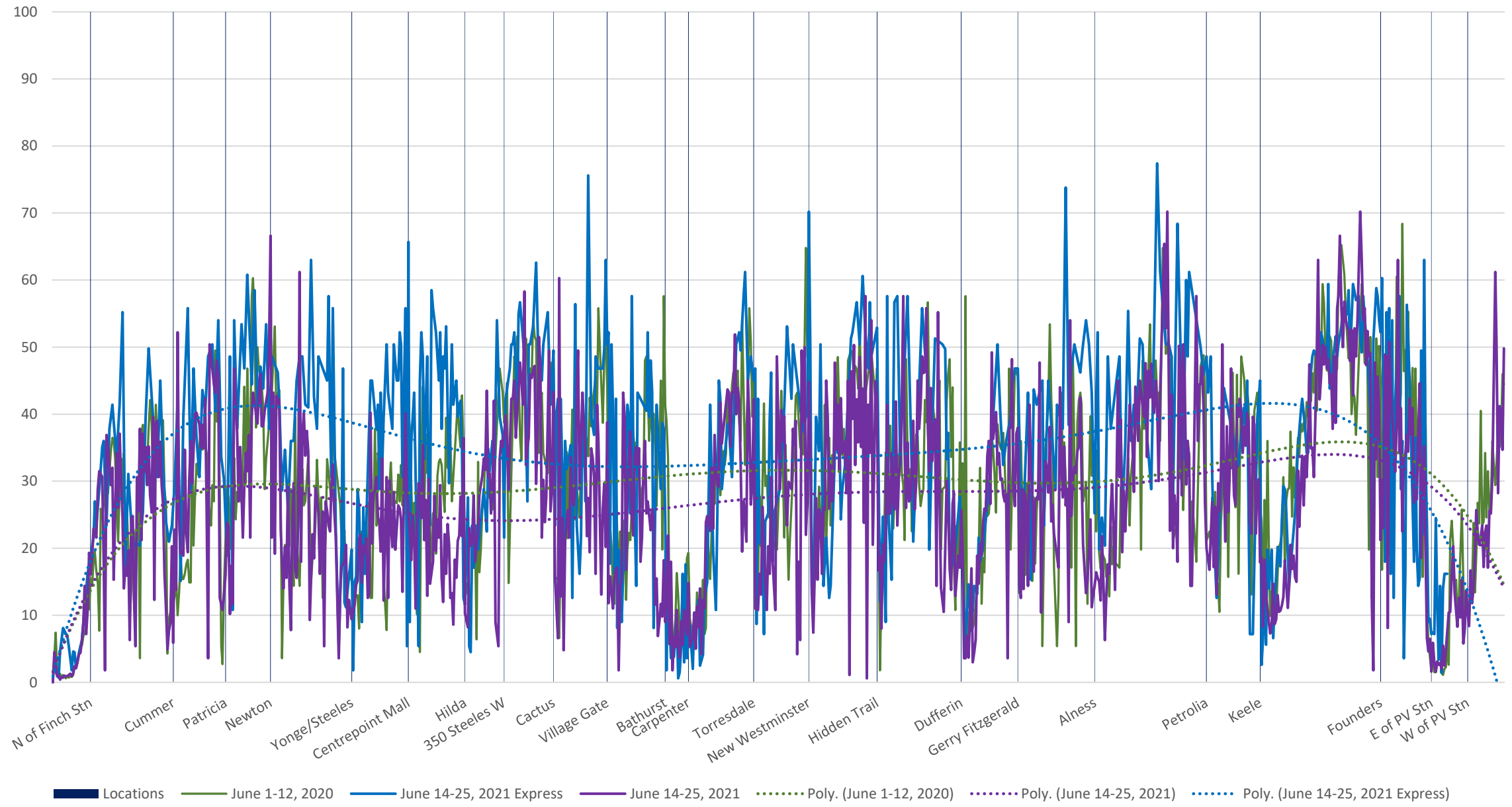
60 Steeles West Eastbound June 2020 vs June 2021 Average Speed 900 to 1000
