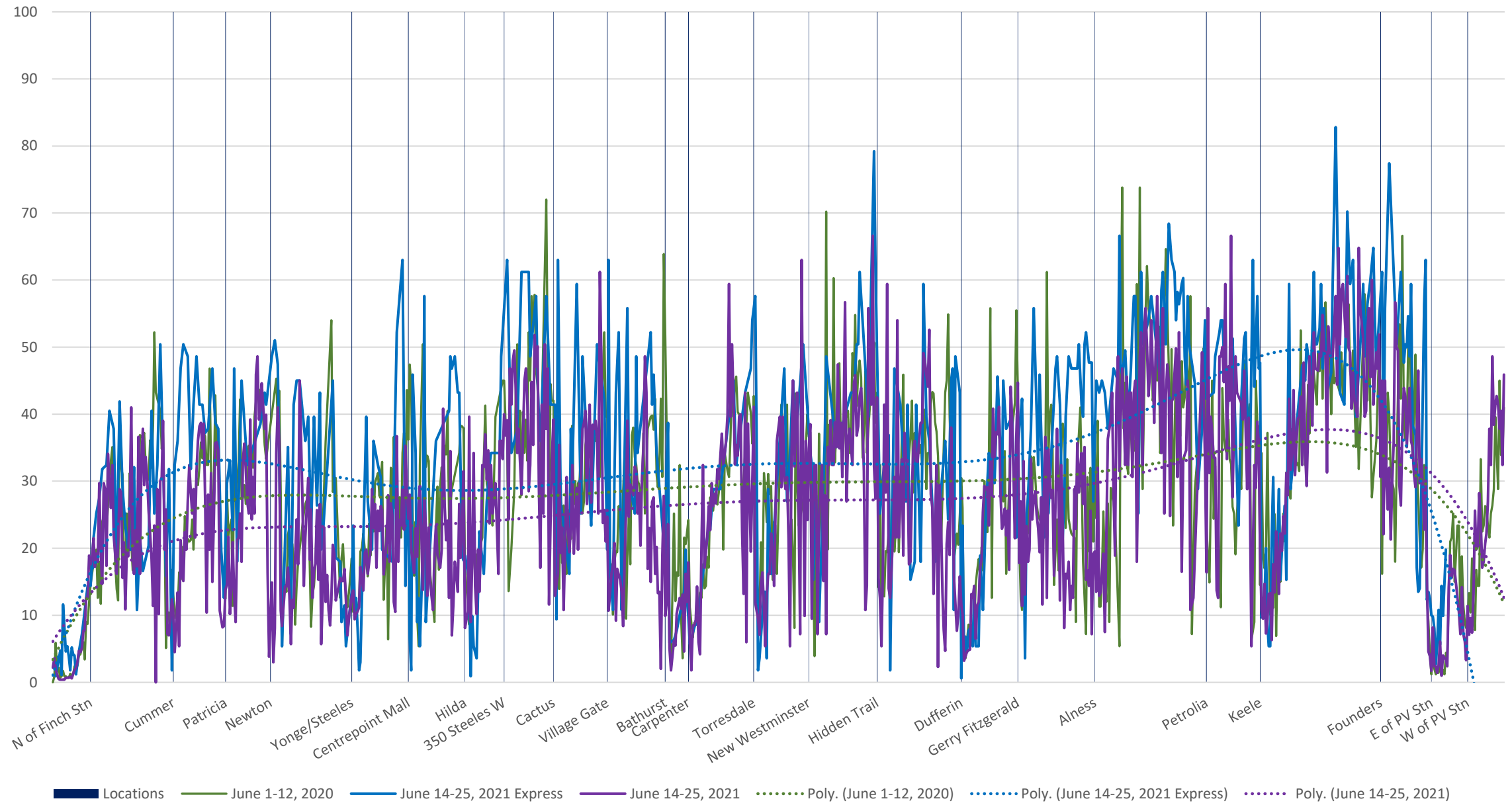
60 Steeles West Eastbound June 2020 vs June 2021 Average Speed 1900 to 2000
