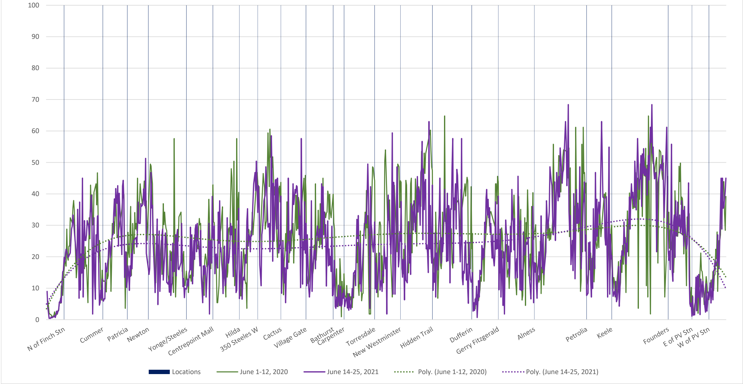
60 Steeles West Eastbound June 2020 vs June 2021 Average Speed 1400 to 1500
