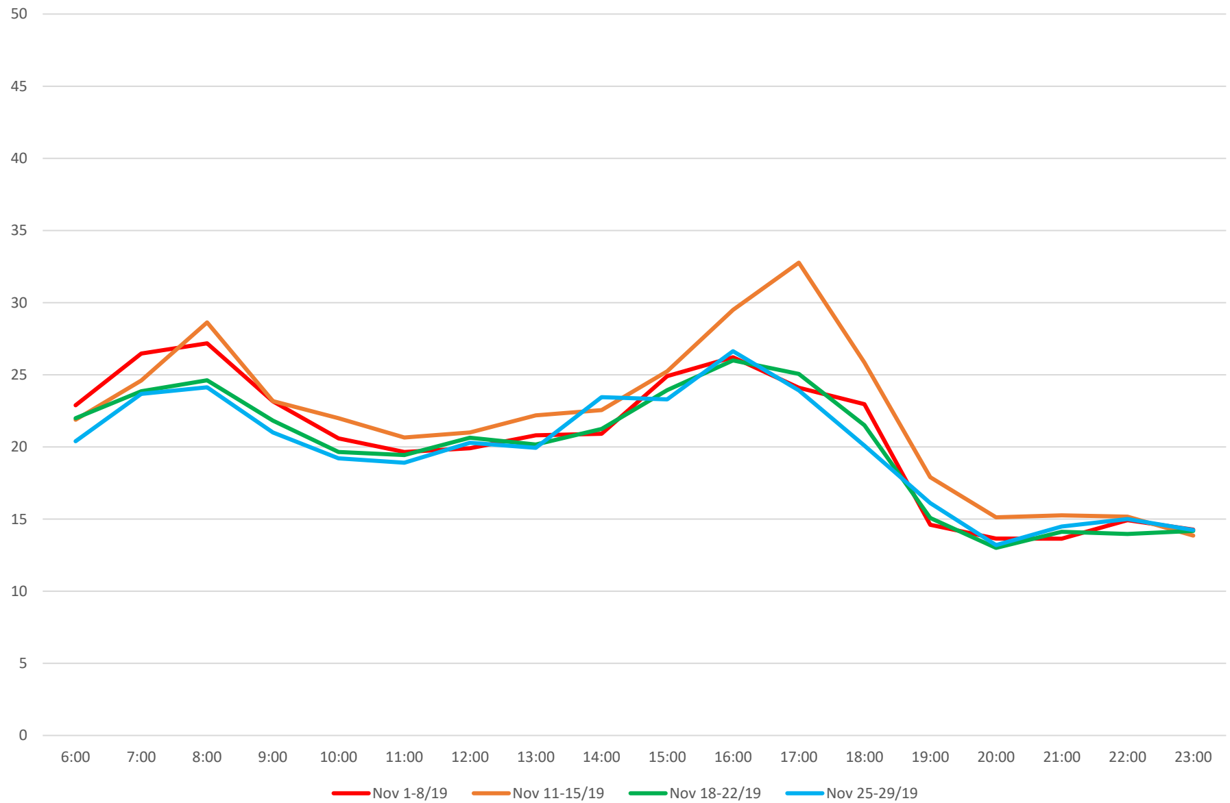
60 Steeles West Travel Times Kipling to W of Pioneer Village Stn Eastbound November 2019
