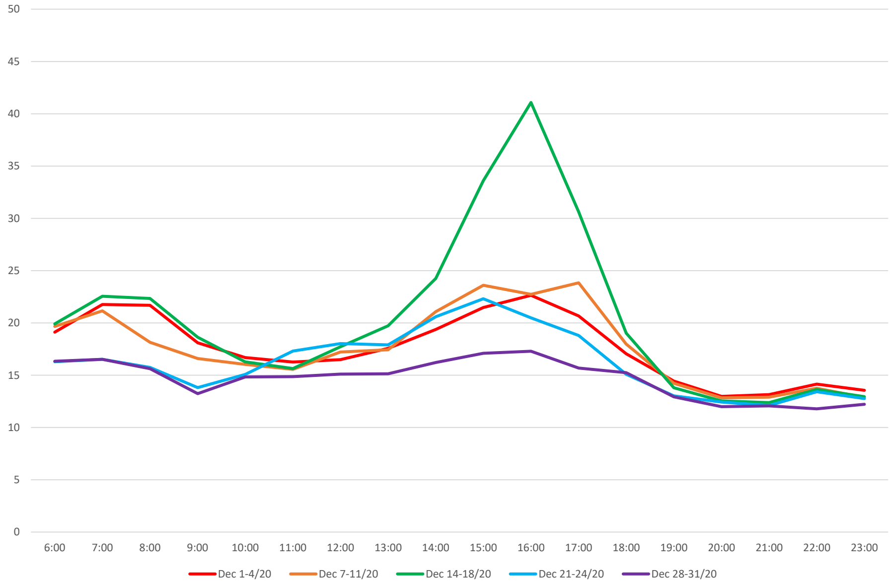
60 Steeles West Travel Times Kipling to W of Pioneer Village Stn Eastbound December 2020
