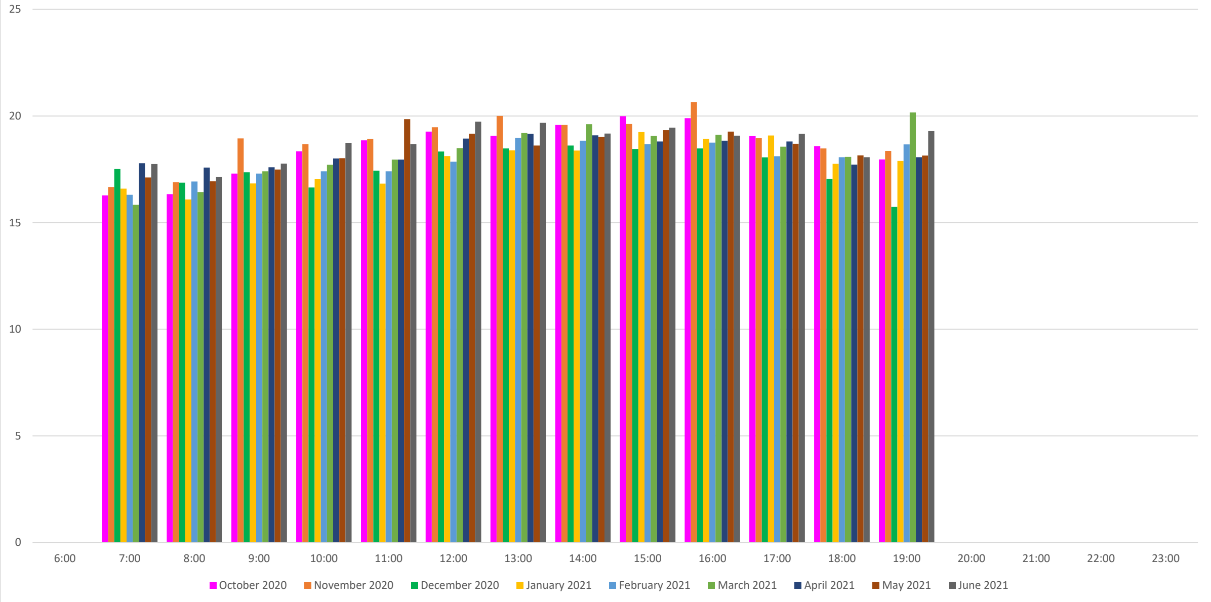
905 Eglinton East Express Travel Times Ellesmere to E of Kennedy Stn Westbound October 2020 to June 2021 Sundays
