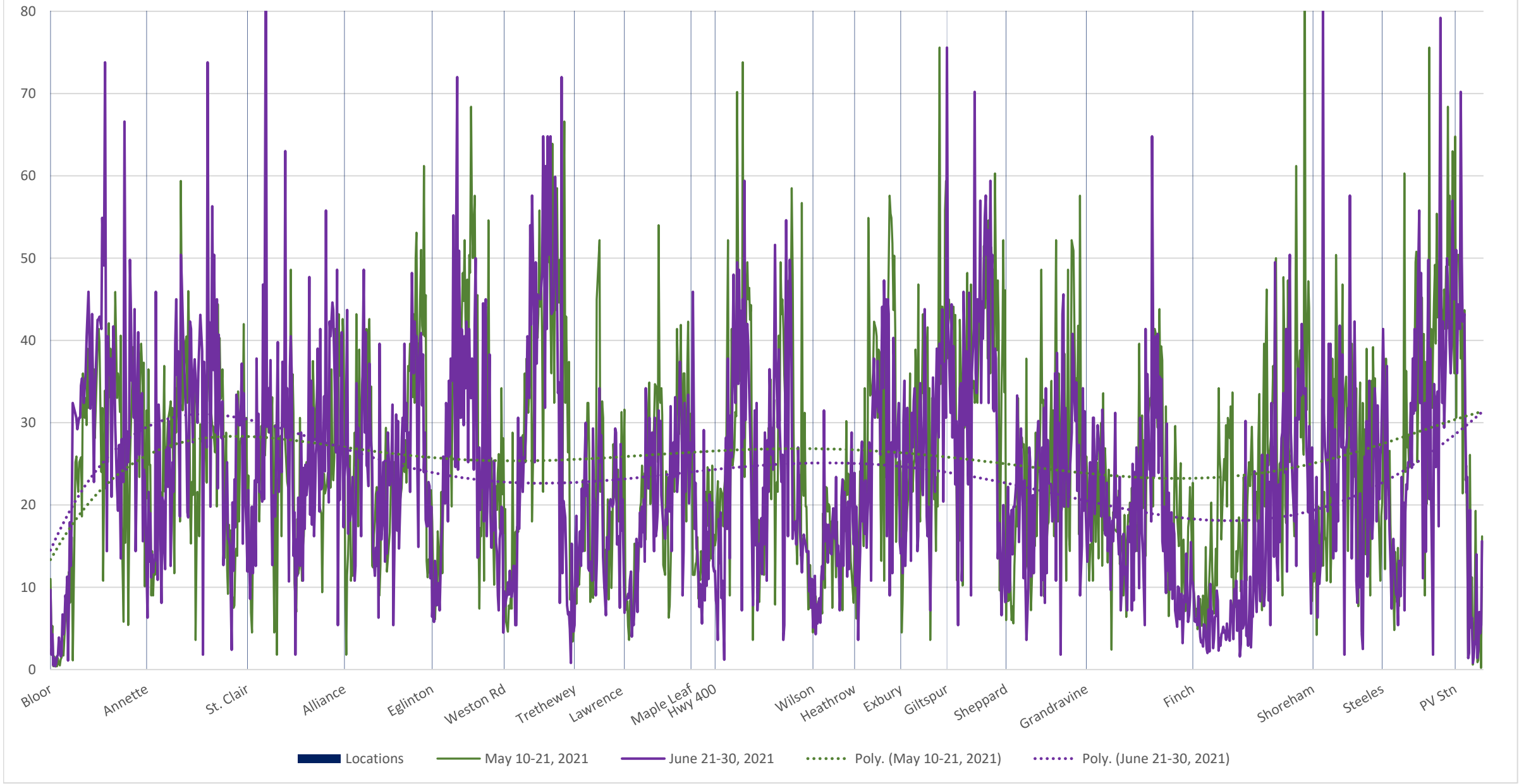
35 Jane Southbound May vs June 2021 Average Speed 1900 to 2000
