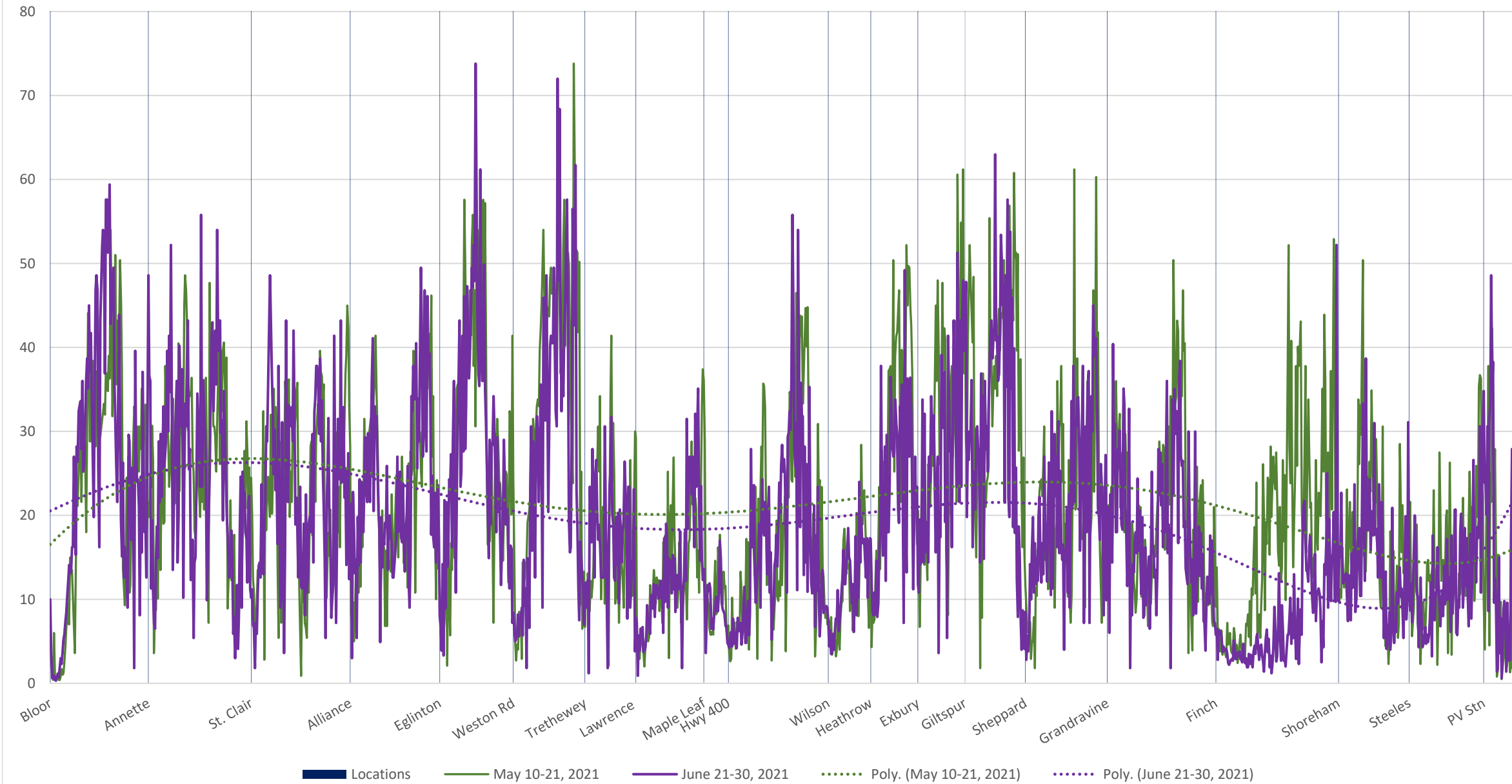
35 Jane Southbound May vs June 2021 Average Speed 1600 to 1700
