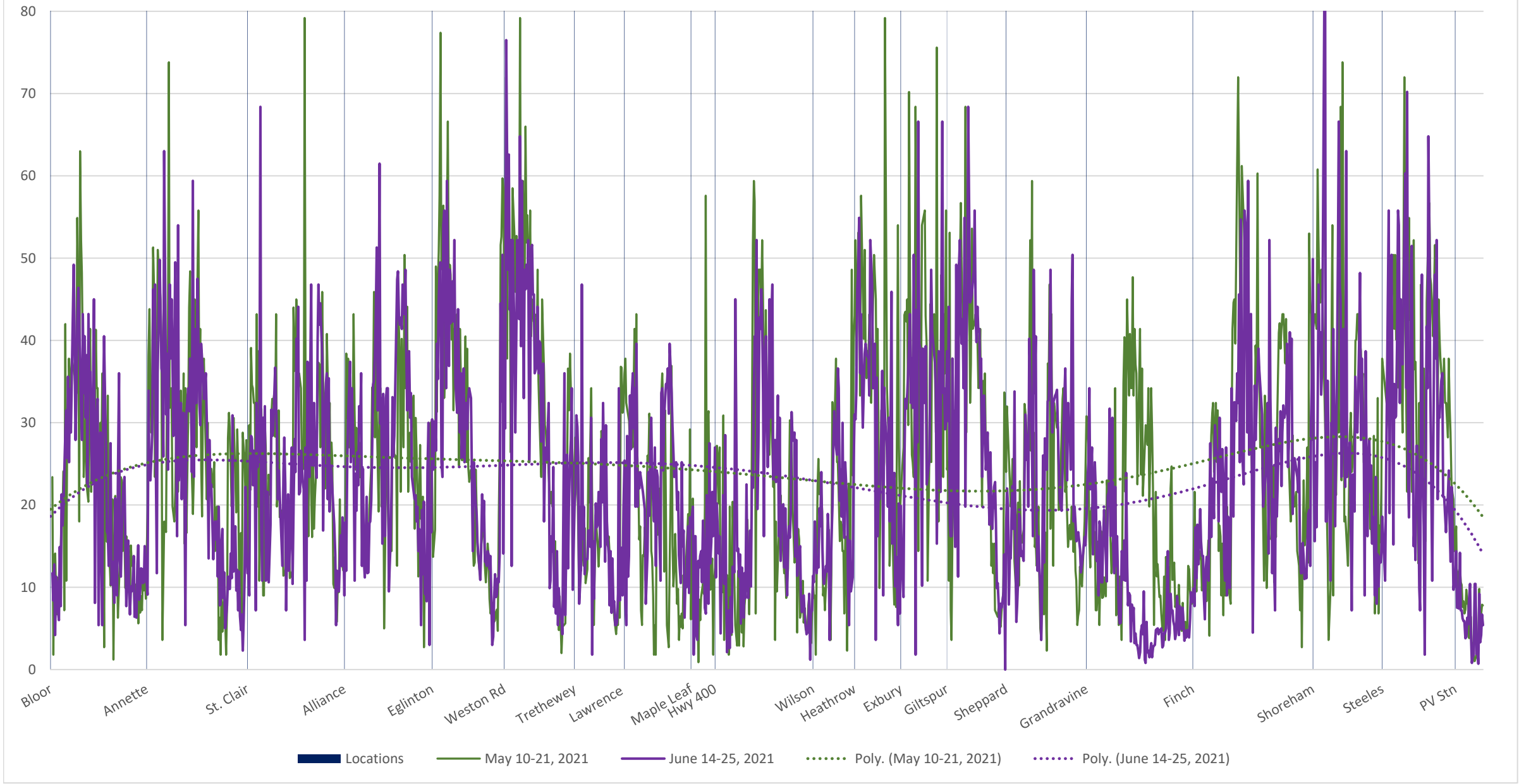
35 Jane Northbound May vs June 2021 Average Speed 1300 to 1400
