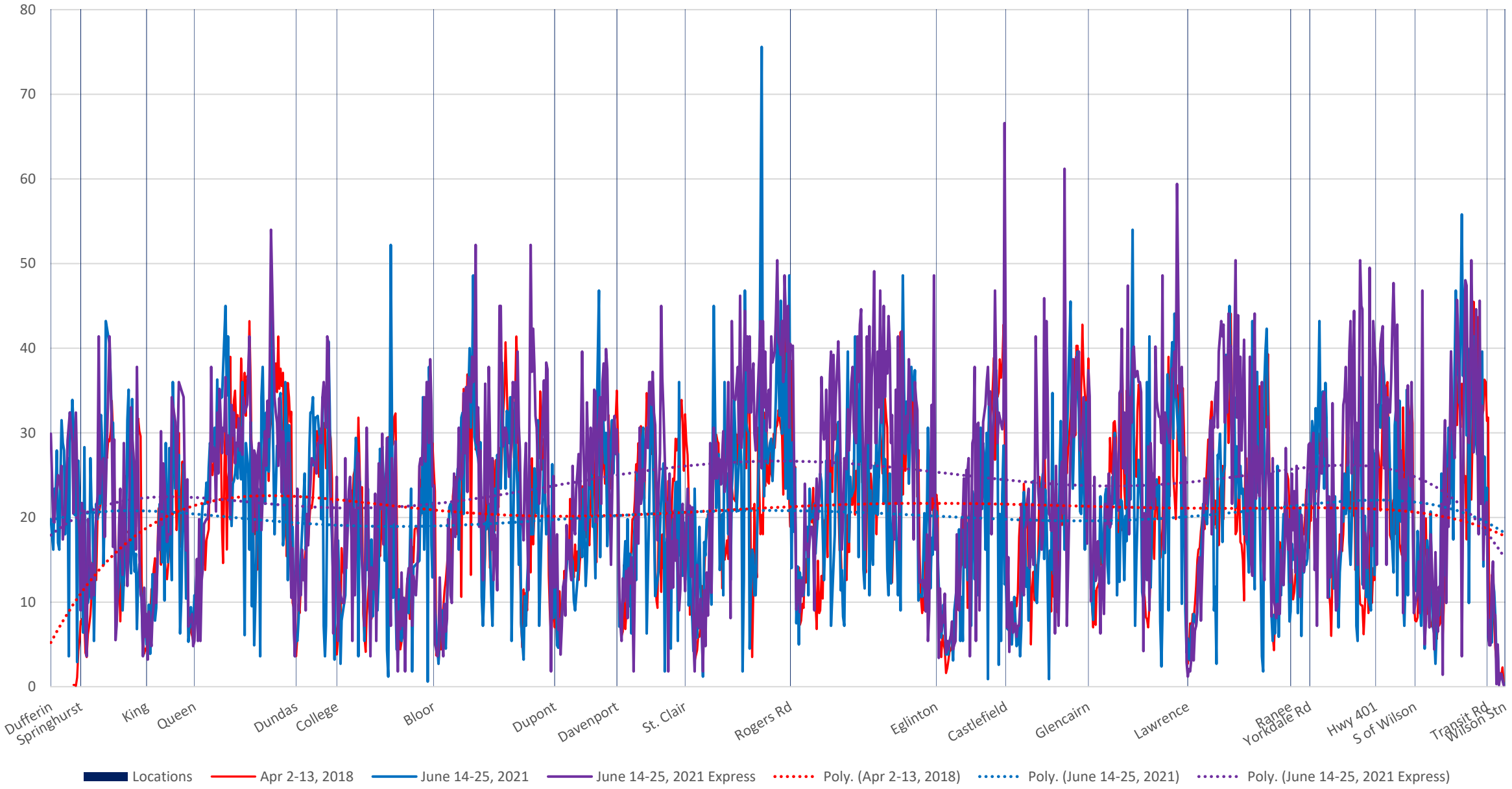
29 Dufferin Southbound June 2021 Local Vs Express Average Speed 1100 to 1200
