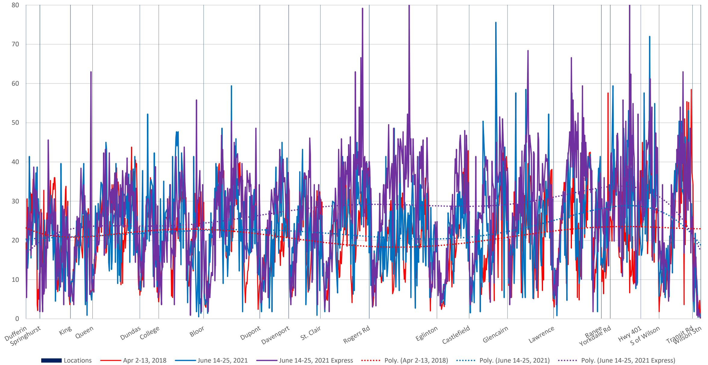
29 Dufferin Southbound June 2021 Local Vs Express Average Speed 700 to 800
