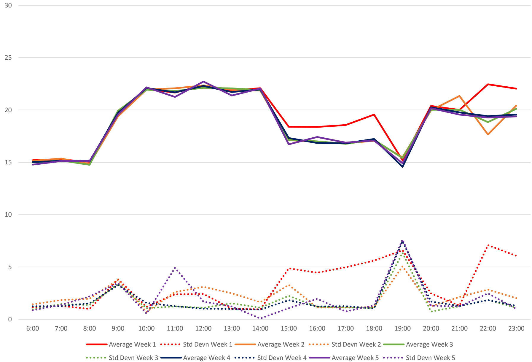
85 Sheppard East Headways at E of Yonge St Eastbound August 2020 Weekday Statistics
