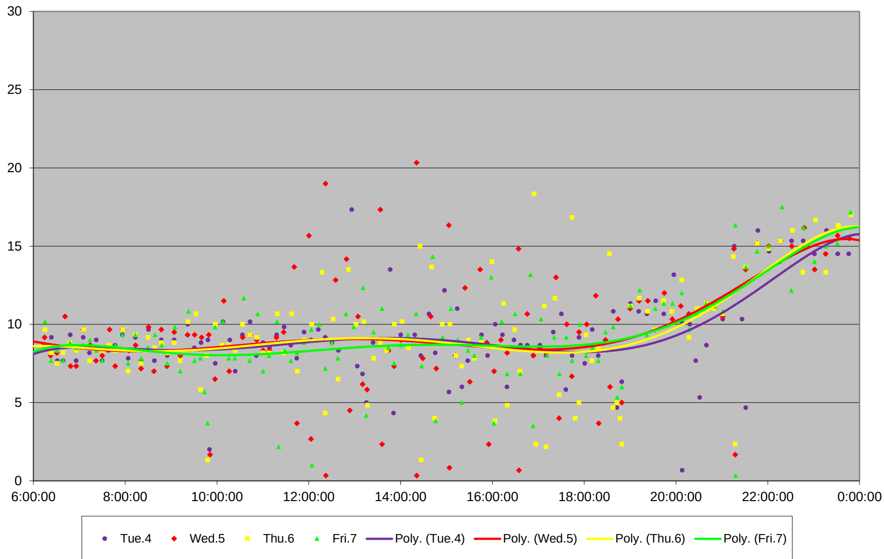
70 O'Connor Headways at Wolverleigh Northbound August 2020
