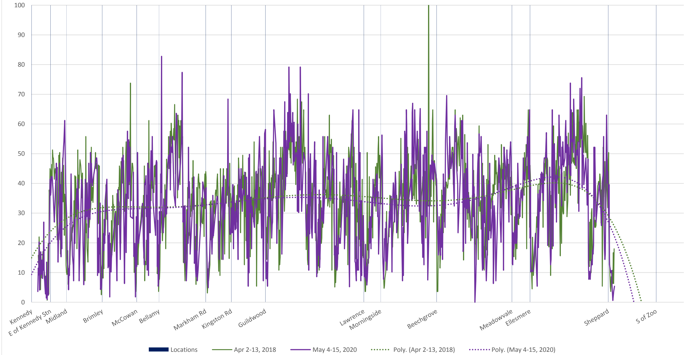
86 Scarborough Northbound April 2018-May 2020 Average Speed 2100 to 2200
