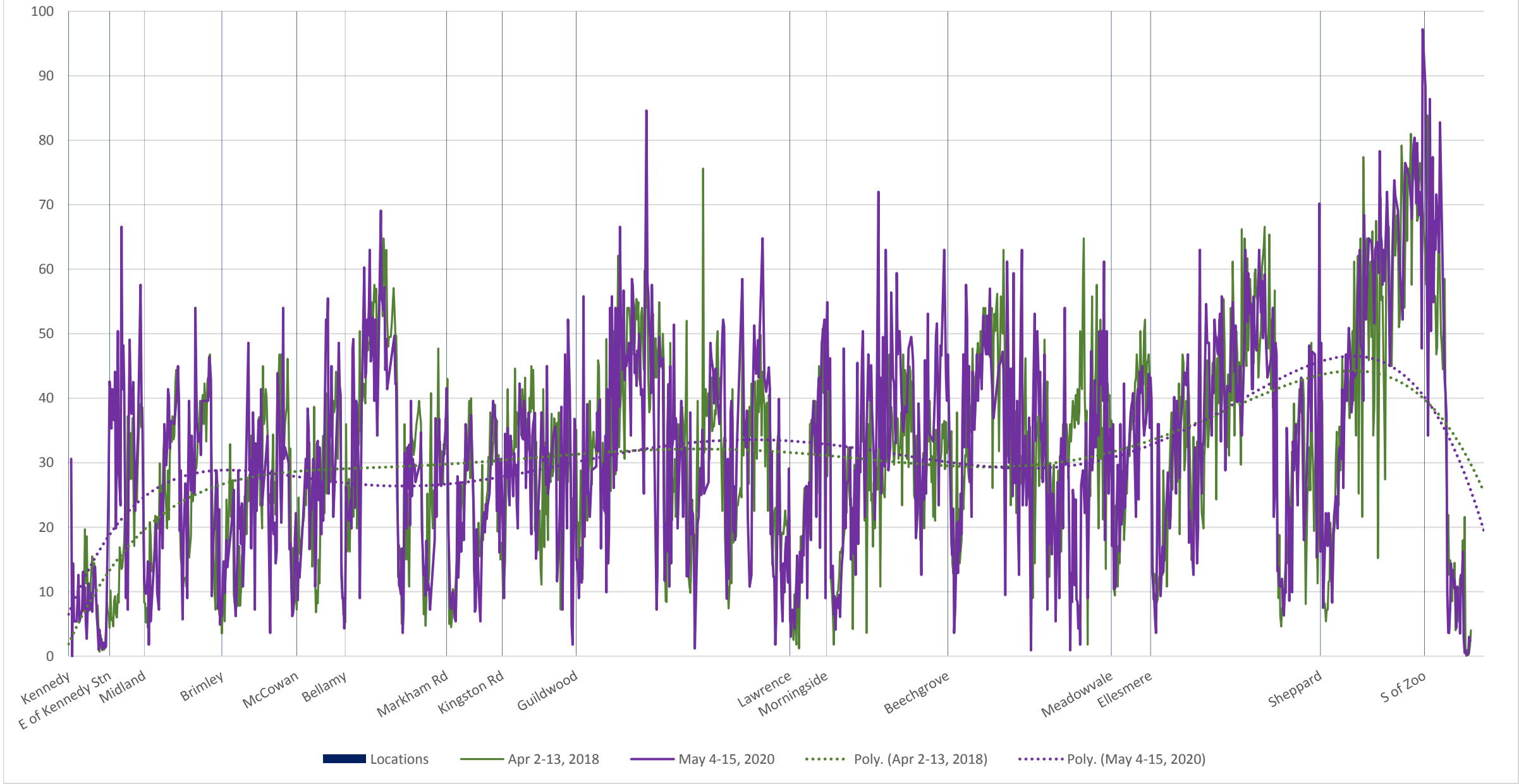
86 Scarborough Northbound April 2018-May 2020 Average Speed 1100 to 1200
