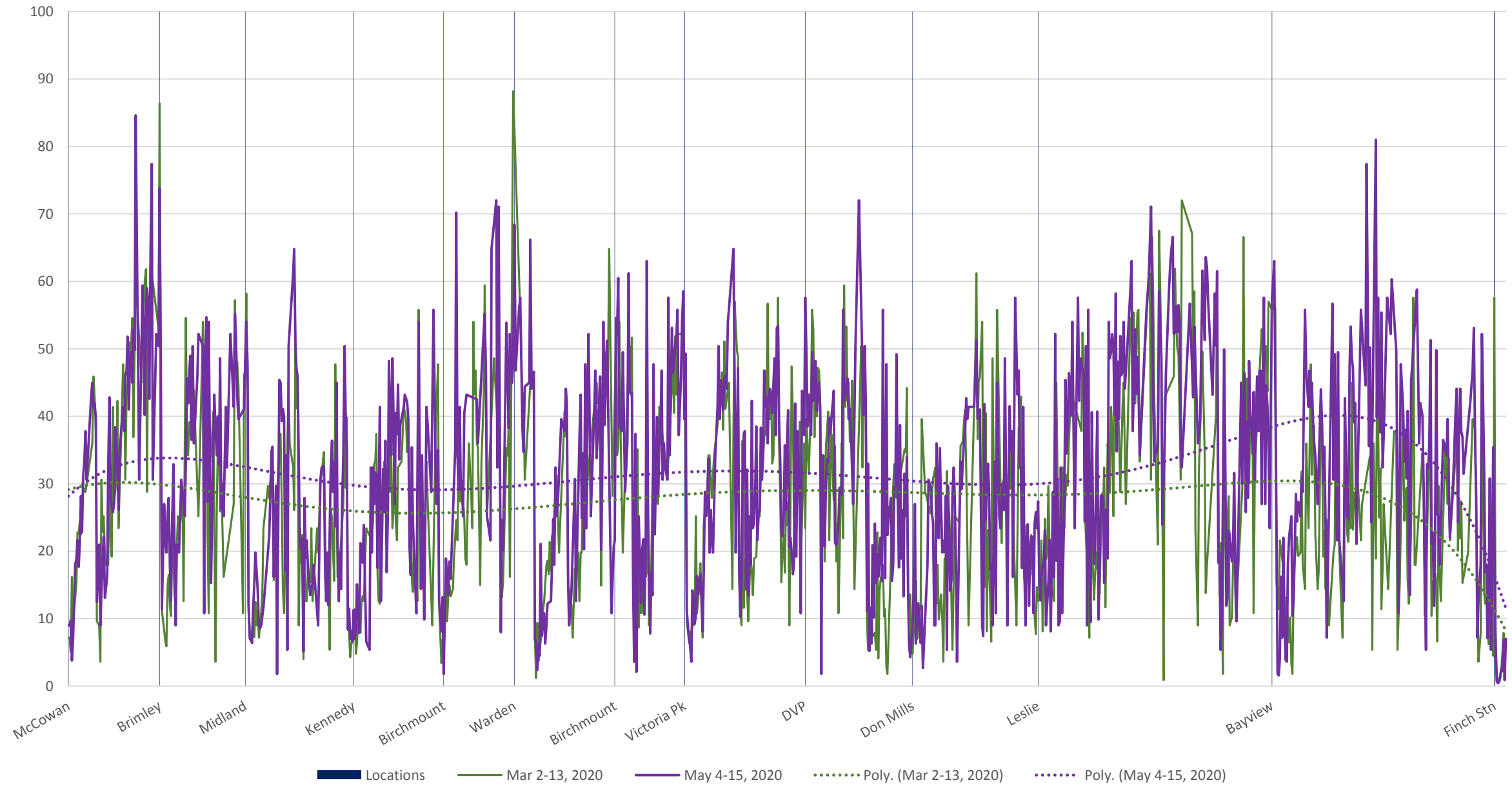
39 Finch East Eastbound March-May 2020 Average Speed 1400 to 1500
