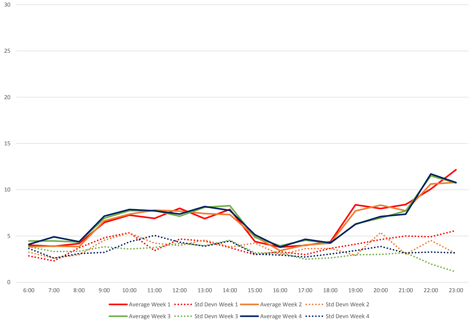
116 Morningside Headways at E of Kennedy Stn Eastbound February 2020 Weekday Statistics
