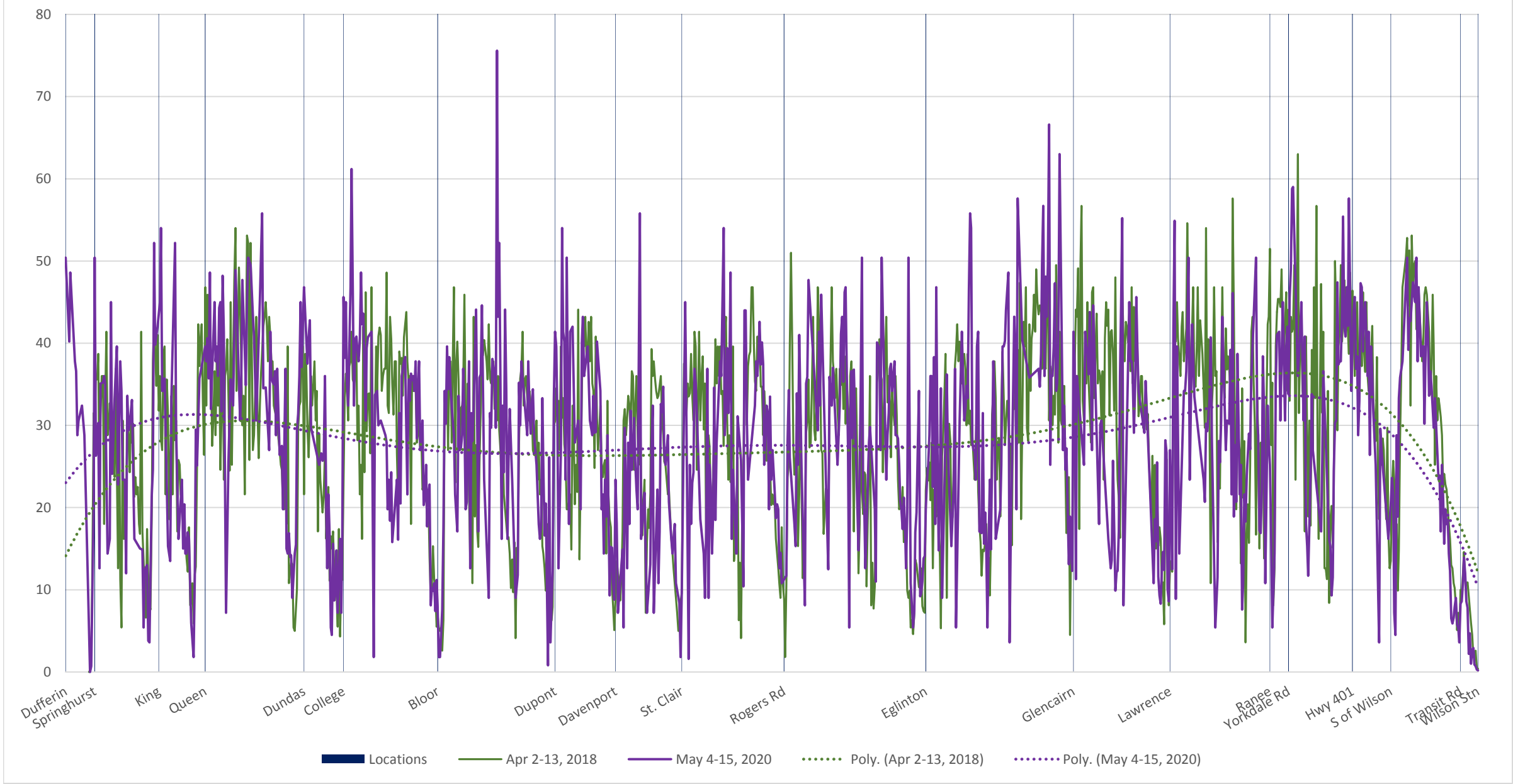
29 Dufferin Northbound April 2018-May 2020 Average Speed 2400 to 2500
