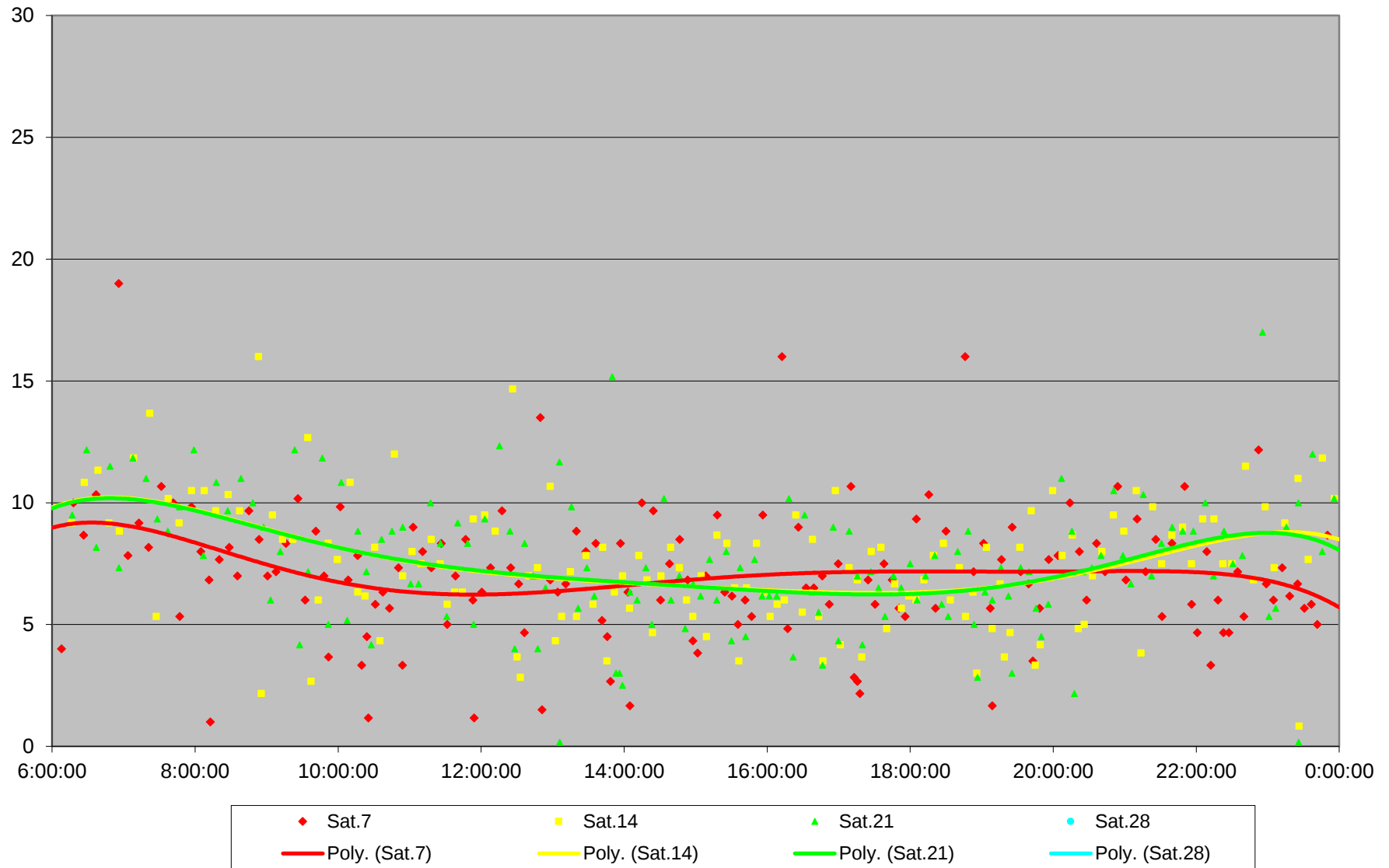
504 King Headways at Danforth Southbound September 2019
