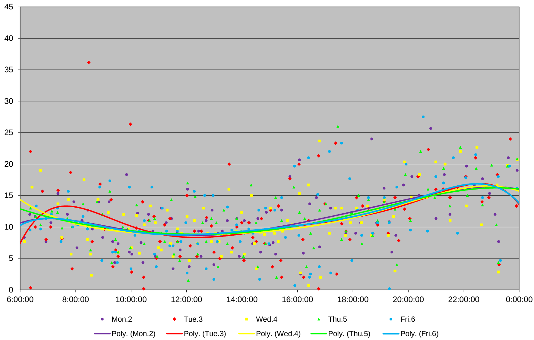
41A Keele Local Headways at N of Finch Southbound April 2018
