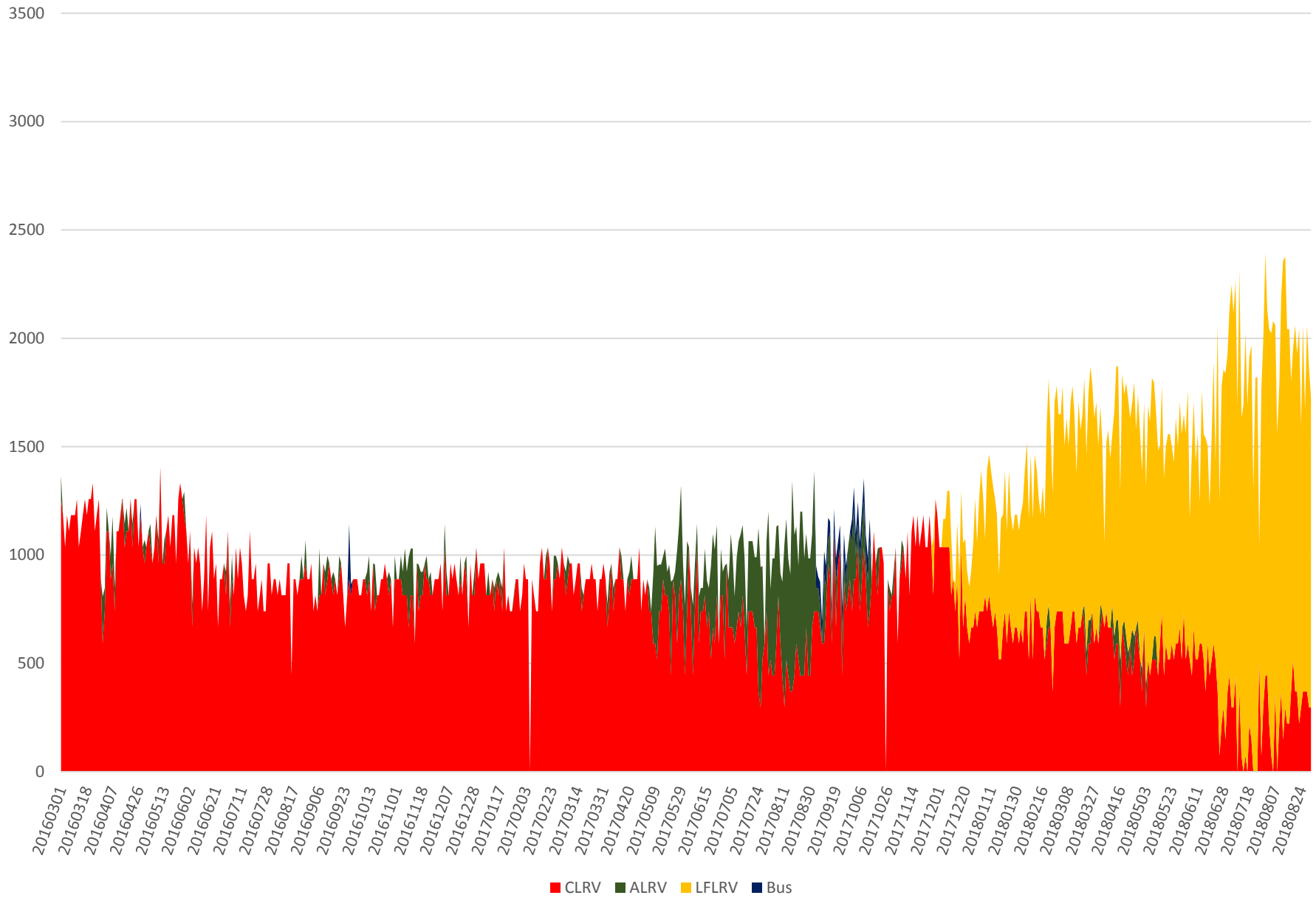
504 King Capacity at Jameson/WB March 2016 to August 2018 1500 to 1600
