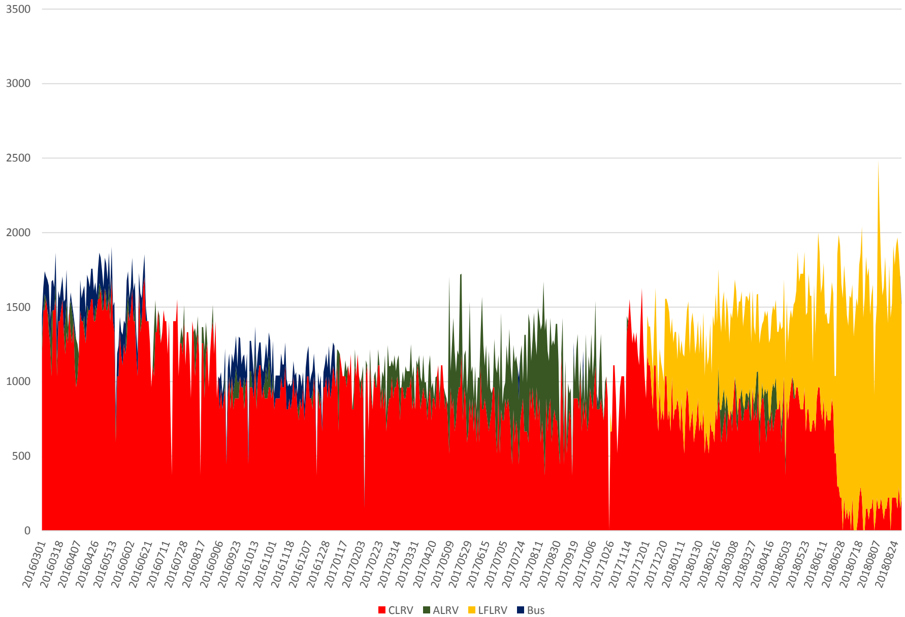
504 King Capacity at Jameson/WB March 2016 to August 2018 1600 to 1700
