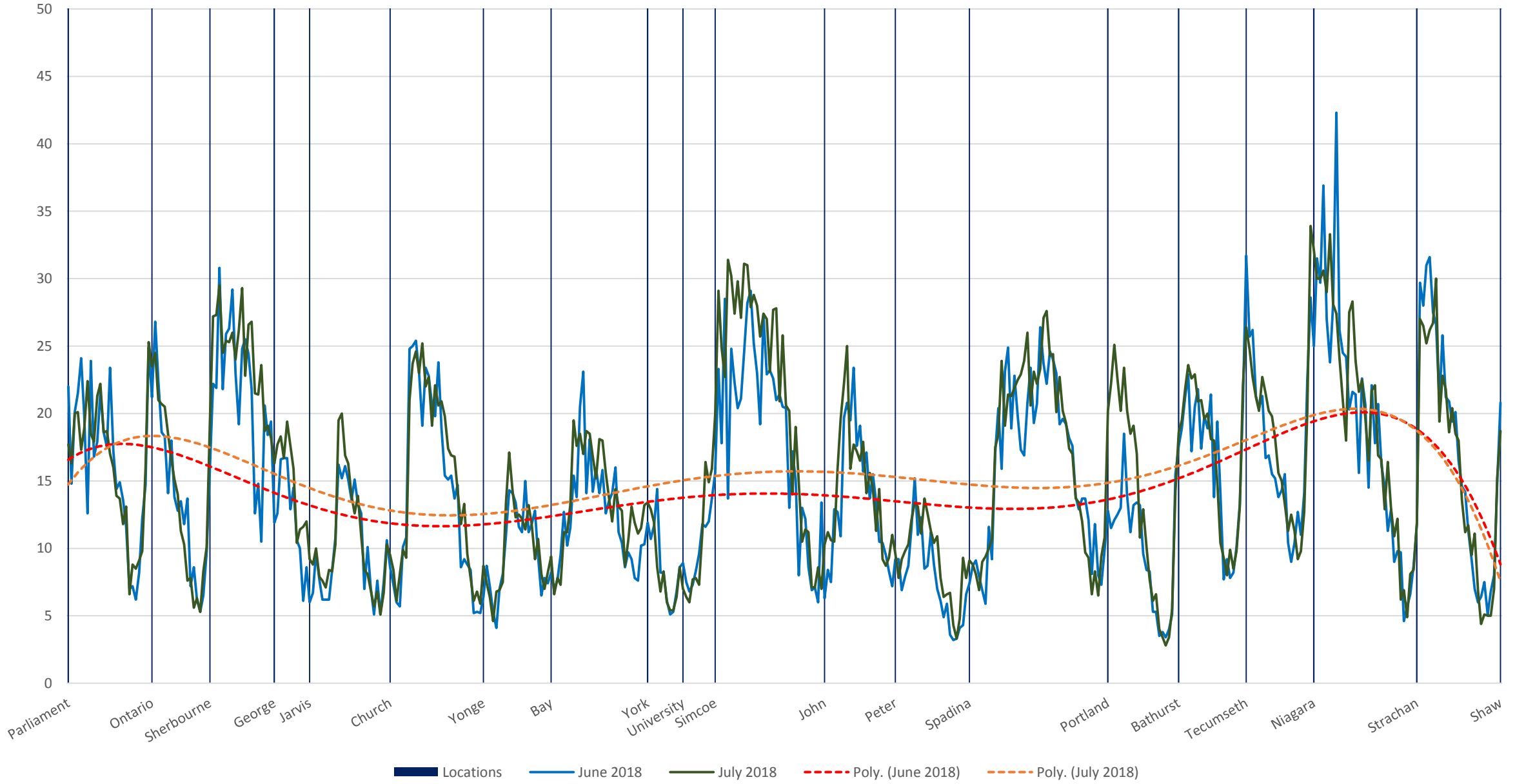
504 King Westbound June 11-22 (Blue) vs July 9-20 (Green) 2018 Average Speed 1400 to 1500
