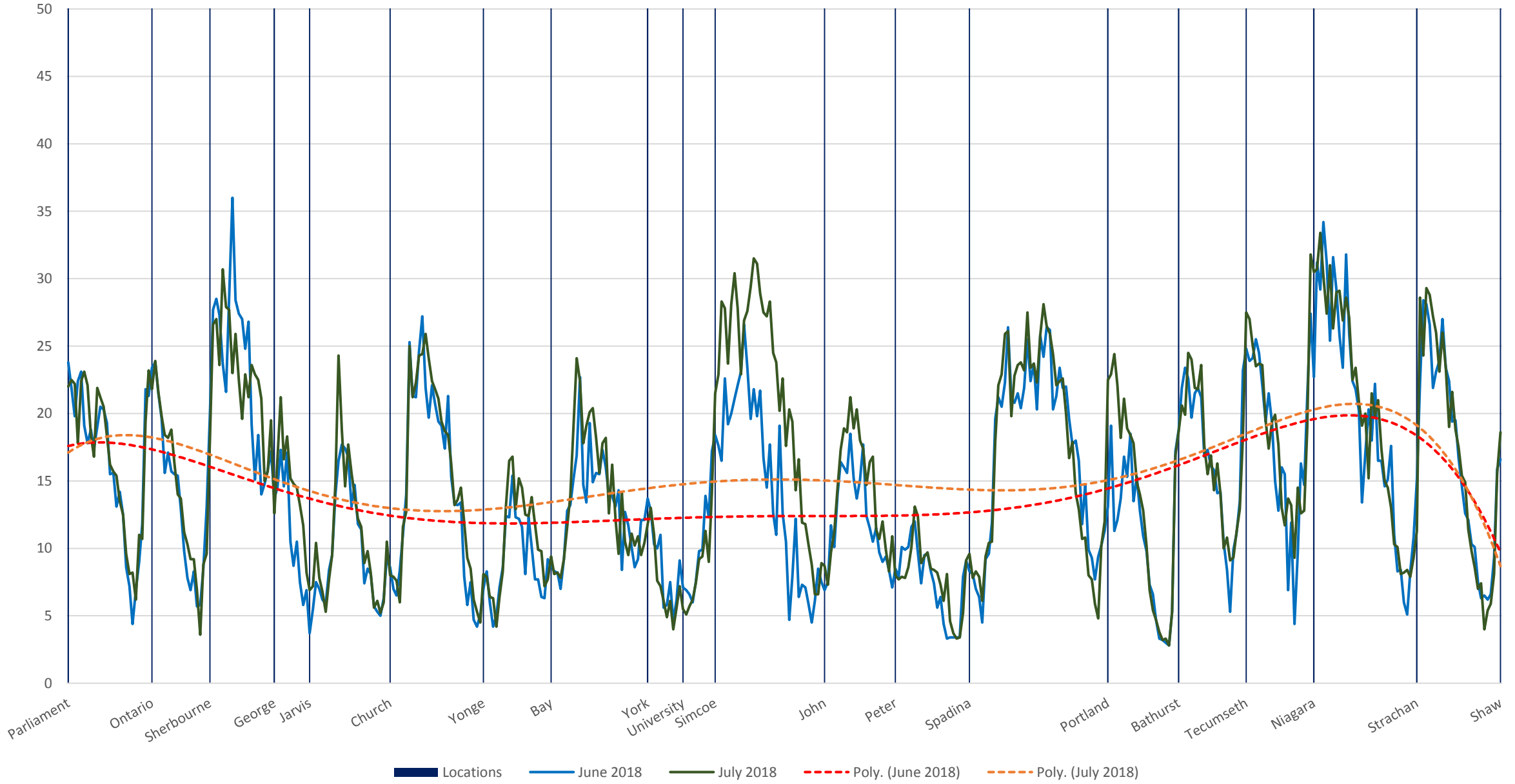
504 King Westbound June 11-22 (Blue) vs July 9-20 (Green) 2018 Average Speed 1500 to 1600
