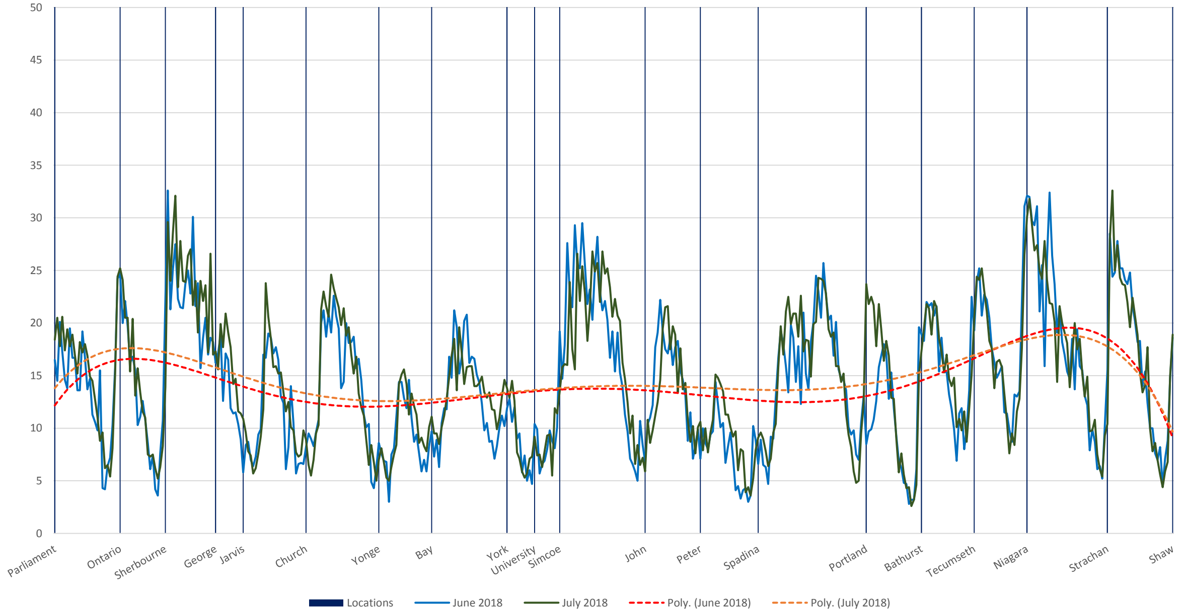
504 King Westbound June 11-22 (Blue) vs July 9-20 (Green) 2018 Average Speed 1200 to 1300
