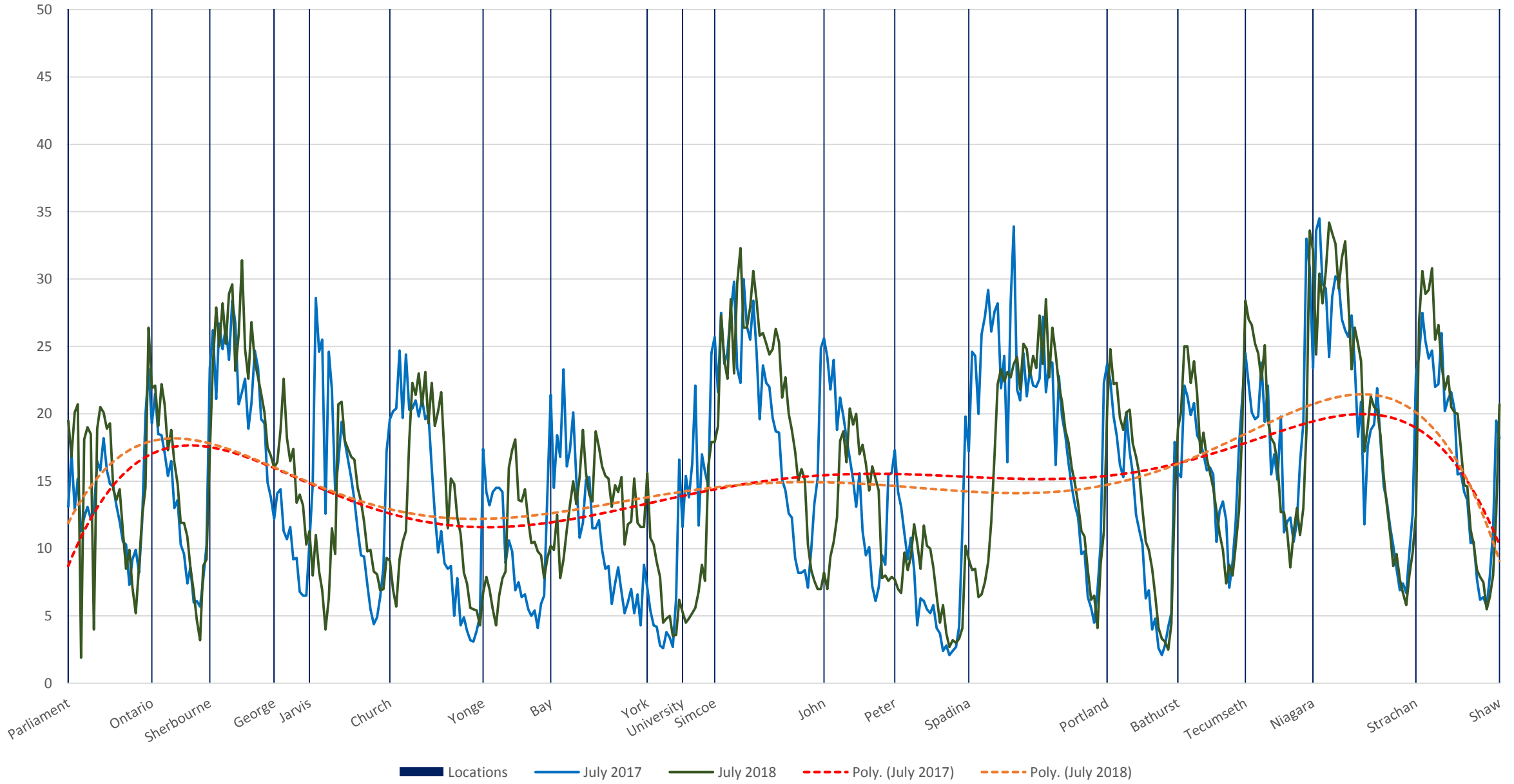
504 King Westbound July 10-21, 2017 (Blue) vs July 9-20, 2018 (Green) Average Speed 900 to 1000
