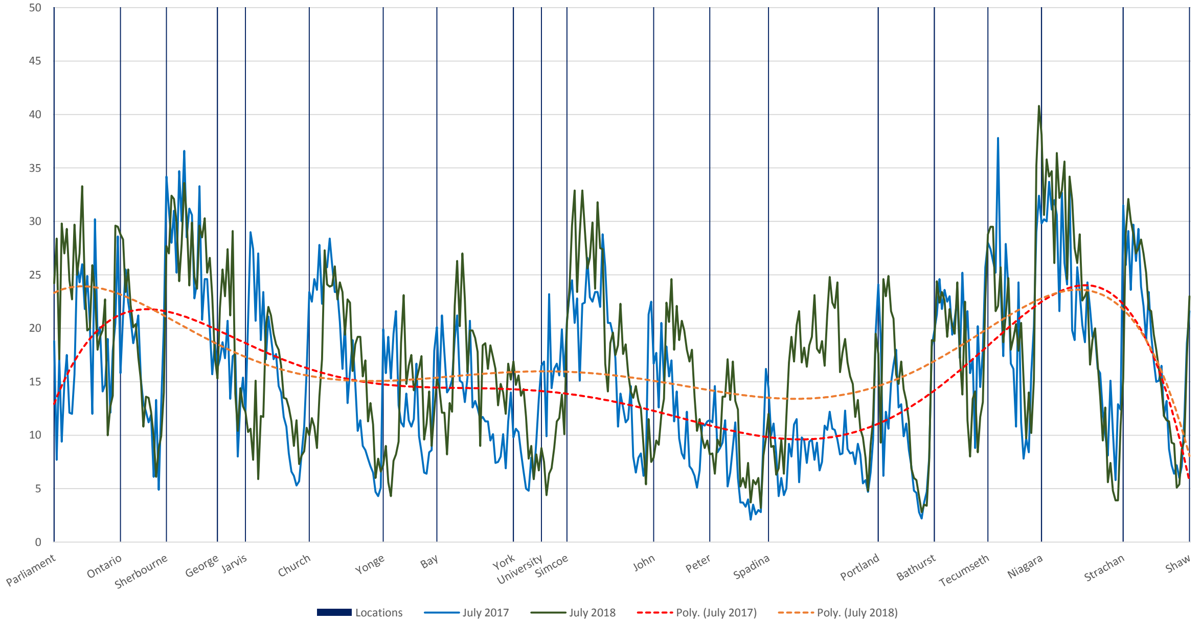
504 King Westbound July 10-21, 2017 (Blue) vs July 9-20, 2018 (Green) Average Speed 2300 to 2400
