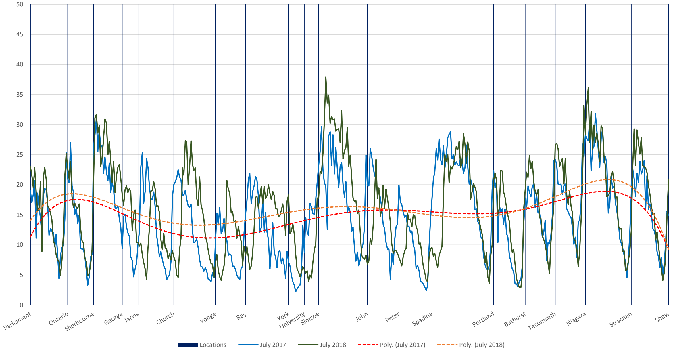
504 King Westbound July 10-21, 2017 (Blue) vs July 9-20, 2018 (Green) Average Speed 800 to 900
