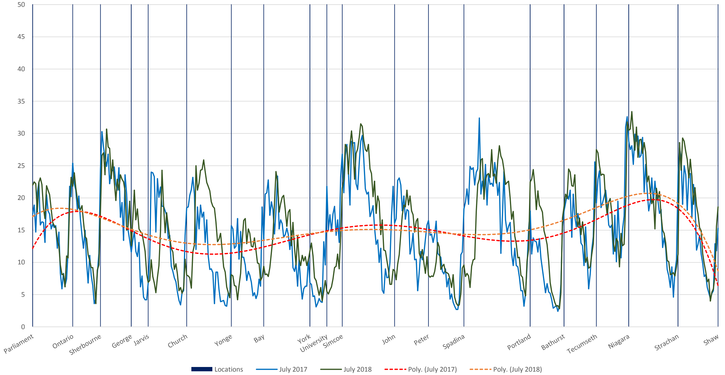
504 King Westbound July 10-21, 2017 (Blue) vs July 9-20, 2018 (Green) Average Speed 1500 to 1600
