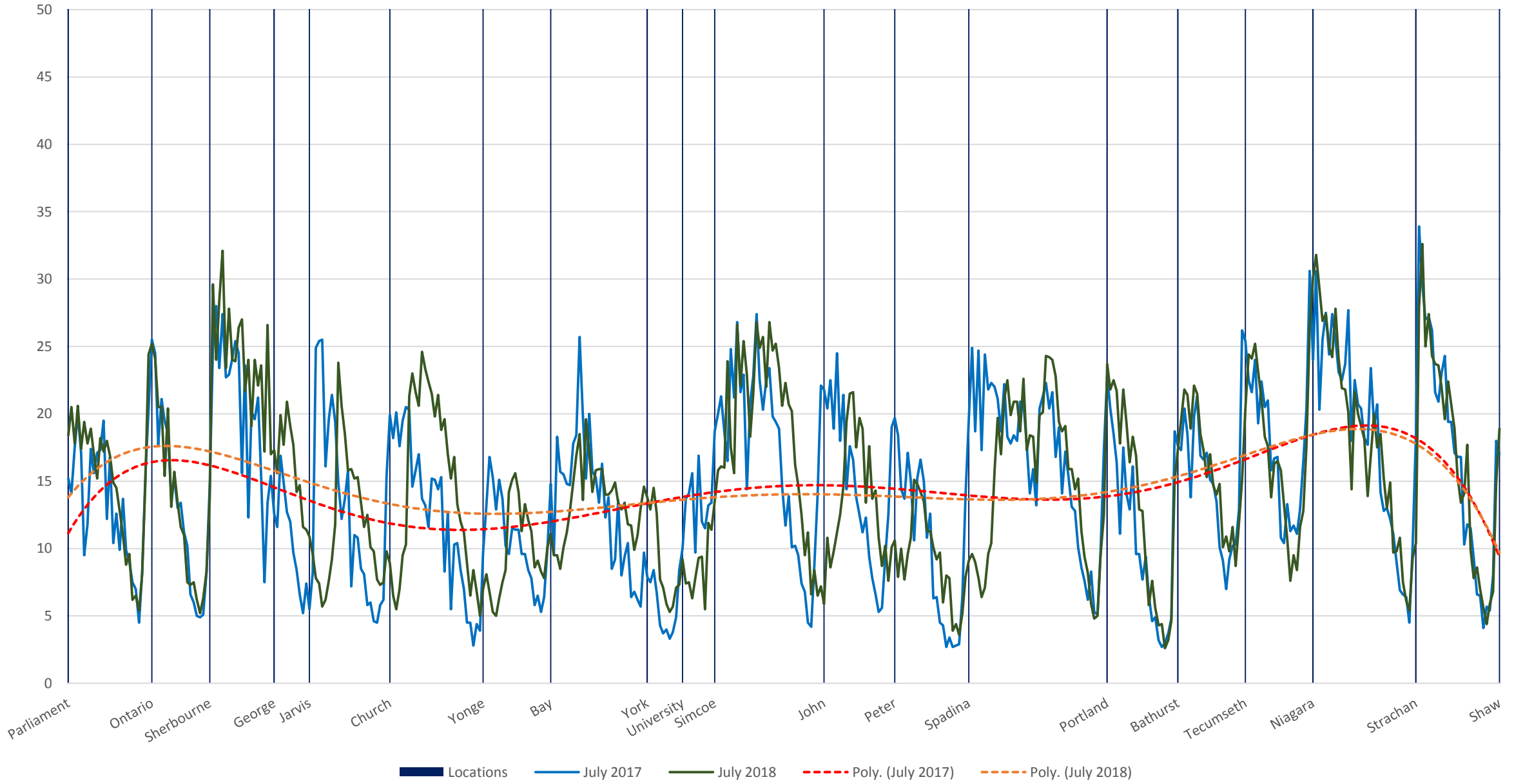
504 King Westbound July 10-21, 2017 (Blue) vs July 9-20, 2018 (Green) Average Speed 1200 to 1300
