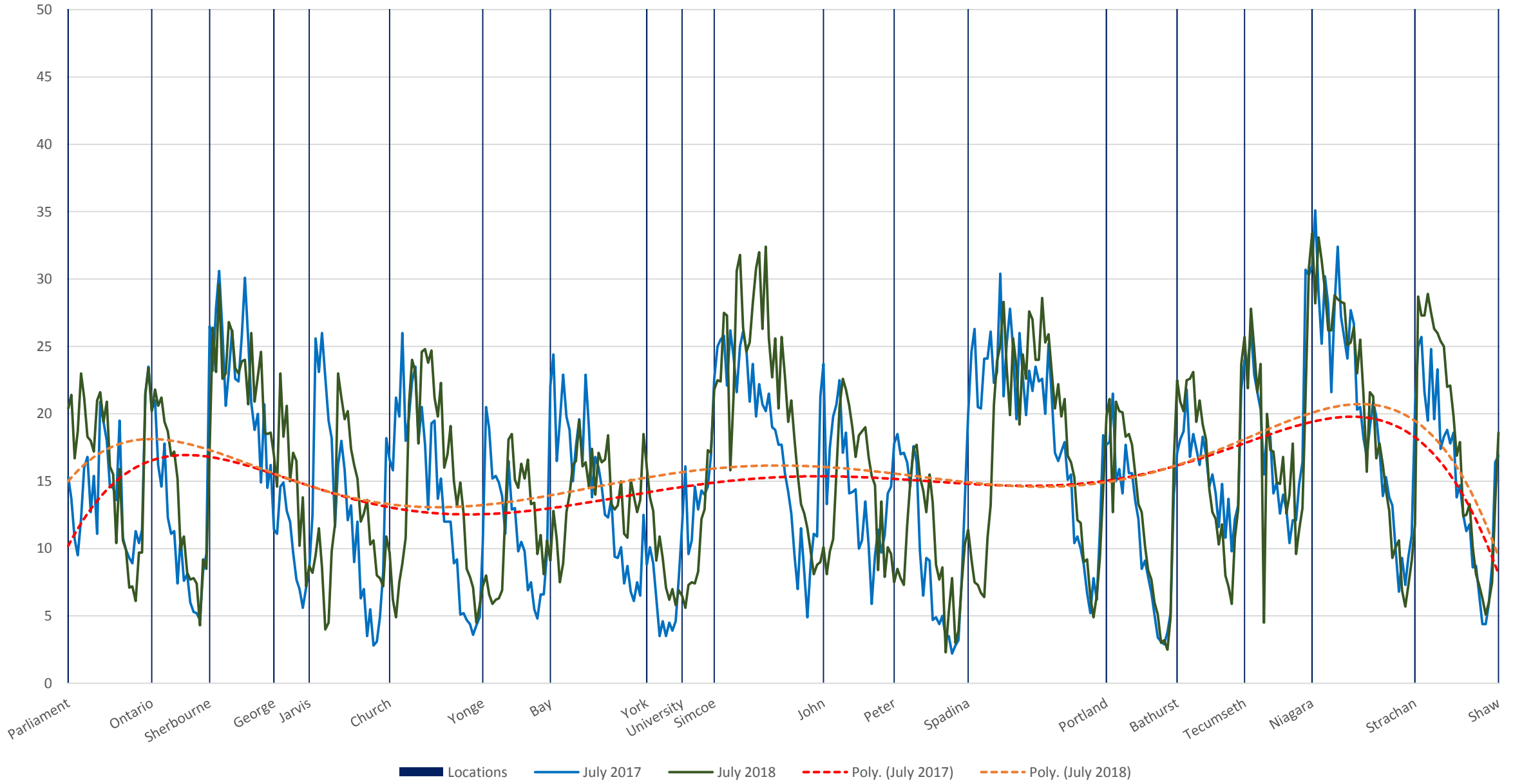
504 King Westbound July 10-21, 2017 (Blue) vs July 9-20, 2018 (Green) Average Speed 1000 to 1100
