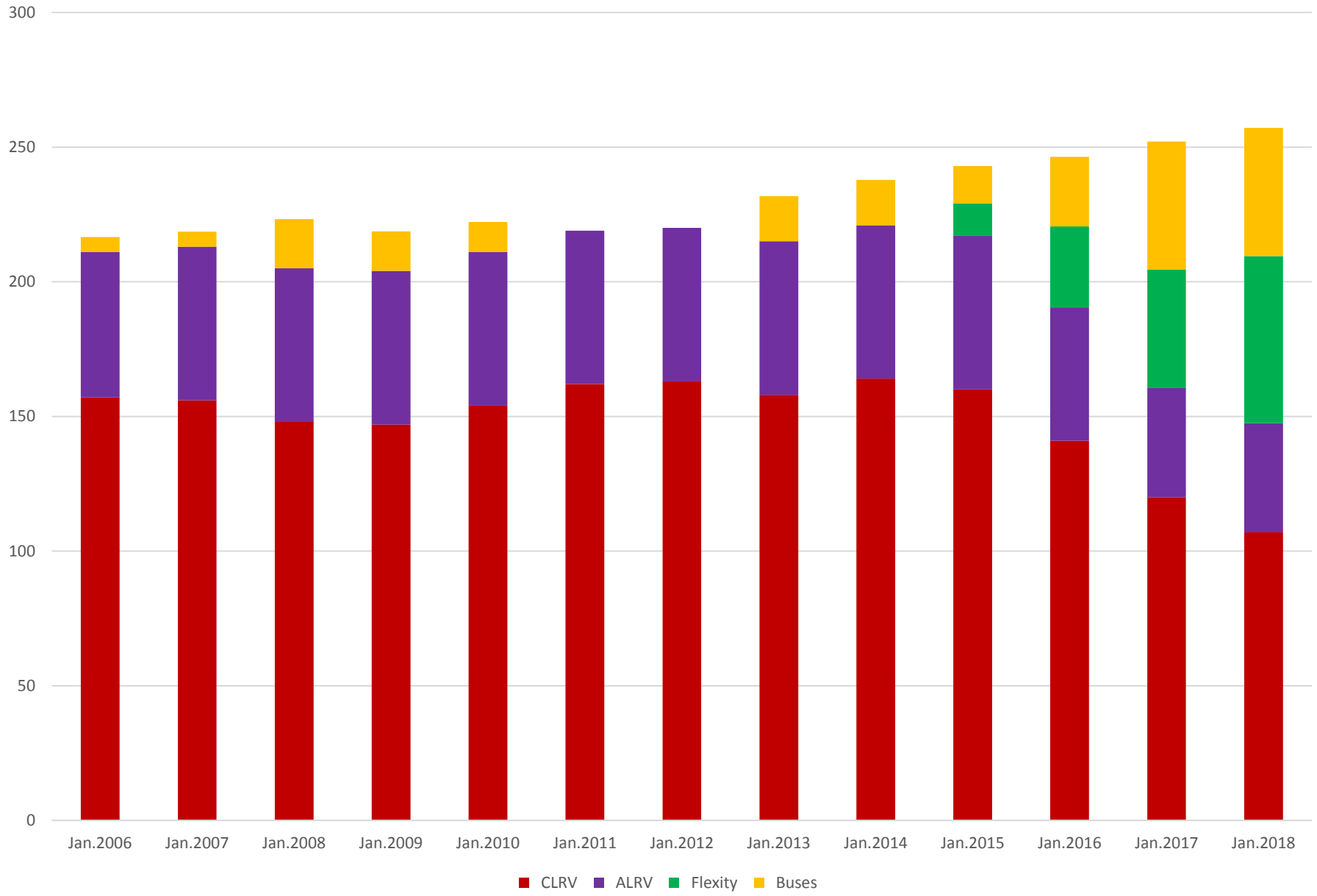
TTC AM Peak Scheduled Streetcar Service Capacity By Vehicle Type 2006 to 2018
