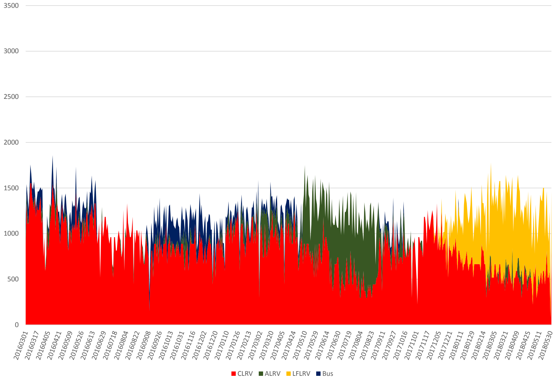
504 King Capacity at Jameson/WB March 2016 to May 2018 1700 to 1800
