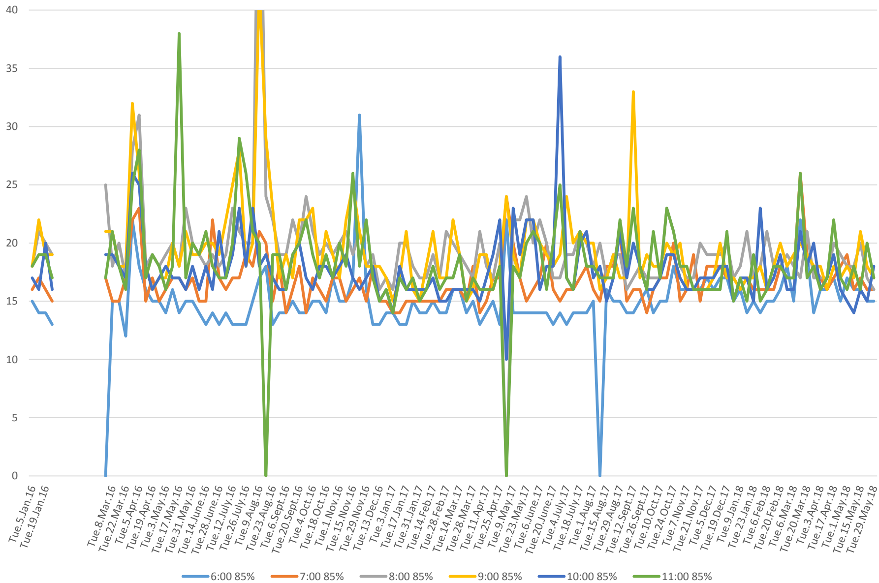
504 King Link Times From Jarvis To Bathurst Westbound From Jan 2016 To May 2018 85th Percentile Tuesday Mornings
