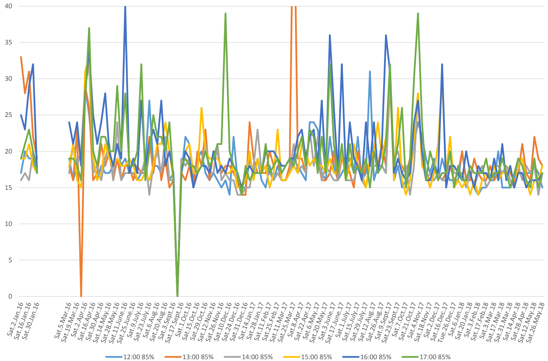
504 King Link Times From Jarvis To Bathurst Westbound From Jan 2016 To May 2018 85th Percentile Saturday Afternoons
