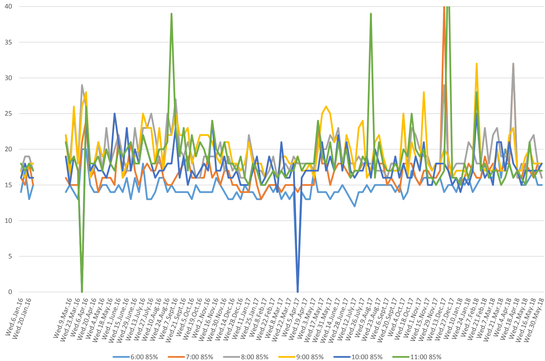
504 King Link Times From Jarvis To Bathurst Westbound From Jan 2016 To May 2018 85th Percentile Wednesday Mornings
