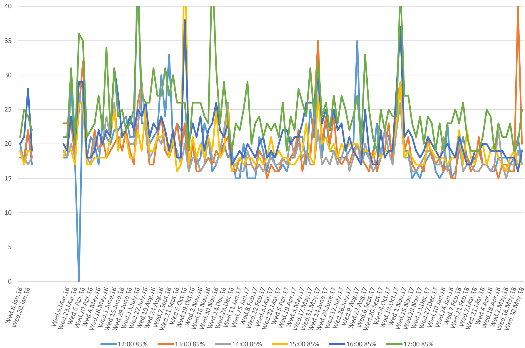
504 King Link Times From Jarvis To Bathurst Westbound From Jan 2016 To May 2018 85th Percentile Wednesday Afternoons
