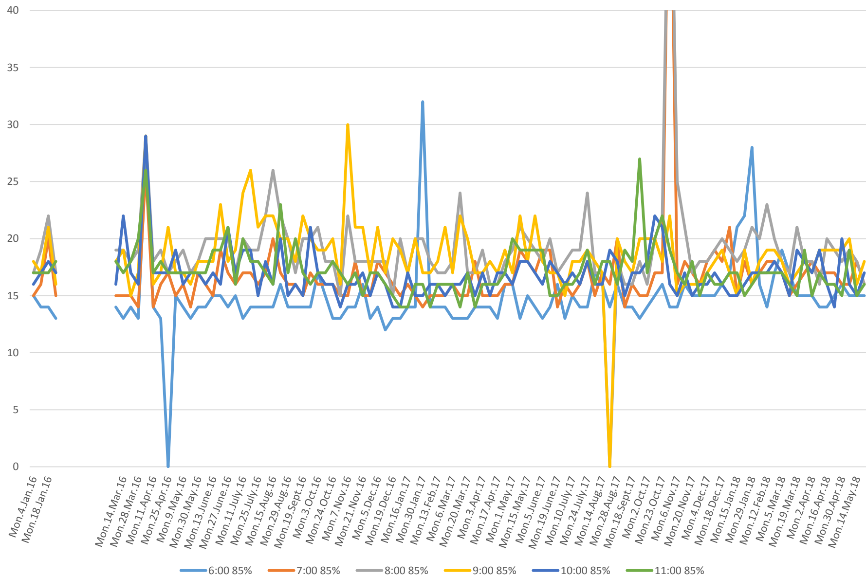
504 King Link Times From Jarvis To Bathurst Westbound From Jan 2016 To May 2018 85th Percentile Monday Mornings
