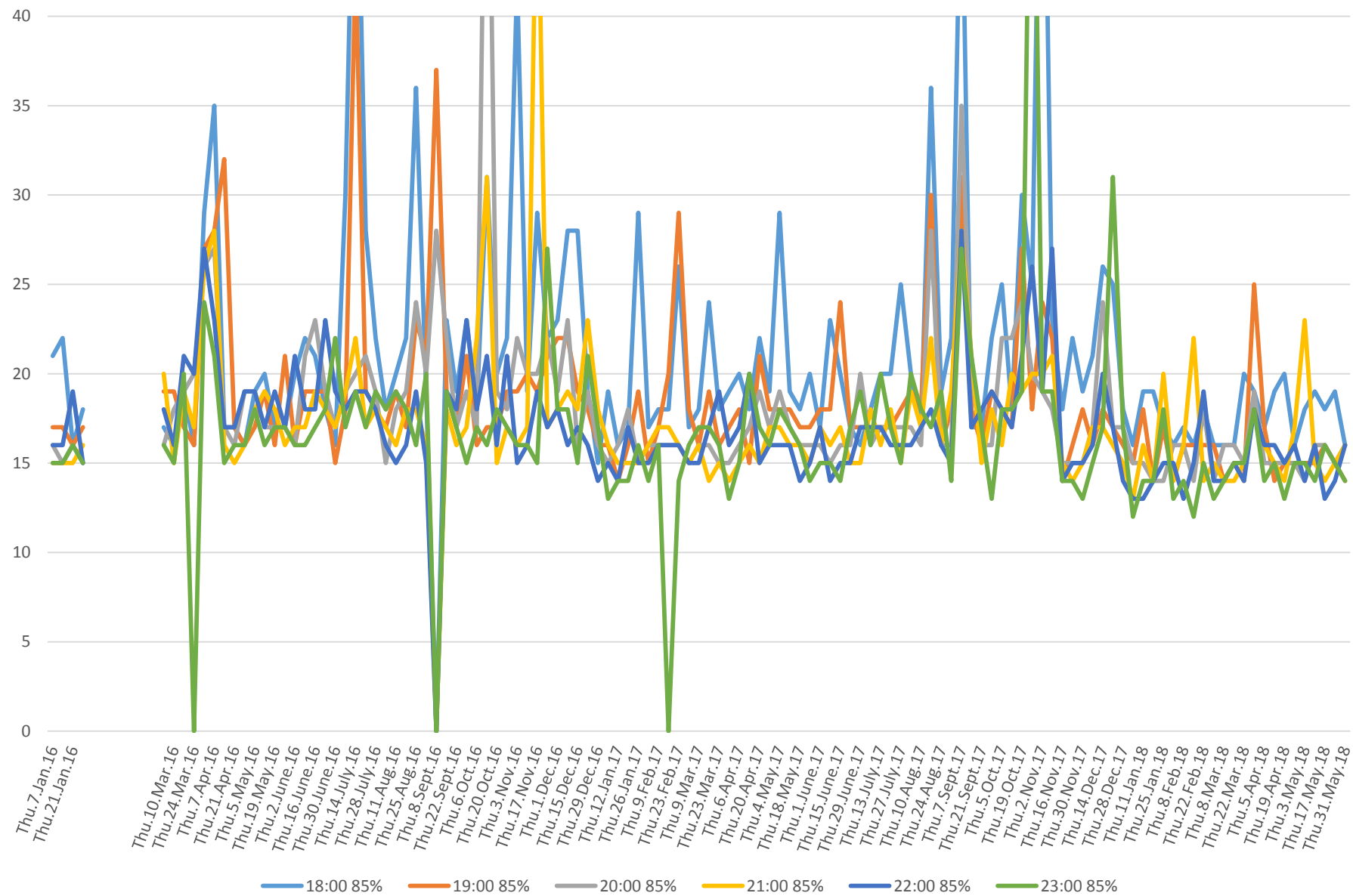
504 King Link Times From Bathurst To Jarvis Eastbound From Jan 2016 To May 2018 85th Percentile Thursday Evenings
