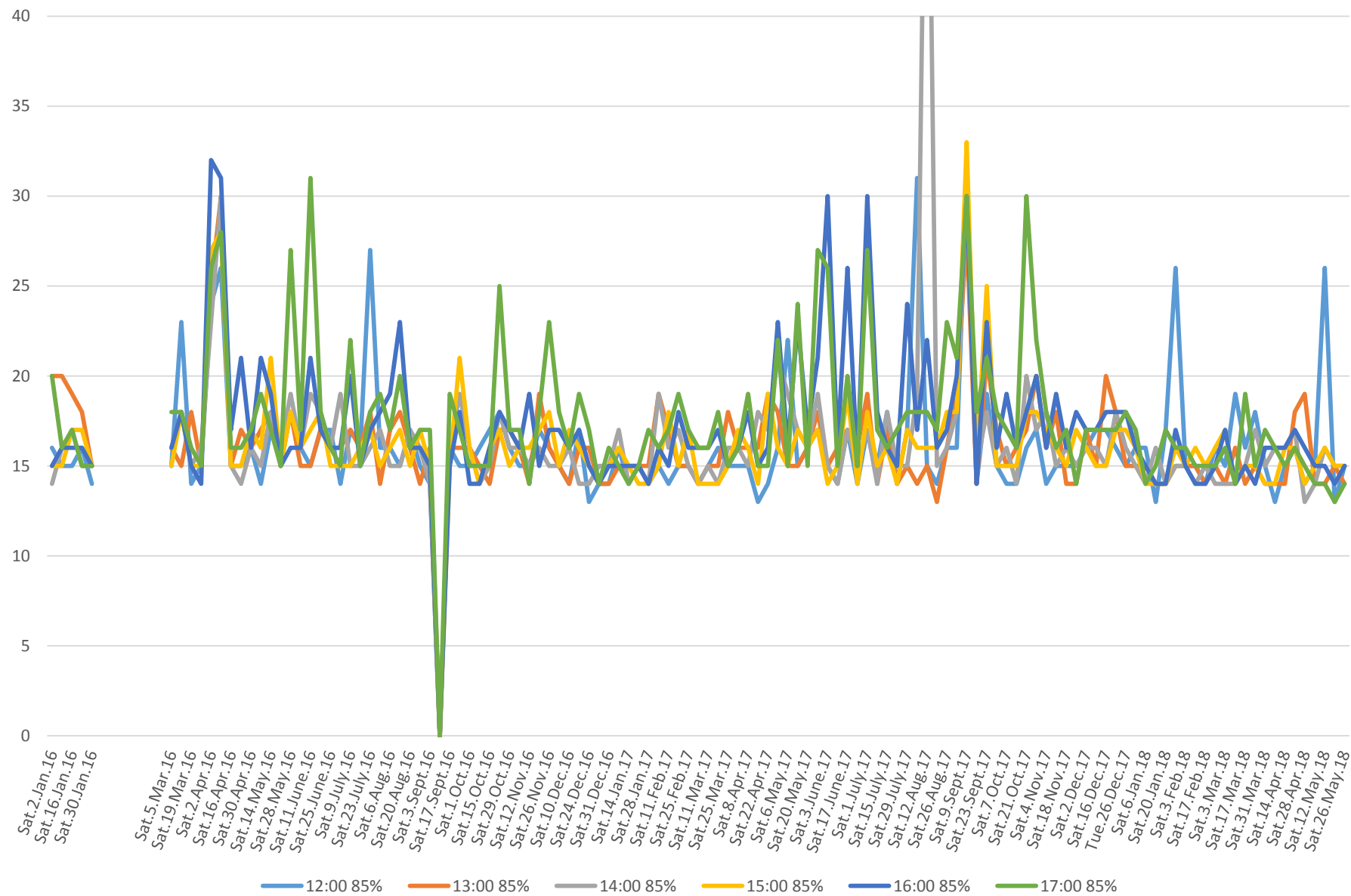
504 King Link Times From Bathurst To Jarvis Eastbound From Jan 2016 To May 2018 85th Percentile Saturday Afternoons
