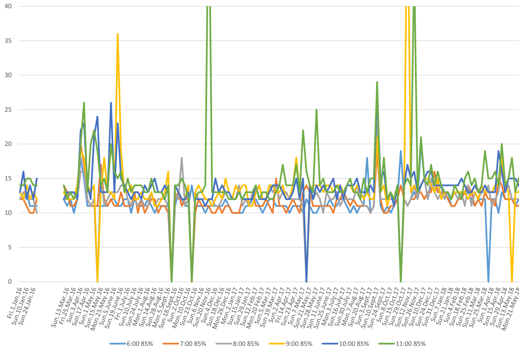
504 King Link Times From Bathurst To Jarvis Eastbound From Jan 2016 To May 2018 85th Percentile Sunday/HolidayMornings
