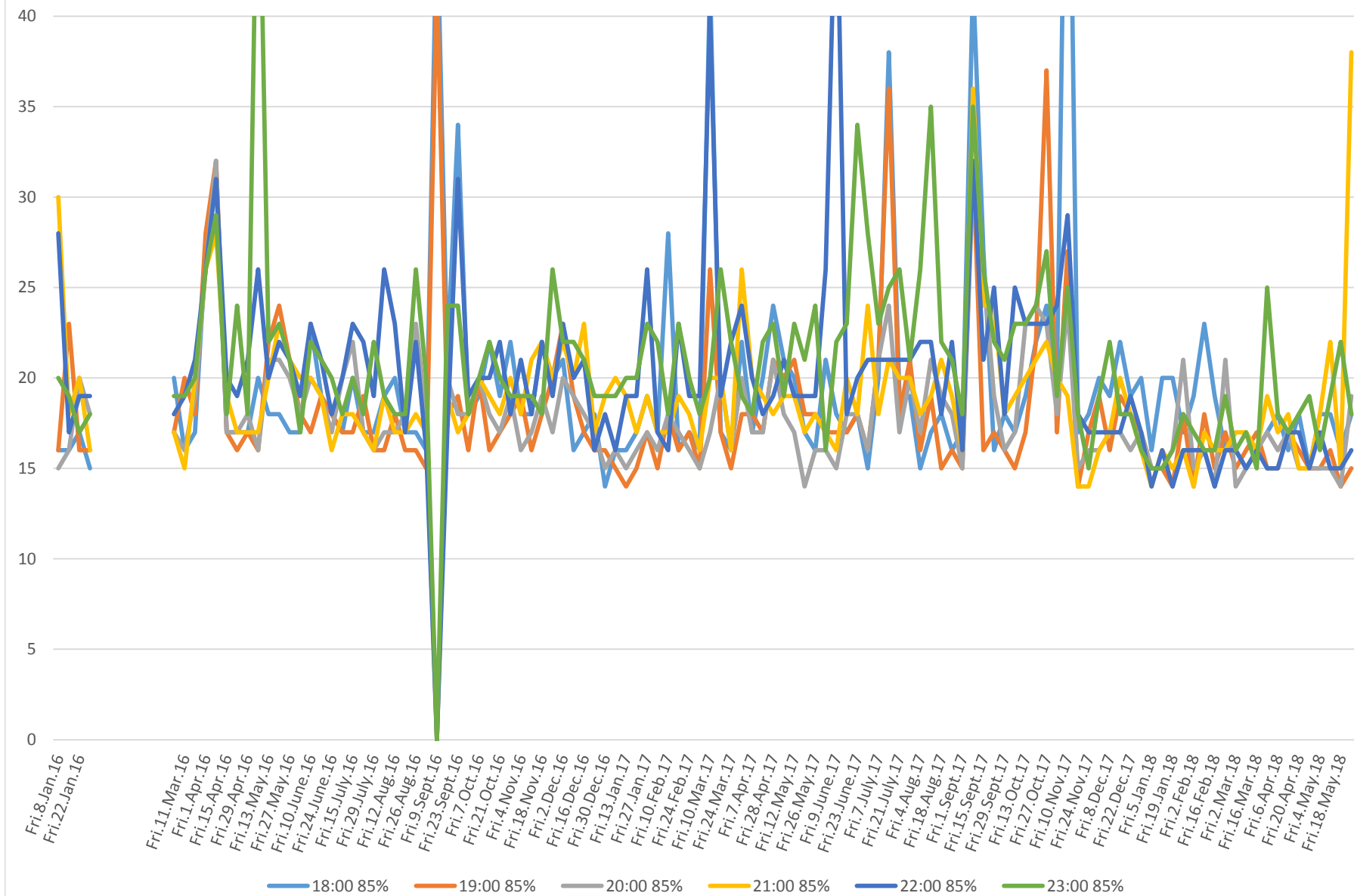
504 King Link Times From Bathurst To Jarvis Eastbound From Jan 2016 To May 2018 85th Percentile Friday Evenings
