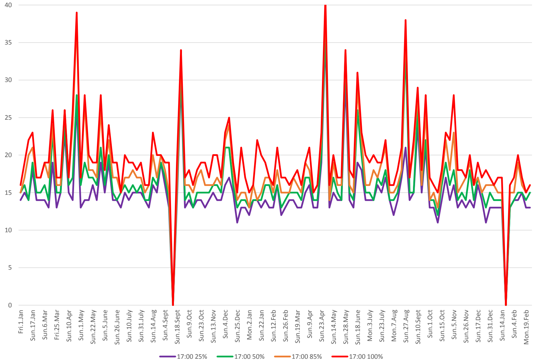
504 King Travel Times Jarvis to Bathurst Westbound 2016 to 2018 5:00 to 6:00 pm Sundays
