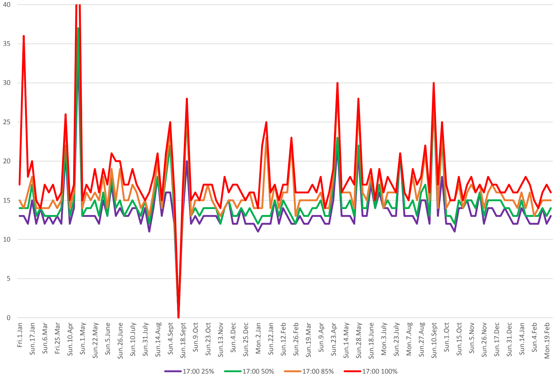
504 King Travel Times Bathurst to Jarvis Eastbound 2016 to 2018 5:00 to 6:00 pm Sundays
