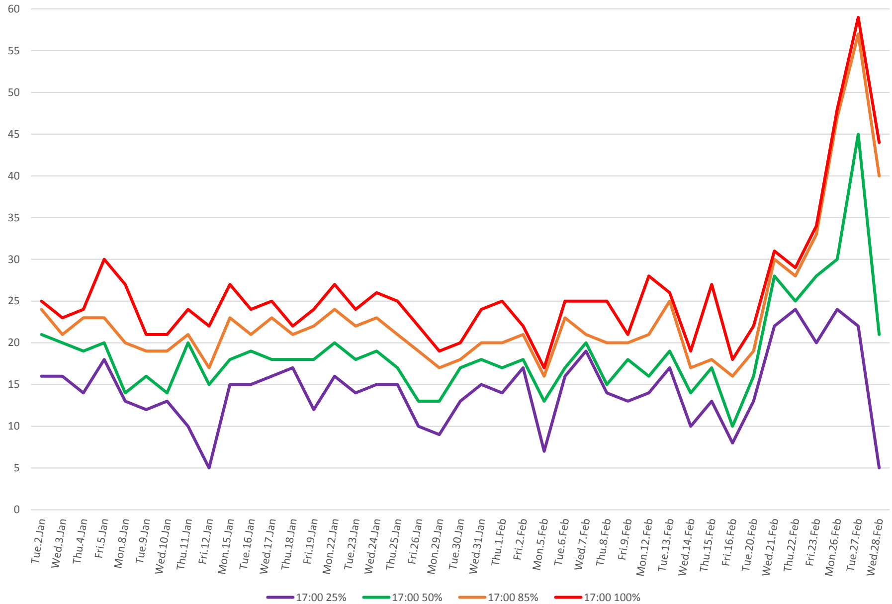
501 Queen Terminal Time at Long Branch Loop 2018 Percentiles 1700 to 1800
