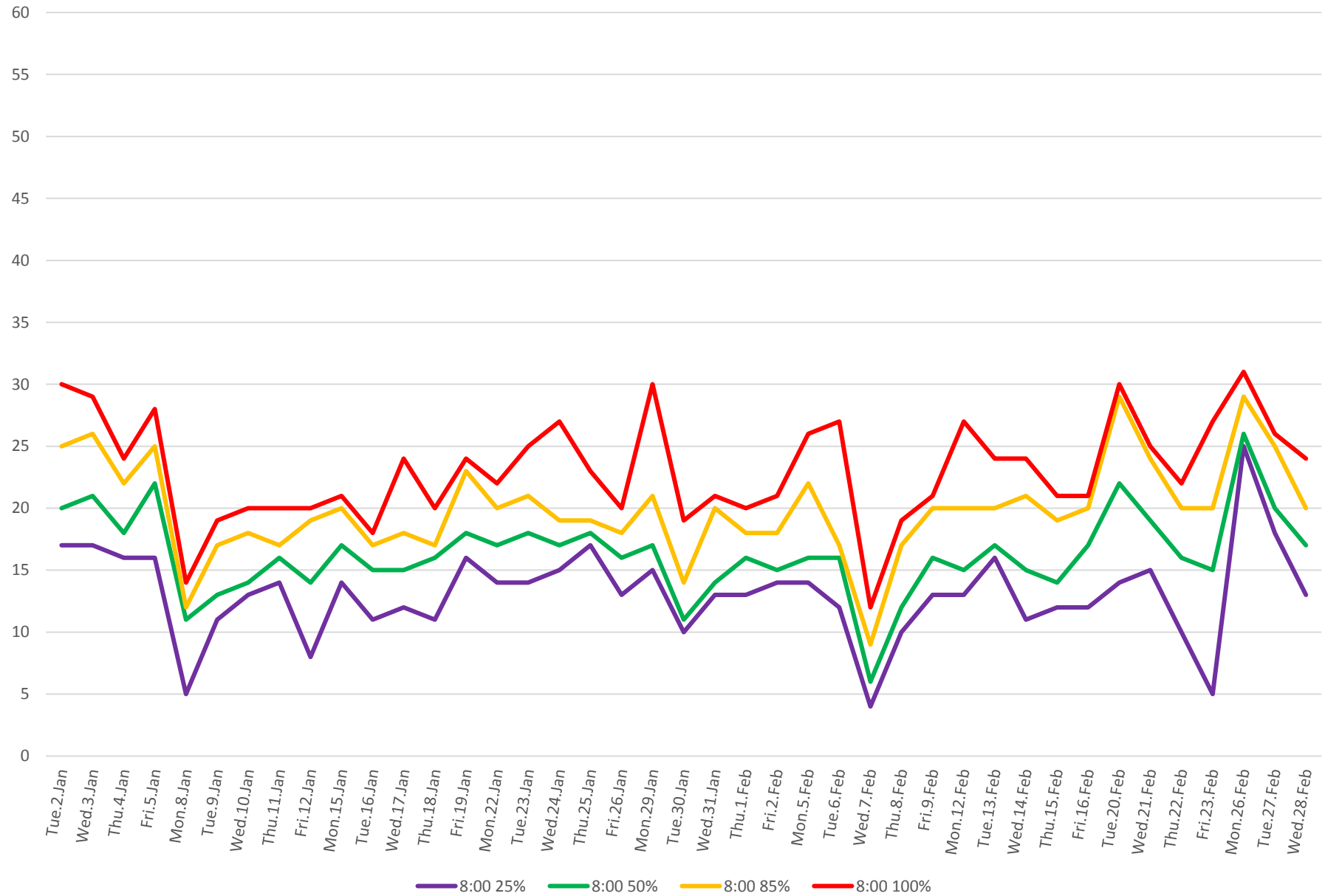
501 Queen Terminal Time at Long Branch Loop 2018 Percentiles 0800 to 0900
