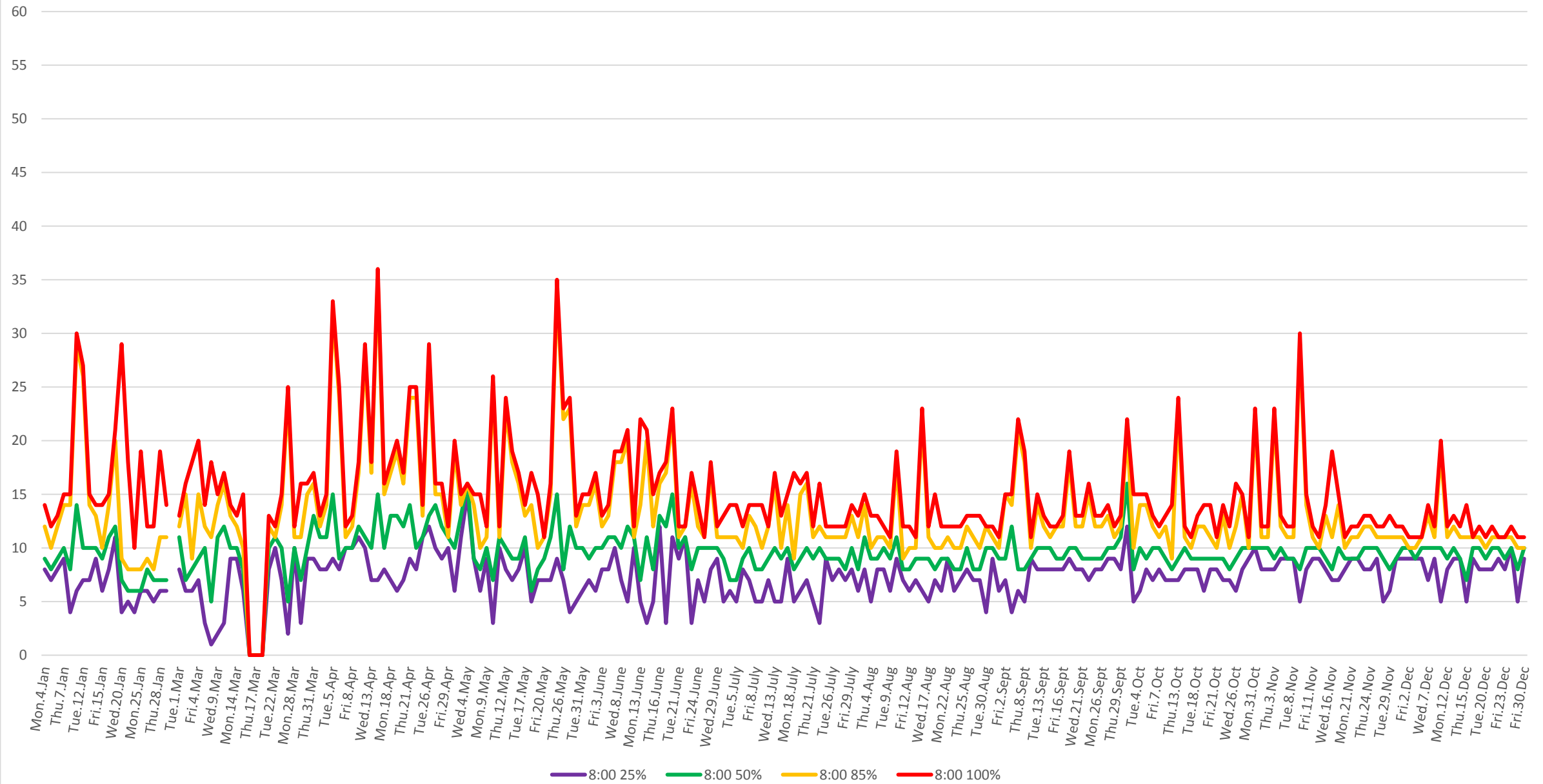
501 Queen Headways at Long Branch Loop Eastbound 2016 Percentiles 0800 to 0900
