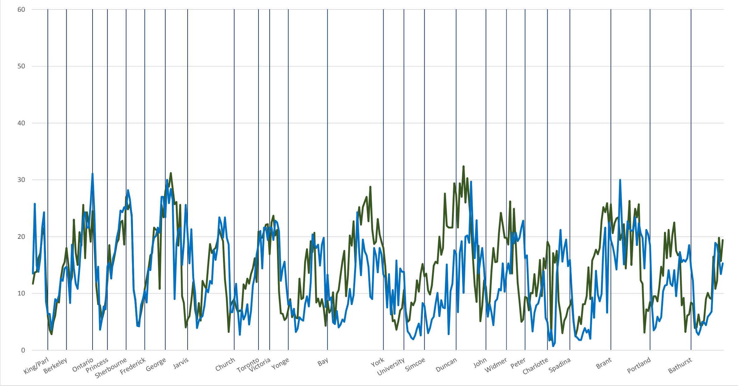
504 King Eastbound Oct 23-27 (Blue) vs Nov 13-17 (Green) 2017 Average Speed 1400 to 1500
