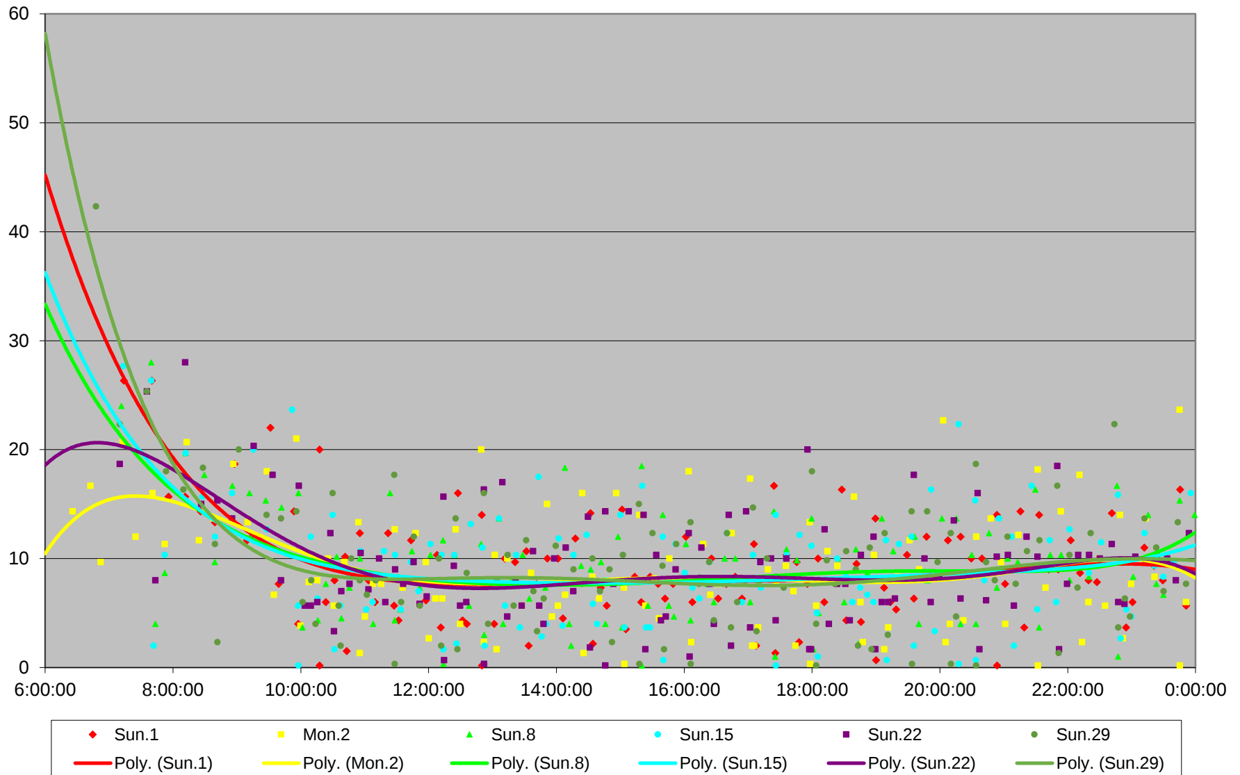
54 Lawrence East Headways at Kennedy Westbound January 2017
