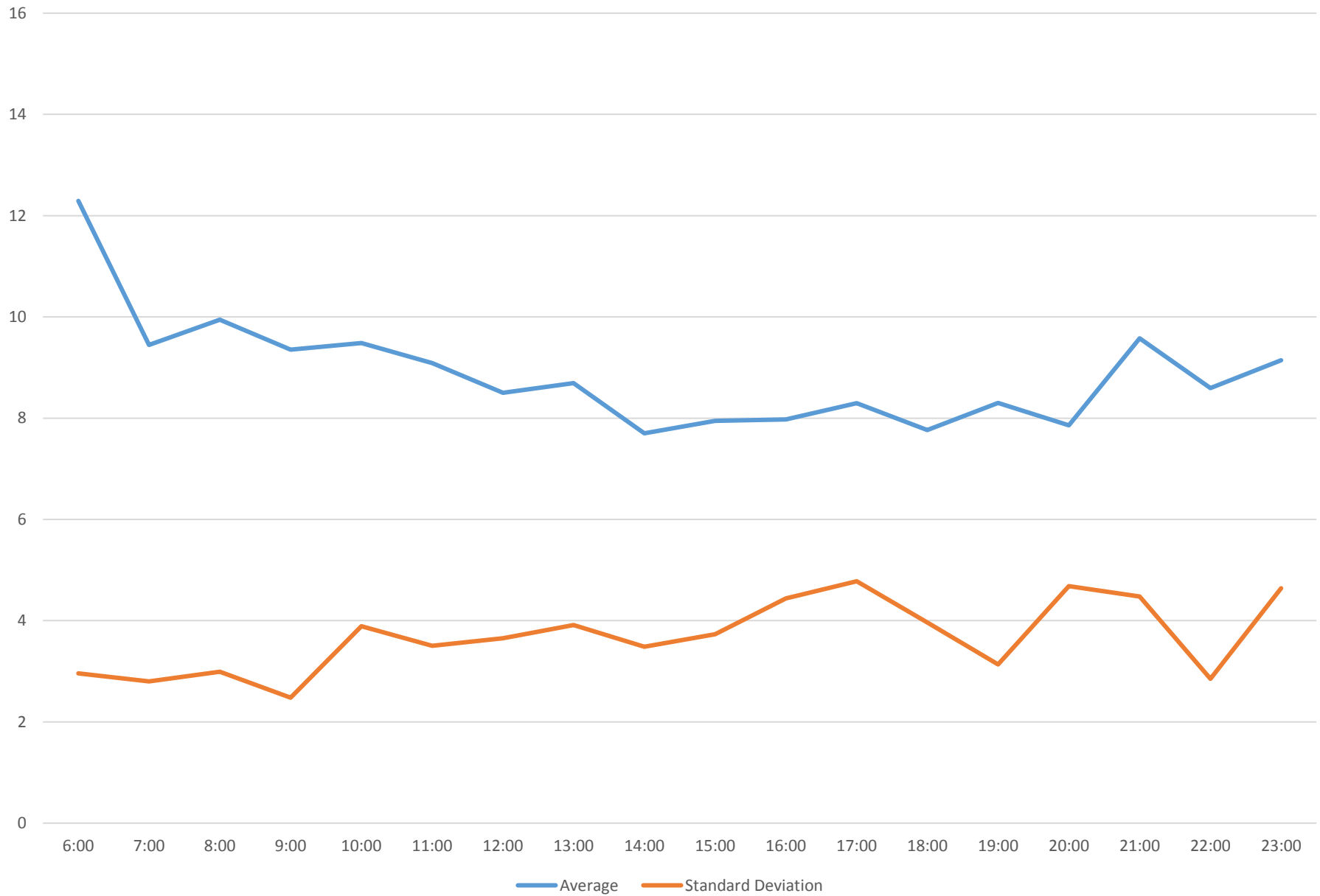
54 Lawrence East Headways at Kennedy Westbound January 2017 Saturday Statistics
