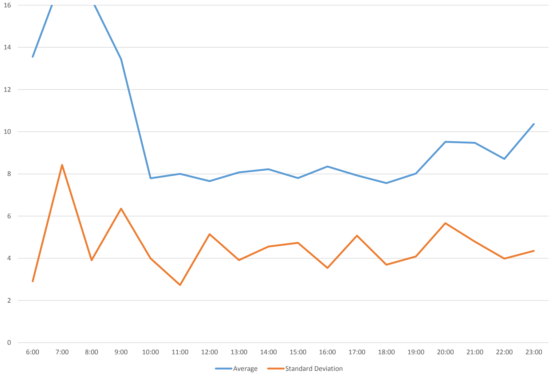
54 Lawrence East Headways at Kennedy Westbound January 2017 Sunday Statistics
