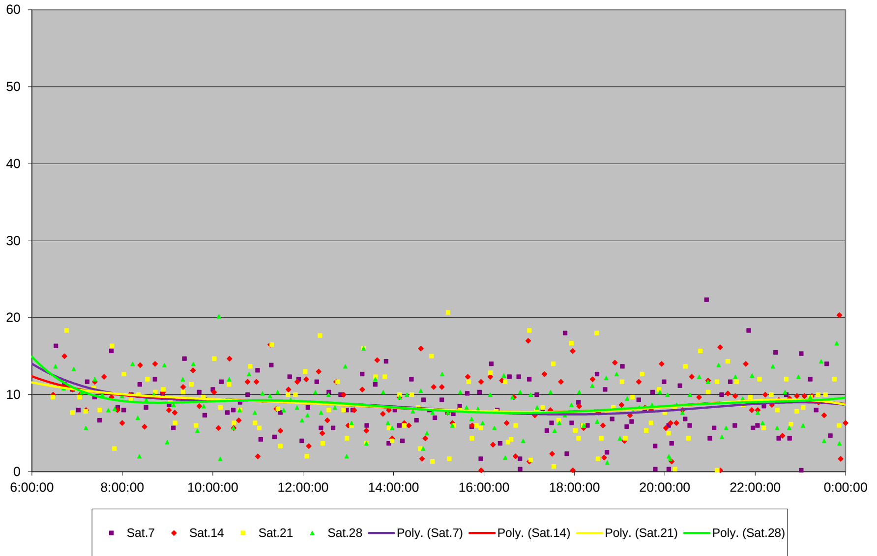
54 Lawrence East Headways at Kennedy Westbound January 2017
