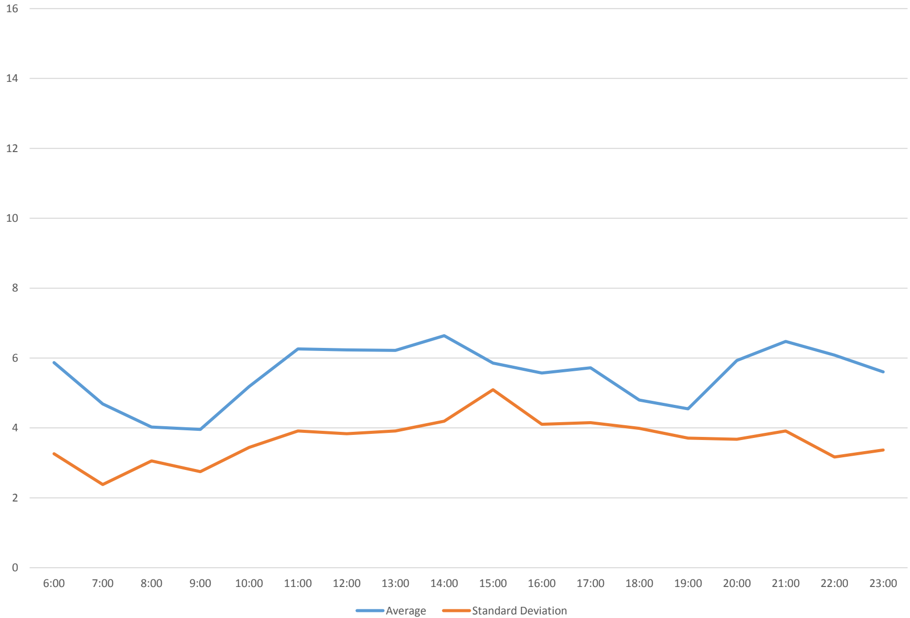
54 Lawrence East Headways at Kennedy Westbound January 2017 Weekday Statistics
