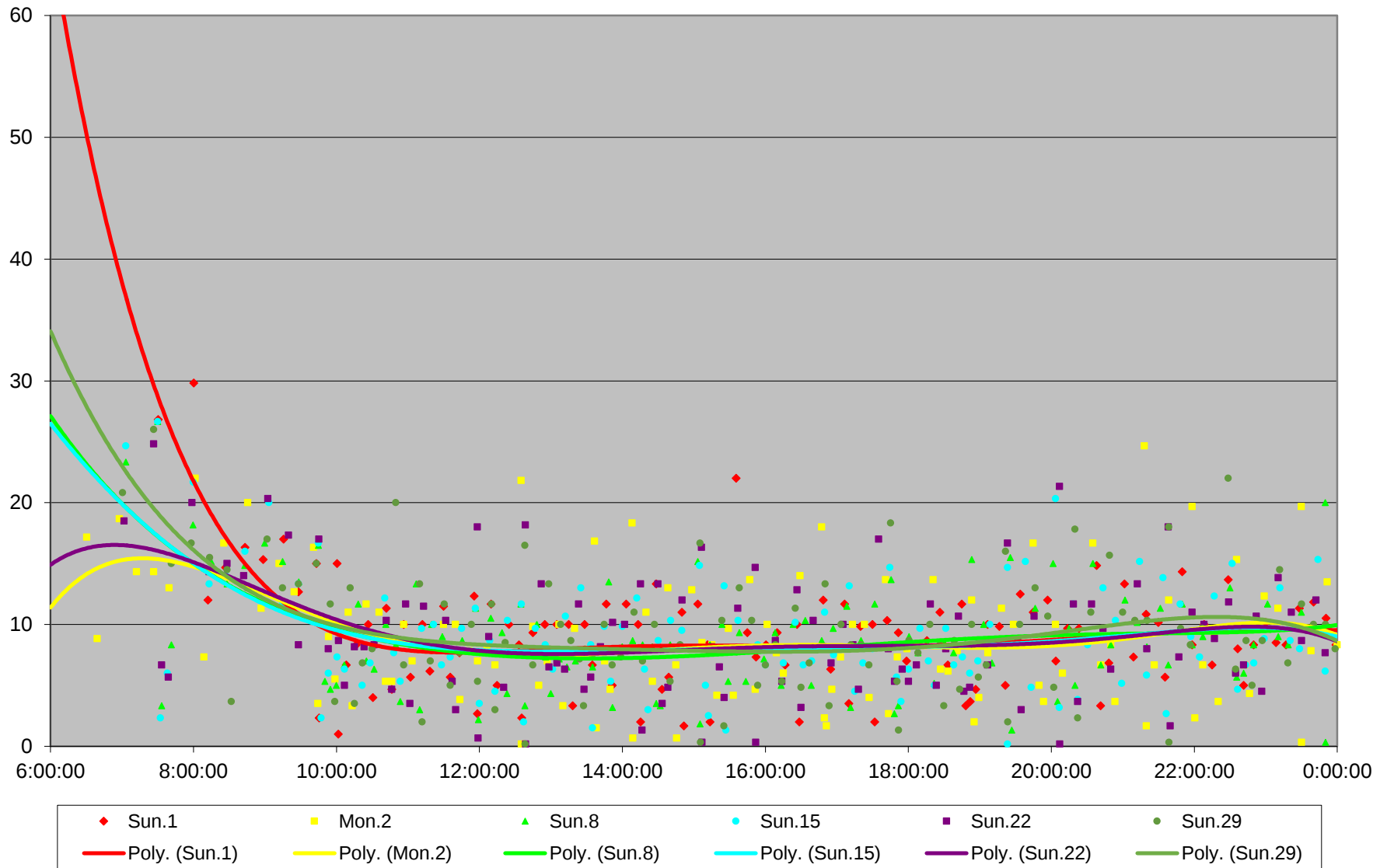
54 Lawrence East Headways at Markham Road Westbound January 2017
