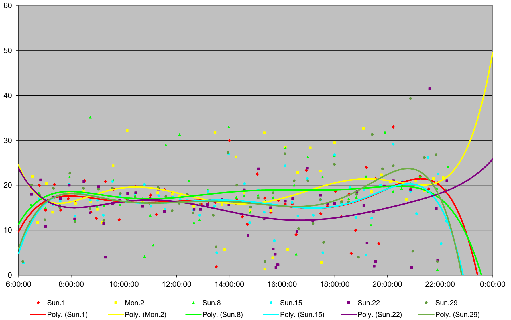
39 Finch East Headways at West of Littles Road Westbound January 2017
