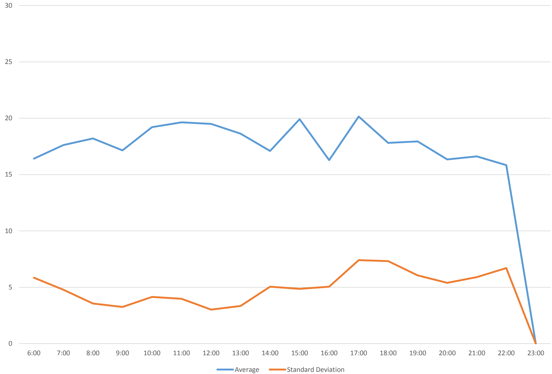
39 Finch East Headways at West of Littles Road Westbound January 2017 Weekday Statistics
