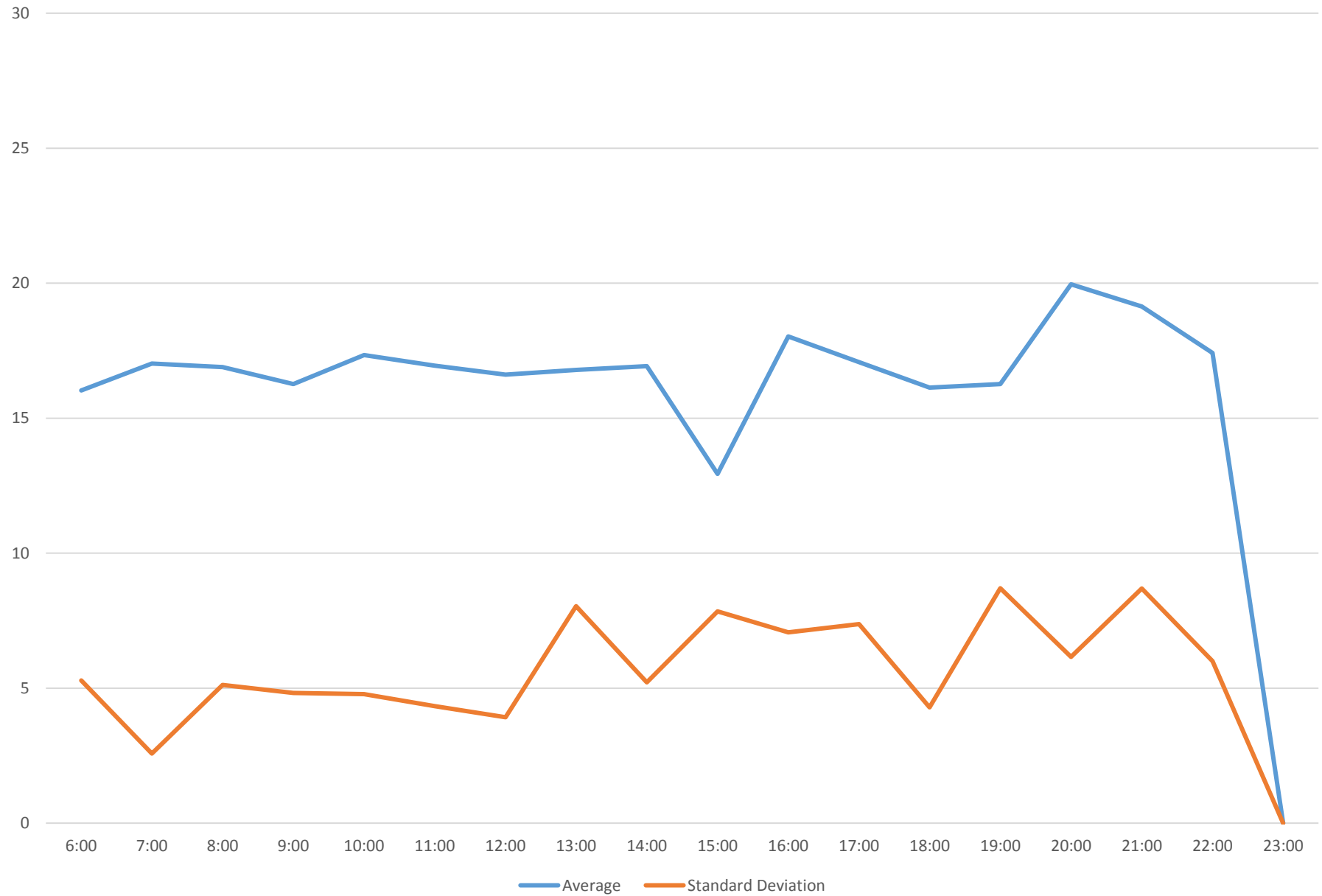
39 Finch East Headways at West of Littles Road Westbound January 2017 Sunday Statistics
