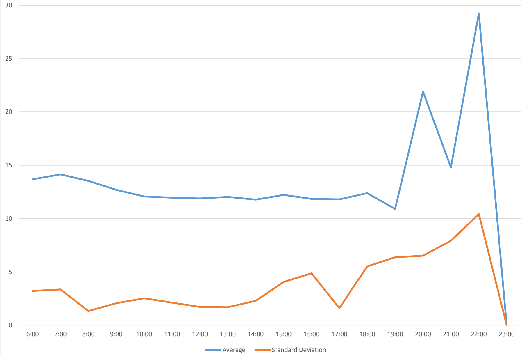
39 Finch East Headways at West of Littles Road Westbound January 2017 Saturday Statistics
