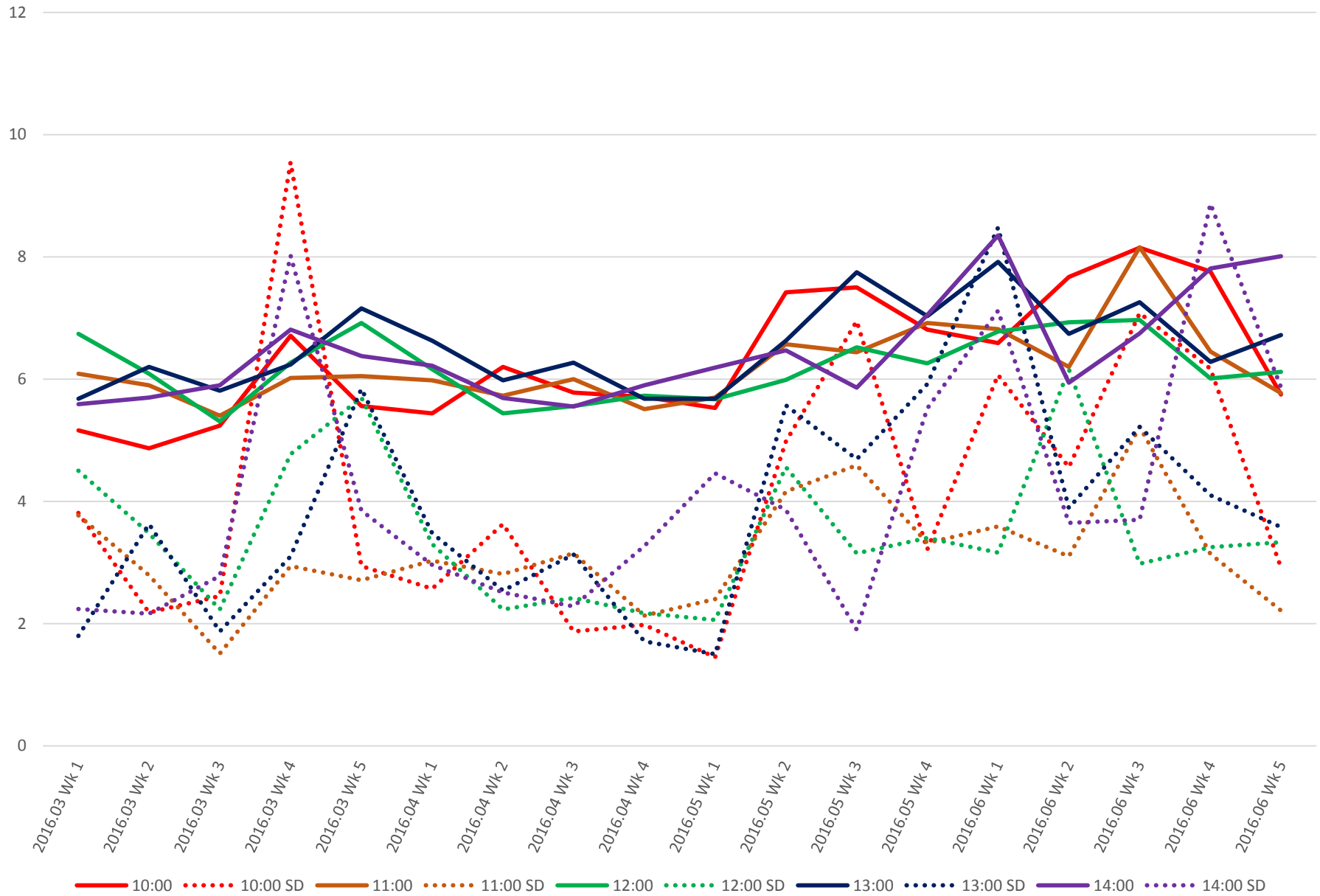
501 Queen Headways at Silver Birch Ave. Westbound Midday
