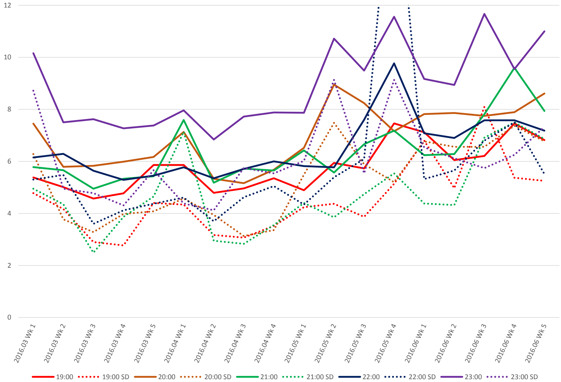
501 Queen Headways at Silver Birch Ave. Westbound Evening
