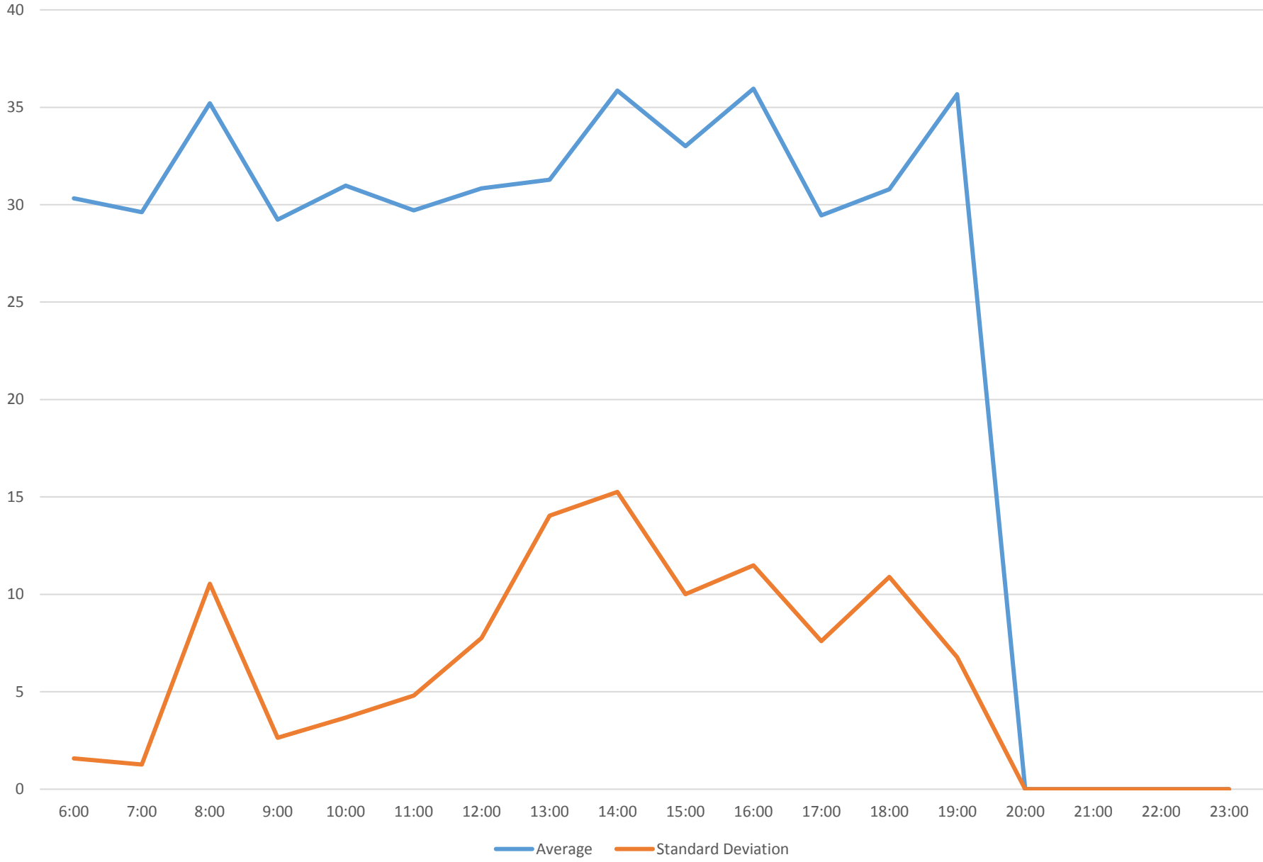
96 Wilson Headways at Thistle Down Loop Northbound September 2015 Sunday Statistics
