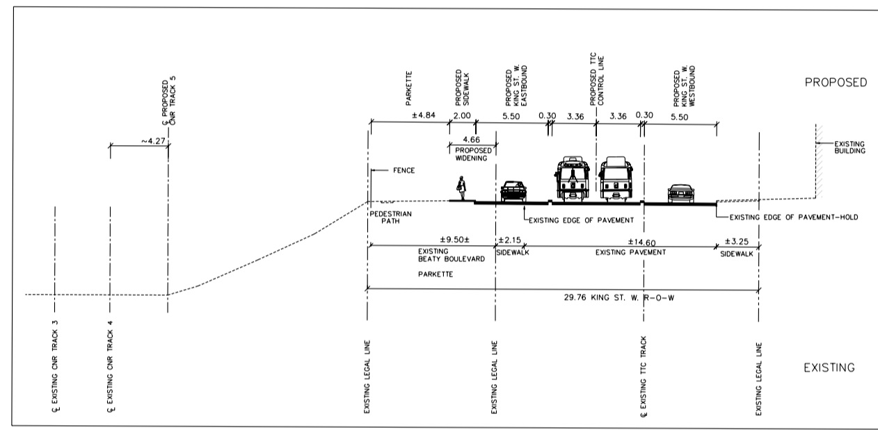
SECTION C-C
