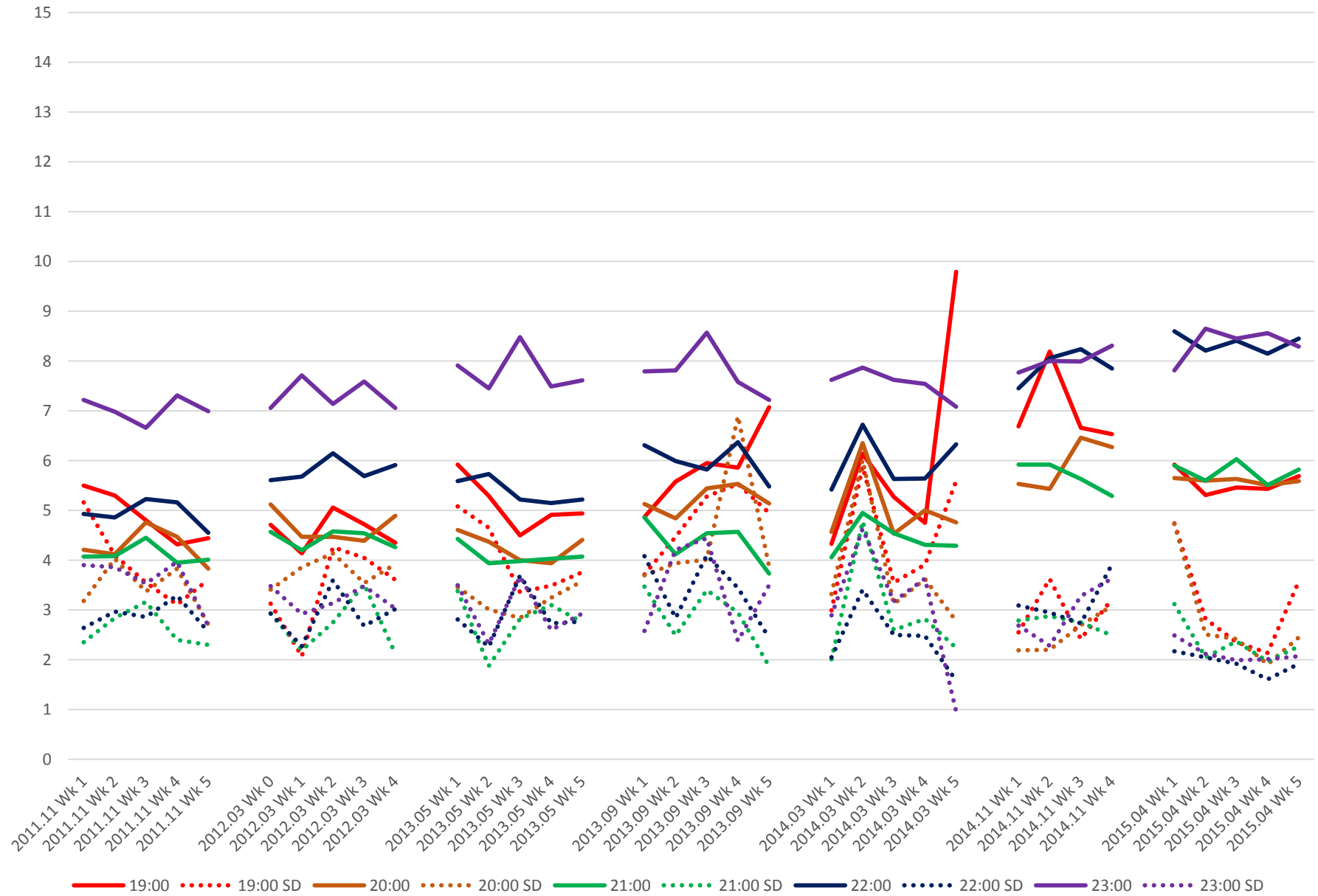
29 Dufferin Headways at Transit Road Southbound Evening
