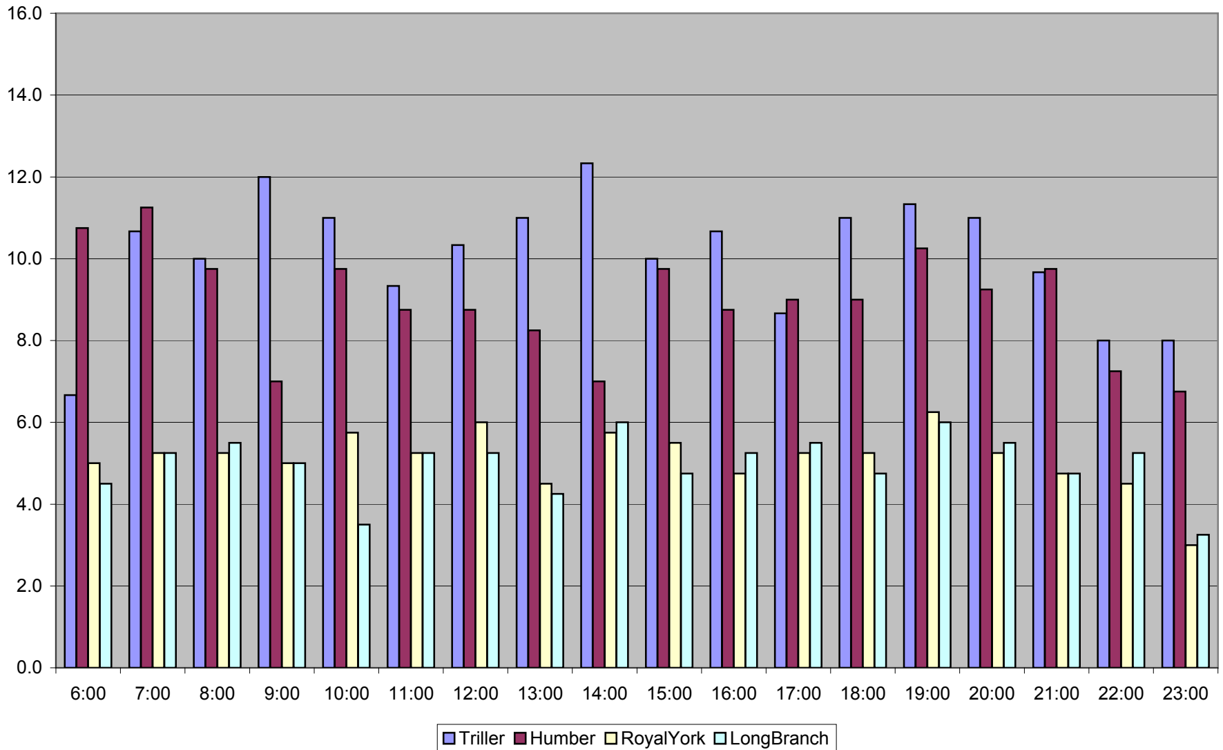
Cars/Hour Comparisons on West Queen 501 Westbound November 2011 Mondays
