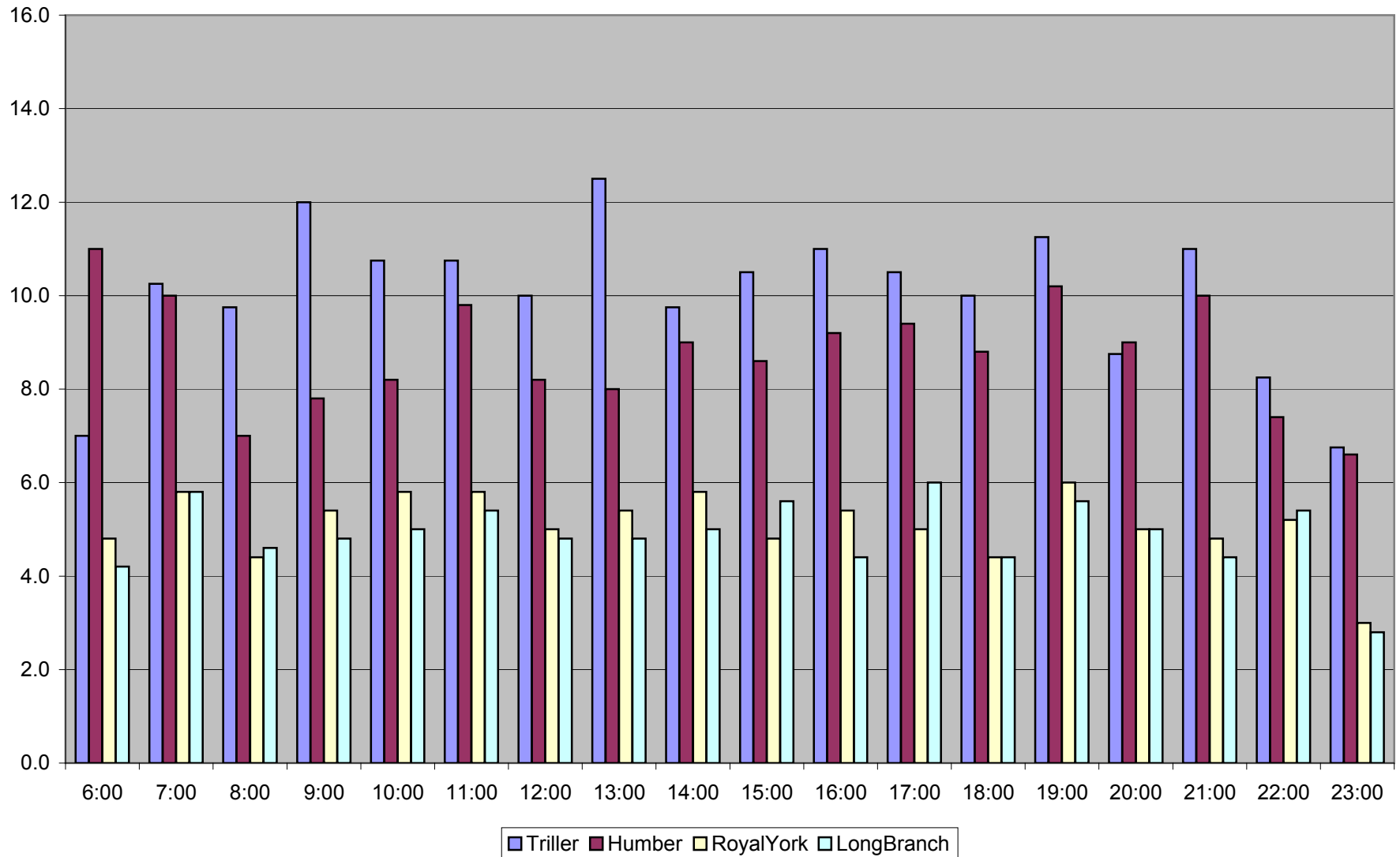
Cars/Hour Comparisons on West Queen 501 Westbound November 2011 Wednesdays
