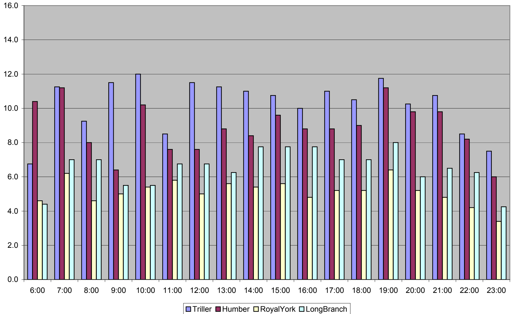
Cars/Hour Comparisons on West Queen 501 Westbound November 2011 Tuesdays
