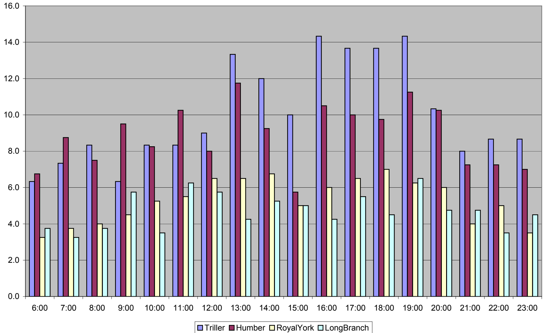
Cars/Hour Comparisons on West Queen 501 Westbound November 2011 Saturdays
