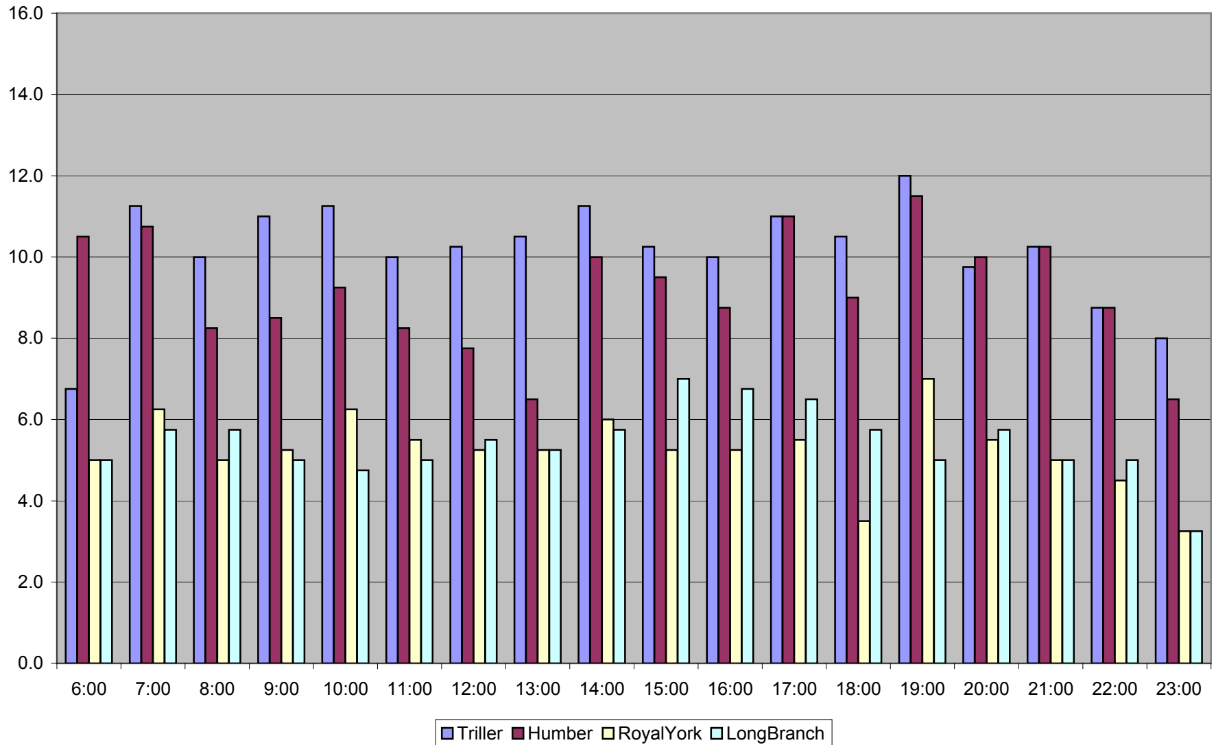
Cars/Hour Comparisons on West Queen 501 Westbound November 2011 Week 1
